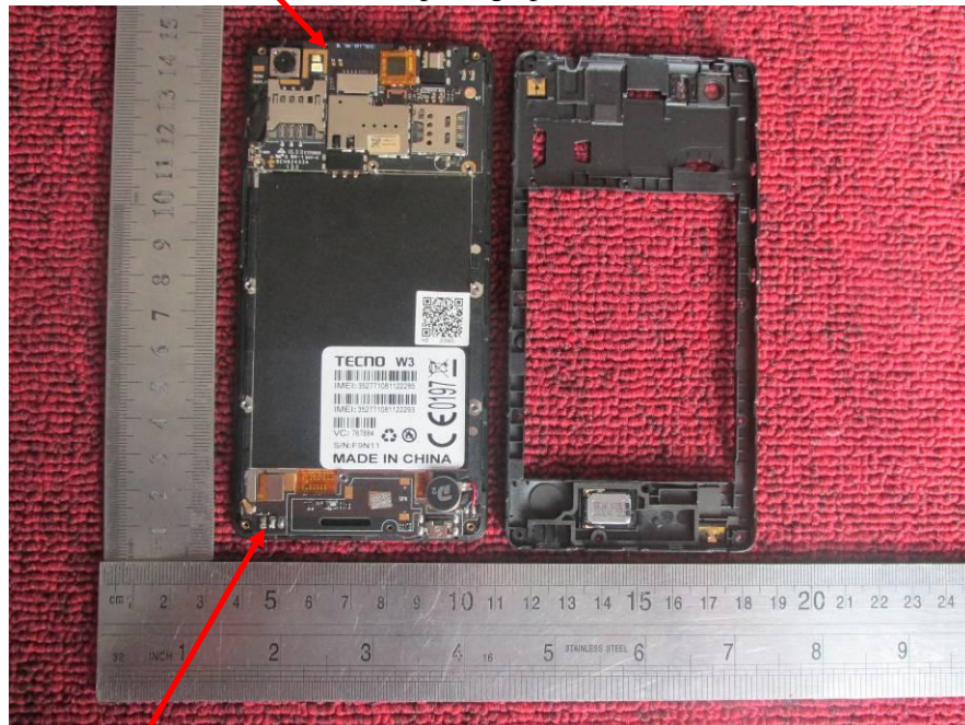
GSM/2/3G Antenna
