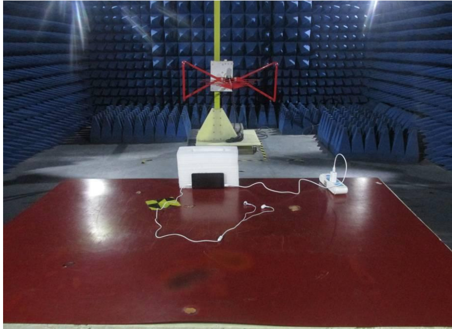
RADIATED EMISSION TEST (From frequency 30MHz to 1GHz)
