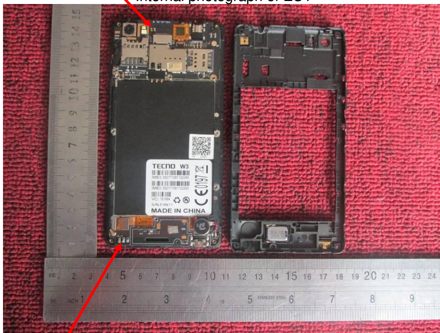
GSM/2/3G Antenna
