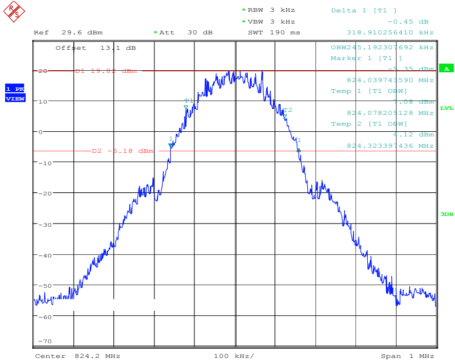
Occupied Bandwidth (99% and -26dBc) GSM 850 BAND CH 128
