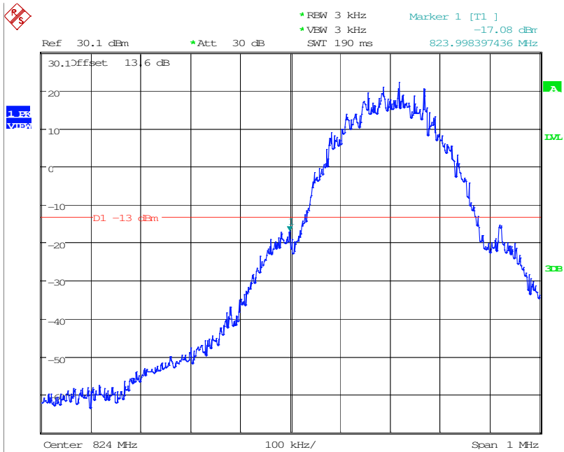
Low Band Edge GSM 850 BAND CH 128
