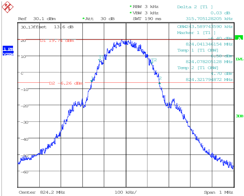
Occupied Bandwidth (99% and -26dBc) GSM 850 BAND CH 128
