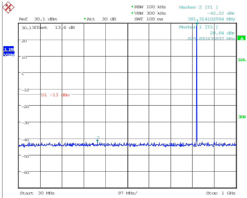
CONDUCTED EMISSION IN GSM850 BAND Conducted Emission Transmitting Mode CH 128 30MHz – 1GHz
