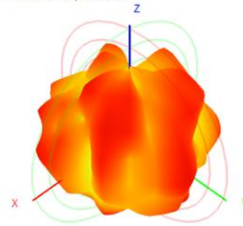
5850.0MHz H+V, Ef: 42.8%
