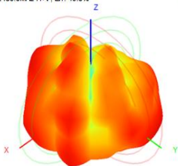
2450.0MHz H+V, Ef: 48.5%
