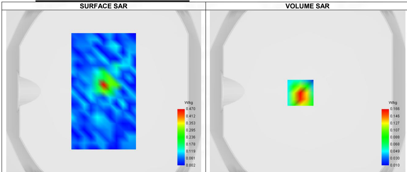
Maximum location: X=-8.00, Y=8.00 ; SAR Peak: 0.046 W/kg
