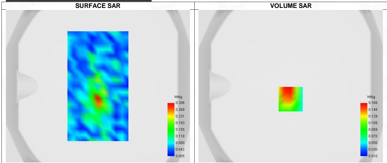
Maximum location: X=0.00, Y=-17.00 ; SAR Peak: 0.23 W/kg
