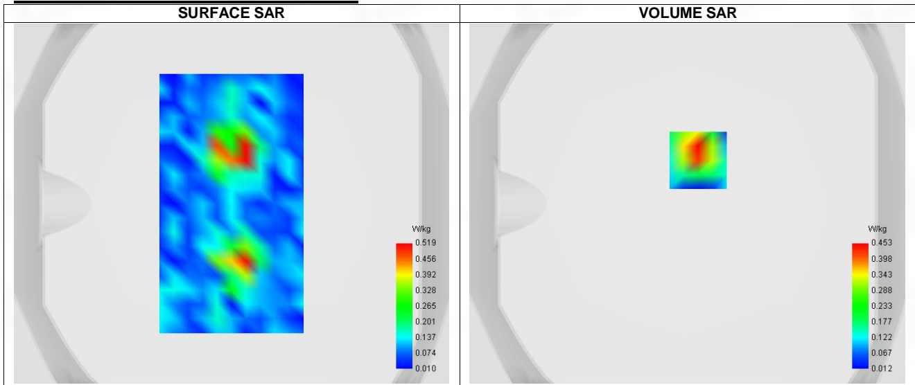
Maximum location: X=6.00, Y=24.00 ; SAR Peak: 0.74 W/kg
