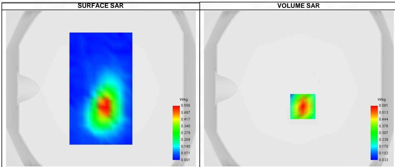
Maximum location: X=5.00, Y=-23.00 ; SAR Peak: 0.89 W/kg
