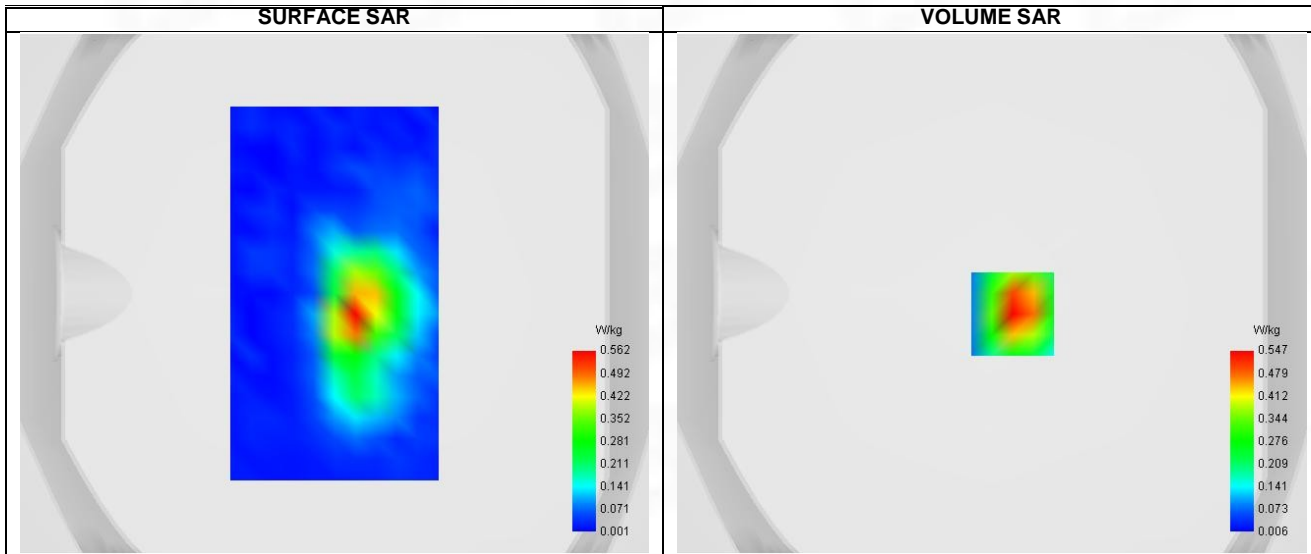
Maximum location: X=8.00, Y=-8.00 ; SAR Peak: 1.09 W/kg
