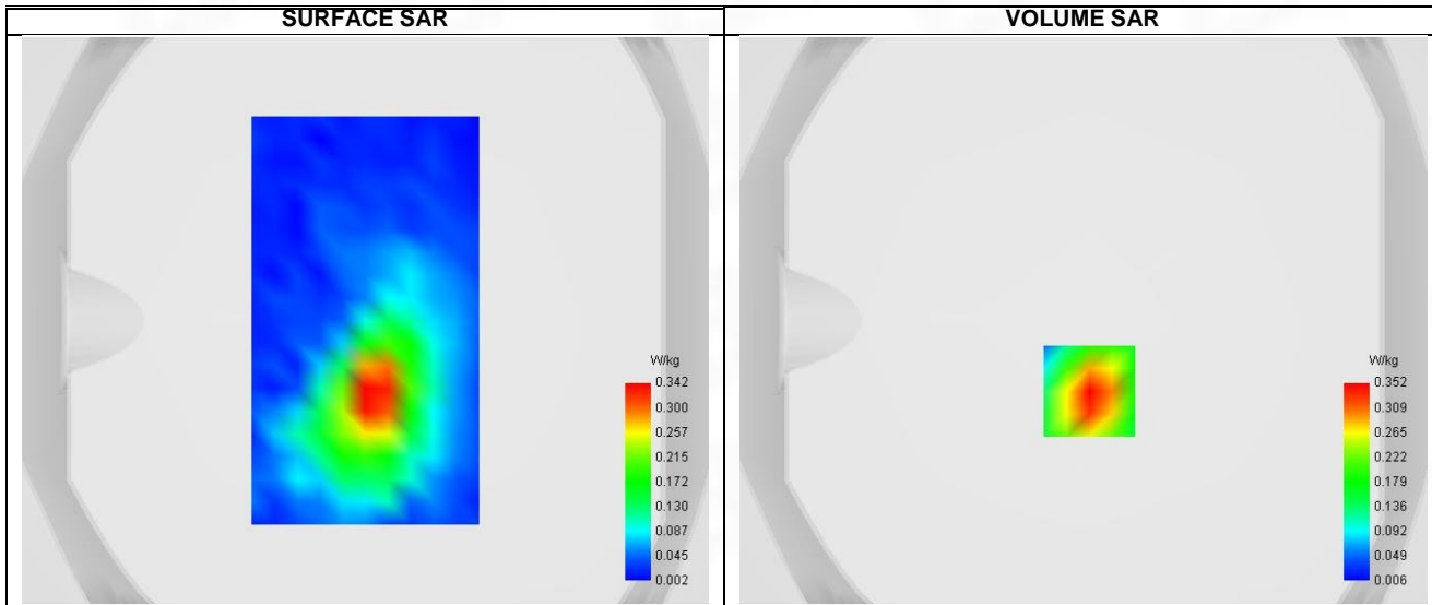
Maximum location: X=2.00, Y=-25.00 ; SAR Peak: 0.54 W/kg
