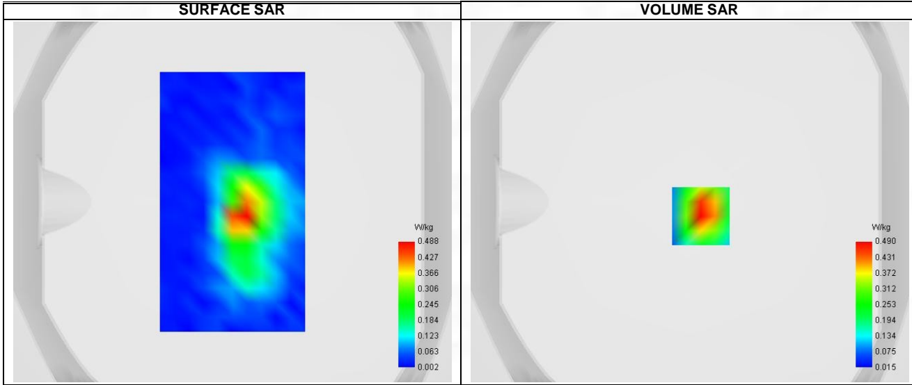
Maximum location: X=6.00, Y=-8.00 ; SAR Peak: 0.97 W/kg
