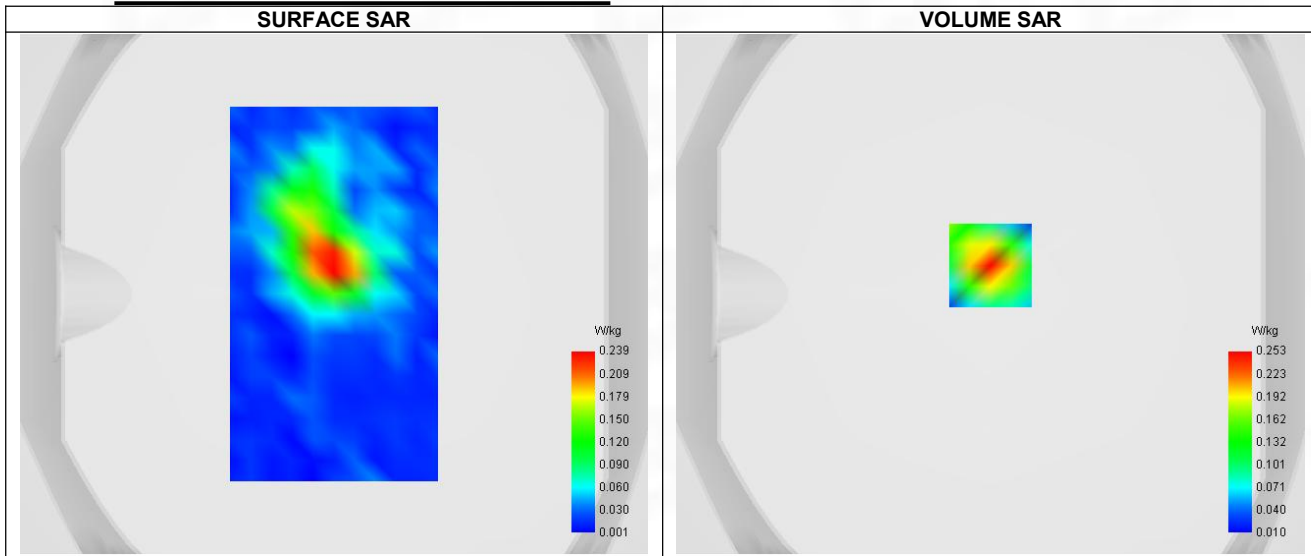
Maximum location: X=0.00, Y=11.00 ; SAR Peak: 0.47 W/kg
