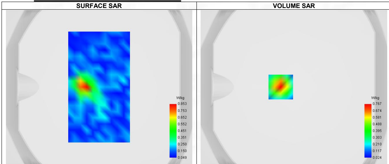
Maximum location: X=-17.00, Y=0.00 ; SAR Peak: 1.10 W/kg
