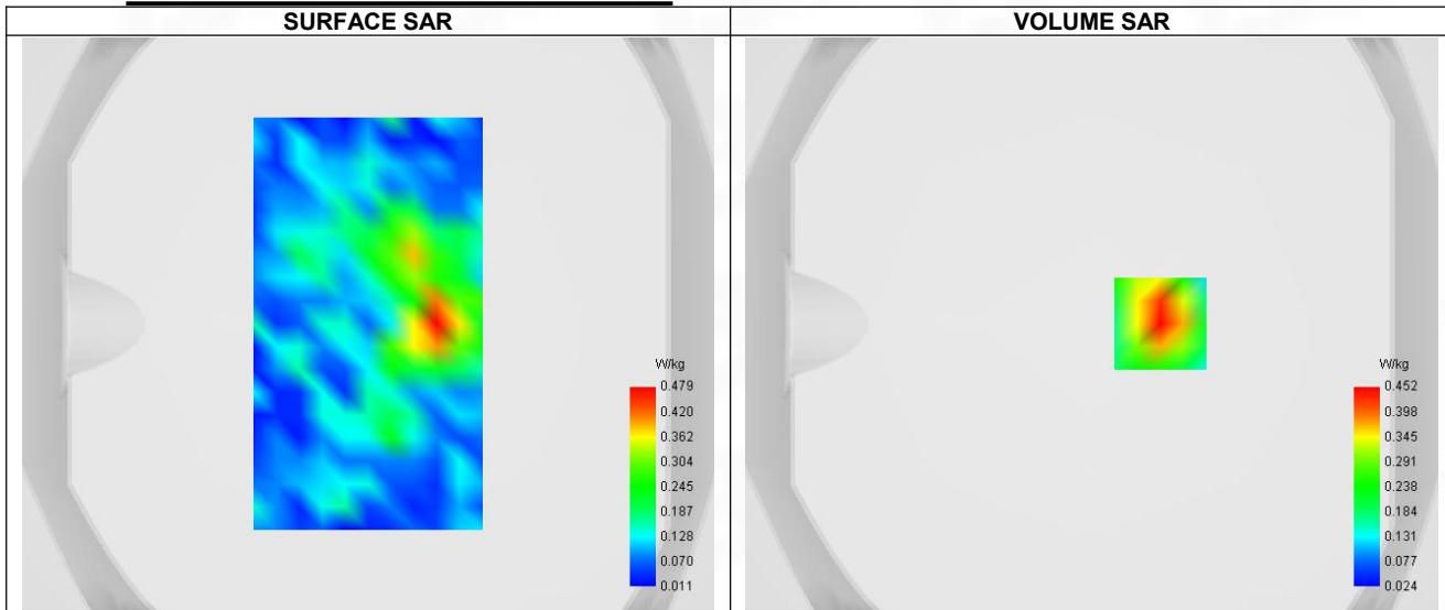
Maximum location: X=24.00, Y=0.00 ; SAR Peak: 0.70 W/kg
