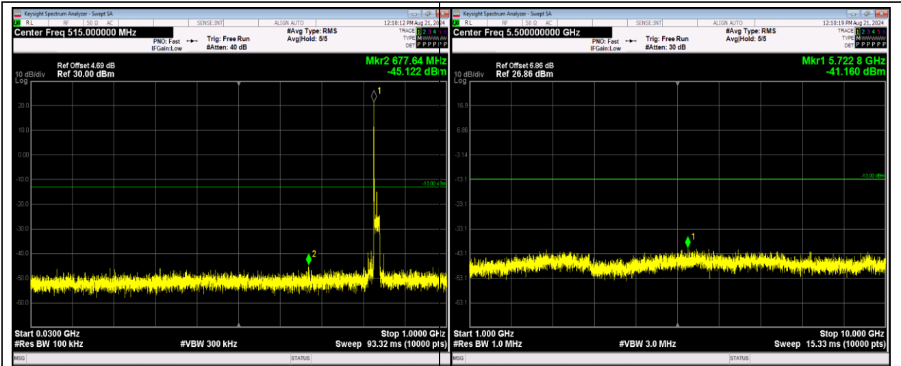
Band26-15MHz-64QAM-26965-1RB#0-Range1:30 ~1000MHz
