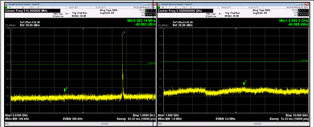
Band13-5MHz-64QAM-23230-1RB#0-Range1:30~1000MHz
