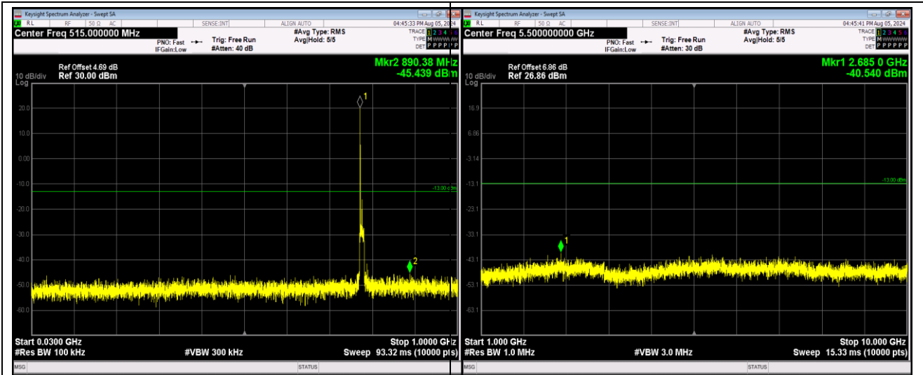
Band13-10MHz-64QAM-23230-1RB#0-Range1:30~1000MHz
