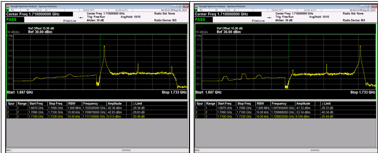
Band66-20MHz-64QAM-132072-100RB#0
