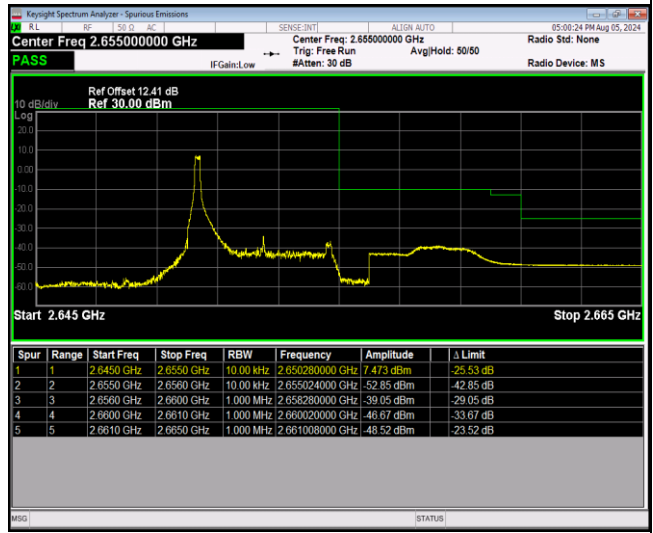
Band41-5MHz-16QAM-41215-25RB#0
