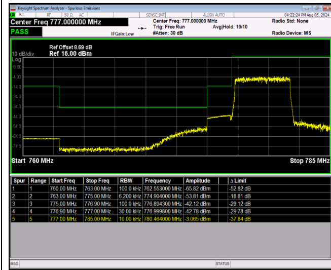
Band13-5MHz-64QAM-23255-1RB#24
