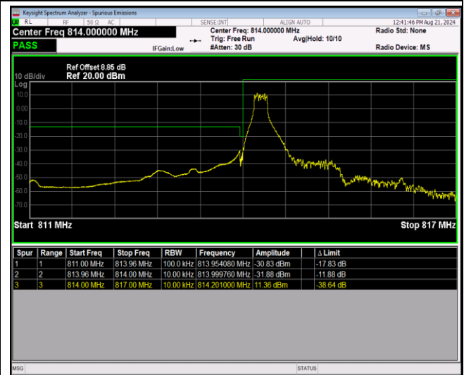
Band26-1.4MHz-64QAM-26697-6RB#0
