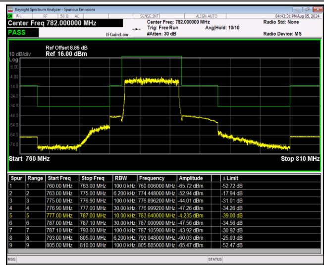
Band13-10MHz-64QAM-23230-1RB#49
