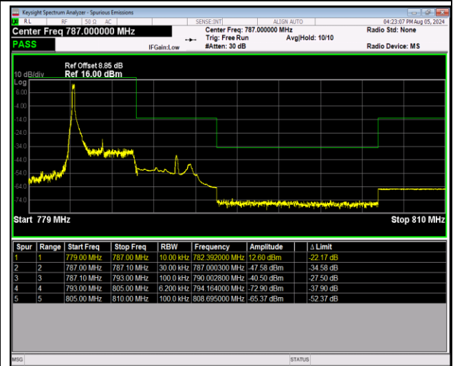
Band13-5MHz-QPSK-23255-25RB#0
