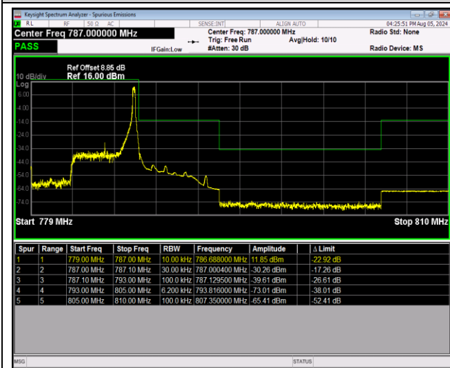
Band13-5MHz-64QAM-23205-1RB#0
