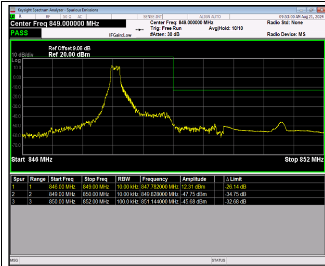
Band26-1.4MHz-16QAM-27033-6RB#0
