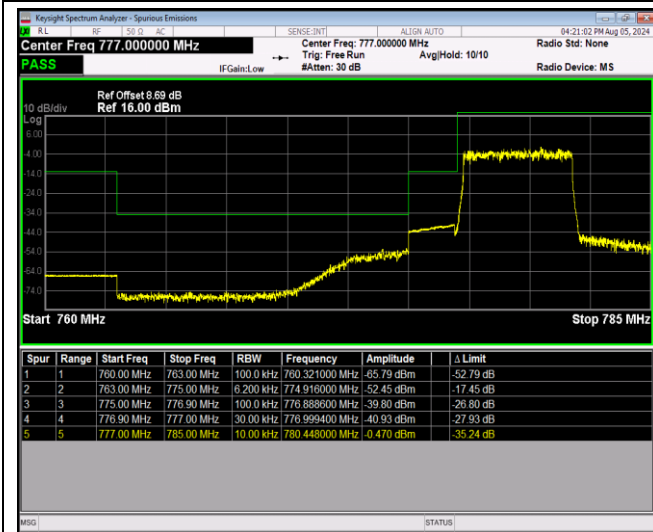
Band13-5MHz-QPSK-23255-1RB#24
