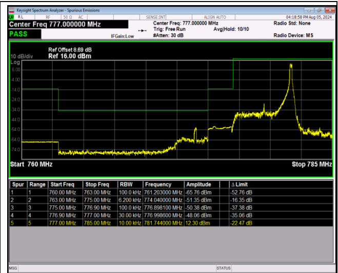
Band13-5MHz-QPSK-23255-1RB#0
