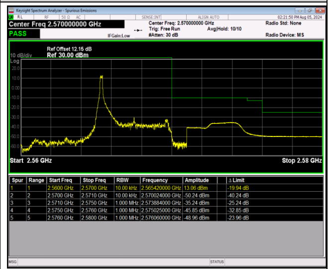
Band7-5MHz-QPSK-27425-25RB#0
