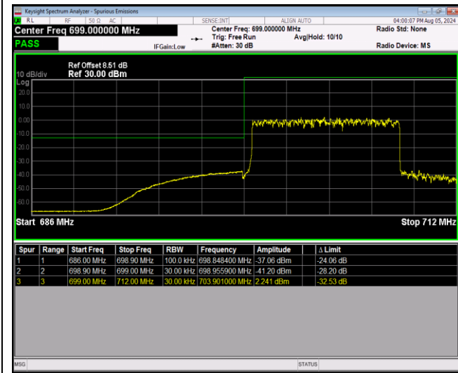
Band12-10MHz-QPSK-23130-1RB#49
