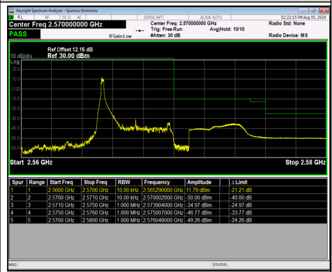
Band7-5MHz-64QAM-21425-25RB#0
