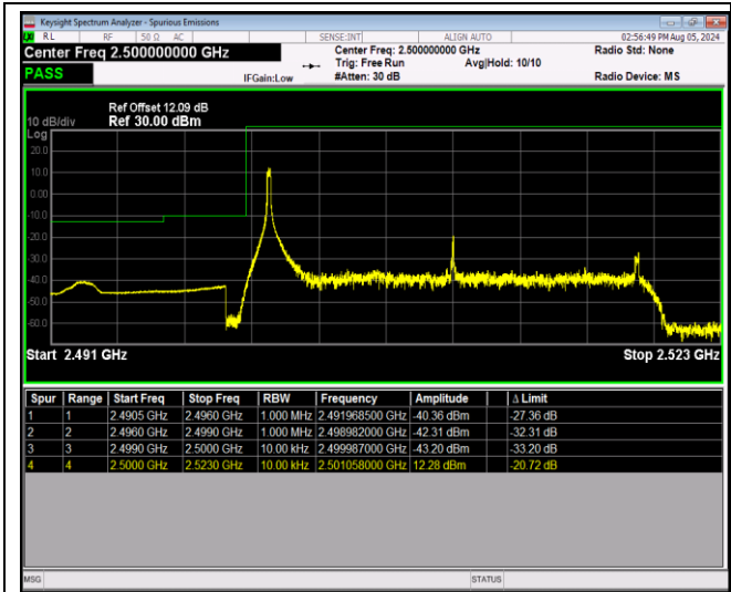
Band7-20MHz-64QAM-20850-100RB#0
