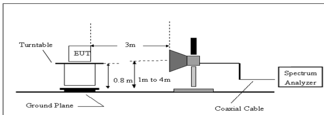
(C) Radiated Emission Test-Up Frequency Above 1GHz
