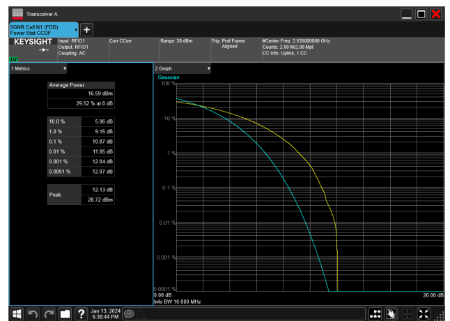
10MHz_15kHz_2535MHz_CP-OFDM 64 QAM_RB52@0&10.87 dB
