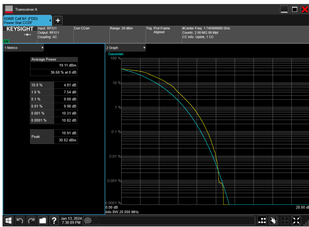
15MHz_15kHz_1745MHz_DFT-s-OFDM 16 QAM_RB75@0&9.08 dB
