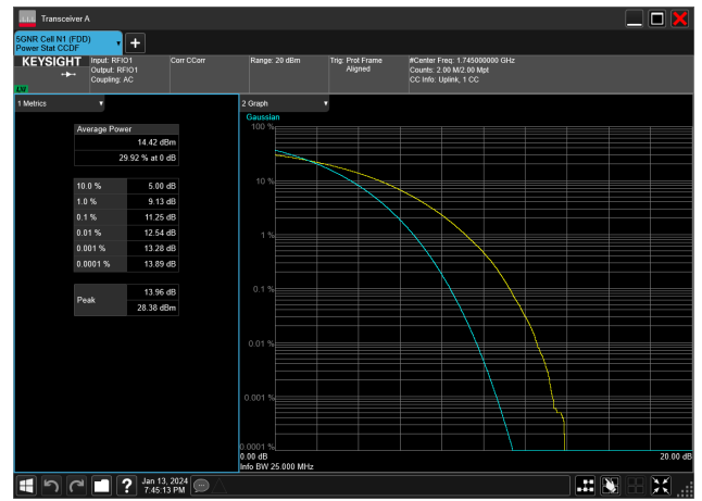
25MHz_15kHz_1745MHz_CP-OFDM 256 QAM_RB133@0&11.25 dB
