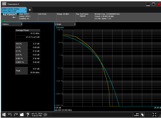
15MHz_15kHz_2535MHz_DFT-s-OFDM QPSK_RB75@0&8.16 dB
