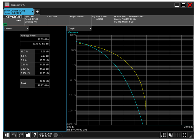
30MHz_15kHz_1745MHz_CP-OFDM 16 QAM_RB160@0&10.80 dB
