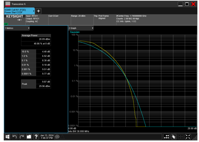
30MHz_15kHz_1745MHz_DFT-s-OFDM QPSK_RB160@0&8.30 dB
