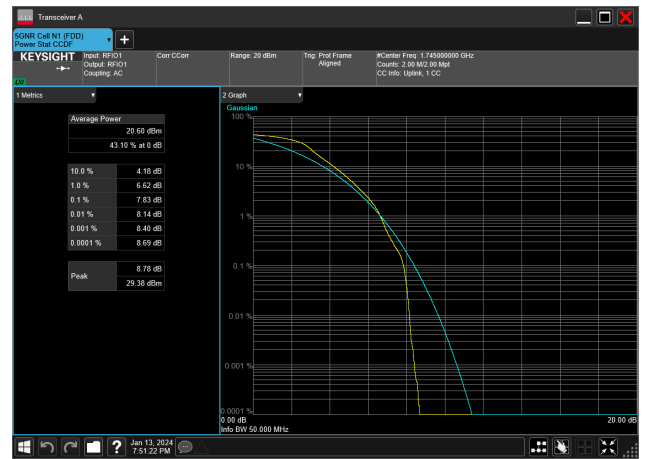
40MHz_15kHz_1745MHz_DFT-s-OFDM PI/2 BPSK_RB216@0&7.83 dB
