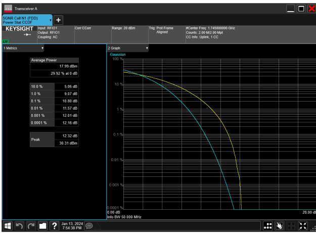
40MHz_15kHz_1745MHz_CP-OFDM 16 QAM_RB216@0&10.80 dB
