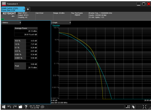
25MHz_15kHz_1745MHz_DFT-s-OFDM QPSK_RB128@0&8.29 dB
