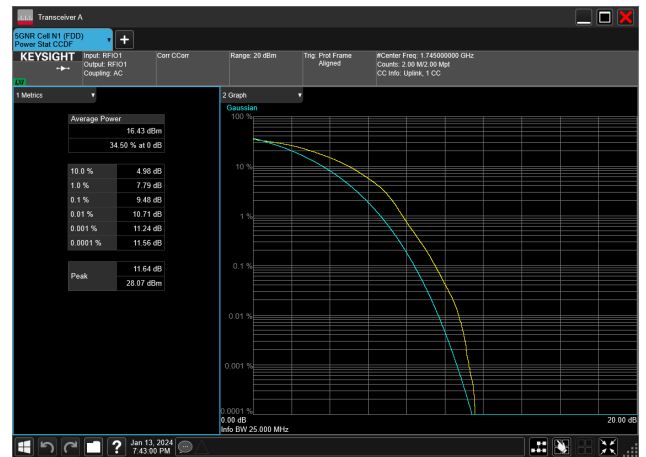
25MHz_15kHz_1745MHz_DFT-s-OFDM 256 QAM_RB128@0&9.48 dB
