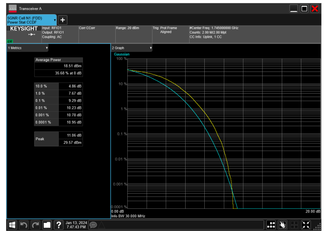
30MHz_15kHz_1745MHz_DFT-s-OFDM 64 QAM_RB160@0&9.29 dB
