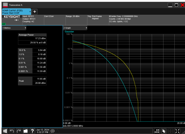
5MHz_15kHz_2535MHz_CP-OFDM 16 QAM_RB25@0&10.68 dB
