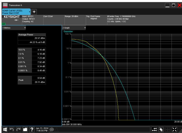
30MHz_15kHz_1745MHz_DFT-s-OFDM PI/2 BPSK_RB160@0&7.23 dB
