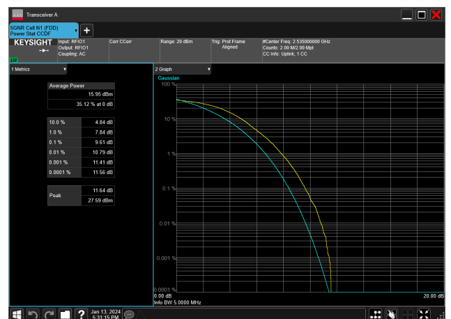
5MHz_15kHz_2535MHz_DFT-s-OFDM 256 QAM_RB25@0&9.61 dB
