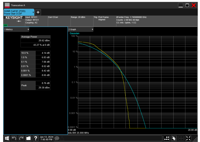
25MHz_15kHz_1745MHz_DFT-s-OFDM PI/2 BPSK_RB128@0&7.66 dB
