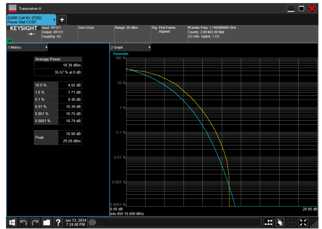
10MHz_15kHz_1745MHz_DFT-s-OFDM 64 QAM_RB50@0&9.38 dB
