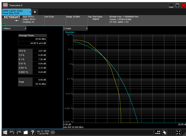
20MHz_15kHz_1745MHz_DFT-s-OFDM PI/2 BPSK_RB100@0&7.26 dB
