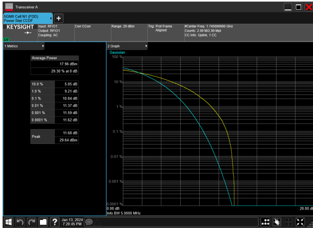
5MHz_15kHz_1745MHz_CP-OFDM 16 QAM_RB25@0&10.84 dB
