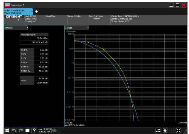
30MHz_15kHz_1745MHz_DFT-s-OFDM 16 QAM_RB160@0&9.05 dB
