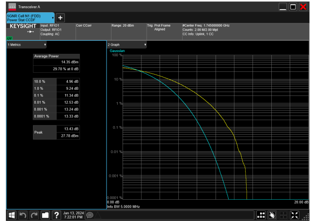
5MHz_15kHz_1745MHz_CP-OFDM 256 QAM_RB25@0&11.34 dB
