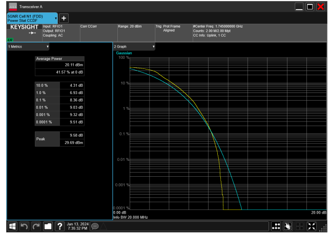
20MHz_15kHz_1745MHz_DFT-s-OFDM QPSK_RB100@0&8.36 dB
