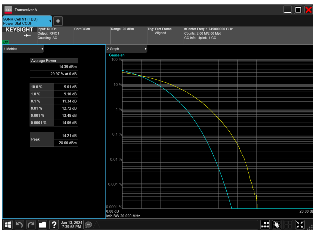
20MHz_15kHz_1745MHz_CP-OFDM 256 QAM_RB106@0&11.34 dB
