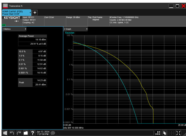
10MHz_15kHz_1745MHz_CP-OFDM 256 QAM_RB52@0&11.50 dB
