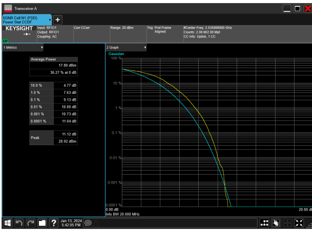
15MHz_15kHz_2535MHz_DFT-s-OFDM 64 QAM_RB75@0&9.13 dB
