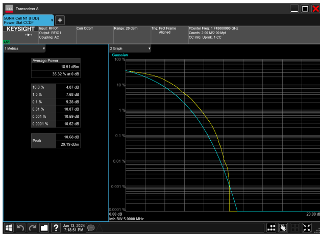
5MHz_15kHz_1745MHz_DFT-s-OFDM 64 QAM_RB25@0&9.28 dB
