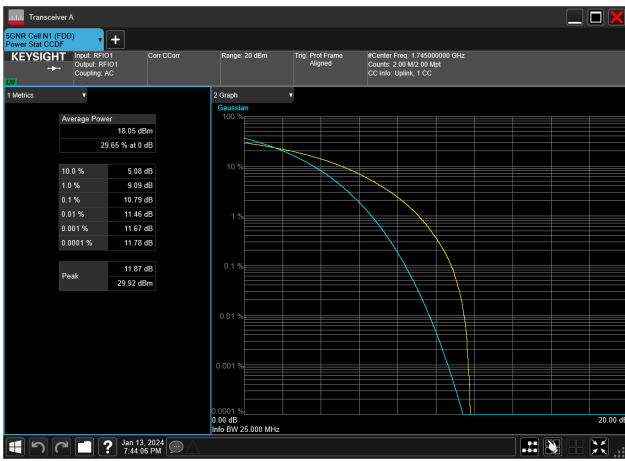
25MHz_15kHz_1745MHz_CP-OFDM 16 QAM_RB133@0&10.79 dB
