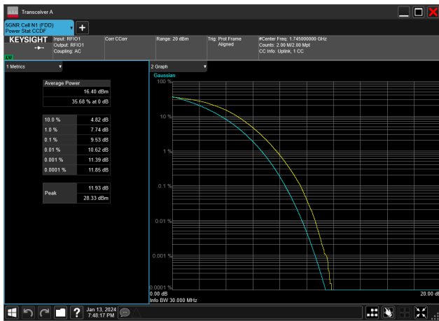
30MHz_15kHz_1745MHz_DFT-s-OFDM 256 QAM_RB160@0&9.53 dB
