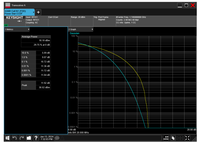
15MHz_15kHz_1745MHz_CP-OFDM QPSK_RB79@0&10.72 dB
