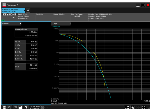
5MHz_15kHz_1745MHz_DFT-s-OFDM 16 QAM_RB25@0&9.00 dB
