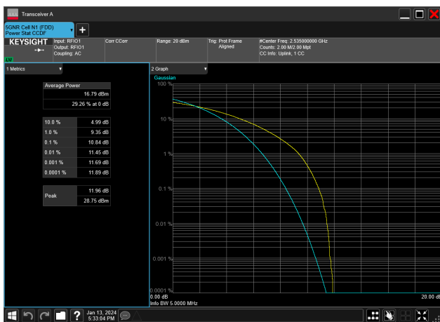
5MHz_15kHz_2535MHz_CP-OFDM 64 QAM_RB25@0&10.84 dB
