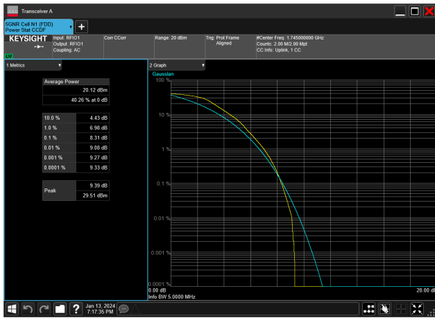
5MHz_15kHz_1745MHz_DFT-s-OFDM QPSK_RB25@0&8.31 dB
