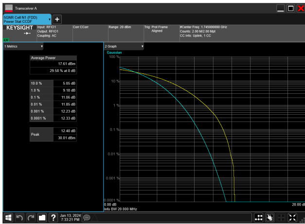
15MHz_15kHz_1745MHz_CP-OFDM 64 QAM_RB79@0&11.06 dB
