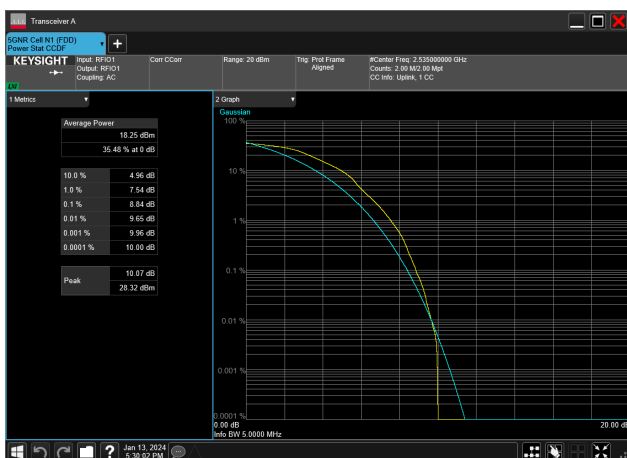
5MHz_15kHz_2535MHz_DFT-s-OFDM 16 QAM_RB25@0&8.84 dB
