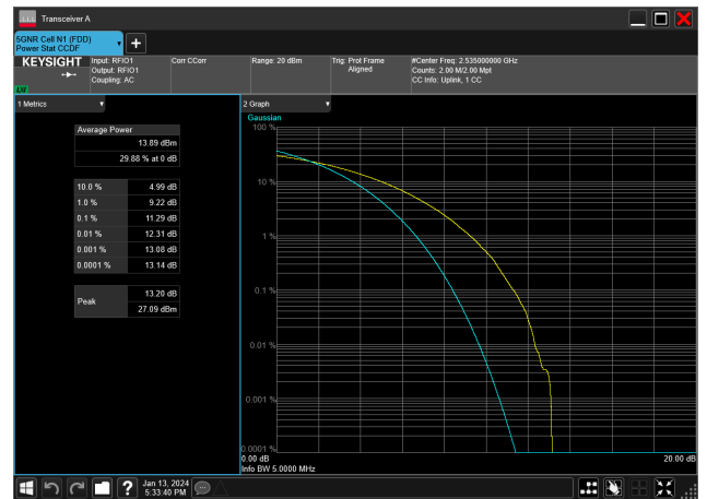
5MHz_15kHz_2535MHz_CP-OFDM 256 QAM_RB25@0&11.29 dB
