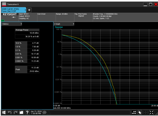
15MHz_15kHz_1745MHz_DFT-s-OFDM 64 QAM_RB75@0&9.28 dB
