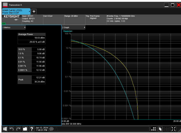
30MHz_15kHz_1745MHz_CP-OFDM QPSK_RB160@0&10.74 dB
