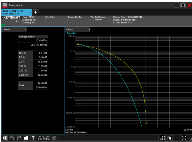
25MHz_15kHz_1745MHz_CP-OFDM 64 QAM_RB133@0&10.92 dB
