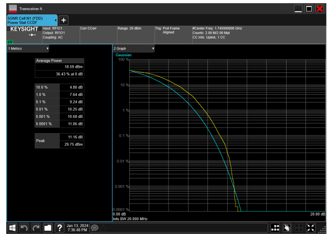
20MHz_15kHz_1745MHz_DFT-s-OFDM 64 QAM_RB100@0&9.24 dB
