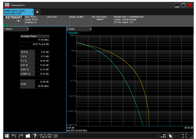
30MHz_15kHz_1745MHz_CP-OFDM 64 QAM_RB160@0&10.95 dB
