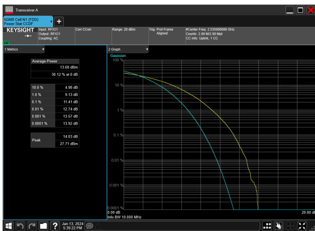
10MHz_15kHz_2535MHz_CP-OFDM 256 QAM_RB52@0&11.41 dB
