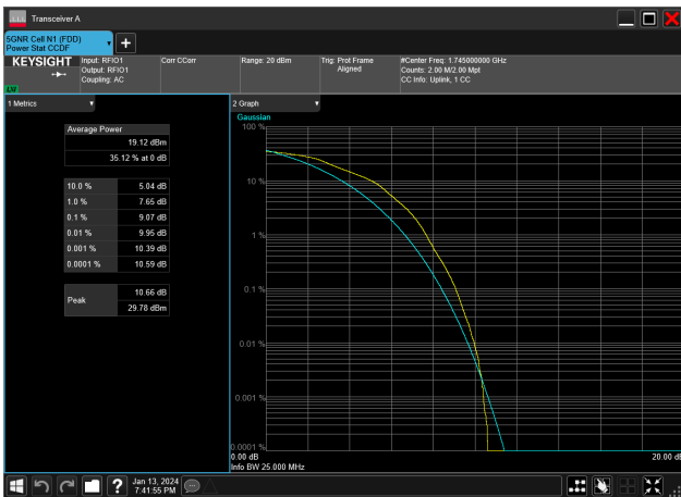
25MHz_15kHz_1745MHz_DFT-s-OFDM 16 QAM_RB128@0&9.07 dB
