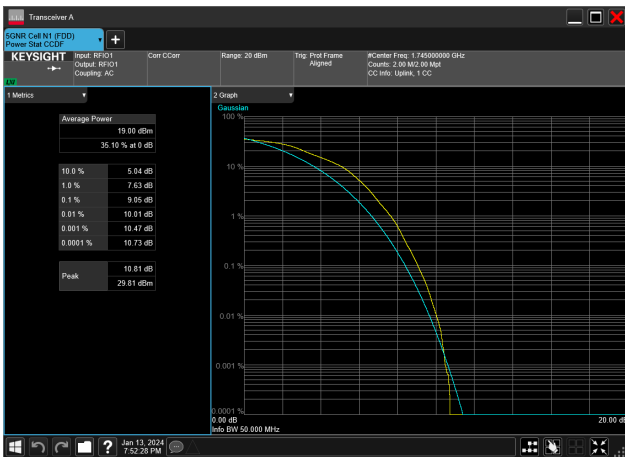
40MHz_15kHz_1745MHz_DFT-s-OFDM 16 QAM_RB216@0&9.05 dB
