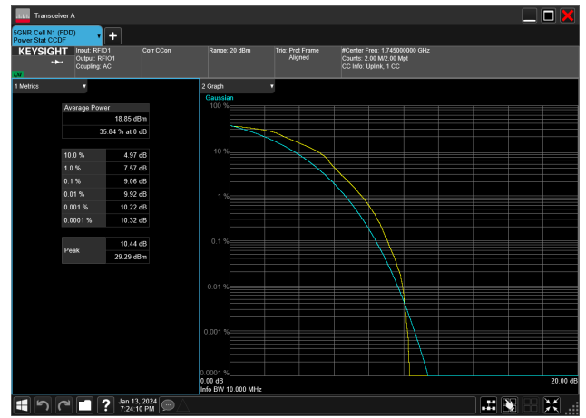
10MHz_15kHz_1745MHz_DFT-s-OFDM 16 QAM_RB50@0&9.06 dB
