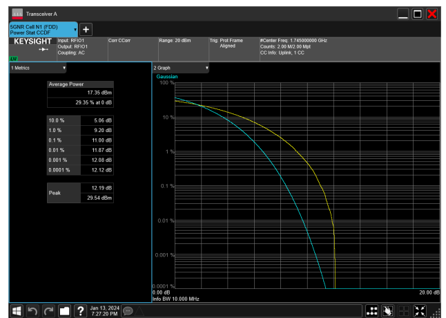
10MHz_15kHz_1745MHz_CP-OFDM 64 QAM_RB52@0&11.00 dB
