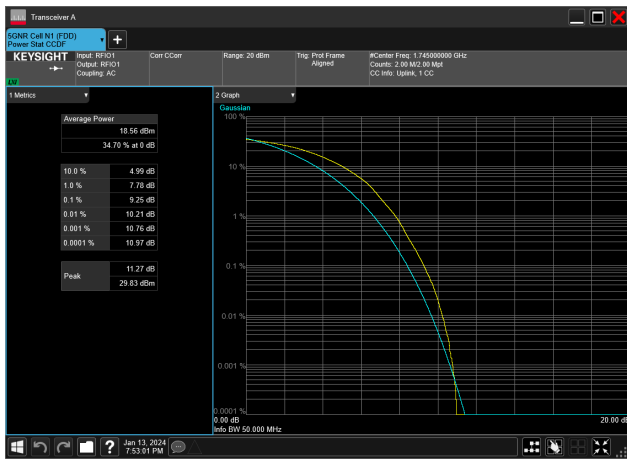
40MHz_15kHz_1745MHz_DFT-s-OFDM 64 QAM_RB216@0&9.25 dB
