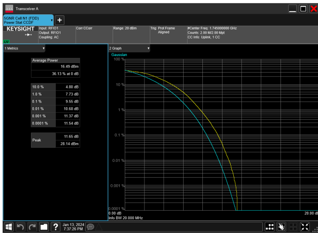
20MHz_15kHz_1745MHz_DFT-s-OFDM 256 QAM_RB100@0&9.55 dB
