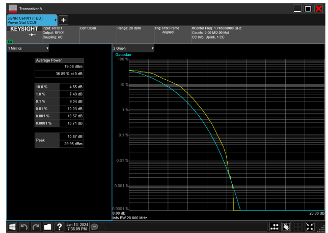
20MHz_15kHz_1745MHz_DFT-s-OFDM 16 QAM_RB100@0&9.04 dB
