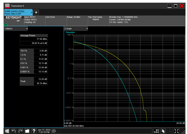
20MHz_15kHz_1745MHz_CP-OFDM 64 QAM_RB106@0&11.07 dB
