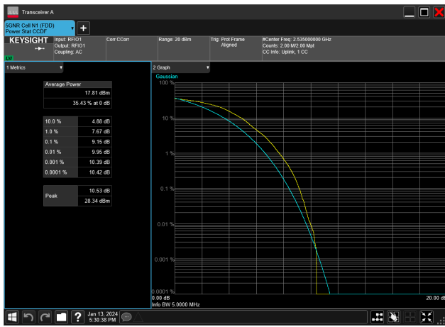
5MHz_15kHz_2535MHz_DFT-s-OFDM 64 QAM_RB25@0&9.15 dB
