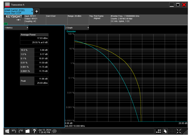
10MHz_15kHz_1745MHz_CP-OFDM 16 QAM_RB52@0&10.81 dB
