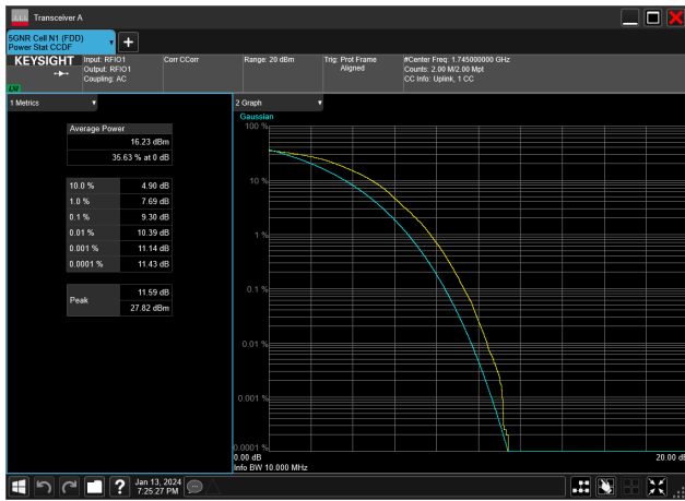
10MHz_15kHz_1745MHz_DFT-s-OFDM 256 QAM_RB50@0&9.30 dB
