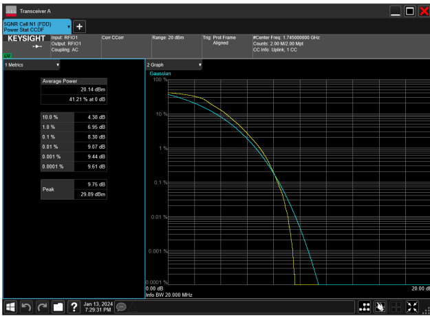
15MHz_15kHz_1745MHz_DFT-s-OFDM QPSK_RB75@0&8.30 dB
