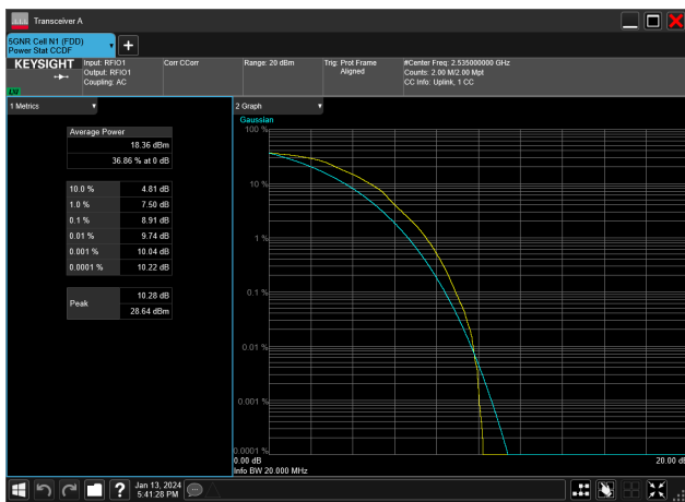
15MHz_15kHz_2535MHz_DFT-s-OFDM 16 QAM_RB75@0&8.91 dB
