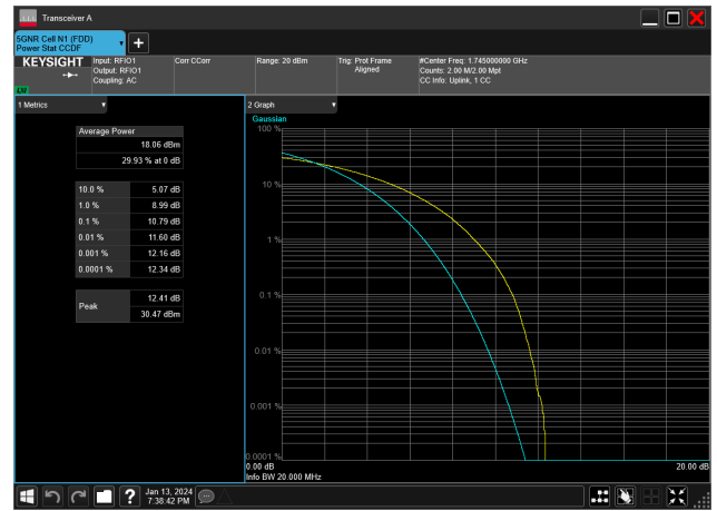
20MHz_15kHz_1745MHz_CP-OFDM 16 QAM_RB106@0&10.79 dB
