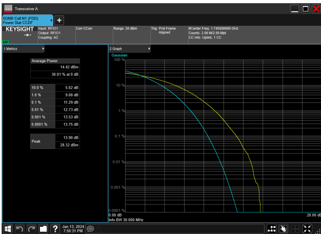
30MHz_15kHz_1745MHz_CP-OFDM 256 QAM_RB160@0&11.29 dB
