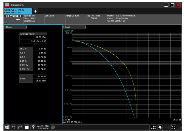
25MHz_15kHz_1745MHz_CP-OFDM QPSK_RB133@0&10.70 dB
