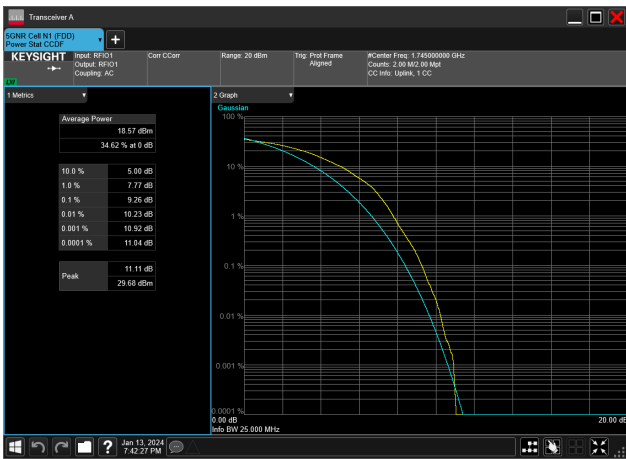
25MHz_15kHz_1745MHz_DFT-s-OFDM 64 QAM_RB128@0&9.26 dB
