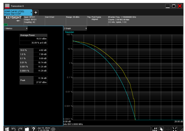
5MHz_15kHz_1745MHz_DFT-s-OFDM 256 QAM_RB25@0&9.69 dB
