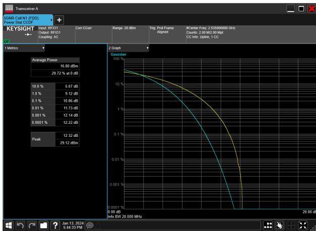
15MHz_15kHz_2535MHz_CP-OFDM 64 QAM_RB79@0&10.85 dB
