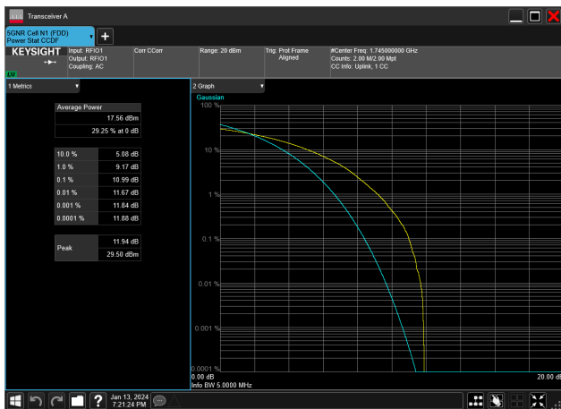
5MHz_15kHz_1745MHz_CP-OFDM 64 QAM_RB25@0&10.99 dB
