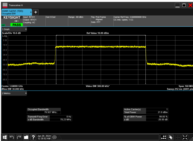
80MHz_30kHz_3840MHz_DFT-s-OFDM 64 QAM_RB216@0&76.927 MHz
