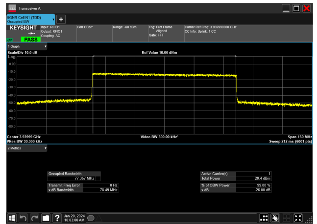
80MHz_30kHz_3940MHz_CP-OFDM 16 QAM_RB217@0&77.357 MHz
