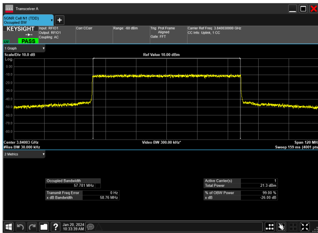
60MHz_30kHz_3840MHz_DFT-s-OFDM 64 QAM_RB162@0&57.781 MHz
