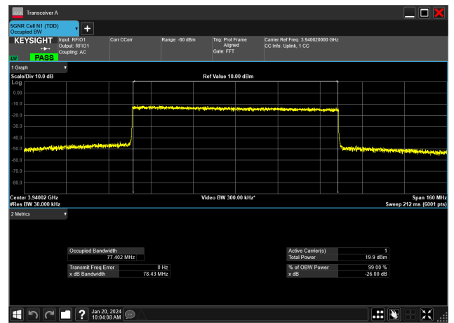
80MHz_30kHz_3940MHz_CP-OFDM 64 QAM_RB217@0&77.402 MHz
