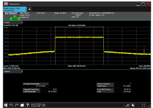
70MHz_30kHz_3945MHz_CP-OFDM 256 QAM_RB189@0&67.375 MHz
