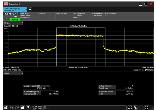
70MHz_30kHz_3945MHz_DFT-s-OFDM PI/2 BPSK_RB180@0&amp;67.050 MHz
