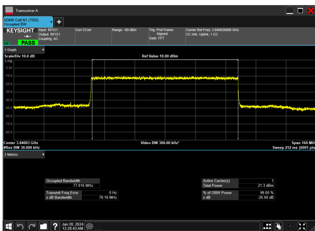
80MHz_30kHz_3840MHz_DFT-s-OFDM 16 QAM_RB216@0&77.016 MHz
