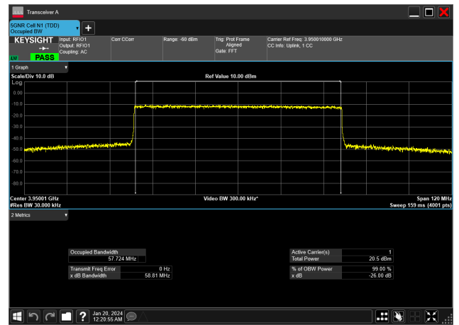
60MHz_30kHz_3950MHz_CP-OFDM 16 QAM_RB162@0&57.724 MHz
