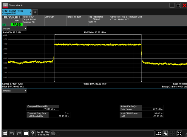
80MHz_30kHz_3740MHz_DFT-s-OFDM PI/2 BPSK_RB216@0&77.018 MHz
