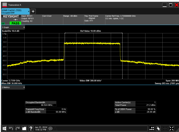
70MHz_30kHz_3735MHz_DFT-s-OFDM 64 QAM_RB180@0&66.924 MHz
