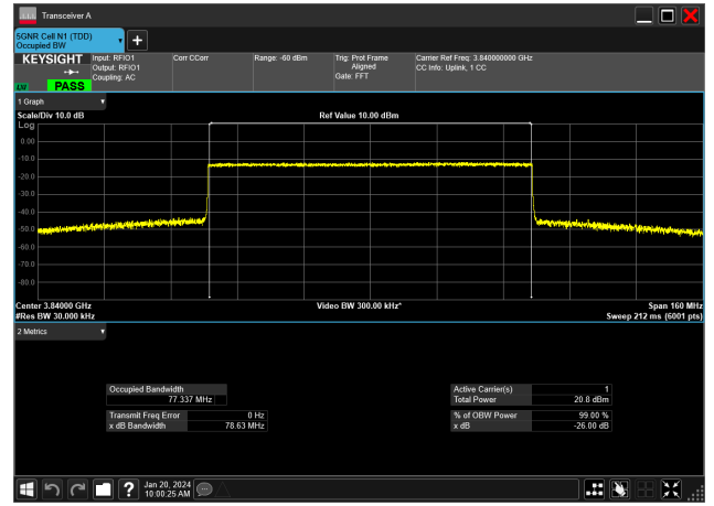
80MHz_30kHz_3840MHz_CP-OFDM QPSK_RB217@0&77.337 MHz
