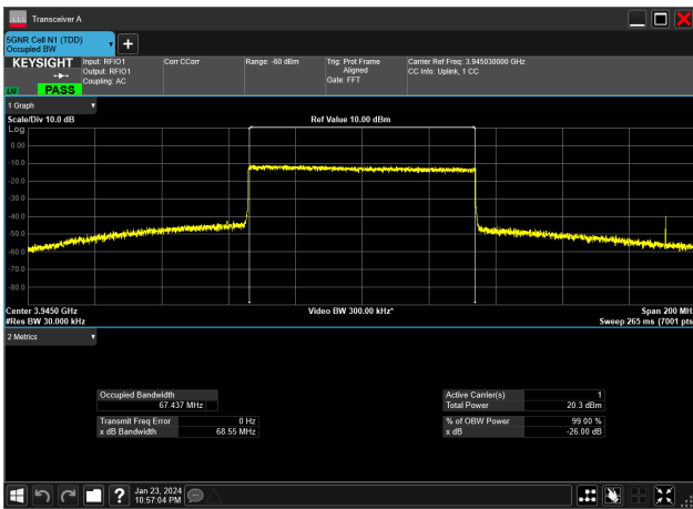
70MHz_30kHz_3945MHz_CP-OFDM 16 QAM_RB189@0&67.437 MHz
