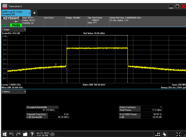
70MHz_30kHz_3840MHz_CP-OFDM 256 QAM_RB189@0&67.379 MHz
