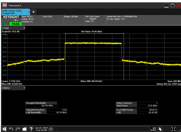
70MHz_30kHz_3735MHz_DFT-s-OFDM QPSK_RB180@0&66.874 MHz
