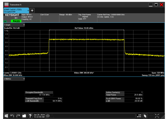
60MHz_30kHz_3950MHz_CP-OFDM 64 QAM_RB162@0&57.734 MHz
