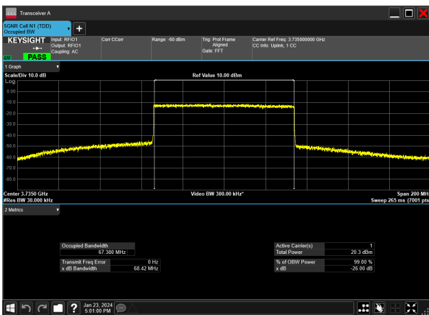
70MHz_30kHz_3735MHz_CP-OFDM 64 QAM_RB189@0&67.380 MHz
