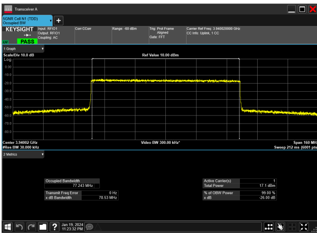
80MHz_30kHz_3940MHz_CP-OFDM 256 QAM_RB217@0&77.243 MHz
