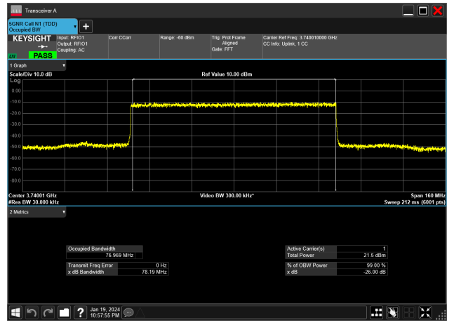
80MHz_30kHz_3740MHz_DFT-s-OFDM 16 QAM_RB216@0&76.969 MHz
