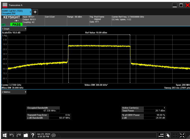
70MHz_30kHz_3735MHz_CP-OFDM 16 QAM_RB189@0&67.330 MHz
