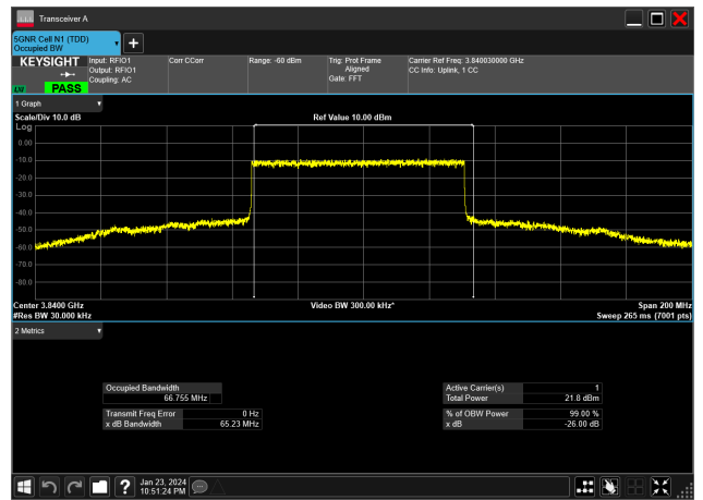
70MHz_30kHz_3840MHz_DFT-s-OFDM 16 QAM_RB180@0&66.755 MHz
