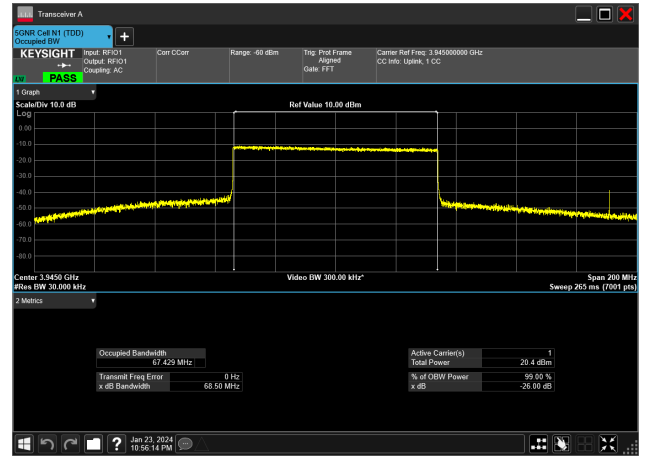
70MHz_30kHz_3945MHz_CP-OFDM QPSK_RB189@0&67.429 MHz
