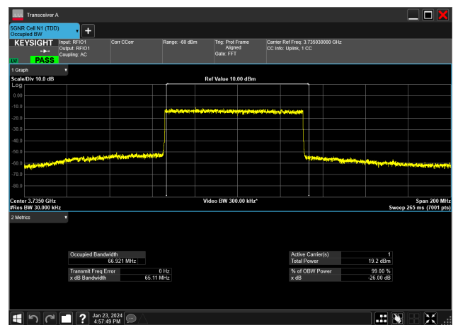
70MHz_30kHz_3735MHz_DFT-s-OFDM 256 QAM_RB180@0&66.921 MHz
