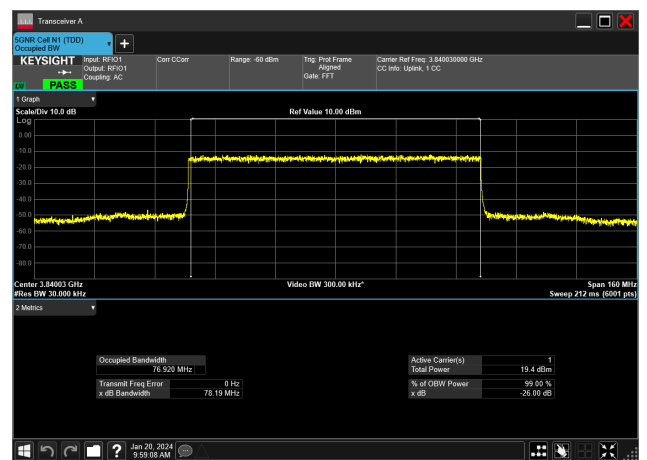
80MHz_30kHz_3840MHz_DFT-s-OFDM 256 QAM_RB216@0&76.920 MHz
