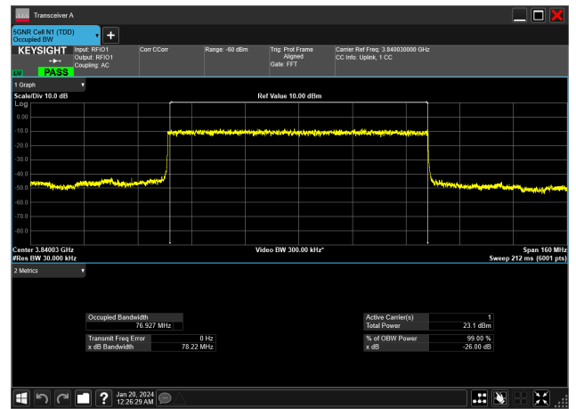
80MHz_30kHz_3840MHz_DFT-s-OFDM PI/2 BPSK_RB216@0&76.927 MHz
