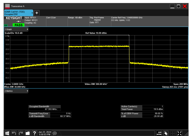
70MHz_30kHz_3840MHz_CP-OFDM 64 QAM_RB189@0&67.393 MHz
