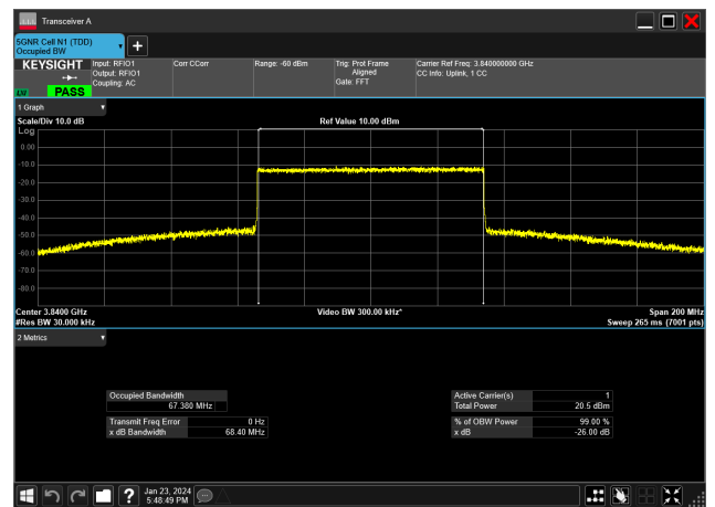
70MHz_30kHz_3840MHz_CP-OFDM 16 QAM_RB189@0&67.380 MHz
