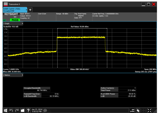
70MHz_30kHz_3840MHz_DFT-s-OFDM 64 QAM_RB180@0&66.744 MHz
