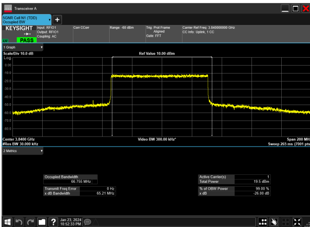
70MHz_30kHz_3840MHz_DFT-s-OFDM 256 QAM_RB180@0&66.755 MHz
