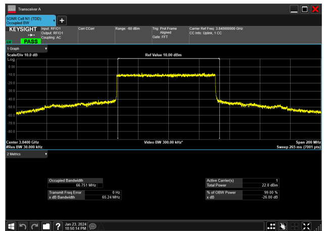
70MHz_30kHz_3840MHz_DFT-s-OFDM QPSK_RB180@0&66.751 MHz
