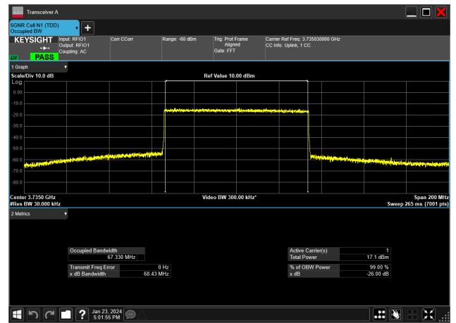
70MHz_30kHz_3735MHz_CP-OFDM 256 QAM_RB189@0&67.330 MHz
