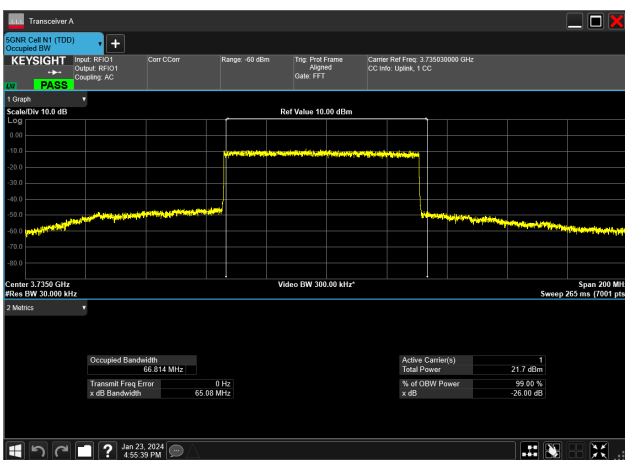
70MHz_30kHz_3735MHz_DFT-s-OFDM 16 QAM_RB180@0&66.814 MHz
