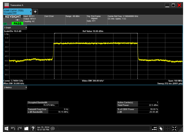
80MHz_30kHz_3740MHz_DFT-s-OFDM QPSK_RB216@0&76.979 MHz
