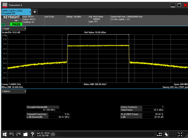
70MHz_30kHz_3840MHz_CP-OFDM QPSK_RB189@0&67.389 MHz
