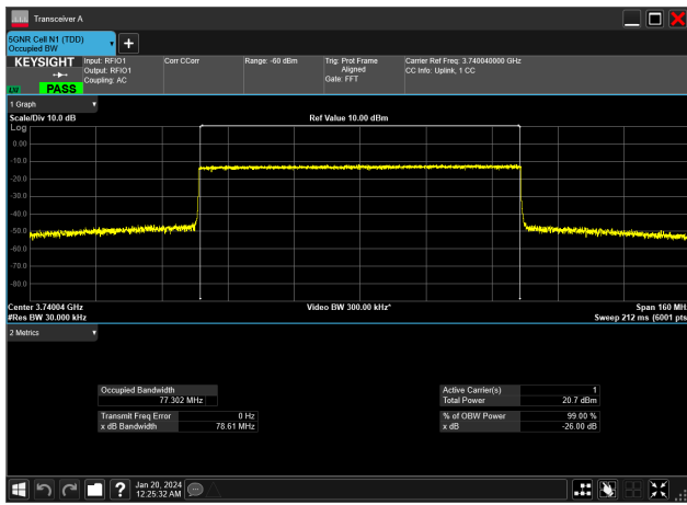
80MHz_30kHz_3740MHz_CP-OFDM QPSK_RB217@0&77.302 MHz
