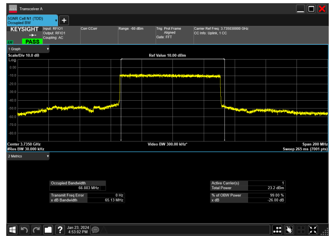
70MHz_30kHz_3735MHz_DFT-s-OFDM PI/2 BPSK_RB180@0&66.883 MHz
