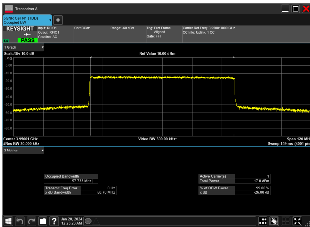
60MHz_30kHz_3950MHz_CP-OFDM 256 QAM_RB162@0&57.733 MHz
