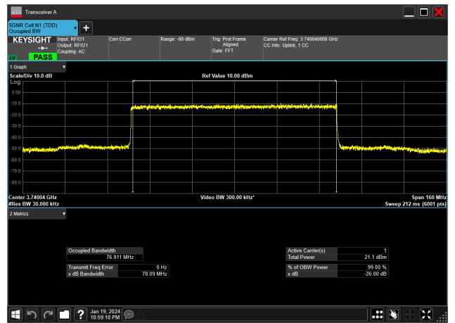
80MHz_30kHz_3740MHz_DFT-s-OFDM 64 QAM_RB216@0&76.911 MHz
