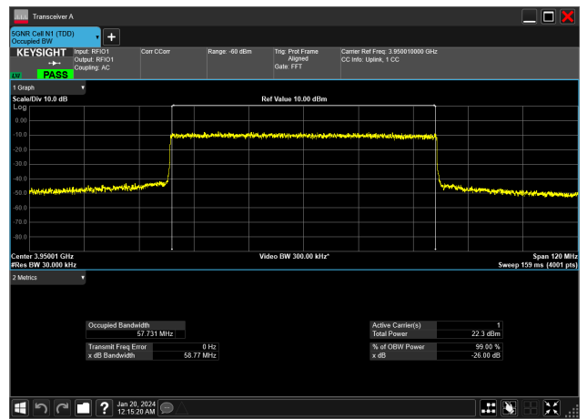
60MHz_30kHz_3950MHz_DFT-s-OFDM QPSK_RB162@0&57.731 MHz
