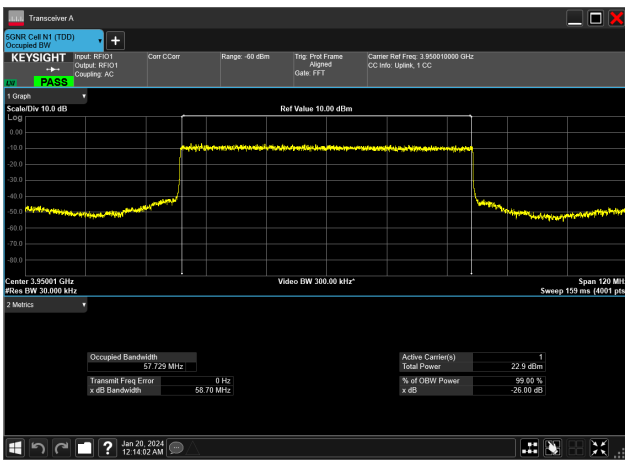
60MHz_30kHz_3950MHz_DFT-s-OFDM PI/2 BPSK_RB162@0&57.729 MHz
