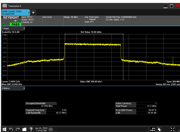
70MHz_30kHz_3945MHz_DFT-s-OFDM 16 QAM_RB180@0&67.094 MHz
