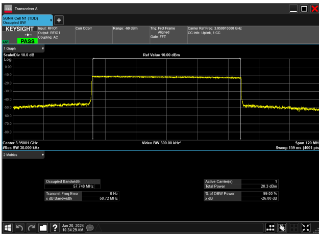
60MHz_30kHz_3950MHz_CP-OFDM QPSK_RB162@0&57.748 MHz
