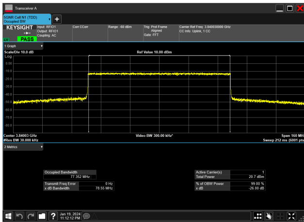
80MHz_30kHz_3840MHz_CP-OFDM 16 QAM_RB217@0&77.352 MHz
