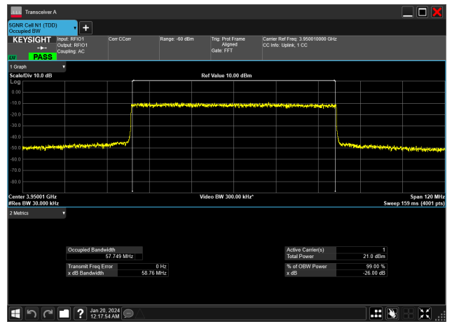
60MHz_30kHz_3950MHz_DFT-s-OFDM 64 QAM_RB162@0&57.749 MHz
