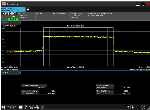
60MHz_30kHz_3950MHz_DFT-s-OFDM 256 QAM_RB162@0&57.781 MHz
