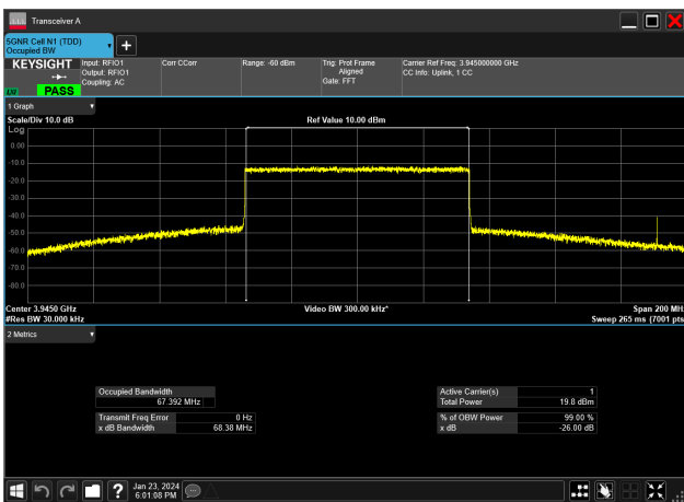
70MHz_30kHz_3945MHz_CP-OFDM 64 QAM_RB189@0&67.392 MHz
