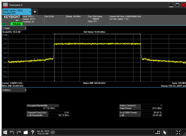
60MHz_30kHz_3840MHz_DFT-s-OFDM QPSK_RB162@0&57.726 MHz
