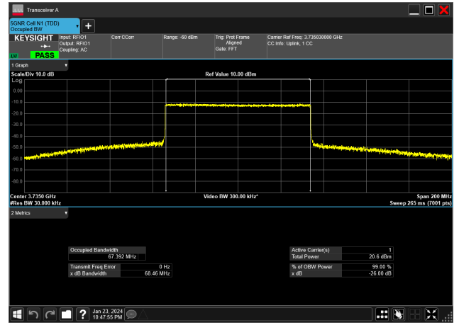
70MHz_30kHz_3735MHz_CP-OFDM QPSK_RB189@0&67.392 MHz
