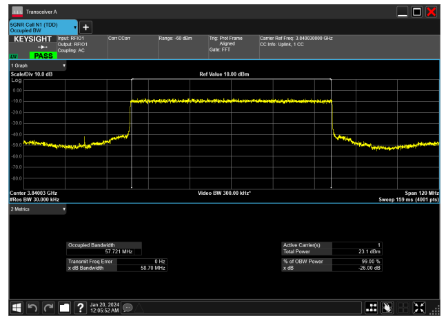
60MHz_30kHz_3840MHz_DFT-s-OFDM PI/2 BPSK_RB162@0&57.721 MHz
