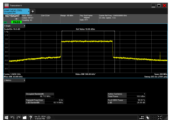
70MHz_30kHz_3945MHz_DFT-s-OFDM 256 QAM_RB180@0&66.712 MHz
