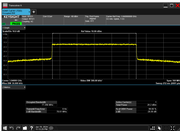
80MHz_30kHz_3840MHz_CP-OFDM 64 QAM_RB217@0&77.296 MHz
