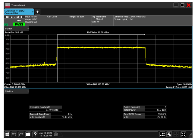
80MHz_30kHz_3840MHz_CP-OFDM 256 QAM_RB217@0&77.194 MHz
