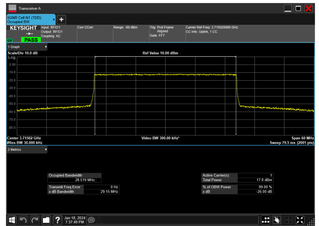
30MHz_15kHz_3715MHz_CP-OFDM 256 QAM_RB160@0&28.519 MHz
