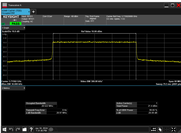
30MHz_15kHz_3715MHz_DFT-s-OFDM 16 QAM_RB160@0&28.522 MHz
