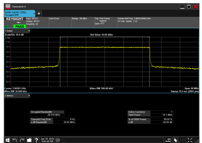
30MHz_15kHz_3965MHz_DFT-s-OFDM 256 QAM_RB160@0&28.518 MHz
