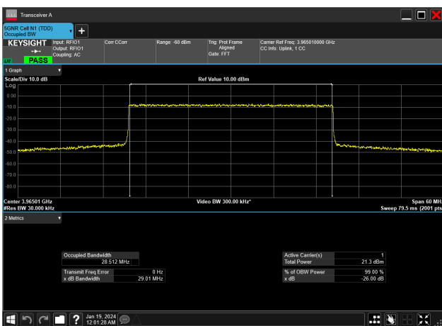
30MHz_15kHz_3965MHz_DFT-s-OFDM 16 QAM_RB160@0&28.512 MHz
