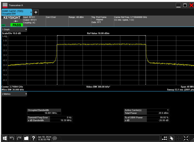
20MHz_15kHz_3710MHz_CP-OFDM 16 QAM_RB106@0&18.891 MHz
