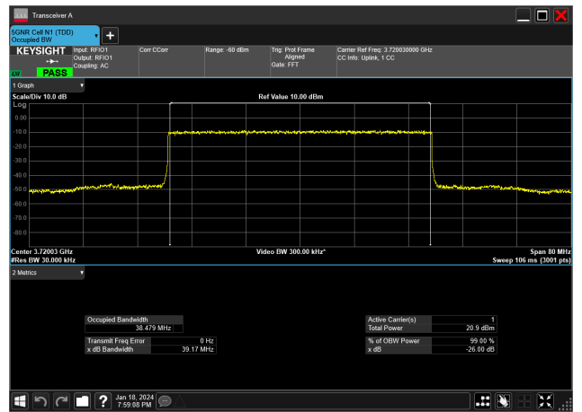
40MHz_15kHz_3720MHz_DFT-s-OFDM 64 QAM_RB216@0&38.479 MHz
