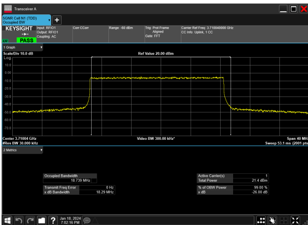
20MHz_15kHz_3710MHz_DFT-s-OFDM 16 QAM_RB100@0&18.739 MHz
