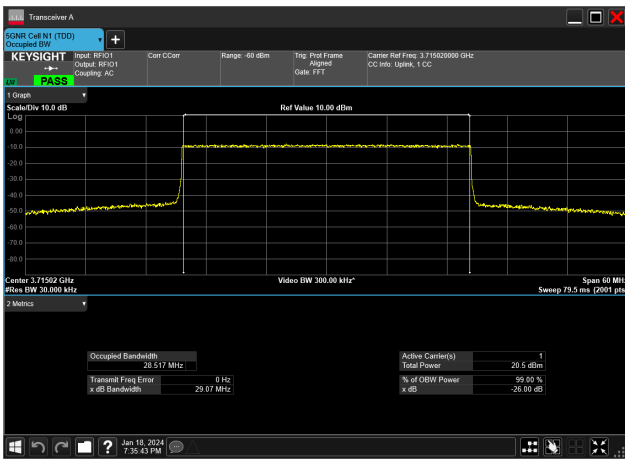
30MHz_15kHz_3715MHz_CP-OFDM 16 QAM_RB160@0&28.517 MHz
