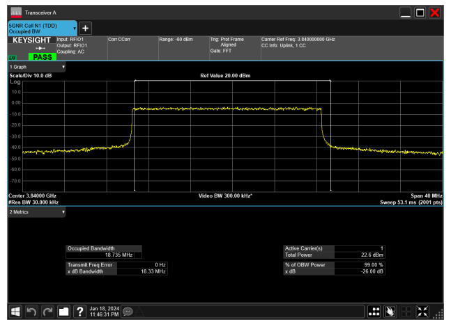
20MHz_15kHz_3840MHz_DFT-s-OFDM QPSK_RB100@0&18.735 MHz
