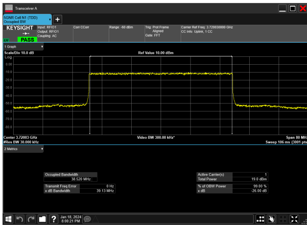
40MHz_15kHz_3720MHz_DFT-s-OFDM 256 QAM_RB216@0&38.520 MHz
