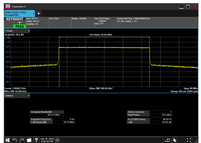
40MHz_15kHz_3960MHz_CP-OFDM 64 QAM_RB216@0&38.512 MHz
