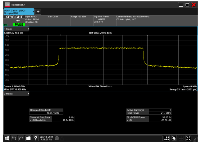
20MHz_15kHz_3840MHz_DFT-s-OFDM 16 QAM_RB100@0&18.657 MHz
