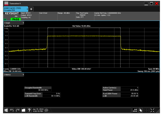
40MHz_15kHz_3840MHz_CP-OFDM QPSK_RB216@0&38.508 MHz
