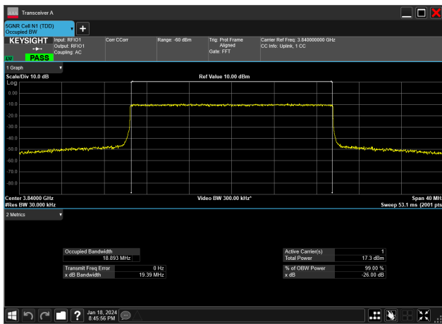
20MHz_15kHz_3840MHz_CP-OFDM 256 QAM_RB106@0&18.893 MHz
