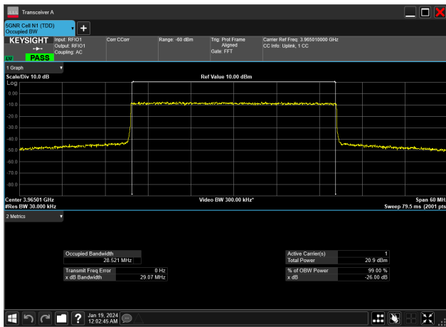
30MHz_15kHz_3965MHz_DFT-s-OFDM 64 QAM_RB160@0&28.521 MHz
