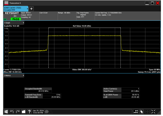
30MHz_15kHz_3715MHz_CP-OFDM QPSK_RB160@0&28.518 MHz
