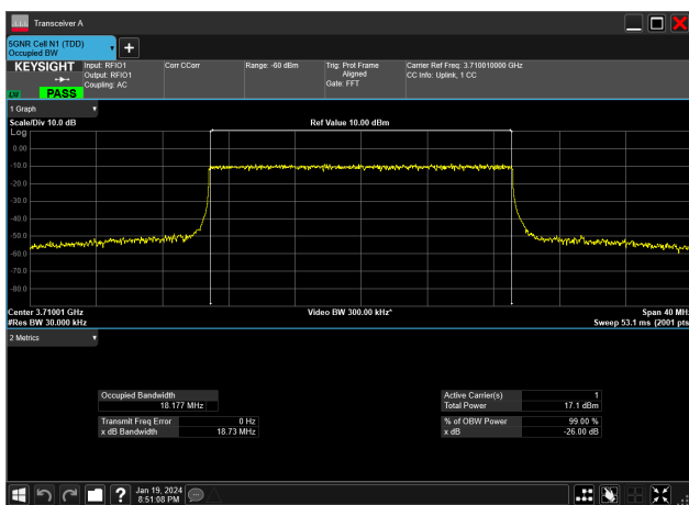
20MHz_30kHz_3710MHz_CP-OFDM 256 QAM_RB51@0&18.177 MHz
