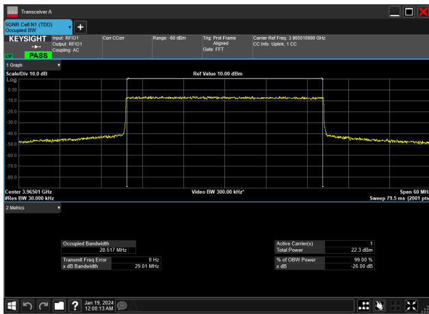
30MHz_15kHz_3965MHz_DFT-s-OFDM QPSK_RB160@0&28.517 MHz
