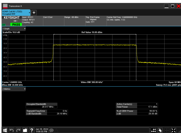
30MHz_15kHz_3840MHz_CP-OFDM 256 QAM_RB160@0&28.517 MHz
