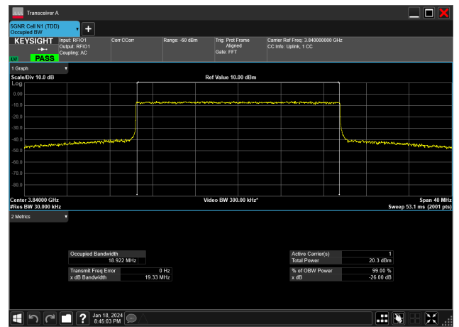
20MHz_15kHz_3840MHz_CP-OFDM 64 QAM_RB106@0&18.922 MHz
