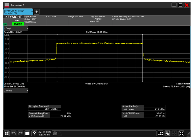
30MHz_15kHz_3840MHz_DFT-s-OFDM 64 QAM_RB160@0&28.515 MHz
