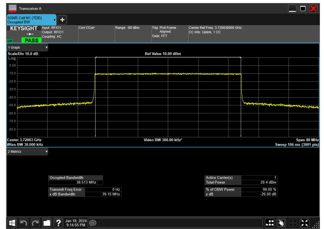
40MHz_15kHz_3720MHz_CP-OFDM 16 QAM_RB216@0&38.513 MHz
