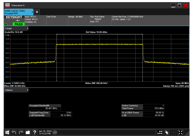
40MHz_15kHz_3720MHz_CP-OFDM 64 QAM_RB216@0&38.467 MHz
