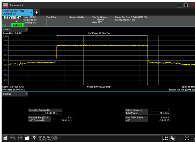
40MHz_15kHz_3840MHz_DFT-s-OFDM 64 QAM_RB216@0&38.514 MHz
