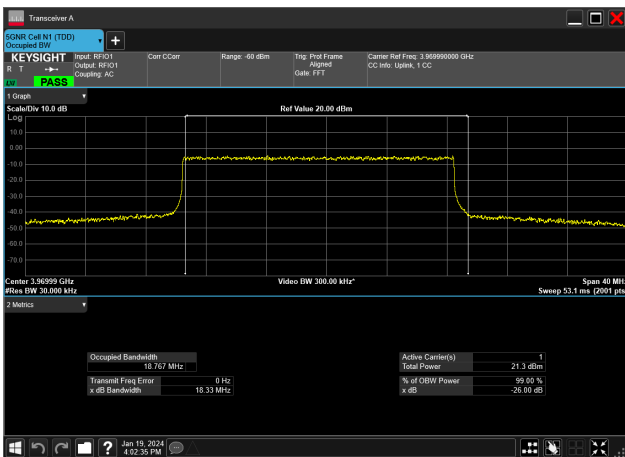
20MHz_15kHz_3970MHz_DFT-s-OFDM 16 QAM_RB100@0&18.767 MHz
