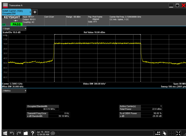
40MHz_15kHz_3720MHz_DFT-s-OFDM PI/2 BPSK_RB216@0&38.519 MHz
