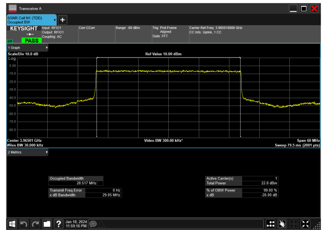
30MHz_15kHz_3965MHz_DFT-s-OFDM PI/2 BPSK_RB160@0&28.517 MHz
