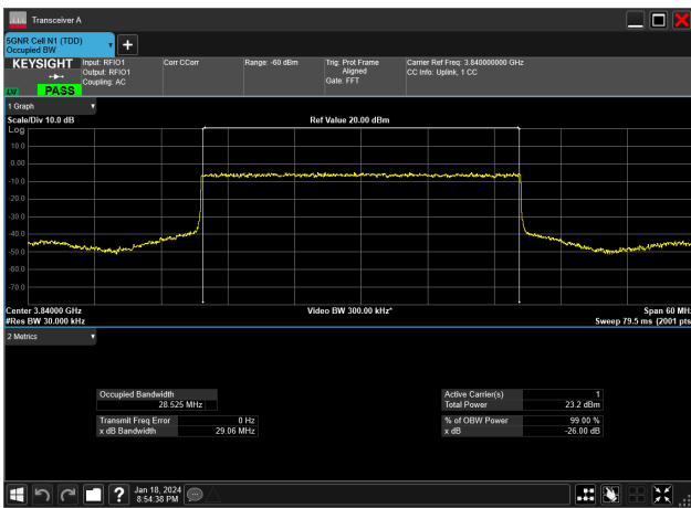
30MHz_15kHz_3840MHz_DFT-s-OFDM PI/2 BPSK_RB160@0&28.525 MHz
