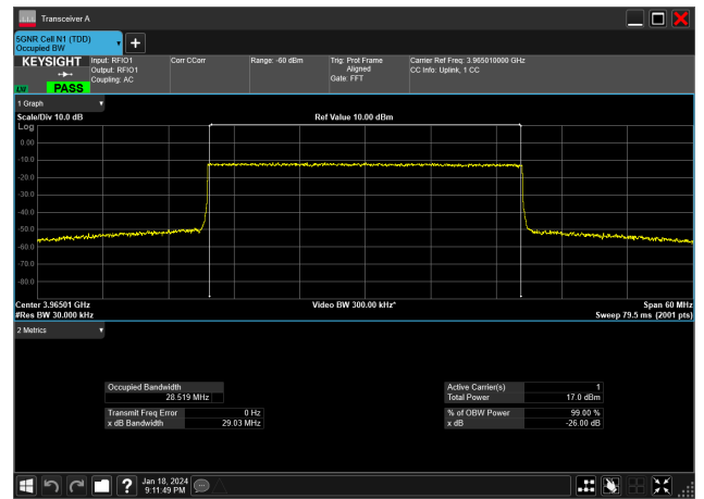
30MHz_15kHz_3965MHz_CP-OFDM 256 QAM_RB160@0&28.519 MHz
