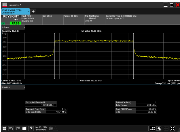
20MHz_30kHz_3840MHz_CP-OFDM 16 QAM_RB51@0&18.204 MHz
