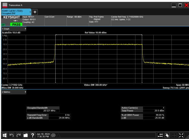
30MHz_15kHz_3715MHz_CP-OFDM 64 QAM_RB160@0&28.521 MHz
