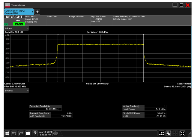
20MHz_15kHz_3710MHz_CP-OFDM 256 QAM_RB106@0&18.893 MHz
