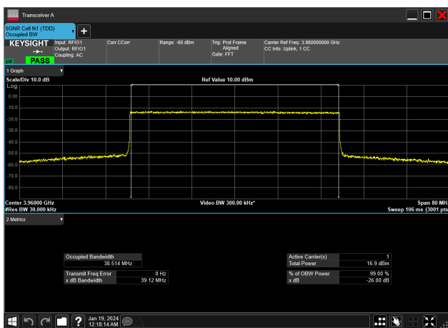
40MHz_15kHz_3960MHz_CP-OFDM 256 QAM_RB216@0&38.514 MHz
