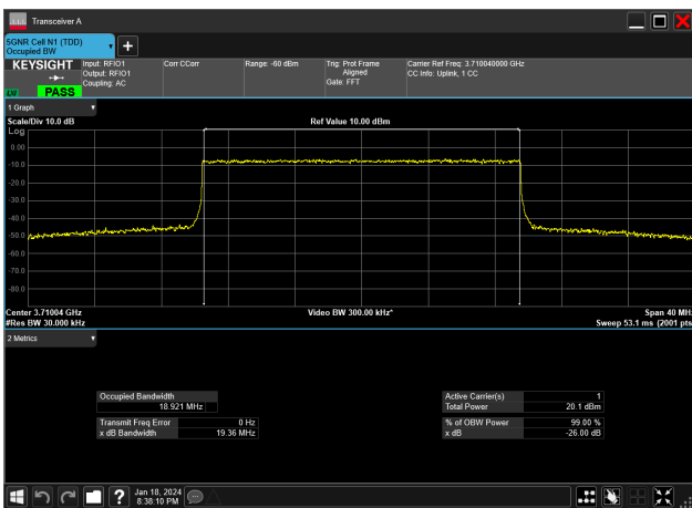
20MHz_15kHz_3710MHz_CP-OFDM 64 QAM_RB106@0&18.921 MHz
