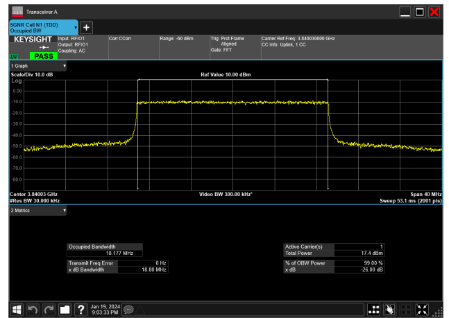
20MHz_30kHz_3840MHz_CP-OFDM 256 QAM_RB51@0&18.177 MHz
