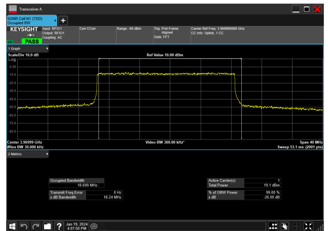
20MHz_15kHz_3970MHz_DFT-s-OFDM 256 QAM_RB100@0&18.699 MHz
