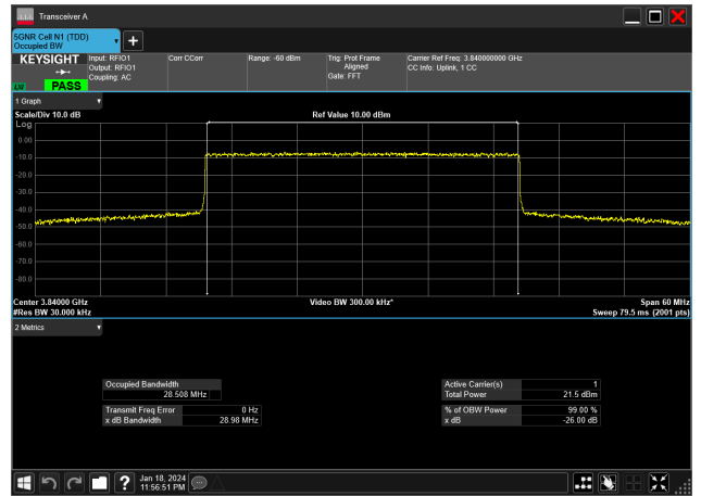
30MHz_15kHz_3840MHz_DFT-s-OFDM 16 QAM_RB160@0&28.508 MHz
