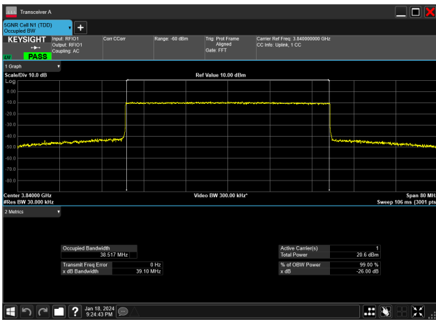
40MHz_15kHz_3840MHz_CP-OFDM 16 QAM_RB216@0&38.517 MHz
