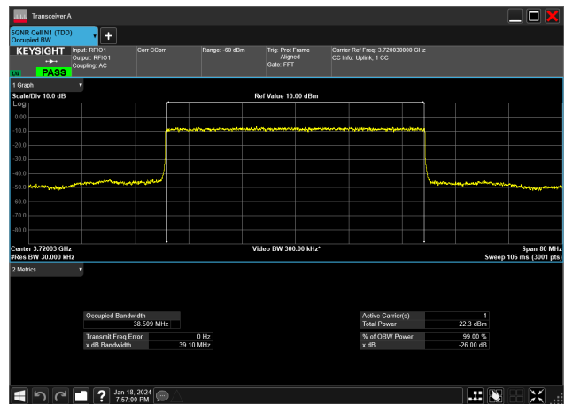
40MHz_15kHz_3720MHz_DFT-s-OFDM QPSK_RB216@0&38.509 MHz
