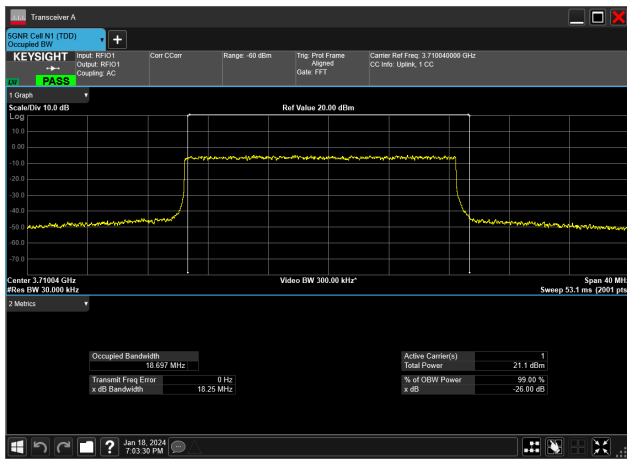
20MHz_15kHz_3710MHz_DFT-s-OFDM 64 QAM_RB100@0&18.697 MHz
