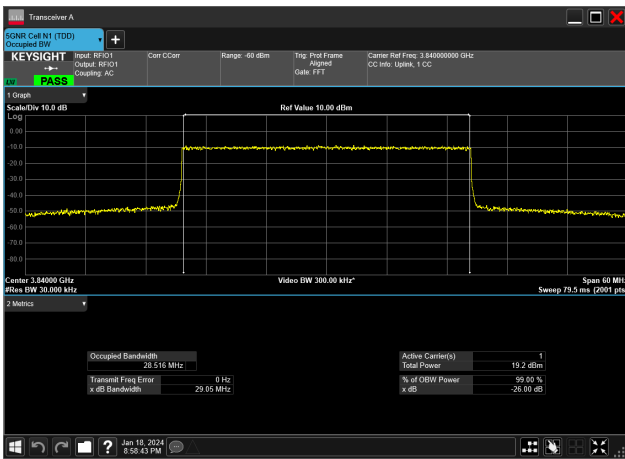
30MHz_15kHz_3840MHz_DFT-s-OFDM 256 QAM_RB160@0&28.516 MHz
