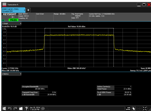
30MHz_15kHz_3715MHz_DFT-s-OFDM QPSK_RB160@0&28.500 MHz
