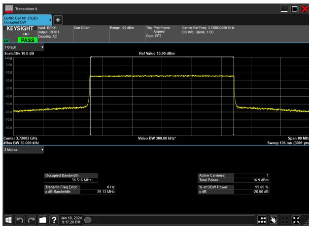
40MHz_15kHz_3720MHz_CP-OFDM 256 QAM_RB216@0&38.516 MHz
