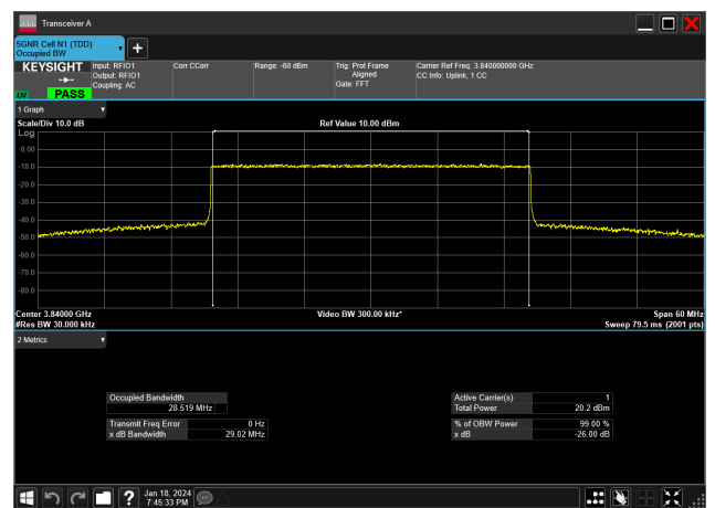
30MHz_15kHz_3840MHz_CP-OFDM 64 QAM_RB160@0&28.519 MHz
