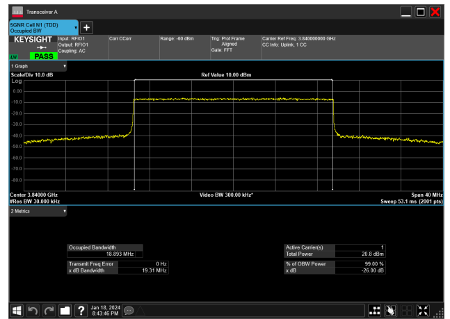
20MHz_15kHz_3840MHz_CP-OFDM 16 QAM_RB106@0&18.893 MHz
