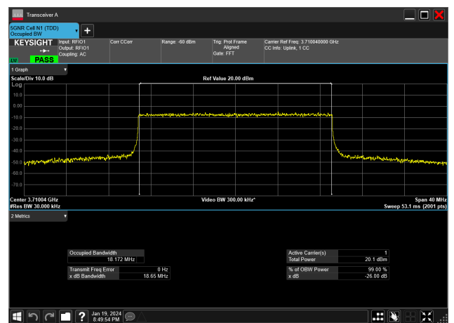
20MHz_30kHz_3710MHz_CP-OFDM 64 QAM_RB51@0&18.172 MHz
