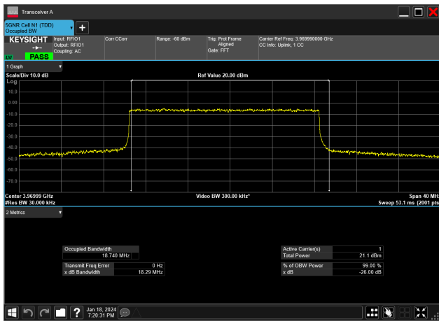
20MHz_15kHz_3970MHz_DFT-s-OFDM 64 QAM_RB100@0&18.740 MHz
