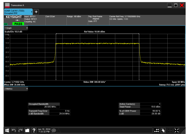
30MHz_15kHz_3715MHz_DFT-s-OFDM 256 QAM_RB160@0&28.505 MHz
