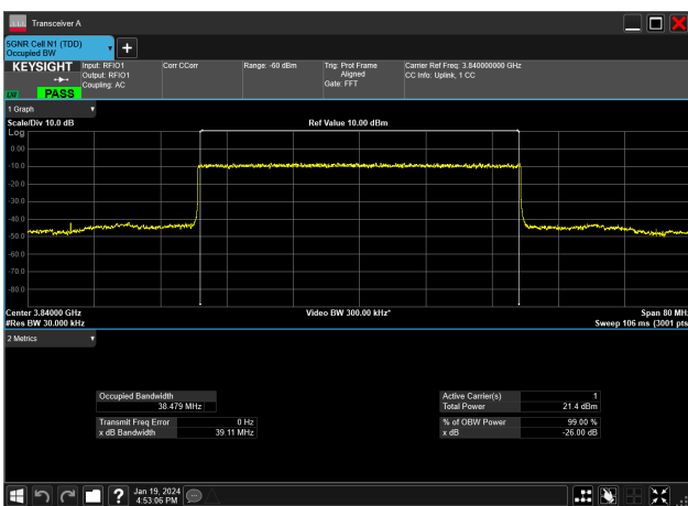
40MHz_15kHz_3840MHz_DFT-s-OFDM 16 QAM_RB216@0&38.479 MHz
