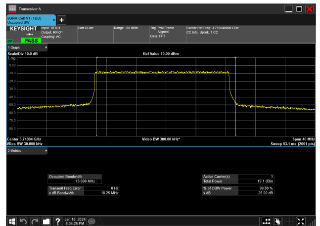
20MHz_15kHz_3710MHz_DFT-s-OFDM 256 QAM_RB100@0&18.698 MHz
