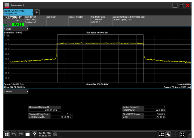
30MHz_15kHz_3840MHz_DFT-s-OFDM QPSK_RB160@0&28.517 MHz
