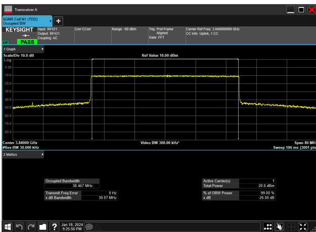
40MHz_15kHz_3840MHz_CP-OFDM 64 QAM_RB216@0&38.467 MHz
