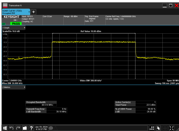
40MHz_15kHz_3840MHz_DFT-s-OFDM QPSK_RB216@0&38.514 MHz
