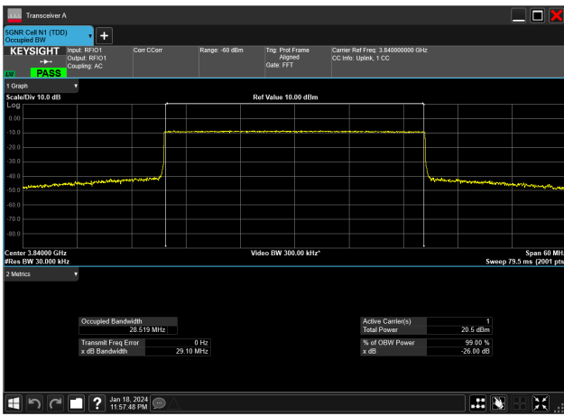
30MHz_15kHz_3840MHz_CP-OFDM QPSK_RB160@0&28.519 MHz
