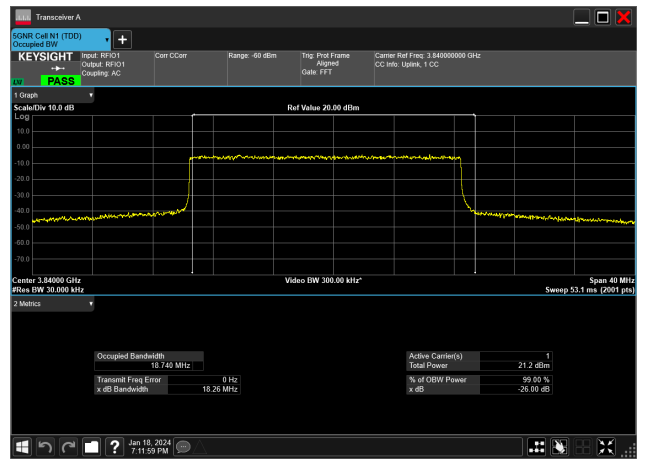
20MHz_15kHz_3840MHz_DFT-s-OFDM 64 QAM_RB100@0&18.740 MHz
