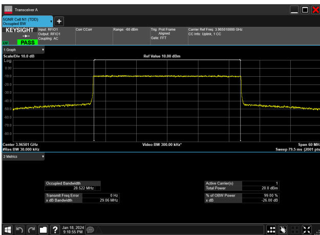
30MHz_15kHz_3965MHz_CP-OFDM 64 QAM_RB160@0&28.522 MHz
