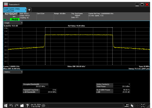
30MHz_15kHz_3840MHz_CP-OFDM 16 QAM_RB160@0&28.523 MHz
