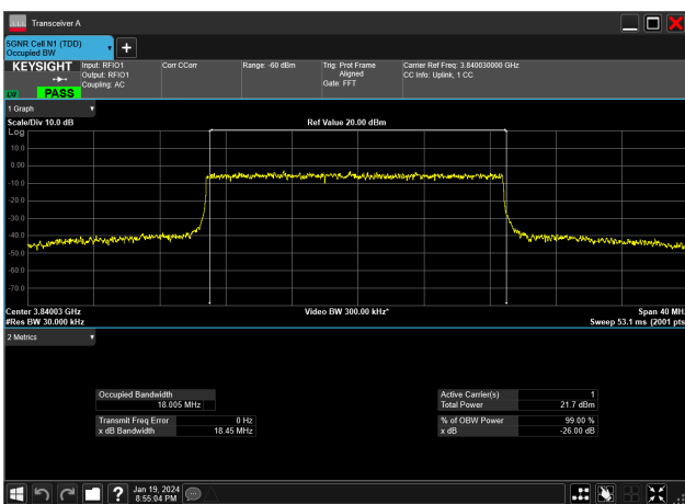
20MHz_30kHz_3840MHz_DFT-s-OFDM 16 QAM_RB50@0&18.005 MHz
