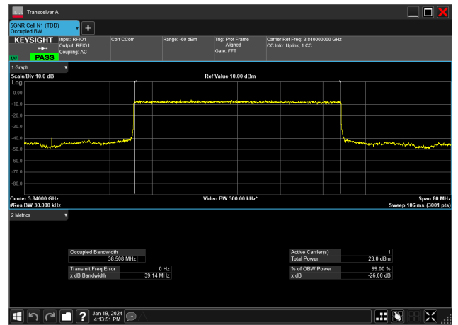
40MHz_15kHz_3840MHz_DFT-s-OFDM PI/2 BPSK_RB216@0&38.508 MHz
