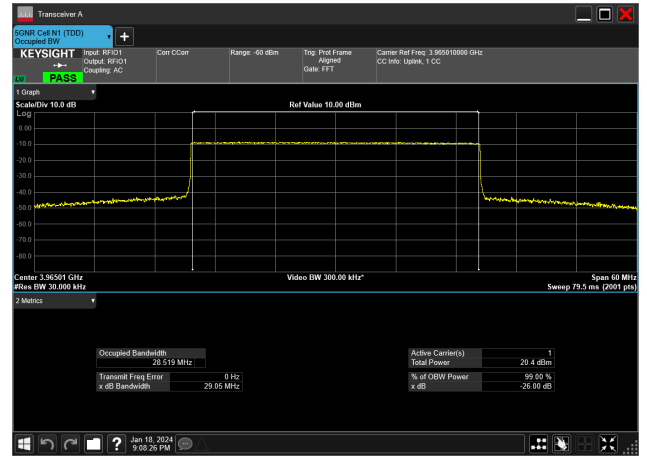
30MHz_15kHz_3965MHz_CP-OFDM QPSK_RB160@0&28.519 MHz
