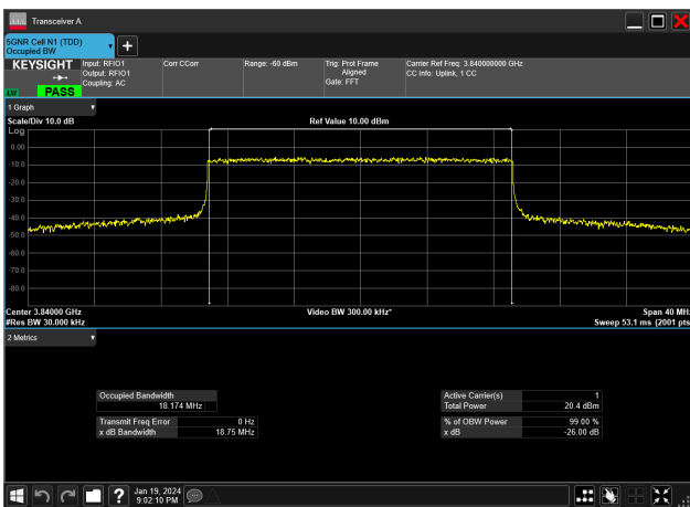
20MHz_30kHz_3840MHz_CP-OFDM 64 QAM_RB51@0&18.174 MHz
