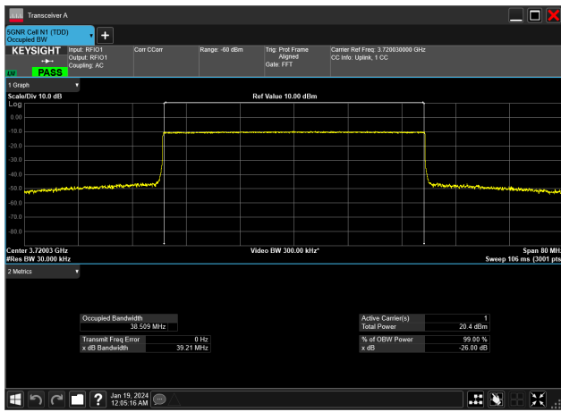
40MHz_15kHz_3720MHz_CP-OFDM QPSK_RB216@0&38.509 MHz
