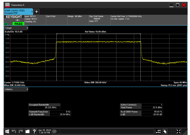
30MHz_15kHz_3715MHz_DFT-s-OFDM PI/2 BPSK_RB160@0&28.525 MHz
