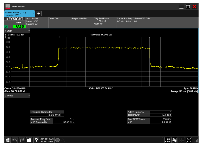
40MHz_15kHz_3840MHz_DFT-s-OFDM 256 QAM_RB216@0&38.510 MHz
