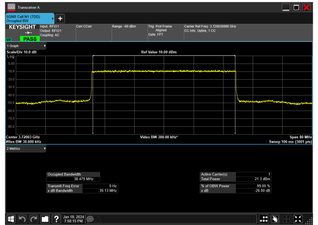
40MHz_15kHz_3720MHz_DFT-s-OFDM 16 QAM_RB216@0&38.479 MHz
