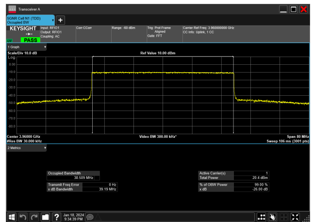
40MHz_15kHz_3960MHz_CP-OFDM 16 QAM_RB216@0&38.509 MHz
