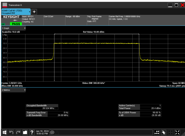
30MHz_15kHz_3965MHz_CP-OFDM 16 QAM_RB160@0&28.524 MHz
