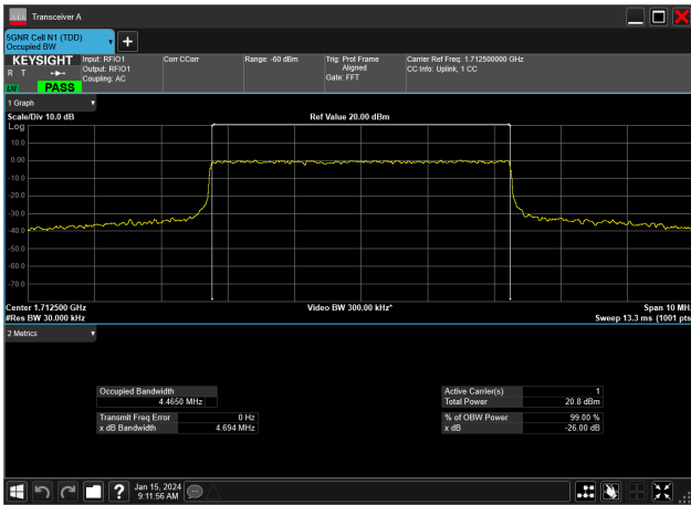
5MHz_15kHz_1712.5MHz_CP-OFDM 16 QAM_RB25@0&4.465 MHz
