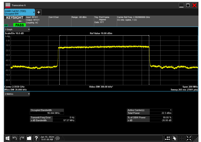
100MHz_30kHz_2592.99MHz_DFT-s-OFDM PI/2 BPSK_RB270@0&95.844 MHz
