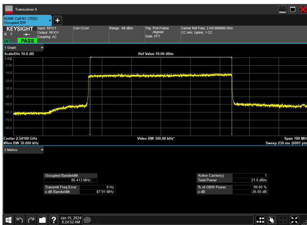
90MHz_30kHz_2541MHz_DFT-s-OFDM QPSK_RB243@0&86.413 MHz
