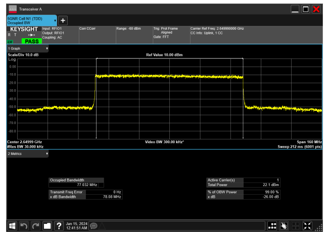
80MHz_30kHz_2649.99MHz_DFT-s-OFDM QPSK_RB216@0&77.032 MHz
