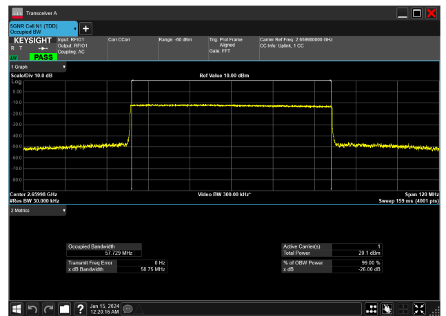
60MHz_30kHz_2659.98MHz_CP-OFDM QPSK_RB162@0&57.729 MHz
