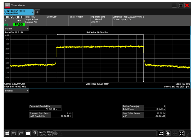
80MHz_30kHz_2592.99MHz_DFT-s-OFDM 256 QAM_RB216@0&76.826 MHz
