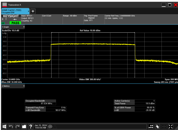
100MHz_30kHz_2640MHz_CP-OFDM QPSK_RB273@0&97.034 MHz
