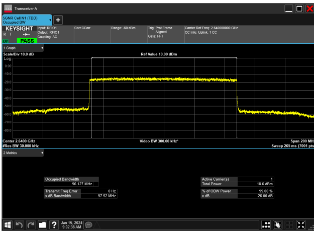
100MHz_30kHz_2640MHz_DFT-s-OFDM 256 QAM_RB270@0&96.127 MHz
