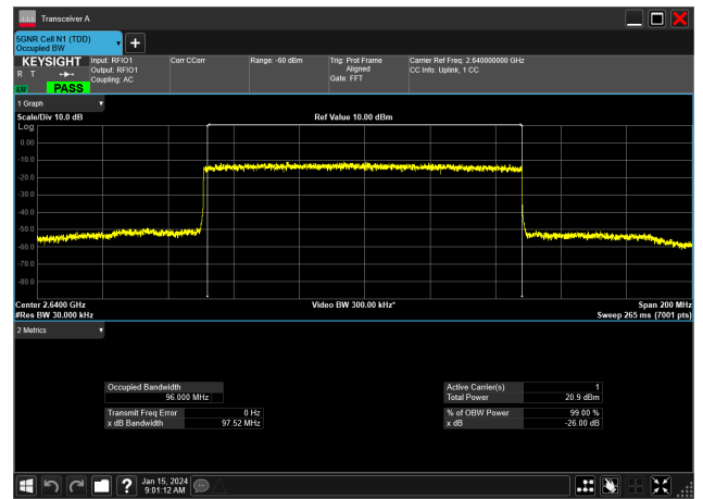
100MHz_30kHz_2640MHz_DFT-s-OFDM 16 QAM_RB270@0&96.000 MHz
