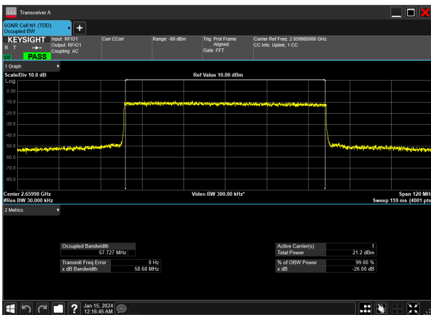
60MHz_30kHz_2659.98MHz_DFT-s-OFDM 16 QAM_RB162@0&57.727 MHz
