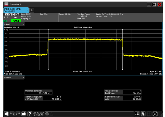
100MHz_30kHz_2640MHz_DFT-s-OFDM 64 QAM_RB270@0&96.070 MHz
