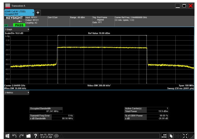
90MHz_30kHz_2644.98MHz_CP-OFDM QPSK_RB245@0&87.241 MHz
