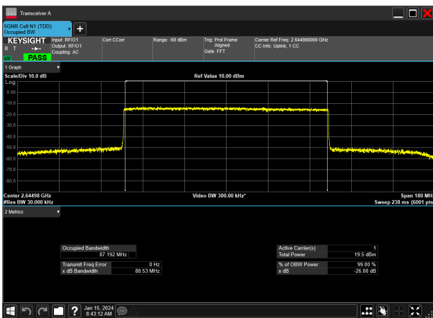
90MHz_30kHz_2644.98MHz_CP-OFDM 64 QAM_RB245@0&87.192 MHz
