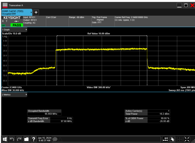
100MHz_30kHz_2546.01MHz_DFT-s-OFDM 256 QAM_RB270@0&95.959 MHz
