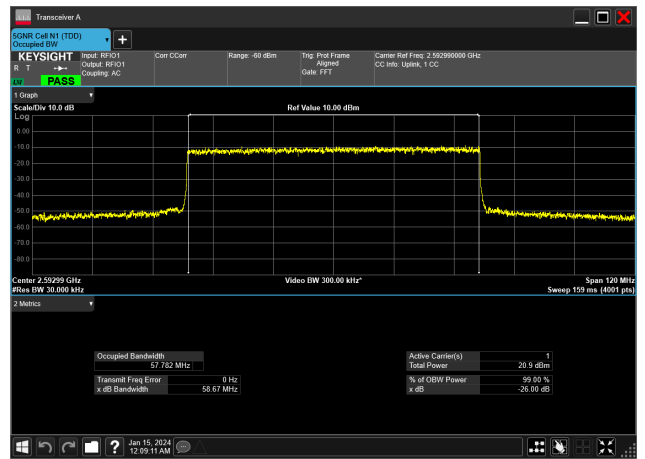
60MHz_30kHz_2592.99MHz_DFT-s-OFDM 16 QAM_RB162@0&57.782 MHz
