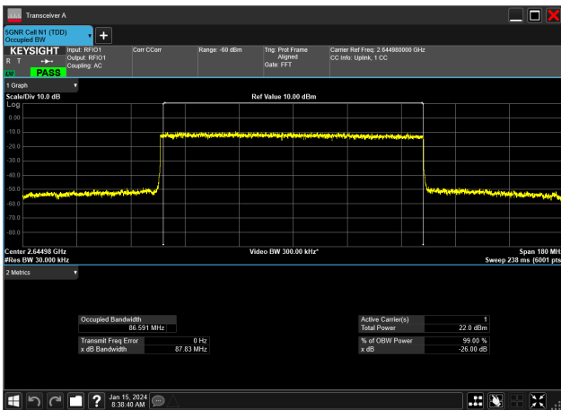
90MHz_30kHz_2644.98MHz_DFT-s-OFDM QPSK_RB243@0&86.591 MHz
