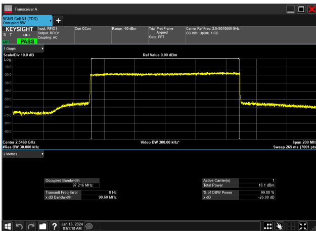
100MHz_30kHz_2546.01MHz_CP-OFDM 256 QAM_RB273@0&97.216 MHz
