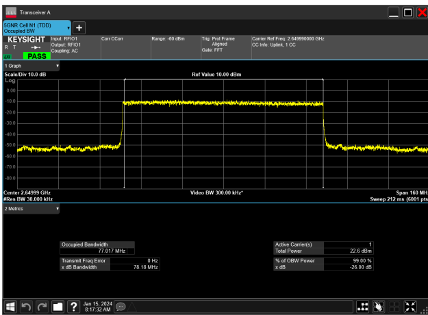
80MHz_30kHz_2649.99MHz_DFT-s-OFDM PI/2 BPSK_RB216@0&77.017 MHz
