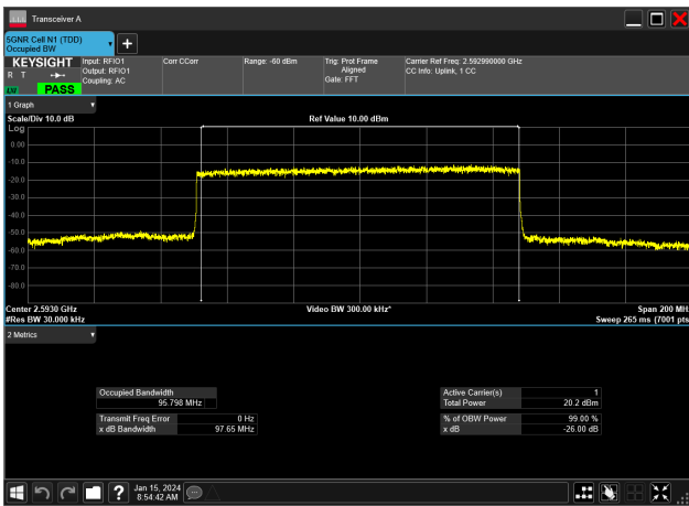
100MHz_30kHz_2592.99MHz_DFT-s-OFDM 64 QAM_RB270@0&95.798 MHz
