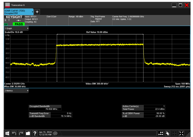
80MHz_30kHz_2592.99MHz_DFT-s-OFDM 1/2 BPSK_RB216@0&76.858 MHz
