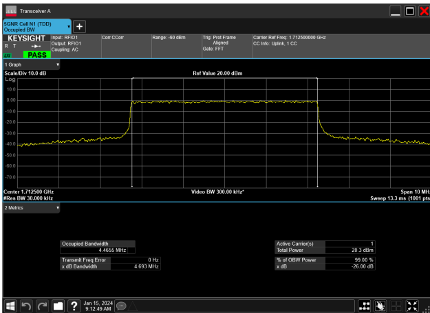
5MHz_15kHz_1712.5MHz_CP-OFDM 64 QAM_RB25@0&4.466 MHz
