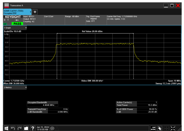
5MHz_15kHz_1712.5MHz_DFT-s-OFDM 256 QAM_RB25@0&4.465 MHz
