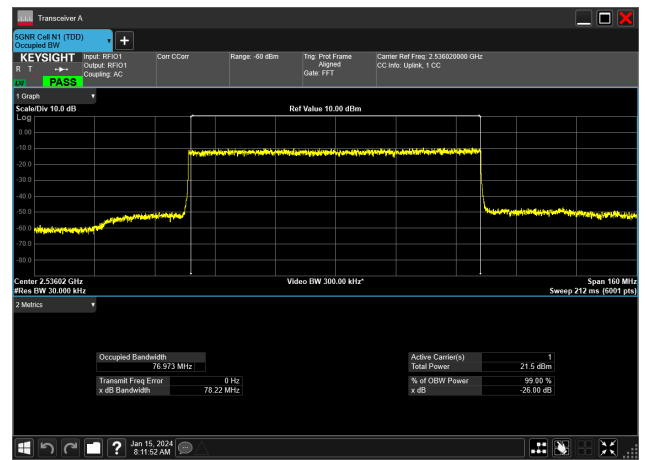
80MHz_30kHz_2536.02MHz_DFT-s-OFDM QPSK_RB216@0&76.973 MHz
