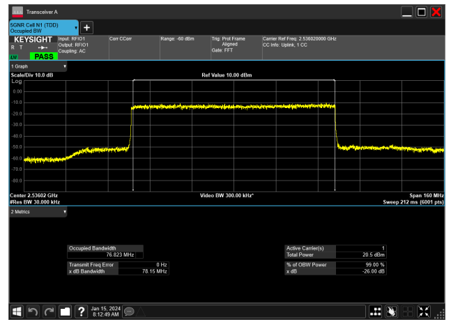
80MHz_30kHz_2536.02MHz_DFT-s-OFDM 16 QAM_RB216@0&76.823 MHz
