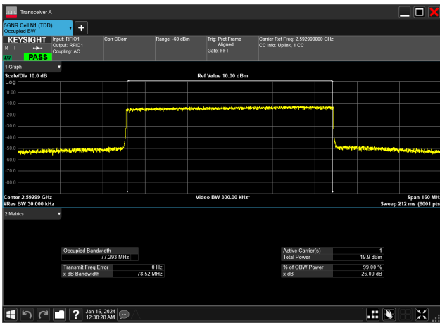
80MHz_30kHz_2592.99MHz_CP-OFDM 16 QAM_RB217@0&77.293 MHz
