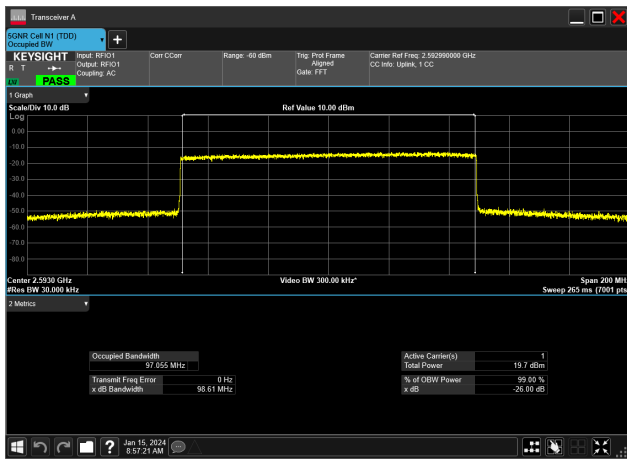
100MHz_30kHz_2592.99MHz_CP-OFDM 16 QAM_RB273@0&97.055 MHz
