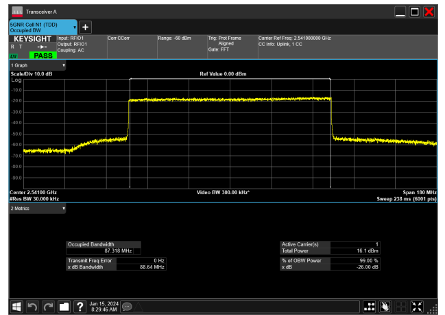
90MHz_30kHz_2541MHz_CP-OFDM 256 QAM_RB245@0&87.318 MHz
