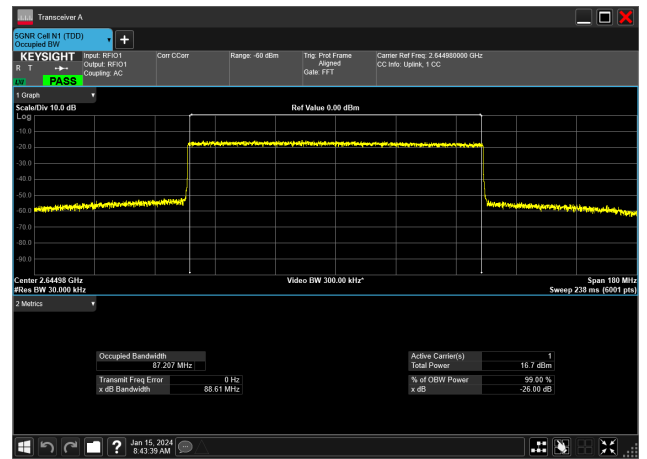
90MHz_30kHz_2644.98MHz_CP-OFDM 256 QAM_RB245@0&87.207 MHz
