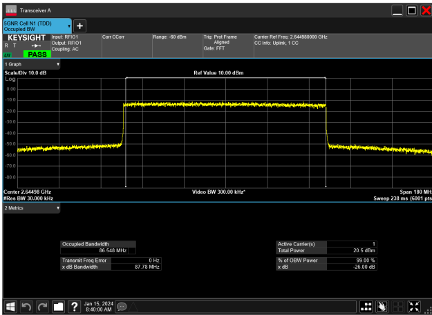
90MHz_30kHz_2644.98MHz_DFT-s-OFDM 64 QAM_RB243@0&86.548 MHz
