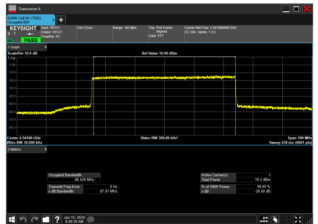
90MHz_30kHz_2541MHz_DFT-s-OFDM 256 QAM_RB243@0&86.429 MHz
