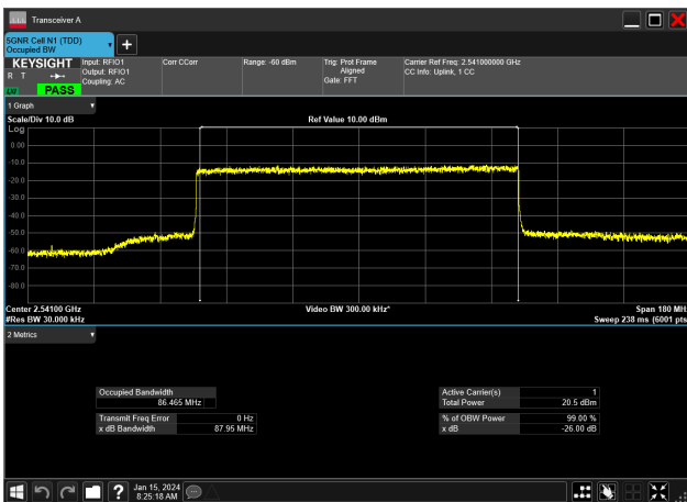
90MHz_30kHz_2541MHz_DFT-s-OFDM 16 QAM_RB243@0&86.465 MHz
