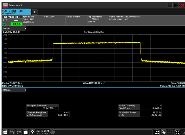
90MHz_30kHz_2592.99MHz_CP-OFDM 256 QAM_RB245@0&87.242 MHz
