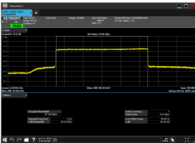
90MHz_30kHz_2541MHz_CP-OFDM 64 QAM_RB245@0&87.308 MHz
