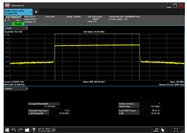
80MHz_30kHz_2592.99MHz_CP-OFDM QPSK_RB217@0&77.295 MHz
