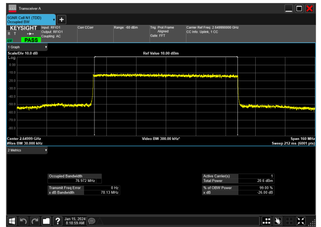
80MHz_30kHz_2649.99MHz_DFT-s-OFDM 64 QAM_RB216@0&76.972 MHz
