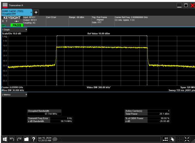
60MHz_30kHz_2659.98MHz_CP-OFDM 16 QAM_RB162@0&57.744 MHz
