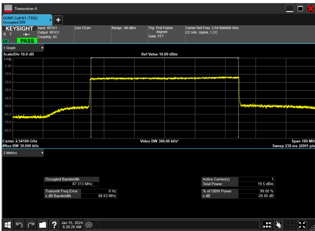
90MHz_30kHz_2541MHz_CP-OFDM 16 QAM_RB245@0&87.313 MHz
