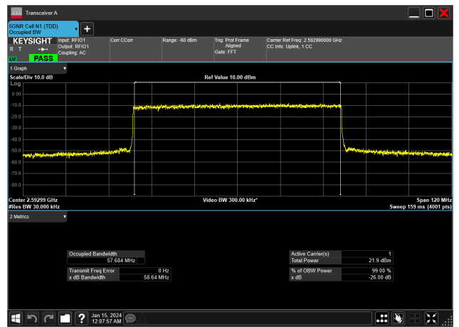
60MHz_30kHz_2592.99MHz_DFT-s-OFDM QPSK_RB162@0&57.684 MHz
