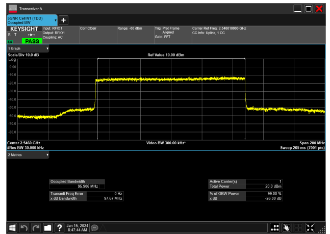
100MHz_30kHz_2546.01MHz_DFT-s-OFDM 64 QAM_RB270@0&95.906 MHz
