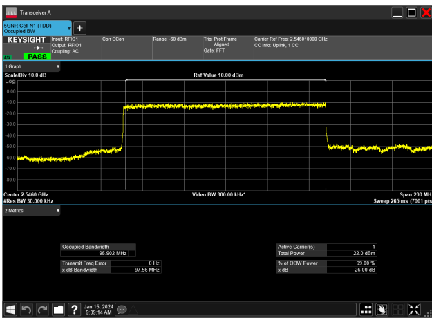
100MHz_30kHz_2546.01MHz_DFT-s-OFDM PI/2 BPSK_RB270@0&95.902 MHz
