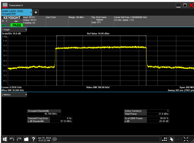
100MHz_30kHz_2592.99MHz_DFT-s-OFDM QPSK_RB270@0&95.789 MHz
