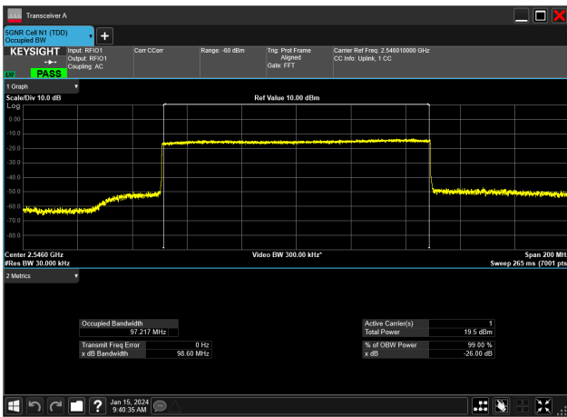
100MHz_30kHz_2546.01MHz_CP-OFDM QPSK_RB273@0&97.217 MHz
