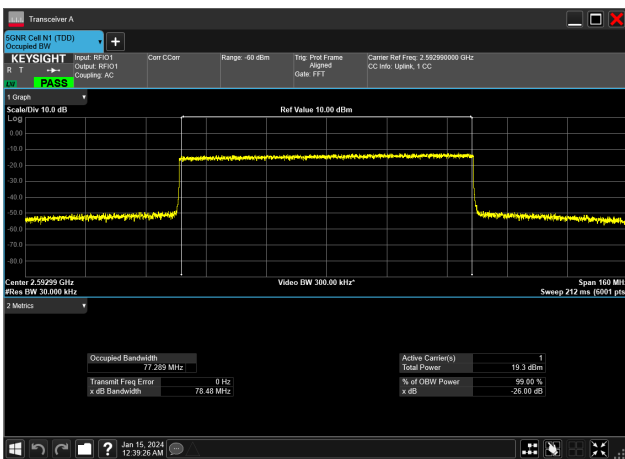
80MHz_30kHz_2592.99MHz_CP-OFDM 64 QAM_RB217@0&77.289 MHz
