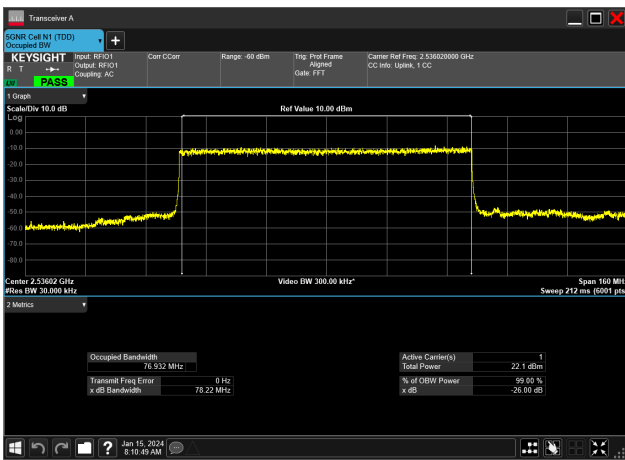
80MHz_30kHz_2536.02MHz_DFT-s-OFDM PI/2 BPSK_RB216@0&76.932 MHz
