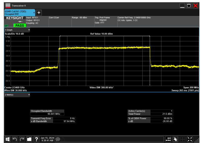
100MHz_30kHz_2546.01MHz_DFT-s-OFDM QPSK_RB270@0&95.841 MHz
