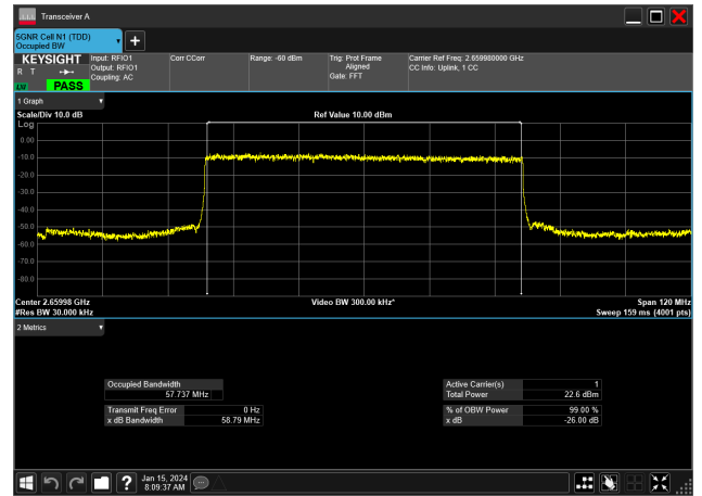
60MHz_30kHz_2659.98MHz_DFT-s-OFDM 16/2 BPSK_RB162@0&57.737 MHz
