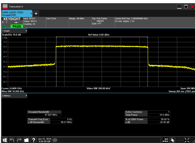
100MHz_30kHz_2640MHz_CP-OFDM 256 QAM_RB273@0&97.087 MHz
