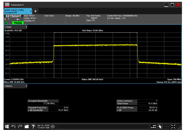
80MHz_30kHz_2592.99MHz_CP-OFDM 256 QAM_RB217@0&77.296 MHz
