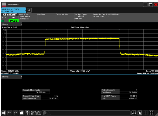
80MHz_30kHz_2592.99MHz_DFT-s-OFDM 16 QAM_RB216@0&76.757 MHz
