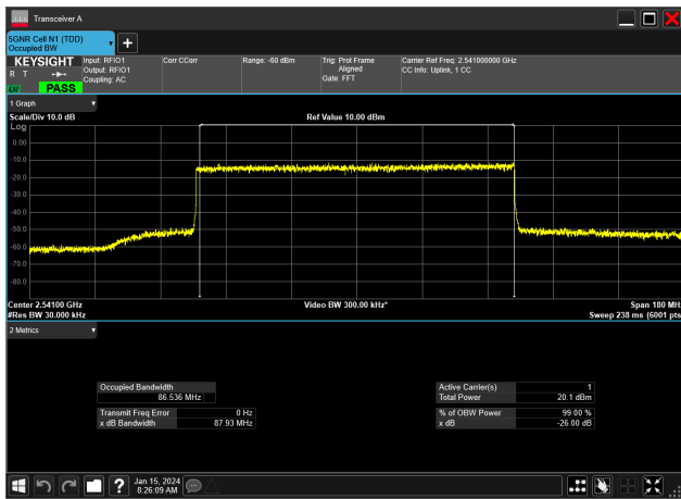
90MHz_30kHz_2541MHz_DFT-s-OFDM 64 QAM_RB243@0&86.536 MHz
