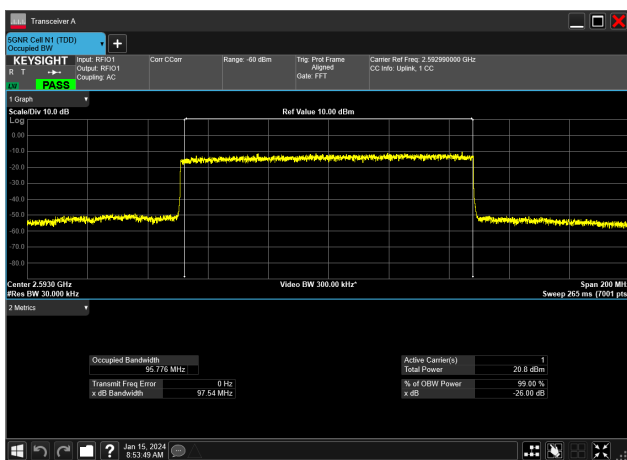
100MHz_30kHz_2592.99MHz_DFT-s-OFDM 16 QAM_RB270@0&95.776 MHz
