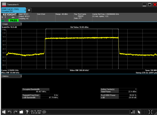
90MHz_30kHz_2592.99MHz_DFT-s-OFDM PI/2 BPSK_RB243@0&86.407 MHz
