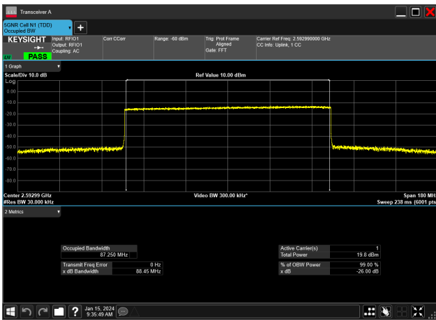
90MHz_30kHz_2592.99MHz_CP-OFDM QPSK_RB245@0&87.250 MHz
