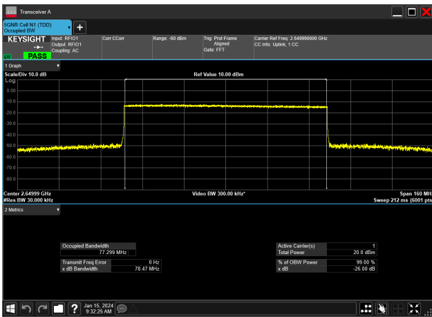
80MHz_30kHz_2649.99MHz_CP-OFDM QPSK_RB217@0&77.299 MHz
