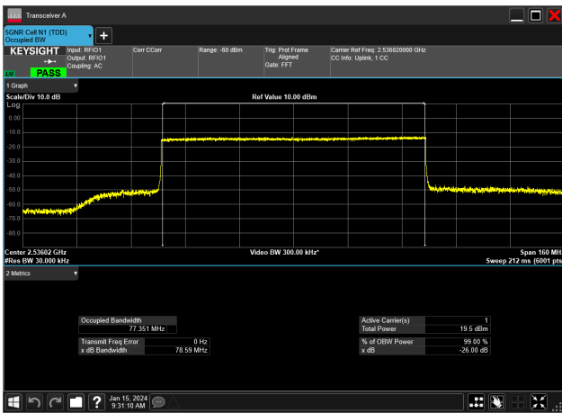
80MHz_30kHz_2536.02MHz_CP-OFDM QPSK_RB217@0&77.351 MHz
