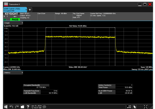
60MHz_30kHz_2659.98MHz_DFT-s-OFDM 256 QAM_RB162@0&57.739 MHz
