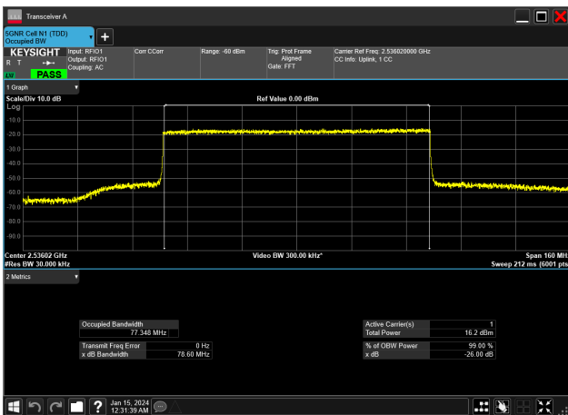
80MHz_30kHz_2536.02MHz_CP-OFDM 256 QAM_RB217@0&77.348 MHz
