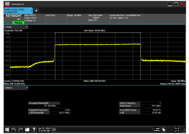
90MHz_30kHz_2541MHz_CP-OFDM QPSK_RB245@0&87.320 MHz
