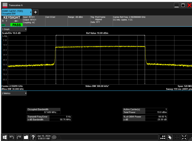
60MHz_30kHz_2592.99MHz_CP-OFDM QPSK_RB162@0&57.689 MHz
