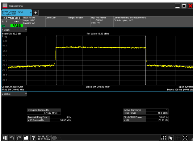
60MHz_30kHz_2659.98MHz_CP-OFDM 64 QAM_RB162@0&57.683 MHz
