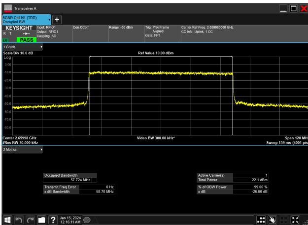
60MHz_30kHz_2659.98MHz_DFT-s-OFDM QPSK_RB162@0&57.724 MHz
