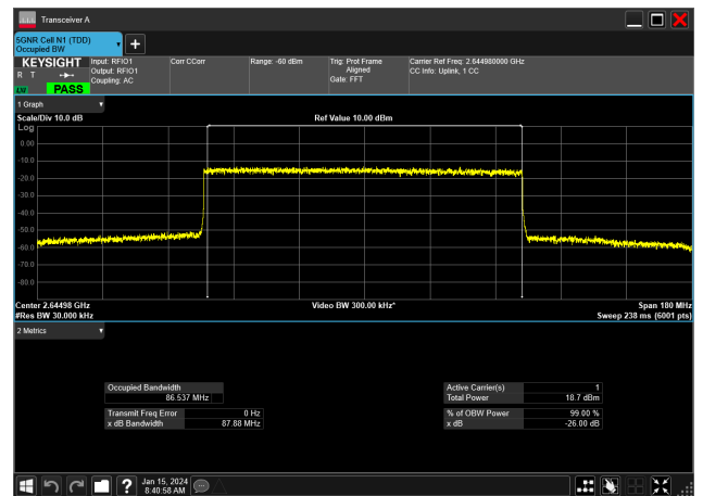
90MHz_30kHz_2644.98MHz_DFT-s-OFDM 256 QAM_RB243@0&86.537 MHz
