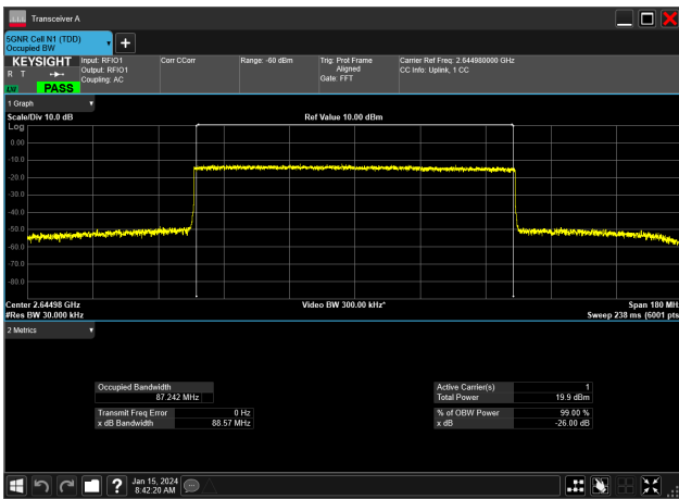
90MHz_30kHz_2644.98MHz_CP-OFDM 16 QAM_RB245@0&87.242 MHz
