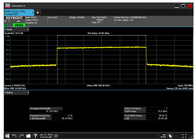
90MHz_30kHz_2592.99MHz_CP-OFDM 16 QAM_RB245@0&87.255 MHz
