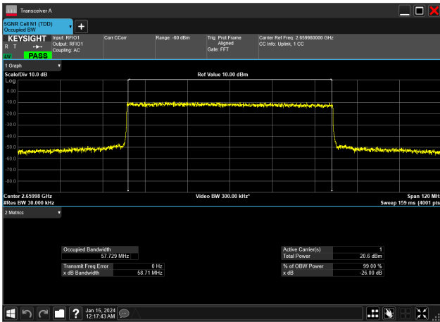
60MHz_30kHz_2659.98MHz_DFT-s-OFDM 64 QAM_RB162@0&57.729 MHz
