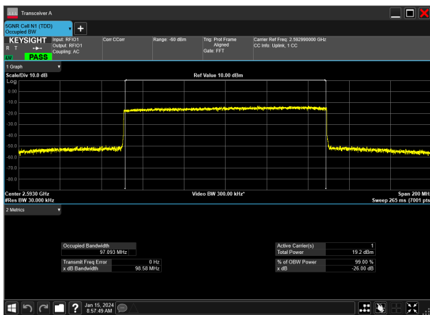
100MHz_30kHz_2592.99MHz_CP-OFDM 64 QAM_RB273@0&97.093 MHz
