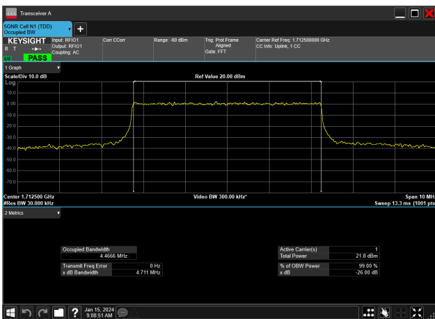
5MHz_15kHz_1712.5MHz_DFT-s-OFDM 16 QAM_RB25@0&4.467 MHz
