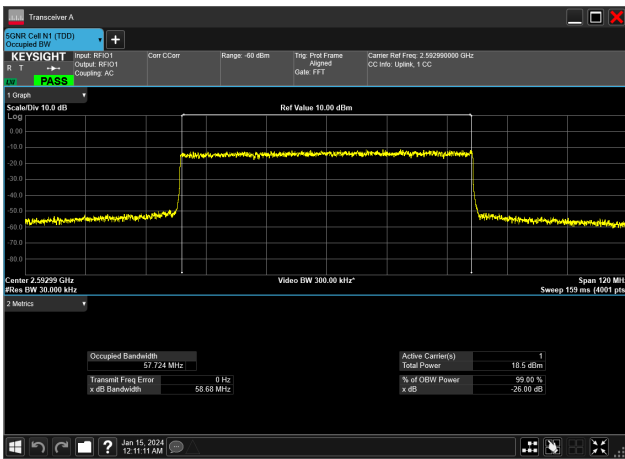
60MHz_30kHz_2592.99MHz_DFT-s-OFDM 256 QAM_RB162@0&57.724 MHz
