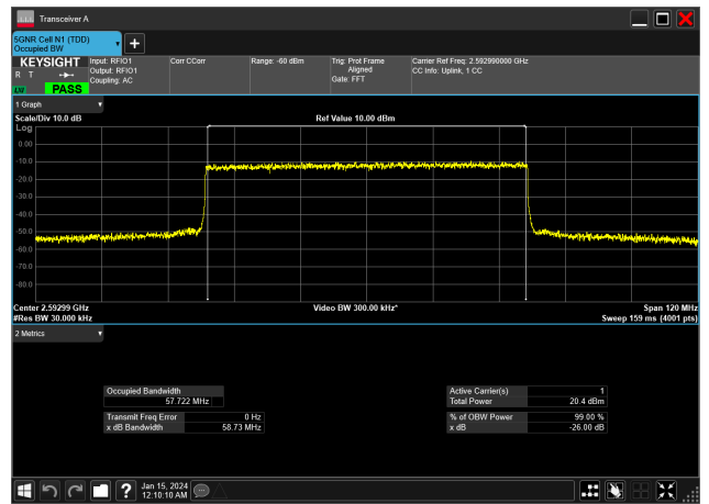
60MHz_30kHz_2592.99MHz_DFT-s-OFDM 64 QAM_RB162@0&57.722 MHz
