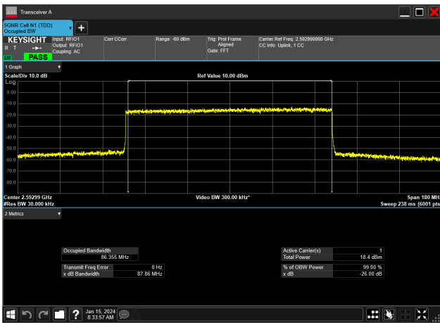
90MHz_30kHz_2592.99MHz_DFT-s-OFDM 256 QAM_RB243@0&86.355 MHz
