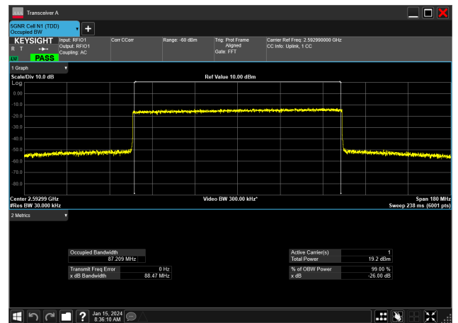
90MHz_30kHz_2592.99MHz_CP-OFDM 64 QAM_RB245@0&87.209 MHz
