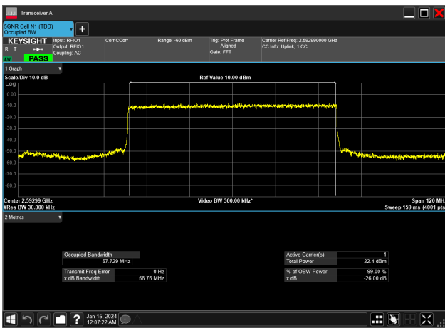
60MHz_30kHz_2592.99MHz_DFT-s-OFDM PI/2 BPSK_RB162@0&57.729 MHz
