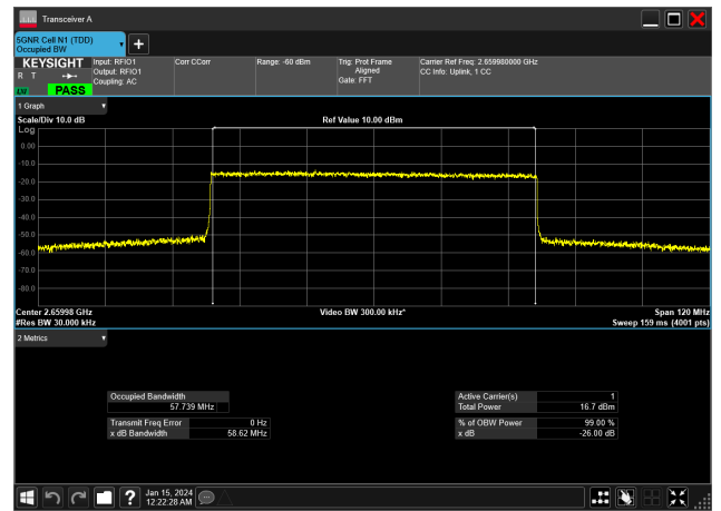
60MHz_30kHz_2659.98MHz_CP-OFDM 256 QAM_RB162@0&57.739 MHz
