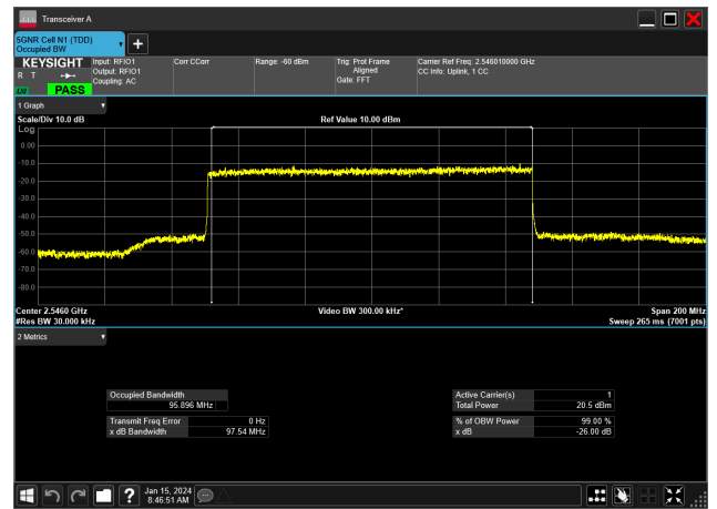
100MHz_30kHz_2546.01MHz_DFT-s-OFDM 16 QAM_RB270@0&95.896 MHz
