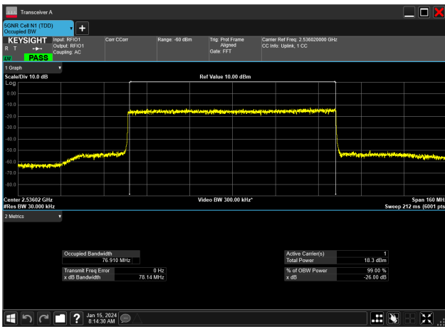
80MHz_30kHz_2536.02MHz_DFT-s-OFDM 256 QAM_RB216@0&76.910 MHz
