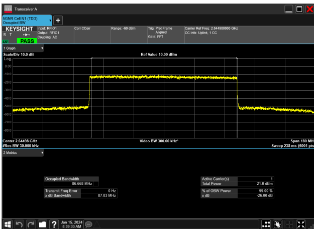
90MHz_30kHz_2644.98MHz_DFT-s-OFDM 16 QAM_RB243@0&86.668 MHz
