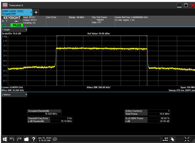
80MHz_30kHz_2649.99MHz_DFT-s-OFDM 256 QAM_RB216@0&76.928 MHz
