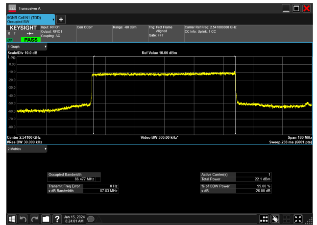
90MHz_30kHz_2541MHz_DFT-s-OFDM PI/2 BPSK_RB243@0&86.477 MHz
