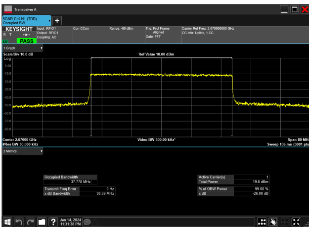
40MHz_30kHz_2670MHz_CP-OFDM 64 QAM_RB106@0&37.778 MHz
