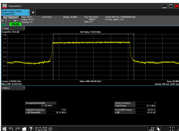
40MHz_30kHz_2592.99MHz_DFT-s-OFDM PI/2 BPSK_RB100@0&amp;37.356 MHz
