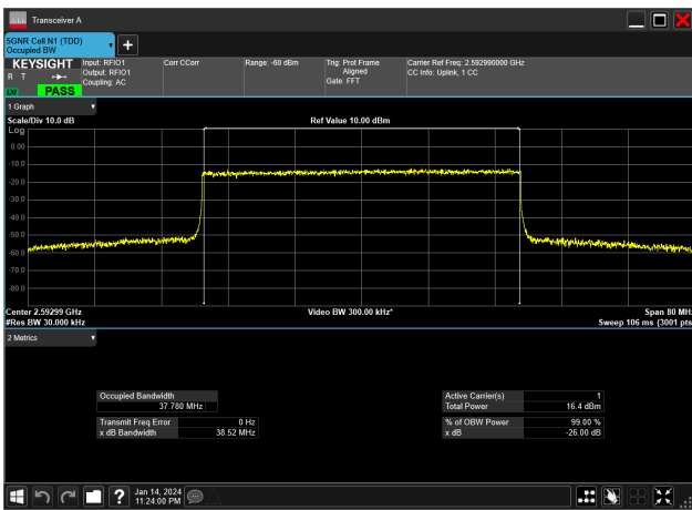
40MHz_30kHz_2592.99MHz_CP-OFDM 256 QAM_RB106@0&37.780 MHz
