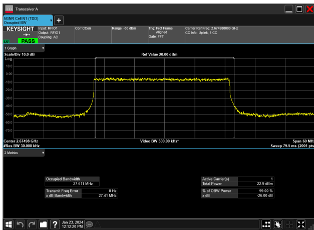
30MHz_30kHz_2674.98MHz_DFT-s-OFDM PI/2 BPSK_RB75@0&27.611 MHz
