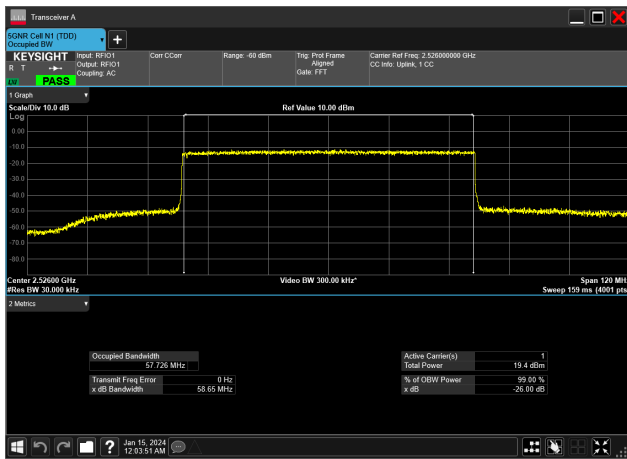
60MHz_30kHz_2526MHz_CP-OFDM 16 QAM_RB162@0&57.726 MHz
