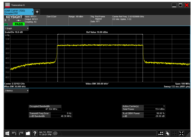
50MHz_30kHz_2521.02MHz_CP-OFDM 16 QAM_RB133@0&47.354 MHz
