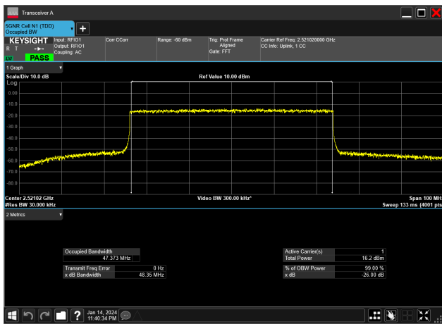
50MHz_30kHz_2521.02MHz_CP-OFDM 256 QAM_RB133@0&47.373 MHz
