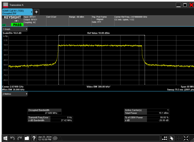
30MHz_30kHz_2674.98MHz_DFT-s-OFDM 256 QAM_RB75@0&27.689 MHz
