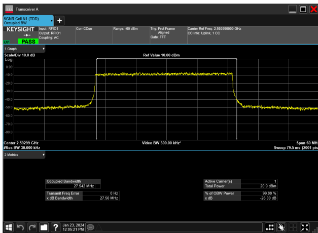
30MHz_30kHz_2592.99MHz_DFT-s-OFDM 16 QAM_RB75@0&27.542 MHz
