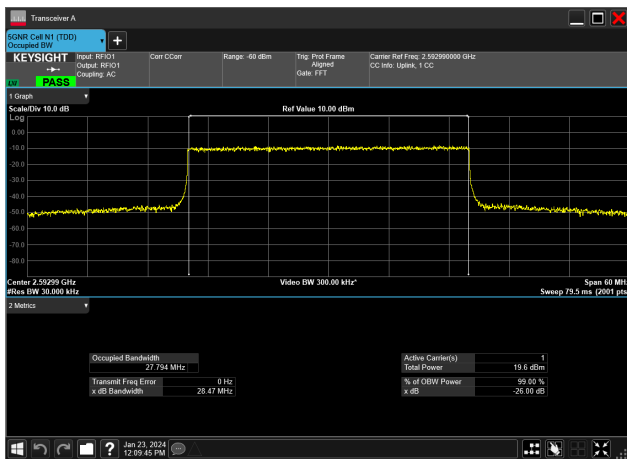
30MHz_30kHz_2592.99MHz_CP-OFDM 64 QAM_RB78@0&27.794 MHz
