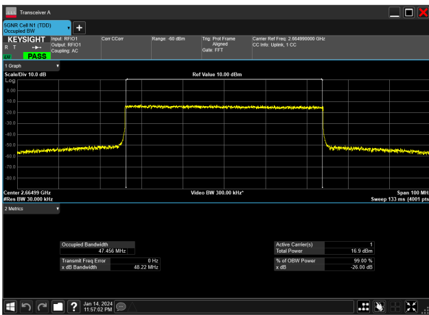
50MHz_30kHz_2664.99MHz_CP-OFDM 256 QAM_RB133@0&47.456 MHz
