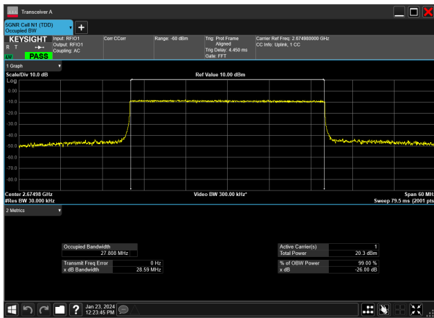
30MHz_30kHz_2674.98MHz_CP-OFDM QPSK_RB78@0&27.808 MHz
