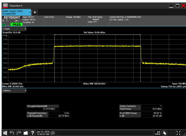
60MHz_30kHz_2526MHz_CP-OFDM 64 QAM_RB162@0&57.674 MHz
