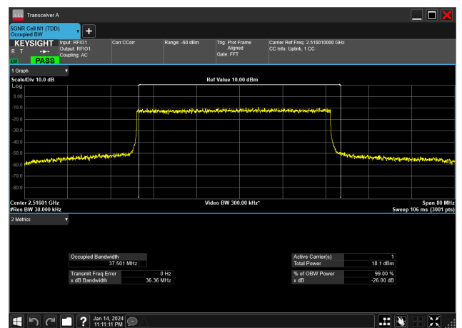
40MHz_30kHz_2516.01MHz_DFT-s-OFDM 256 QAM_RB100@0&37.501 MHz
