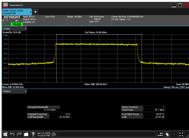
40MHz_30kHz_2670MHz_DFT-s-OFDM 64 QAM_RB100@0&37.515 MHz
