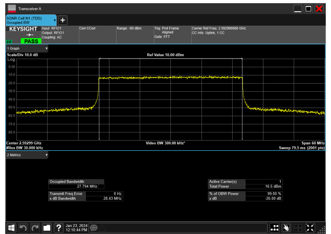
30MHz_30kHz_2592.99MHz_CP-OFDM 256 QAM_RB78@0&27.794 MHz
