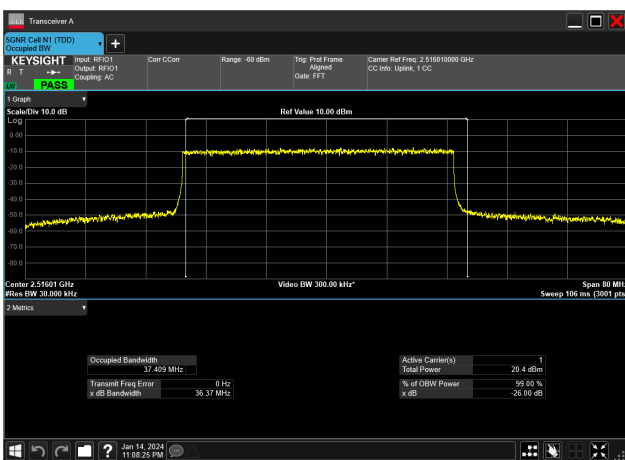
40MHz_30kHz_2516.01MHz_DFT-s-OFDM 16 QAM_RB100@0&37.409 MHz
