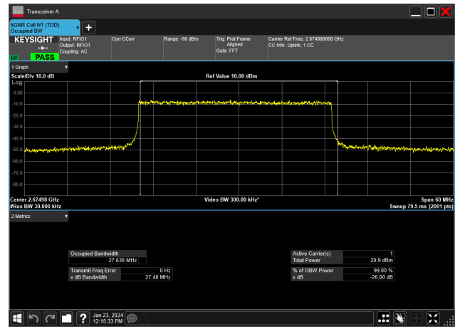
30MHz_30kHz_2674.98MHz_DFT-s-OFDM 64 QAM_RB75@0&27.630 MHz
