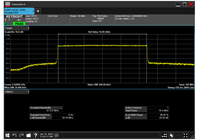
60MHz_30kHz_2526MHz_CP-OFDM QPSK_RB162@0&57.672 MHz
