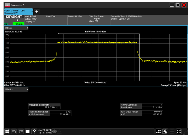
30MHz_30kHz_2674.98MHz_DFT-s-OFDM 16 QAM_RB75@0&27.617 MHz
