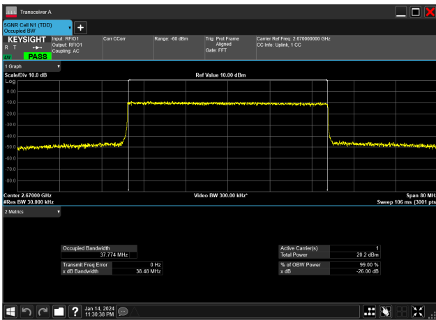
40MHz_30kHz_2670MHz_CP-OFDM 16 QAM_RB106@0&37.774 MHz
