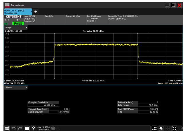
60MHz_30kHz_2526MHz_DFT-s-OFDM 256 QAM_RB162@0&57.688 MHz
