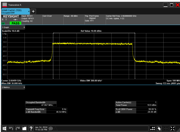
50MHz_30kHz_2664.99MHz_DFT-s-OFDM 256 QAM_RB128@0&47.067 MHz
