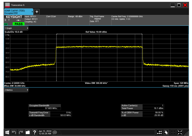
60MHz_30kHz_2526MHz_CP-OFDM 256 QAM_RB162@0&57.683 MHz
