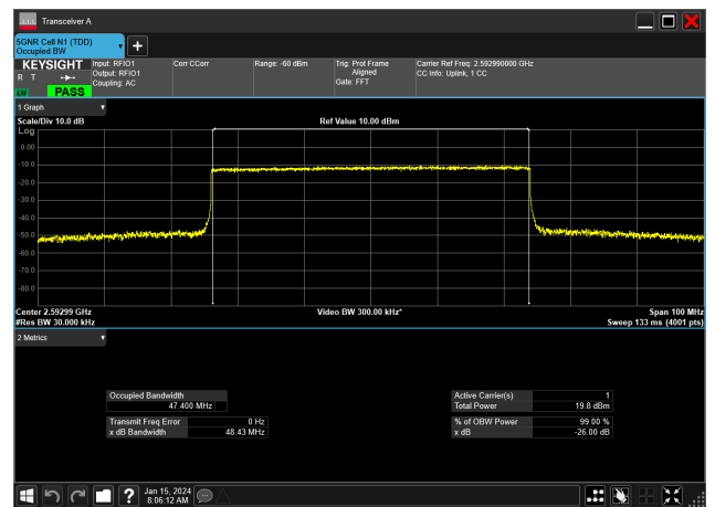
50MHz_30kHz_2592.99MHz_CP-OFDM QPSK_RB133@0&47.400 MHz
