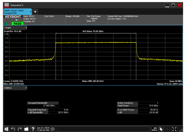
30MHz_30kHz_2592.99MHz_CP-OFDM QPSK_RB78@0&27.805 MHz
