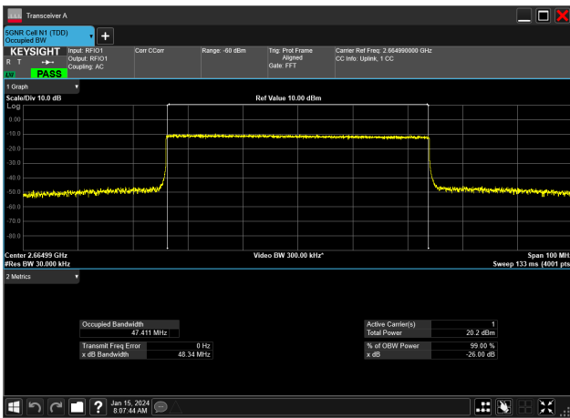
50MHz_30kHz_2664.99MHz_CP-OFDM QPSK_RB133@0&47.411 MHz
