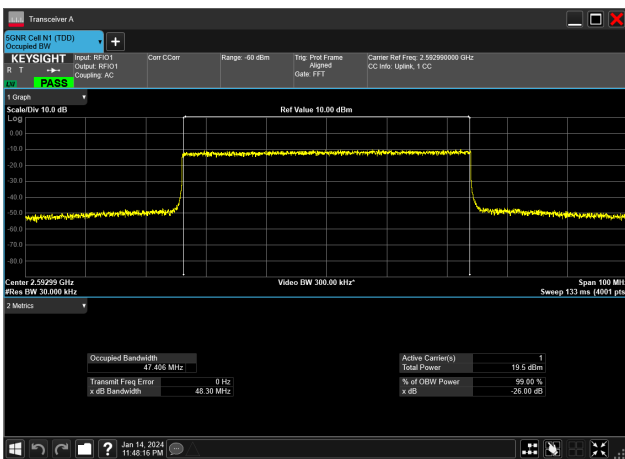
50MHz_30kHz_2592.99MHz_CP-OFDM 64 QAM_RB133@0&47.406 MHz
