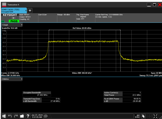
30MHz_30kHz_2511MHz_DFT-s-OFDM PI/2 BPSK_RB75@0&27.492 MHz
