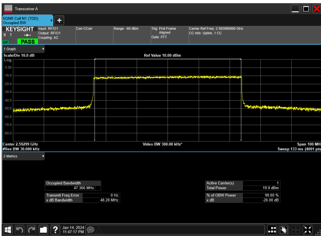
50MHz_30kHz_2592.99MHz_CP-OFDM 16 QAM_RB133@0&47.366 MHz
