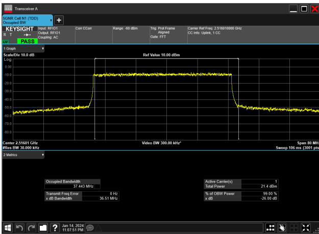
40MHz_30kHz_2516.01MHz_DFT-s-OFDM QPSK_RB100@0&37.443 MHz
