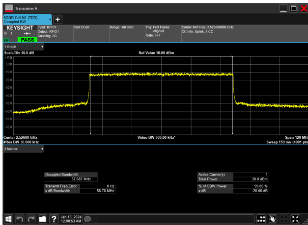
60MHz_30kHz_2526MHz_DFT-s-OFDM 64 QAM_RB162@0&57.687 MHz
