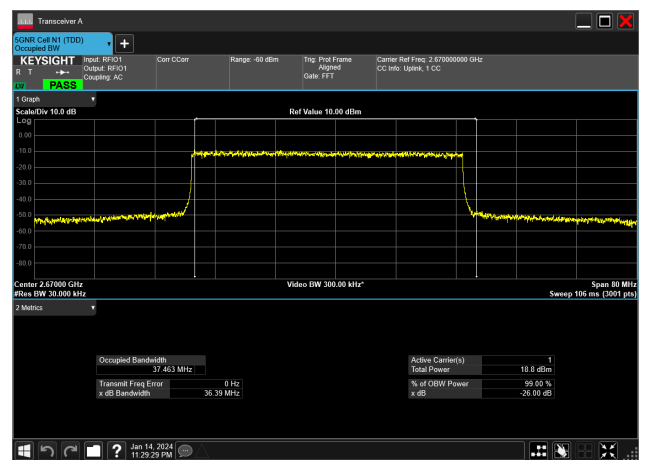
40MHz_30kHz_2670MHz_DFT-s-OFDM 256 QAM_RB100@0&37.463 MHz
