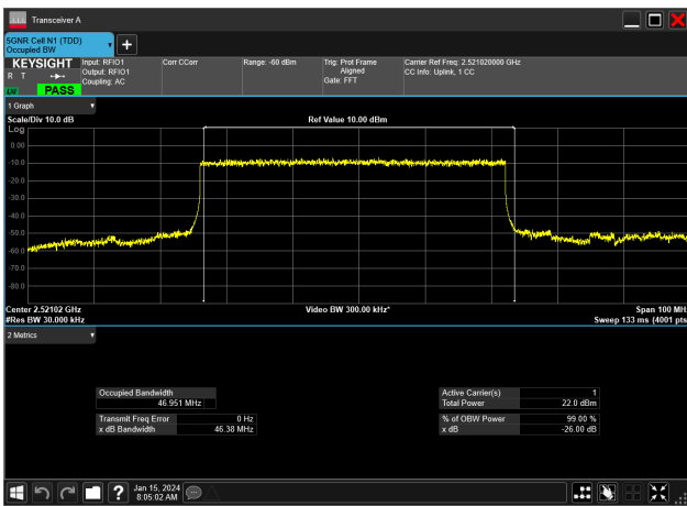
50MHz_30kHz_2521.02MHz_DFT-s-OFDM PI/2 BPSK_RB128@0&46.951 MHz
