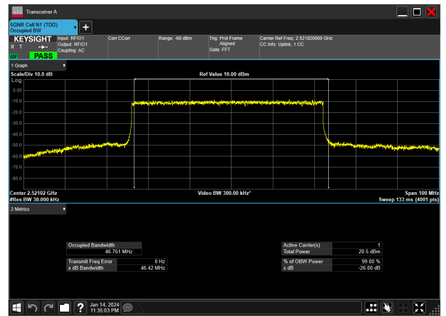
50MHz_30kHz_2521.02MHz_DFT-s-OFDM 16 QAM_RB128@0&46.761 MHz
