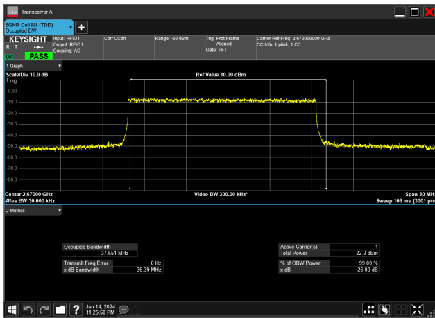
40MHz_30kHz_2670MHz_DFT-s-OFDM QPSK_RB100@0&37.551 MHz
