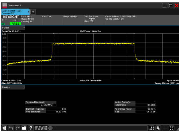
40MHz_30kHz_2516.01MHz_CP-OFDM 64 QAM_RB106@0&37.762 MHz
