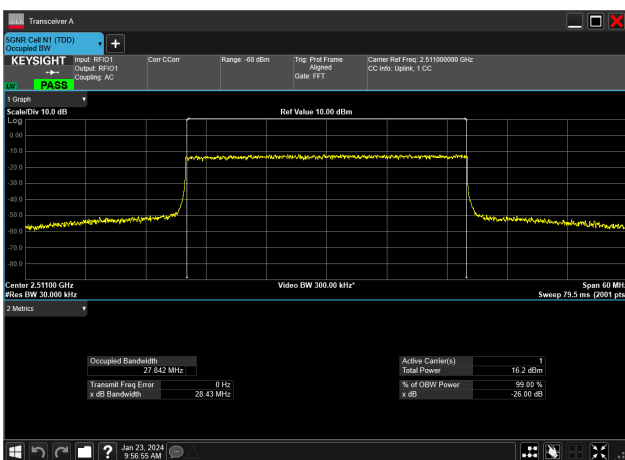
30MHz_30kHz_2511MHz_CP-OFDM 256 QAM_RB78@0&27.842 MHz
