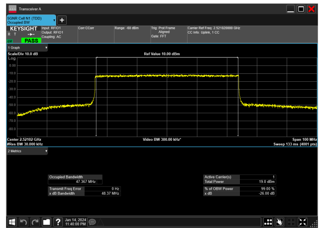
50MHz_30kHz_2521.02MHz_CP-OFDM 64 QAM_RB133@0&47.367 MHz
