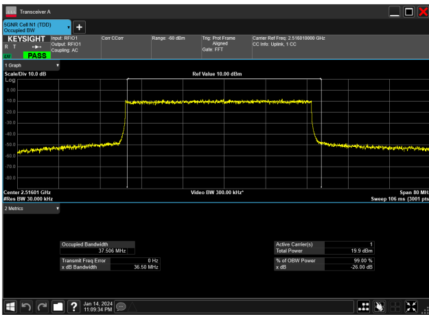
40MHz_30kHz_2516.01MHz_DFT-s-OFDM 64 QAM_RB100@0&37.506 MHz
