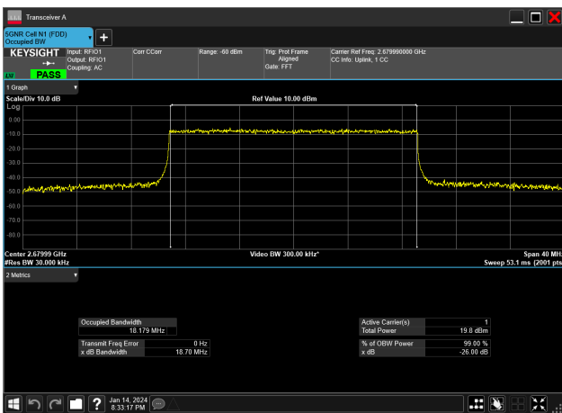
20MHz_30kHz_2679.99MHz_CP-OFDM 64 QAM_RB51@0&18.179 MHz
