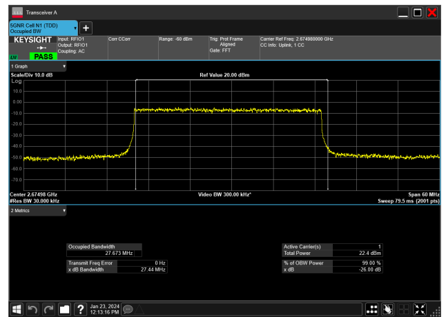
30MHz_30kHz_2674.98MHz_DFT-s-OFDM QPSK_RB75@0&27.673 MHz
