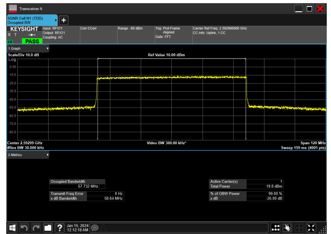
60MHz_30kHz_2592.99MHz_CP-OFDM 16 QAM_RB162@0&57.732 MHz
