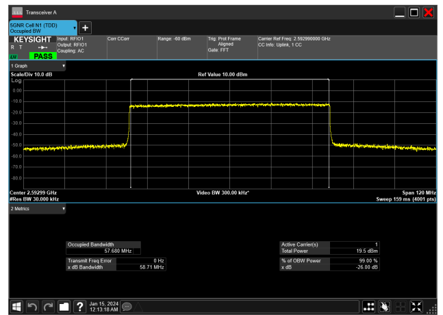
60MHz_30kHz_2592.99MHz_CP-OFDM 64 QAM_RB162@0&57.680 MHz
