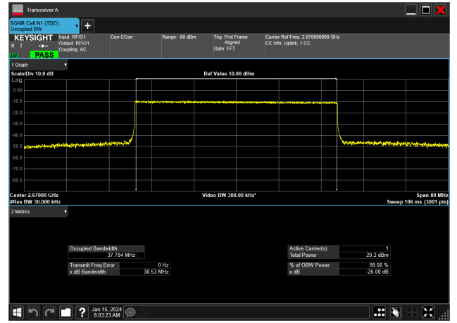
40MHz_30kHz_2670MHz_CP-OFDM QPSK_RB106@0&37.784 MHz
