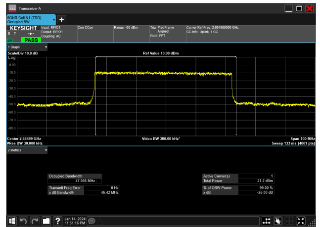
50MHz_30kHz_2664.99MHz_DFT-s-OFDM 16 QAM_RB128@0&47.065 MHz
