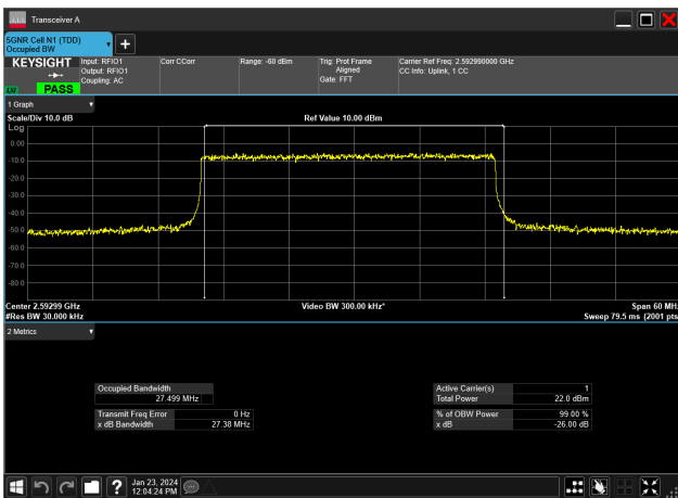
30MHz_30kHz_2592.99MHz_DFT-s-OFDM QPSK_RB75@0&27.499 MHz
