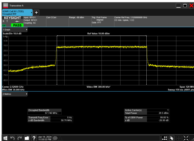
60MHz_30kHz_2526MHz_DFT-s-OFDM 16 QAM_RB162@0&57.746 MHz
