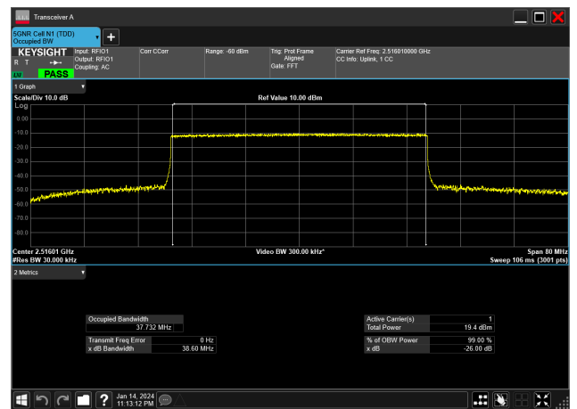
40MHz_30kHz_2516.01MHz_CP-OFDM QPSK_RB106@0&37.732 MHz
