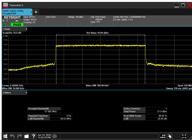
60MHz_30kHz_2526MHz_DFT-s-OFDM QPSK_RB162@0&57.685 MHz
