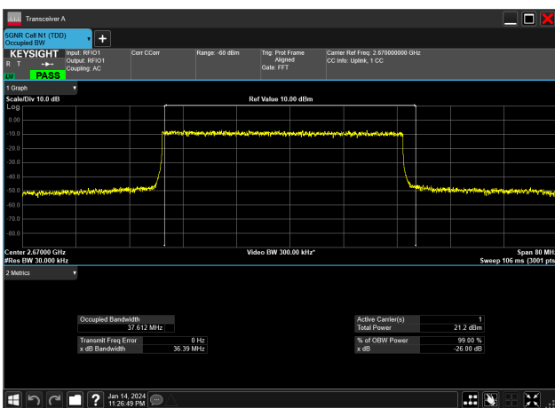
40MHz_30kHz_2670MHz_DFT-s-OFDM 16 QAM_RB100@0&37.612 MHz
