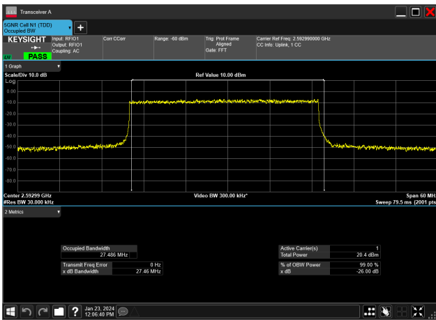
30MHz_30kHz_2592.99MHz_DFT-s-OFDM 64 QAM_RB75@0&27.486 MHz
