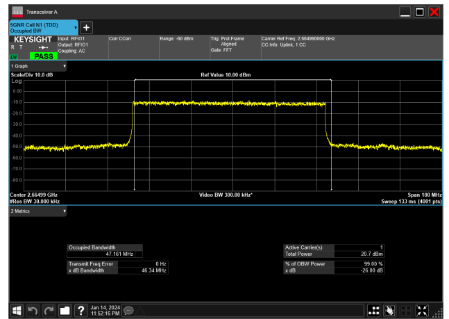
50MHz_30kHz_2664.99MHz_DFT-s-OFDM 64 QAM_RB128@0&47.161 MHz
