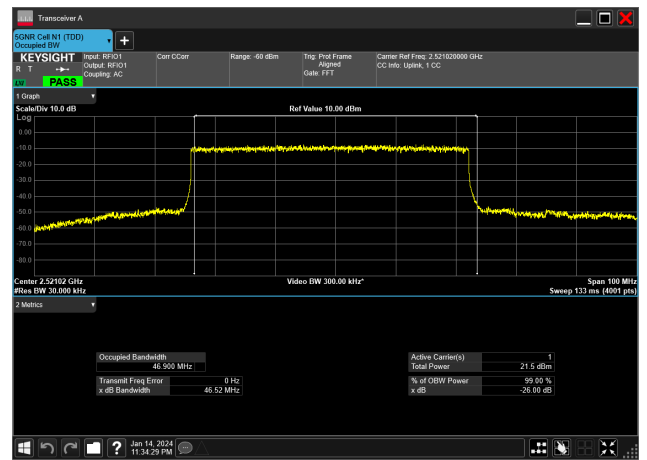
50MHz_30kHz_2521.02MHz_DFT-s-OFDM QPSK_RB128@0&46.900 MHz
