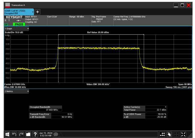
40MHz_30kHz_2670MHz_DFT-s-OFDM PI/2 BPSK_RB100@0&37.660 MHz
