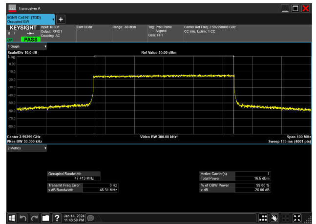
50MHz_30kHz_2592.99MHz_CP-OFDM 256 QAM_RB133@0&47.413 MHz
