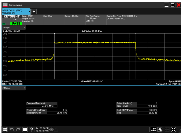
30MHz_30kHz_2592.99MHz_CP-OFDM 16 QAM_RB78@0&27.845 MHz
