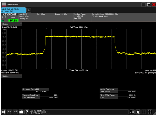
50MHz_30kHz_2664.99MHz_DFT-s-OFDM PI/2 BPSK_RB128@0&47.124 MHz
