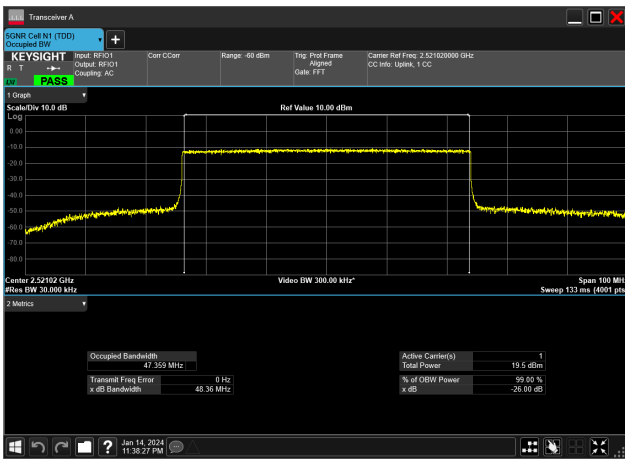
50MHz_30kHz_2521.02MHz_CP-OFDM QPSK_RB133@0&47.359 MHz
