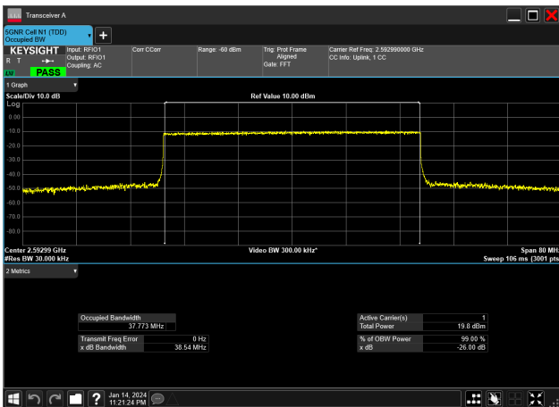
40MHz_30kHz_2592.99MHz_CP-OFDM QPSK_RB106@0&amp;37.773 MHz
