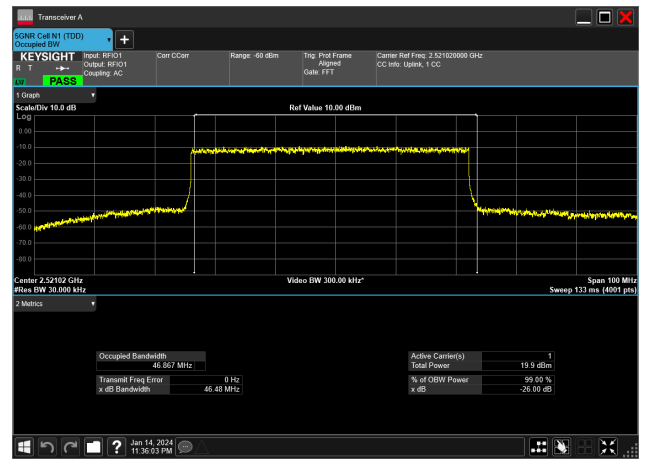
50MHz_30kHz_2521.02MHz_DFT-s-OFDM 64 QAM_RB128@0&46.867 MHz
