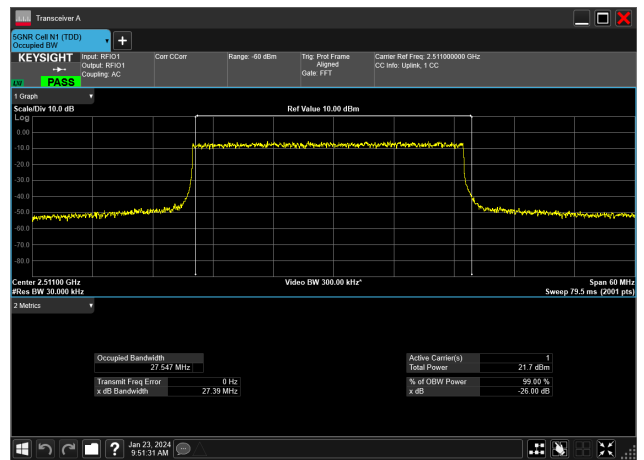
30MHz_30kHz_2511MHz_DFT-s-OFDM QPSK_RB75@0&27.547 MHz
