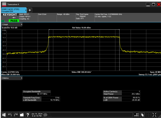
20MHz_30kHz_2679.99MHz_CP-OFDM 16 QAM_RB51@0&18.177 MHz
