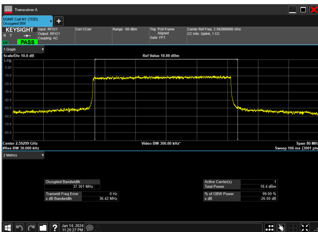
40MHz_30kHz_2592.99MHz_DFT-s-OFDM 256 QAM_RB100@0&amp;37.301 MHz
