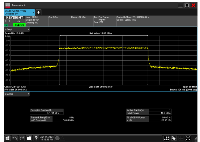
40MHz_30kHz_2516.01MHz_CP-OFDM 256 QAM_RB106@0&37.781 MHz
