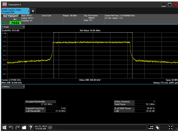
30MHz_30kHz_2511MHz_DFT-s-OFDM 256 QAM_RB75@0&27.553 MHz
