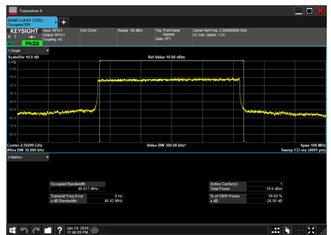
50MHz_30kHz_2592.99MHz_DFT-s-OFDM 256 QAM_RB128@0&46.817 MHz
