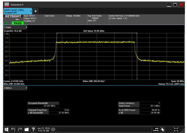
30MHz_30kHz_2511MHz_DFT-s-OFDM 64 QAM_RB75@0&27.541 MHz
