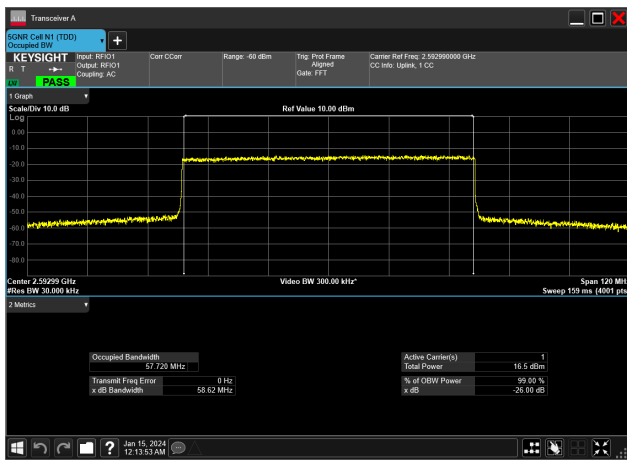
60MHz_30kHz_2592.99MHz_CP-OFDM 256 QAM_RB162@0&57.720 MHz
