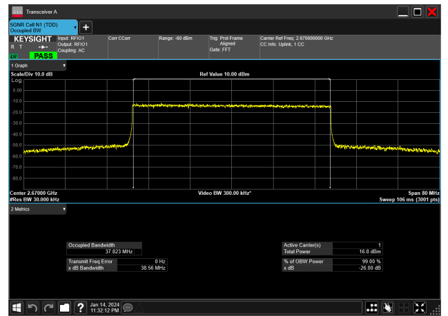
40MHz_30kHz_2670MHz_CP-OFDM 256 QAM_RB106@0&37.823 MHz
