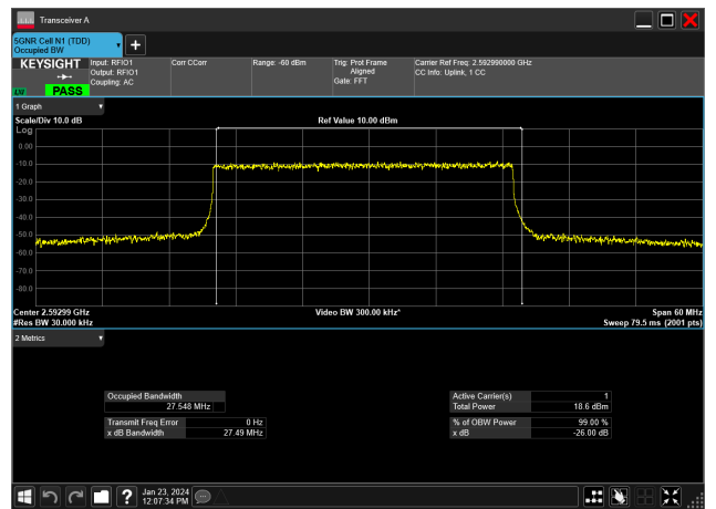
30MHz_30kHz_2592.99MHz_DFT-s-OFDM 256 QAM_RB75@0&27.548 MHz
