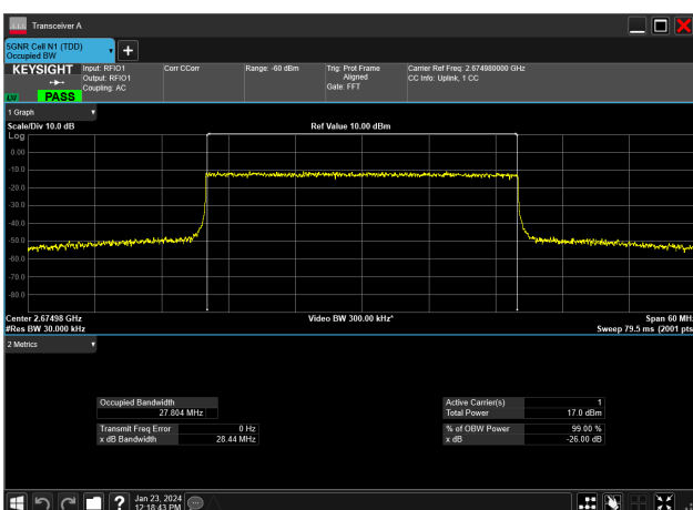
30MHz_30kHz_2674.98MHz_CP-OFDM 256 QAM_RB78@0&27.804 MHz
