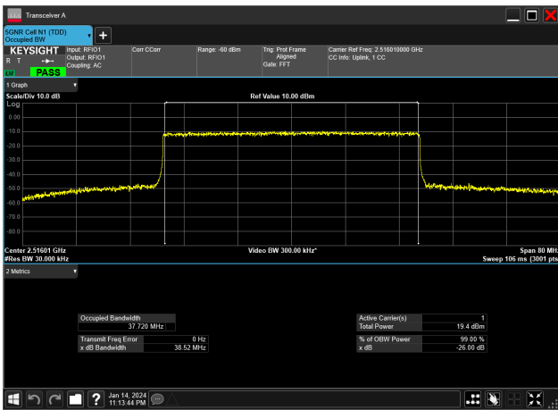
40MHz_30kHz_2516.01MHz_CP-OFDM 16 QAM_RB106@0&37.720 MHz
