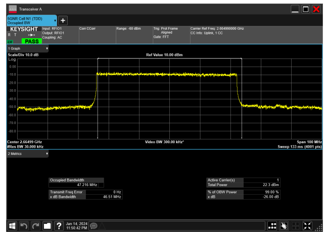
50MHz_30kHz_2664.99MHz_DFT-s-OFDM QPSK_RB128@0&47.216 MHz
