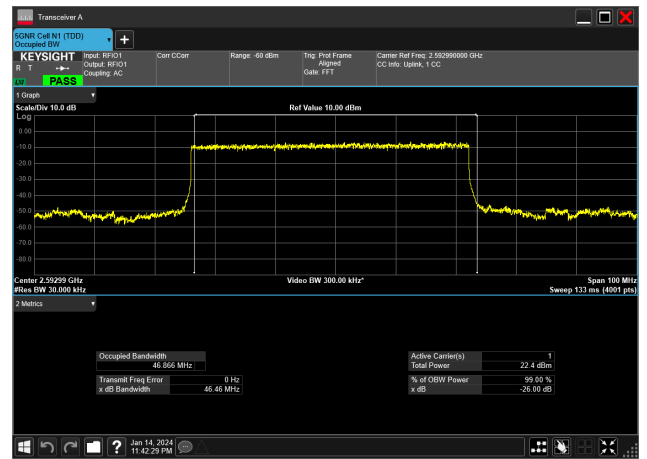
50MHz_30kHz_2592.99MHz_DFT-s-OFDM 1/2 BPSK_RB128@0&46.866 MHz
