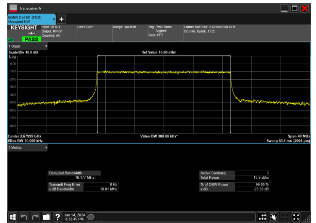
20MHz_30kHz_2679.99MHz_CP-OFDM 256 QAM_RB51@0&18.177 MHz
