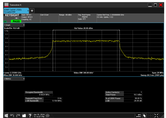
10MHz_30kHz_2355MHz_DFT-s-OFDM 256 QAM_RB24@0&8.602 MHz
