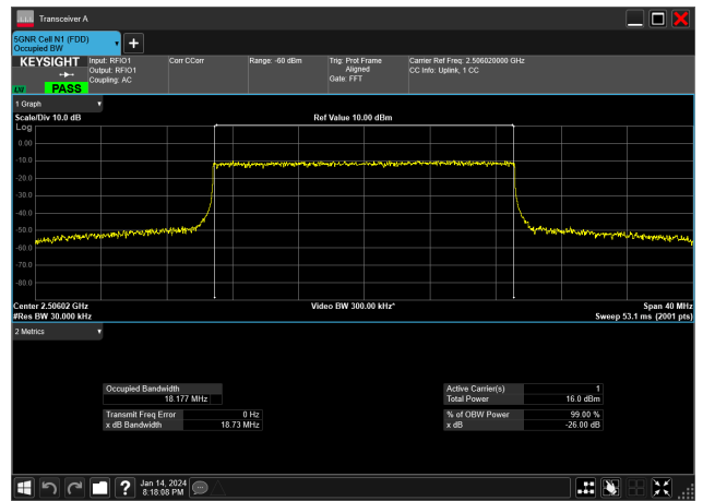
20MHz_30kHz_2506.02MHz_CP-OFDM 256 QAM_RB51@0&18.177 MHz
