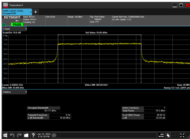
20MHz_30kHz_2506.02MHz_CP-OFDM 16 QAM_RB51@0&18.171 MHz
