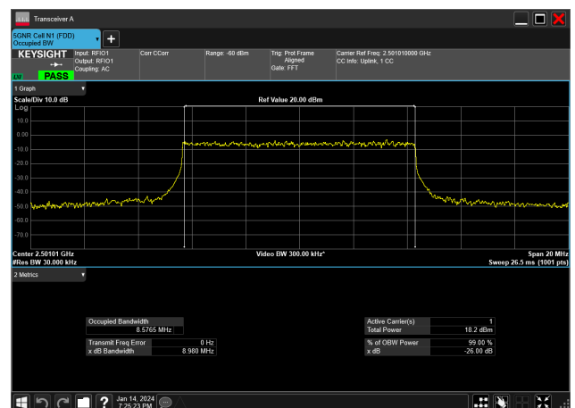
10MHz_30kHz_2501.01MHz_DFT-s-OFDM 256 QAM_RB24@0&amp;8.577 MHz
