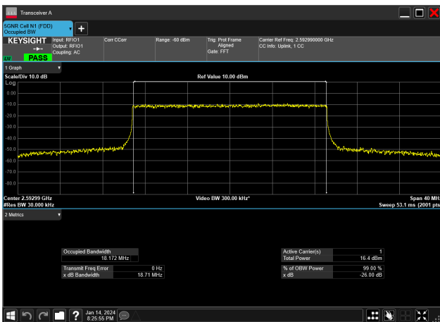
20MHz_30kHz_2592.99MHz_CP-OFDM 256 QAM_RB51@0&18.172 MHz
