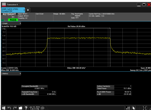
10MHz_30kHz_2501.01MHz_CP-OFDM 64 QAM_RB24@0&amp;8.566 MHz
