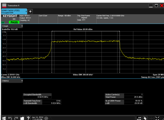
10MHz_30kHz_2501.01MHz_DFT-s-OFDM 16 QAM_RB24@0&amp;8.568 MHz
