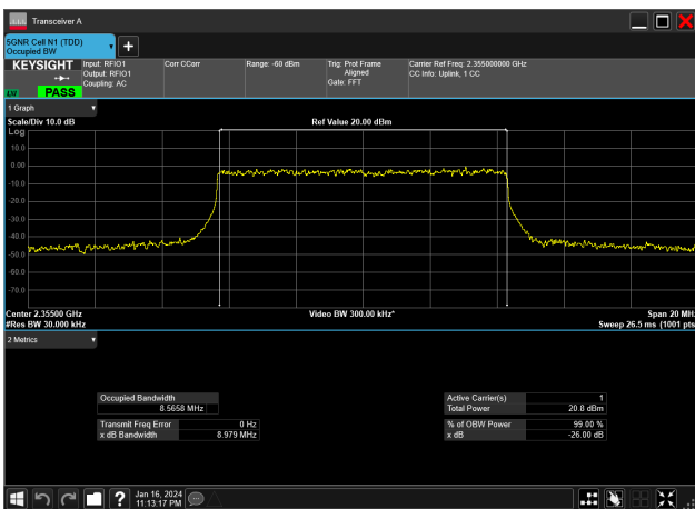
10MHz_30kHz_2355MHz_DFT-s-OFDM 16 QAM_RB24@0&8.566 MHz
