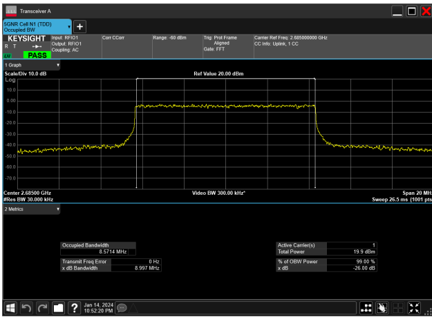
10MHz_30kHz_2685MHz_CP-OFDM 64 QAM_RB24@0&8.571 MHz
