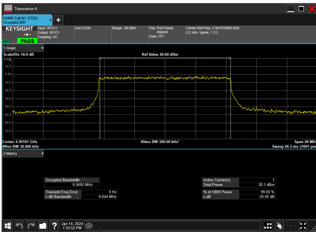
10MHz_30kHz_2501.01MHz_DFT-s-OFDM 64 QAM_RB24@0&8.569 MHz
