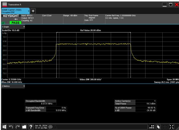
10MHz_30kHz_2355MHz_CP-OFDM 64 QAM_RB24@0&8.573 MHz
