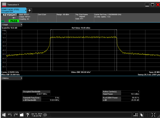
10MHz_30kHz_2592.99MHz_CP-OFDM 256 QAM_RB24@0&8.568 MHz
