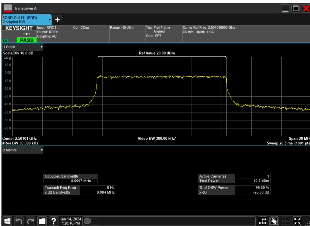
10MHz_30kHz_2501.01MHz_CP-OFDM 16 QAM_RB24@0&amp;8.567 MHz
