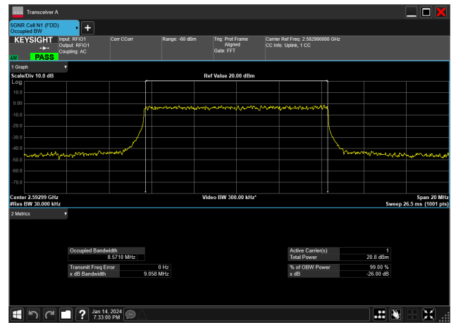
10MHz_30kHz_2592.99MHz_DFT-s-OFDM 16 QAM_RB24@0&8.571 MHz
