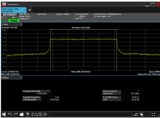
10MHz_30kHz_2685MHz_CP-OFDM 16 QAM_RB24@0&8.570 MHz
