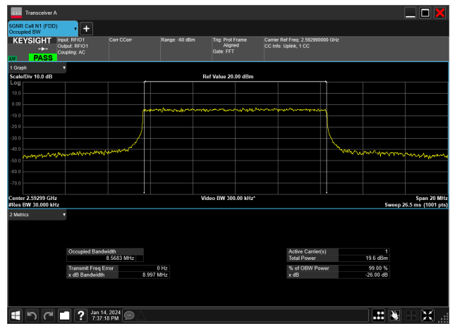
10MHz_30kHz_2592.99MHz_CP-OFDM 64 QAM_RB24@0&8.568 MHz
