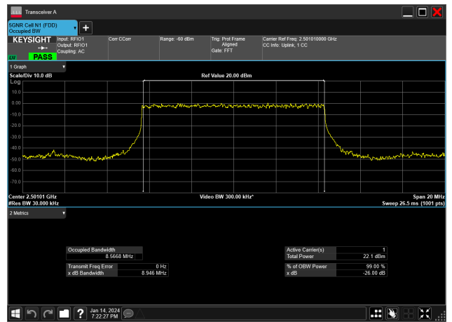
10MHz_30kHz_2501.01MHz_DFT-s-OFDM 1/2 BPSK_RB24@0&8.567 MHz
