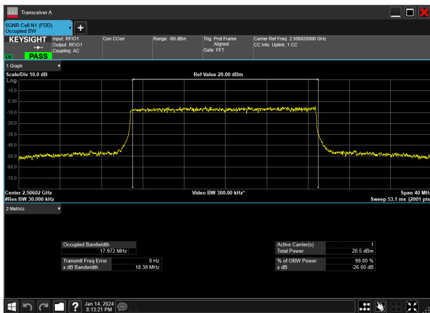
20MHz_30kHz_2506.02MHz_DFT-s-OFDM 16 QAM_RB50@0&17.972 MHz
