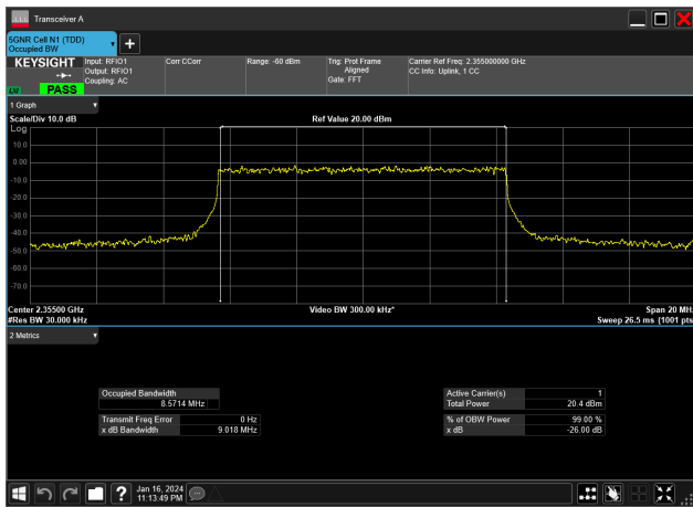
10MHz_30kHz_2355MHz_DFT-s-OFDM 64 QAM_RB24@0&8.571 MHz
