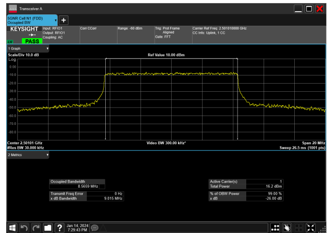
10MHz_30kHz_2501.01MHz_CP-OFDM 256 QAM_RB24@0&amp;8.566 MHz
