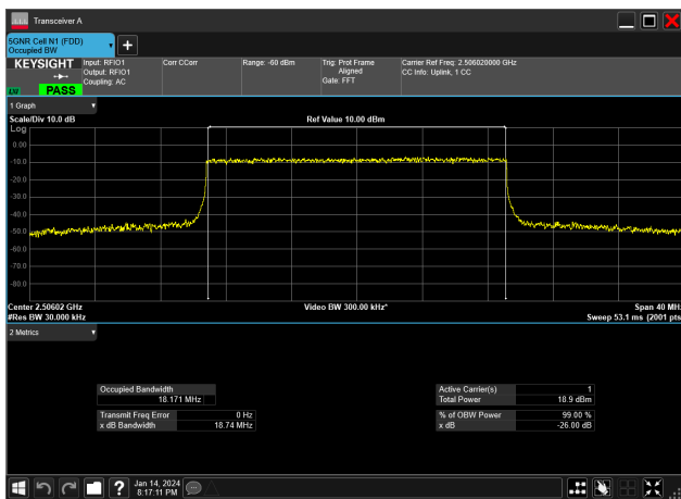
20MHz_30kHz_2506.02MHz_CP-OFDM 64 QAM_RB51@0&18.171 MHz
