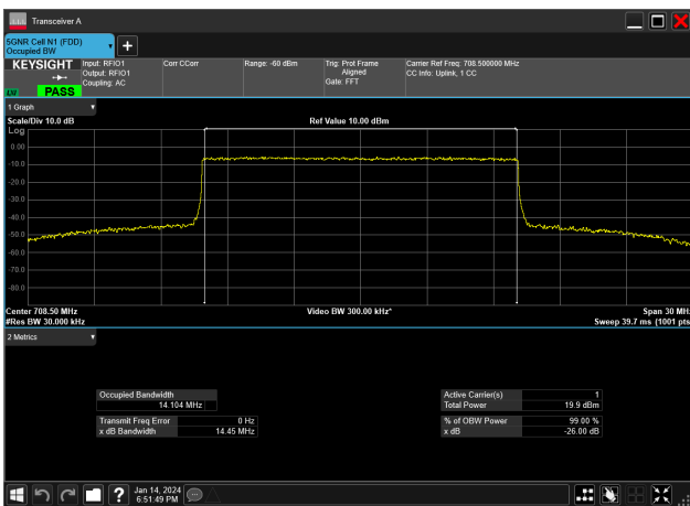
15MHz_15kHz_708.5MHz_CP-OFDM 64 QAM_RB79@0&14.104 MHz
