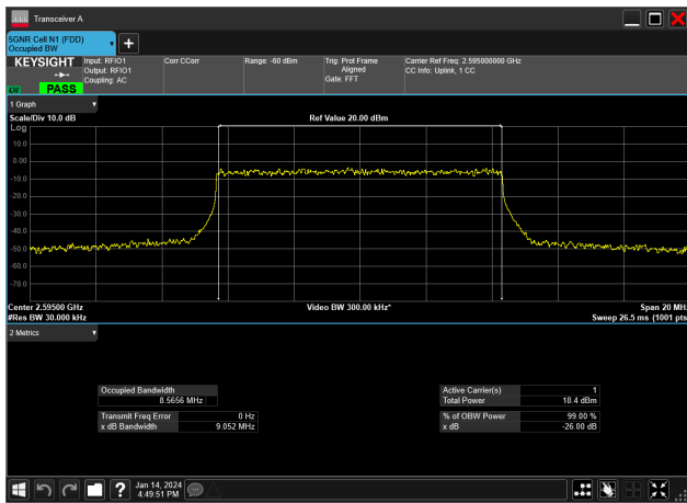
10MHz_30kHz_2595MHz_DFT-s-OFDM 256 QAM_RB24@0&8.566 MHz
