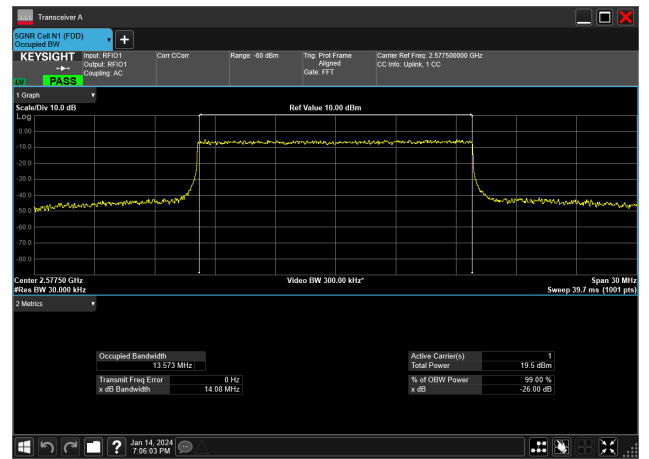
15MHz_30kHz_2577.5MHz_CP-OFDM 16 QAM_RB38@0&13.573 MHz
