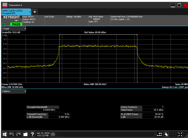
10MHz_30kHz_2615MHz_DFT-s-OFDM 64 QAM_RB24@0&8.567 MHz
