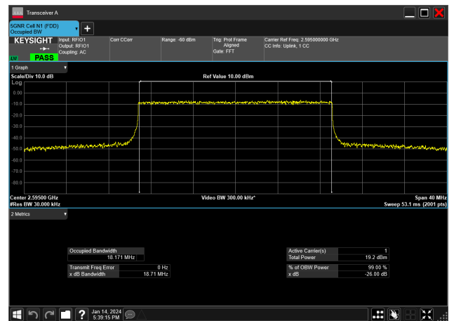
20MHz_30kHz_2595MHz_CP-OFDM 64 QAM_RB51@0&18.171 MHz
