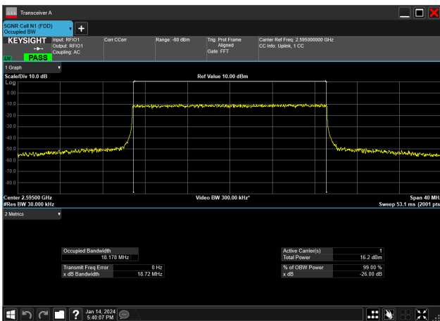
20MHz_30kHz_2595MHz_CP-OFDM 256 QAM_RB51@0&18.178 MHz
