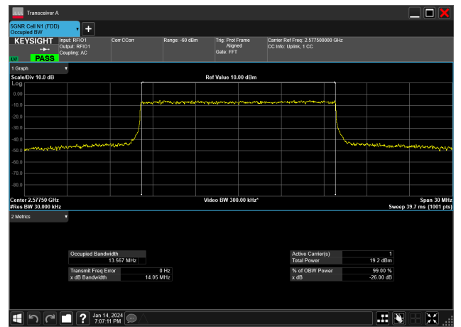
15MHz_30kHz_2577.5MHz_CP-OFDM 64 QAM_RB38@0&13.567 MHz
