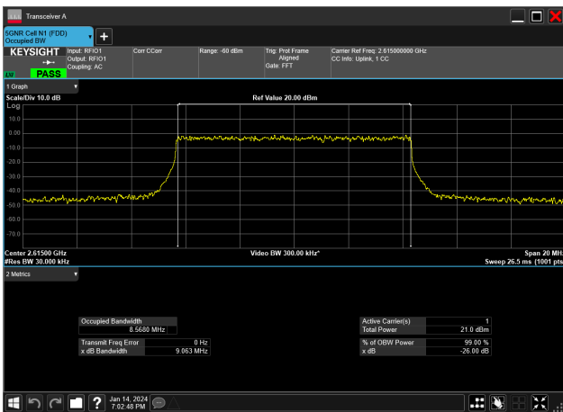
10MHz_30kHz_2615MHz_DFT-s-OFDM 16 QAM_RB24@0&8.568 MHz
