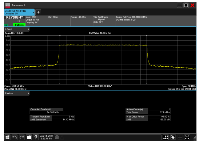
15MHz_15kHz_708.5MHz_CP-OFDM 256 QAM_RB79@0&14.100 MHz
