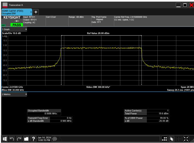
10MHz_30kHz_2615MHz_CP-OFDM 64 QAM_RB24@0&8.569 MHz
