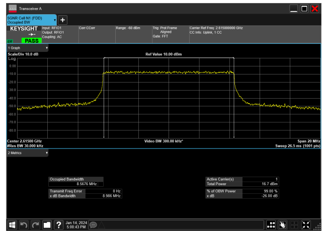
10MHz_30kHz_2615MHz_CP-OFDM 256 QAM_RB24@0&8.568 MHz
