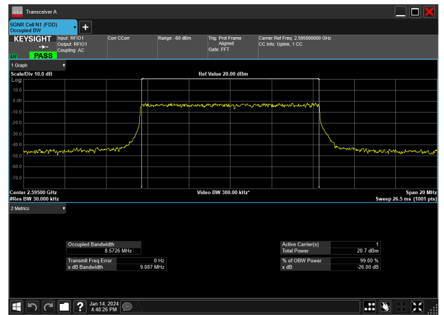
10MHz_30kHz_2595MHz_DFT-s-OFDM 16 QAM_RB24@0&8.573 MHz
