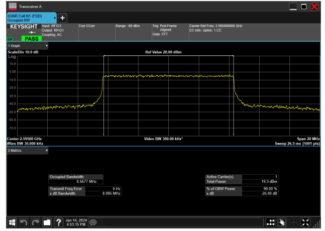
10MHz_30kHz_2595MHz_CP-OFDM 64 QAM_RB24@0&8.568 MHz
