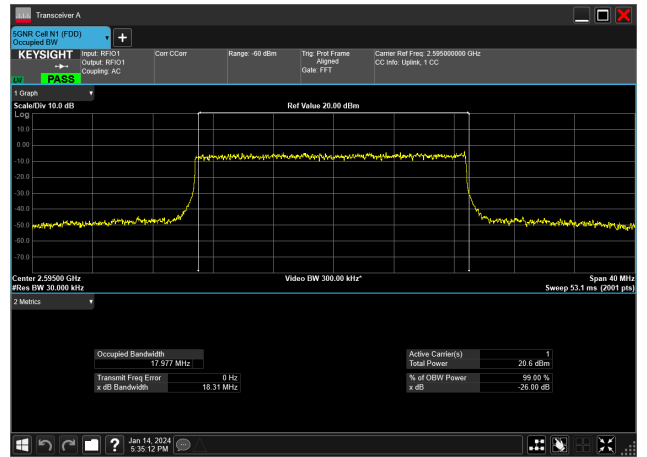
20MHz_30kHz_2595MHz_DFT-s-OFDM 16 QAM_RB50@0&17.977 MHz
