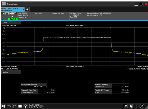
15MHz_15kHz_708.5MHz_CP-OFDM 16 QAM_RB79@0&14.104 MHz
