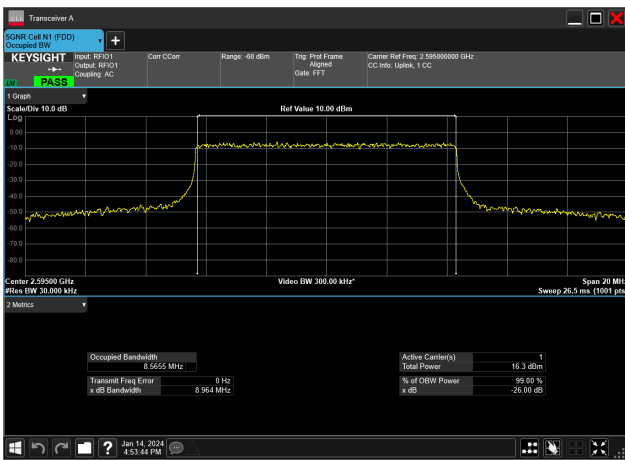
10MHz_30kHz_2595MHz_CP-OFDM 256 QAM_RB24@0&8.565 MHz
