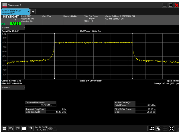
15MHz_30kHz_2577.5MHz_CP-OFDM 256 QAM_RB38@0&13.563 MHz
