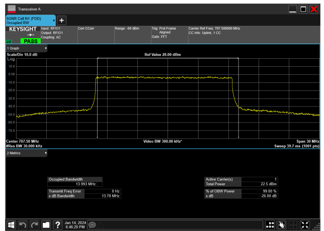
15MHz_15kHz_707.5MHz_DFT-s-OFDM QPSK_RB75@0&13.993 MHz
