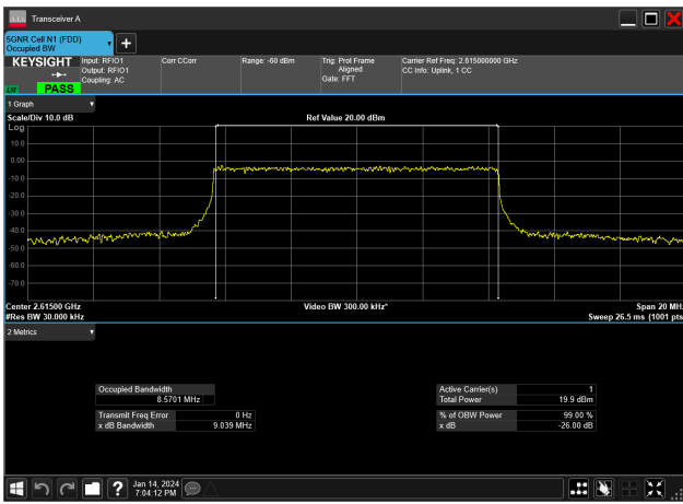
10MHz_30kHz_2615MHz_CP-OFDM 16 QAM_RB24@0&8.570 MHz
