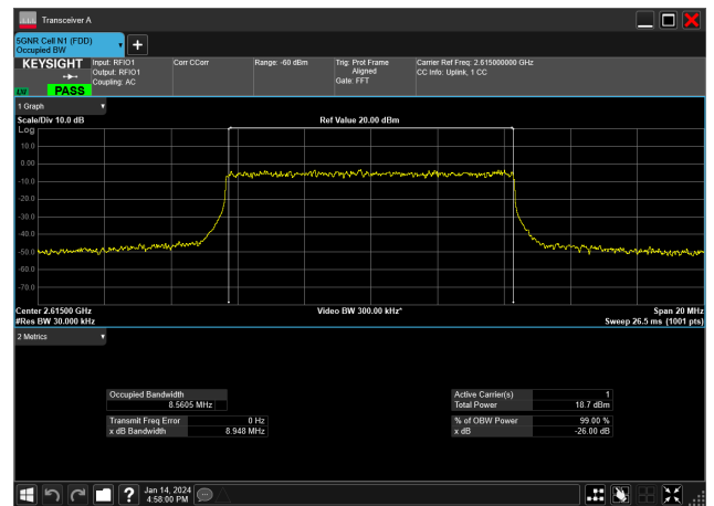
10MHz_30kHz_2615MHz_DFT-s-OFDM 256 QAM_RB24@0&8.560 MHz
