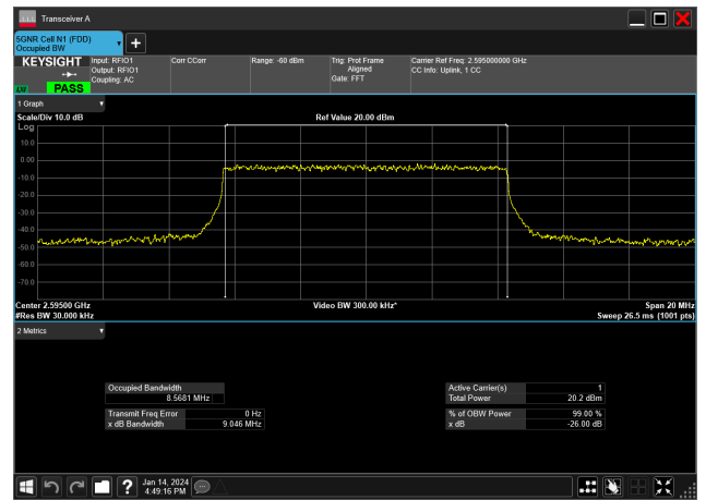
10MHz_30kHz_2595MHz_DFT-s-OFDM 64 QAM_RB24@0&8.568 MHz
