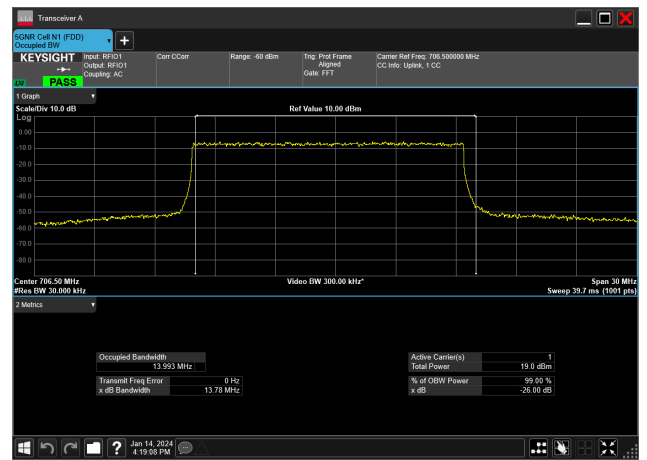
15MHz_15kHz_706.5MHz_DFT-s-OFDM 256 QAM_RB75@0&13.993 MHz
