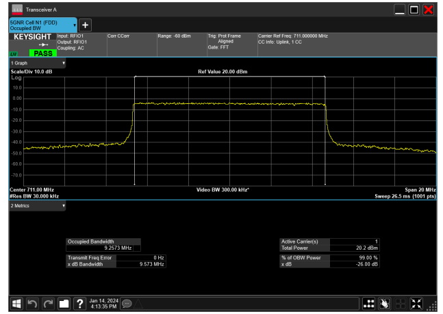
10MHz_15kHz_711MHz_CP-OFDM 16 QAM_RB52@0&9.257 MHz
