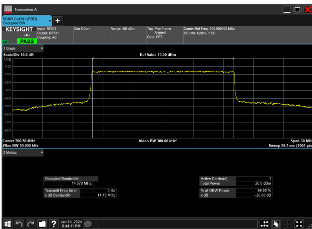
15MHz_15kHz_706.5MHz_CP-OFDM 64 QAM_RB79@0&14.070 MHz
