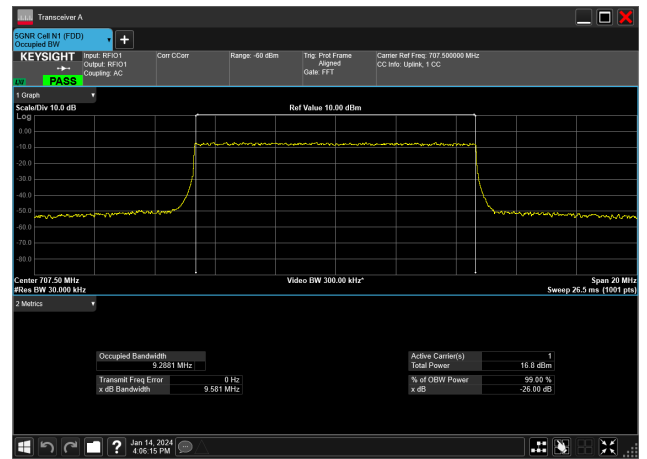
10MHz_15kHz_707.5MHz_CP-OFDM 256 QAM_RB52@0&9.288 MHz
