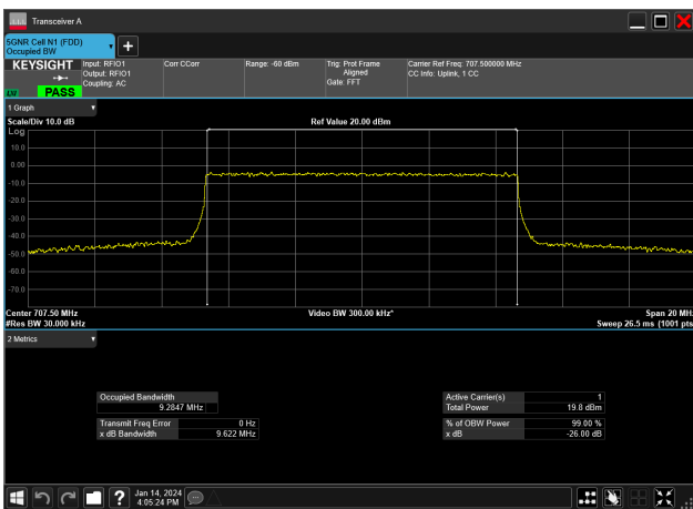
10MHz_15kHz_707.5MHz_CP-OFDM 64 QAM_RB52@0&9.285 MHz
