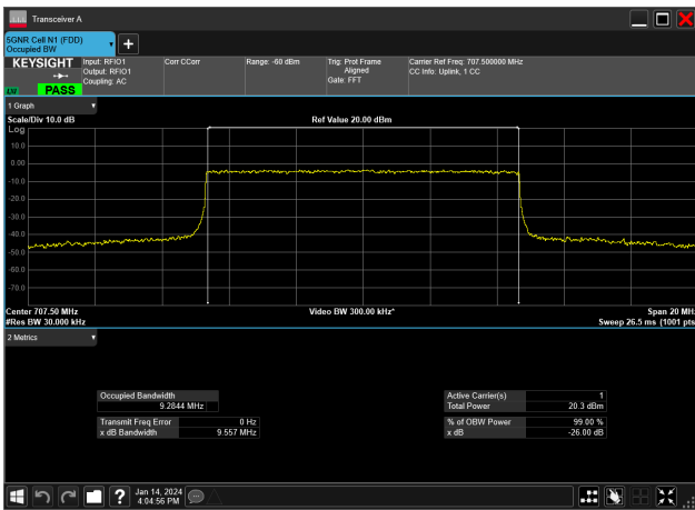
10MHz_15kHz_707.5MHz_CP-OFDM 16 QAM_RB52@0&9.284 MHz
