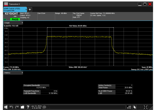
10MHz_15kHz_711MHz_DFT-s-OFDM 64 QAM_RB50@0&9.213 MHz
