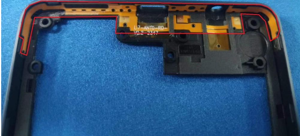
ANT 0 GSM/WCDMA /LTE ANT RX Only
