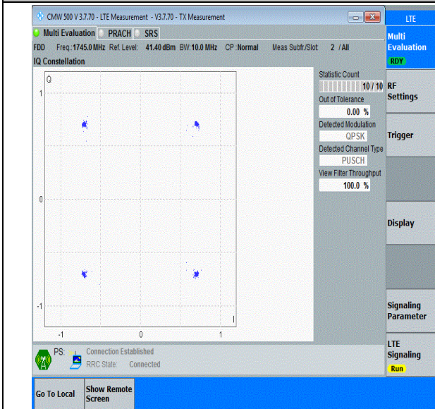
Band66-10MHz-QPSK-132322-50RB#0-PASS
