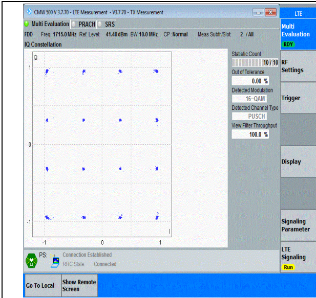
Band66-10MHz-16QAM-132022-50RB#0-PASS
