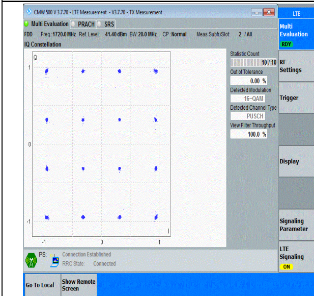
Band66-20MHz-16QAM-132072-100RB#0-PASS
