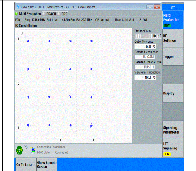
Band66-20MHz-16QAM-132322-100RB#0-PASS
