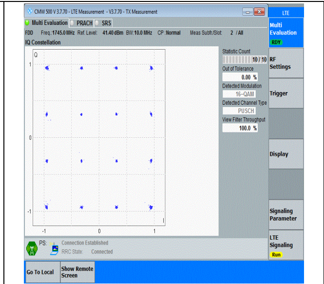
Band66-10MHz-16QAM-132322-50RB#0-PASS
