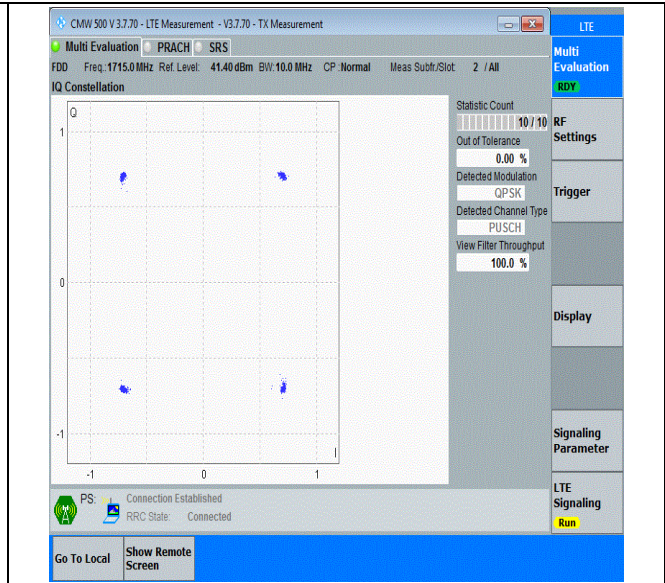
Band66-10MHz-QPSK-132022-50RB#0-PASS
