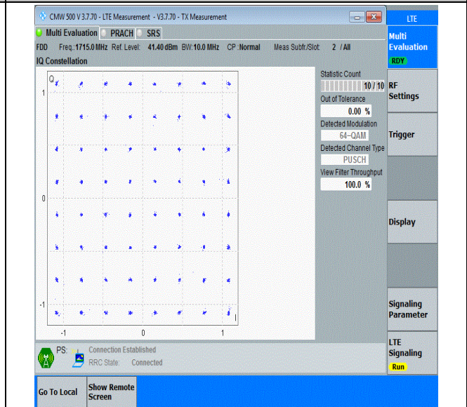
Band66-10MHz-64QAM-132022-50RB#0-PASS
