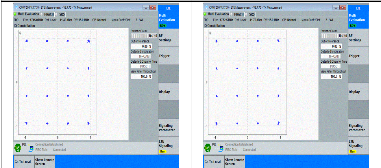
Band66-15MHz-16QAM-132322-75RB#0-PASS
