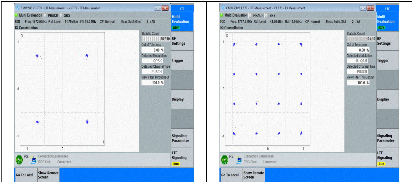
Band66-15MHz-QPSK-132597-75RB#0-PASS
