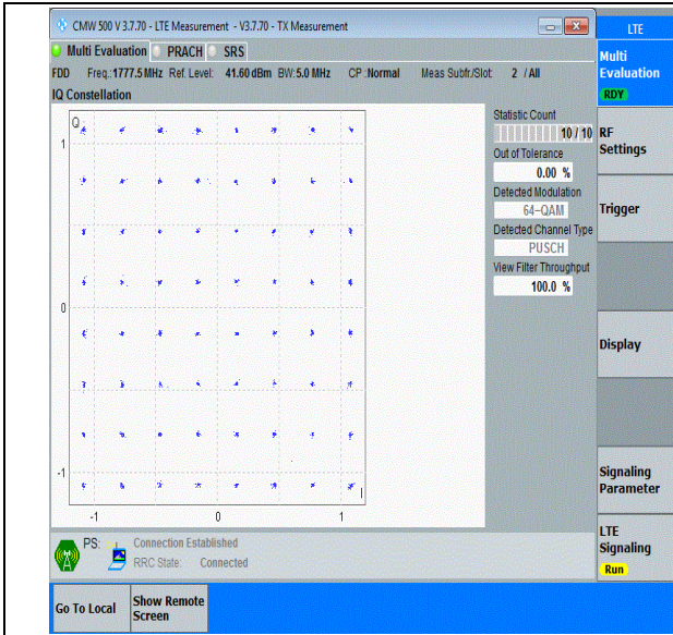
Band66-5MHz-64QAM-132647-25RB#0-PASS
