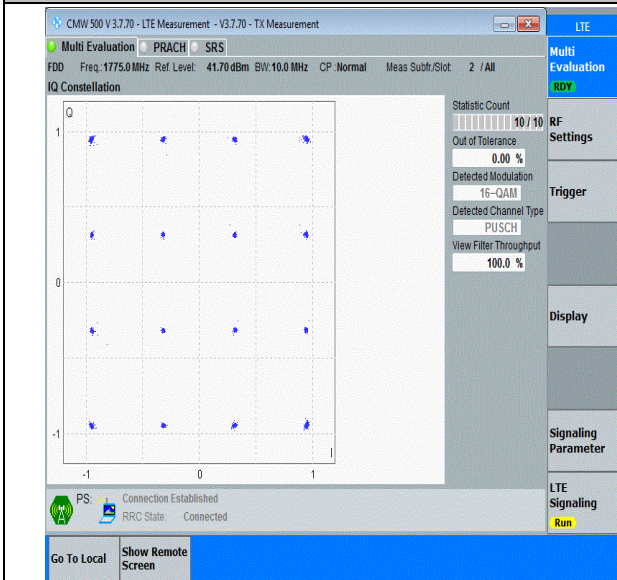
Band66-10MHz-16QAM-132622-50RB#0-PASS
