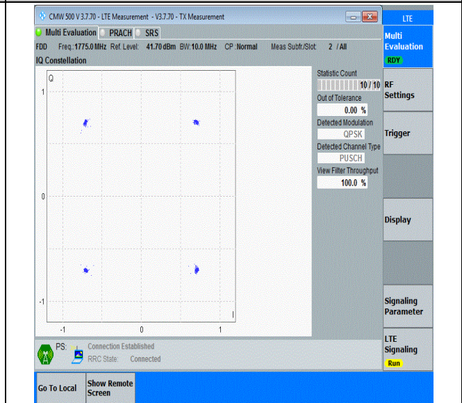
Band66-10MHz-QPSK-132622-50RB#0-PASS
