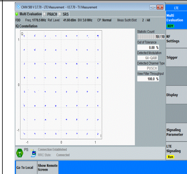
Band66-3MHz-64QAM-132657-15RB#0-PASS
