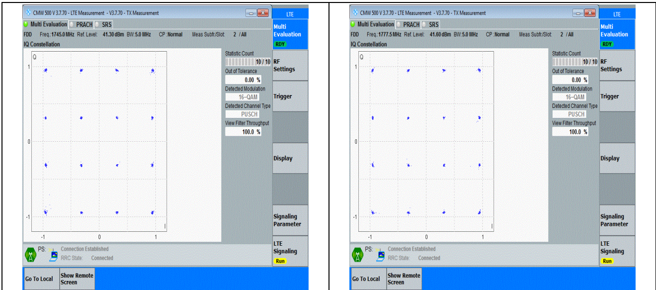
Band66-5MHz-16QAM-132322-25RB#0-PASS
