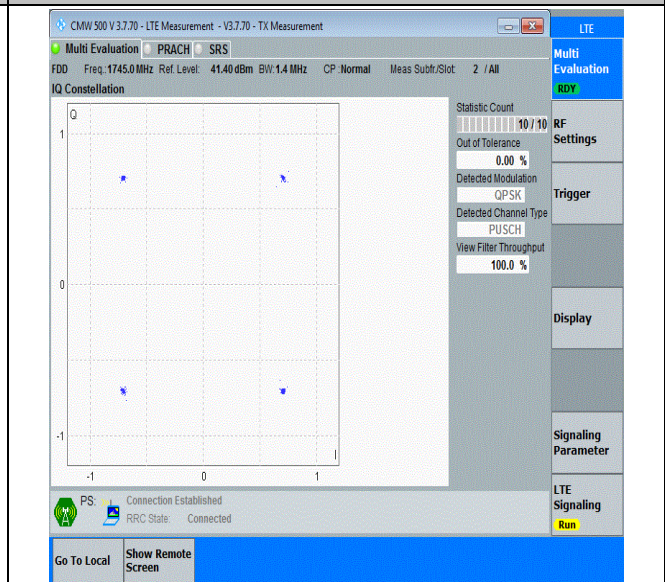
Band66-1.4MHz-QPSK-132322-6RB#0-PASS
