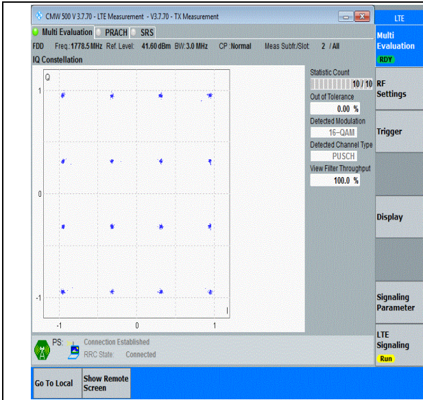
Band66-3MHz-16QAM-132657-15RB#0-PASS
