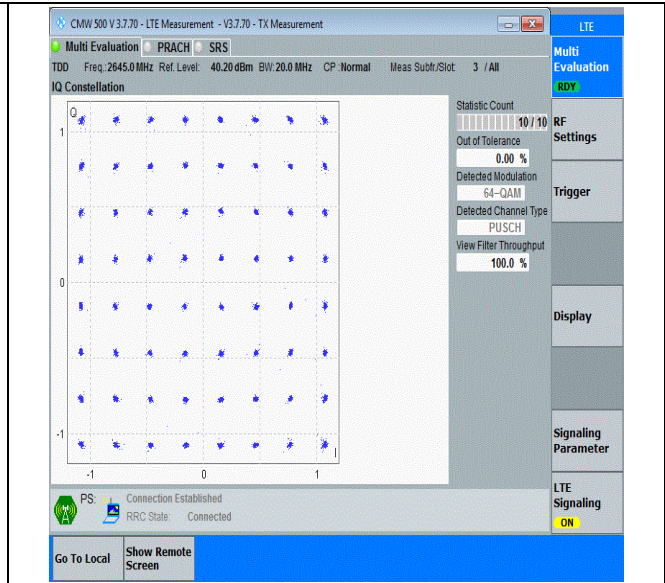
41(2535-2655)-20MHz-64QAM-41140-100RB#0-PASS
