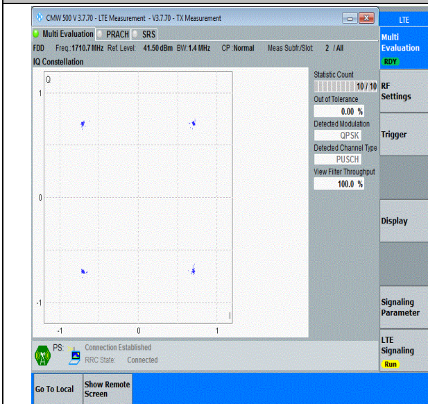
Band66-1.4MHz-QPSK-131979-6RB#0-PASS
