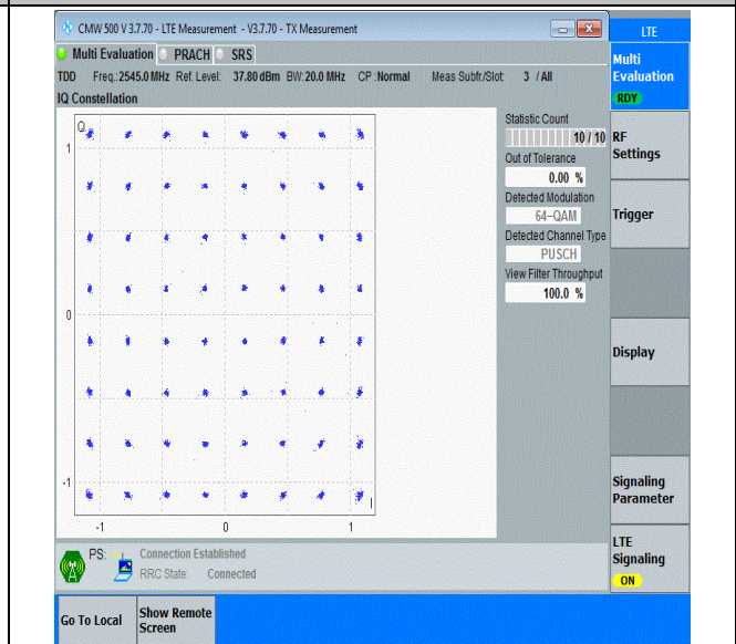
41(2535-2655)-20MHz-64QAM-40140-100RB#0-PASS
