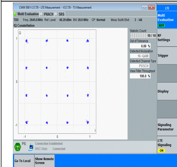
41(2535-2655)-20MHz-16QAM-41140-100RB#0-PASS
