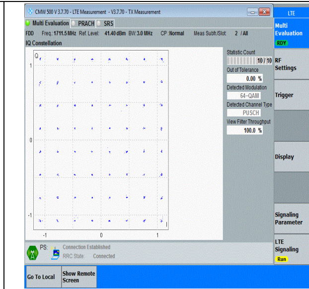
Band66-3MHz-64QAM-131987-15RB#0-PASS
