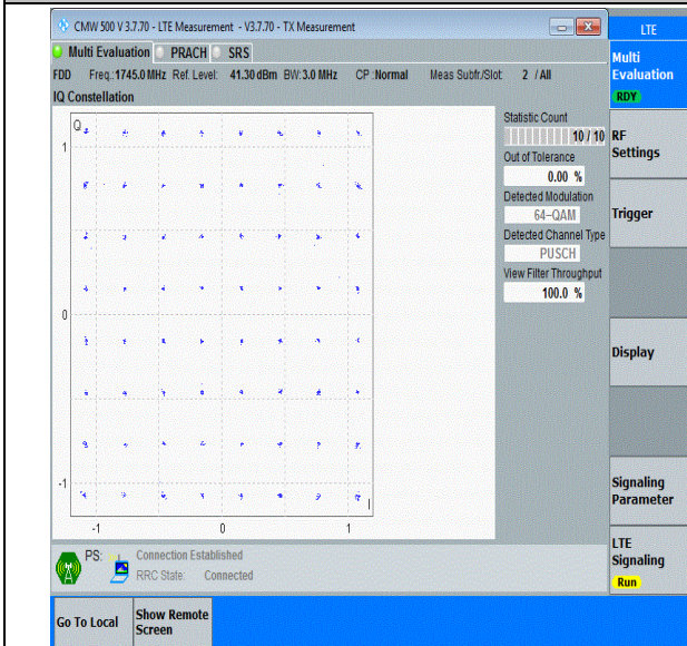
Band66-3MHz-64QAM-132322-15RB#0-PASS
