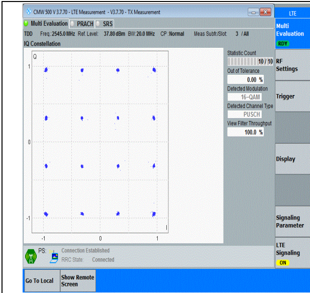
41(2535-2655)-20MHz-16QAM-40140-100RB#0-PASS
