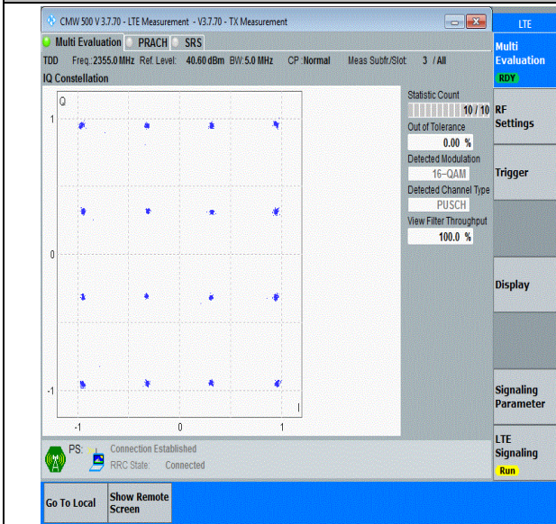
40(2350-2360)-5MHz-16QAM-39200-25RB#0-PASS
