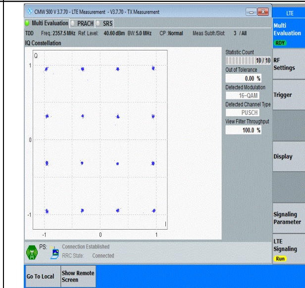
40(2350-2360)-5MHz-16QAM-39225-25RB#0-PASS
