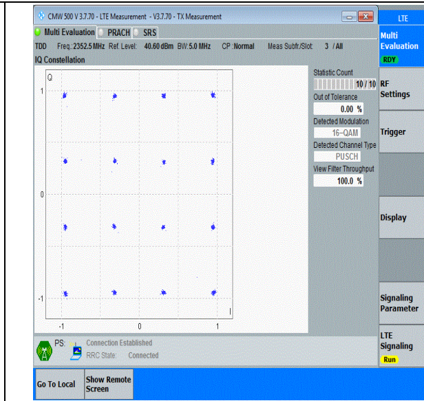
40(2350-2360)-5MHz-16QAM-39175-25RB#0-PASS
