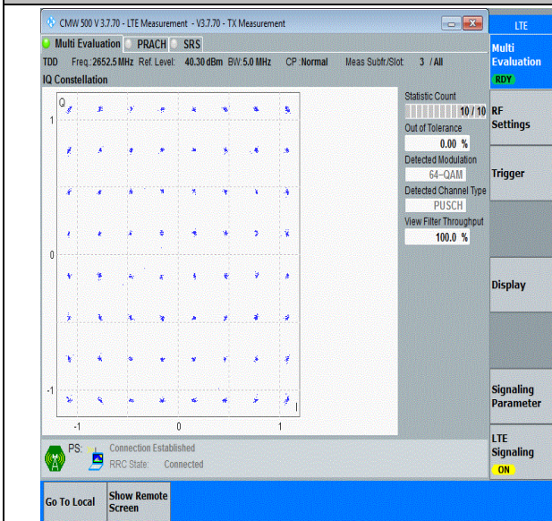
41(2535-2655)-5MHz-64QAM-41215-25RB#0-PASS
