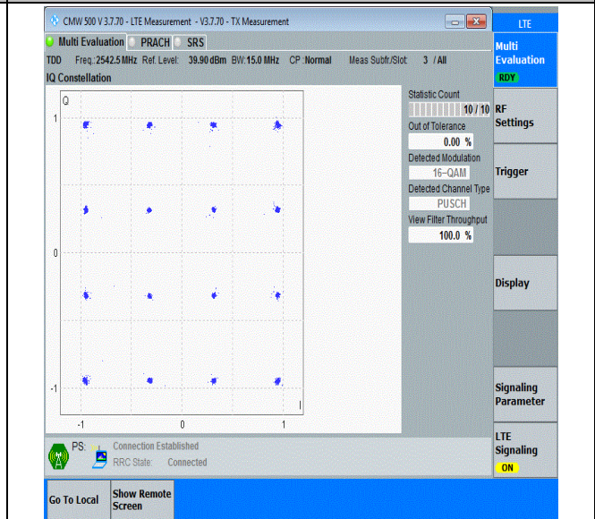
41(2535-2655)-15MHz-16QAM-40115-75RB#0-PASS
