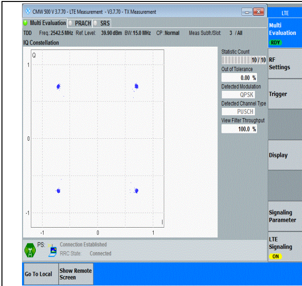
41(2535-2655)-15MHz-QPSK-40115-75RB#0-PASS
