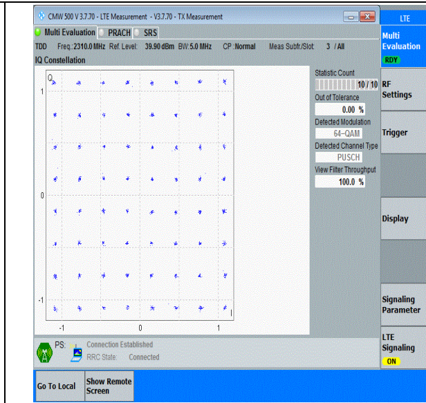
40(2305-2315)-5MHz-64QAM-38750-25RB#0-PASS
