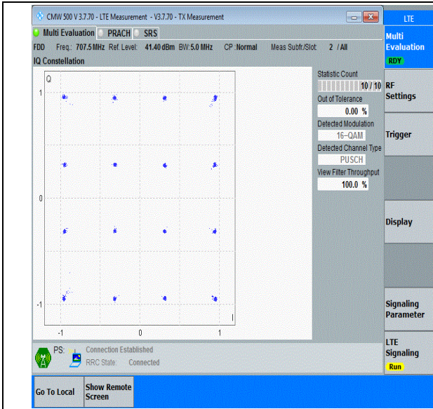
Band12-5MHz-16QAM-23095-25RB#0-PASS
