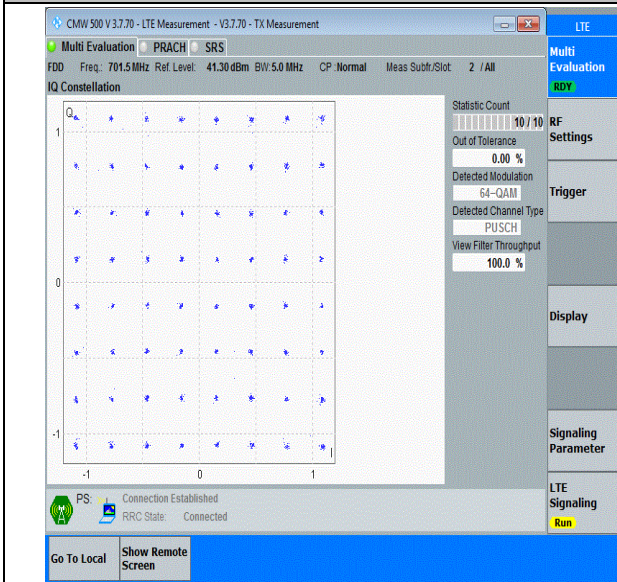
Band12-5MHz-64QAM-23035-25RB#0-PASS
