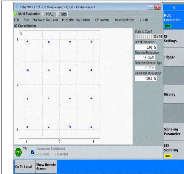
Band12-3MHz-16QAM-23165-15RB#0-PASS
