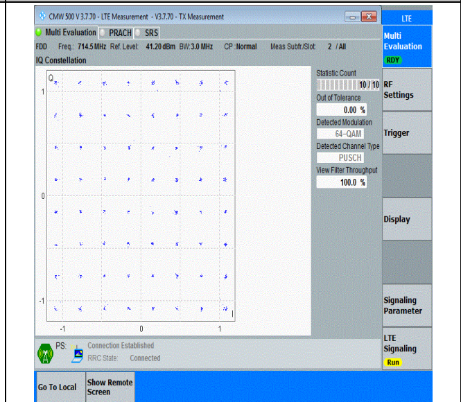
Band12-3MHz-64QAM-23165-15RB#0-PASS
