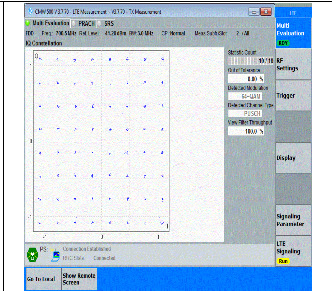
Band12-3MHz-64QAM-23025-15RB#0-PASS
