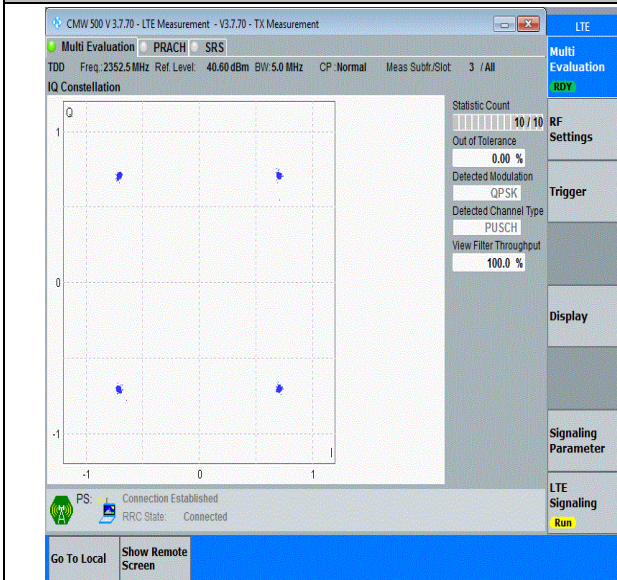
40(2350-2360)-5MHz-QPSK-39175-25RB#0-PASS
