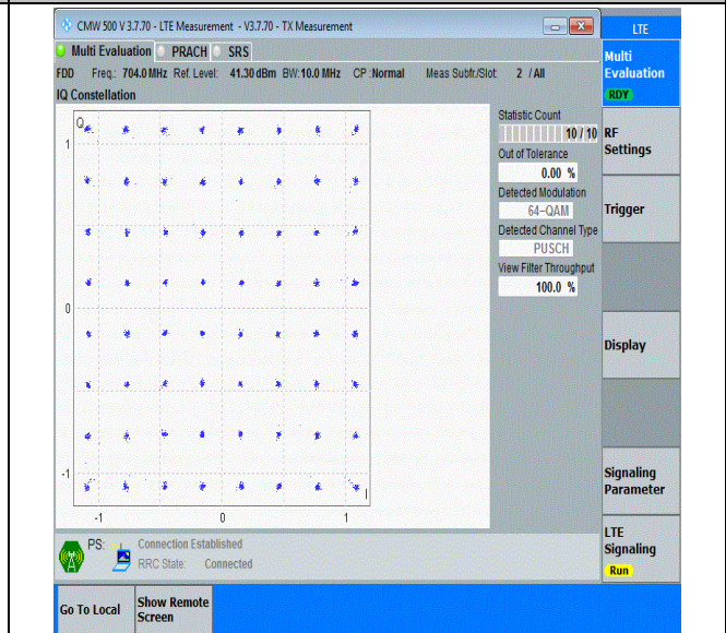
Band12-10MHz-64QAM-23060-50RB#0-PASS
