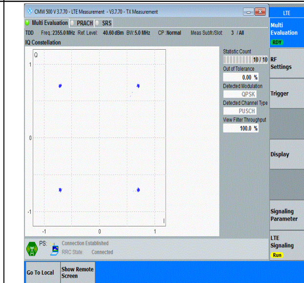
40(2350-2360)-5MHz-QPSK-39200-25RB#0-PASS
