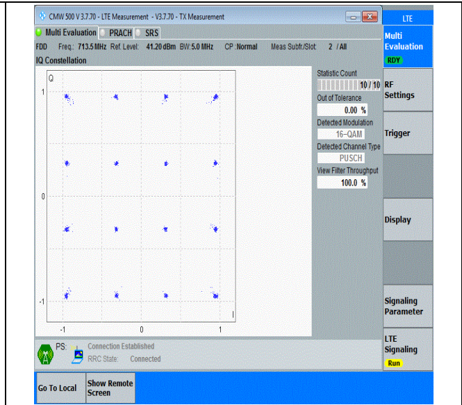
Band12-5MHz-16QAM-23155-25RB#0-PASS
