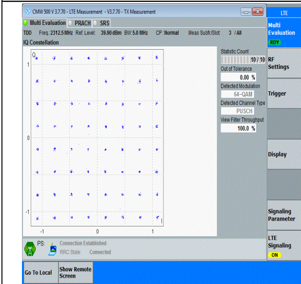
40(2305-2315)-5MHz-64QAM-38775-25RB#0-PASS
