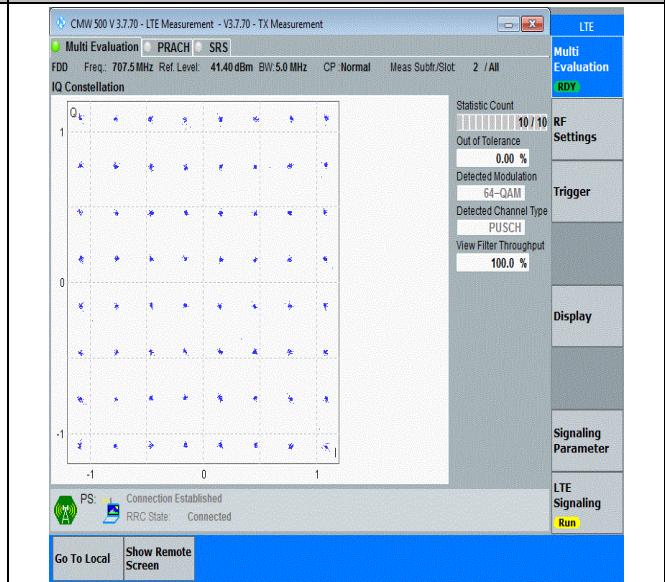
Band12-5MHz-64QAM-23095-25RB#0-PASS
