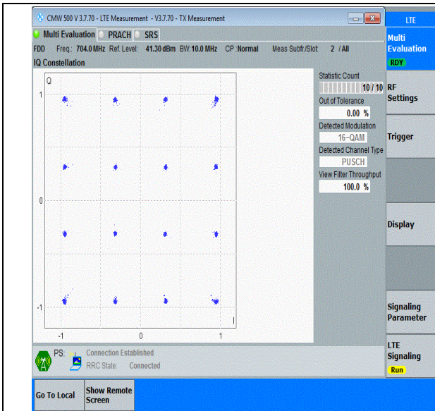
Band12-10MHz-16QAM-23060-50RB#0-PASS
