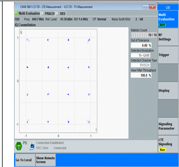
Band12-1.4MHz-16QAM-23017-6RB#0-PASS
