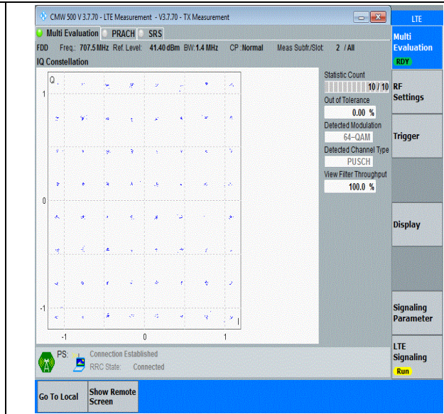
Band12-1.4MHz-64QAM-23095-6RB#0-PASS
