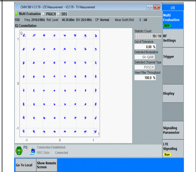
Band7-20MHz-64QAM-20850-100RB#0-PASS
