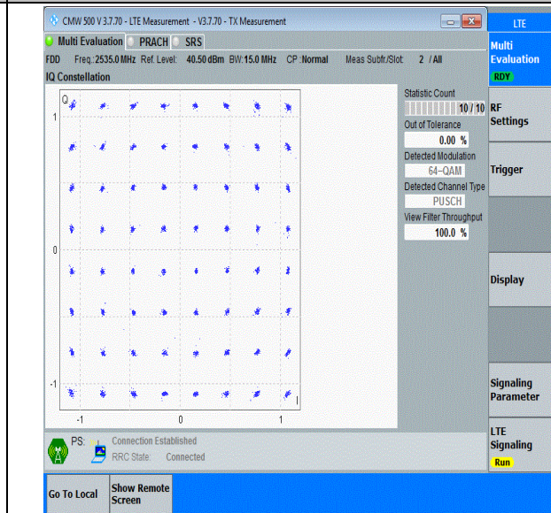
Band7-15MHz-64QAM-21100-75RB#0-PASS
