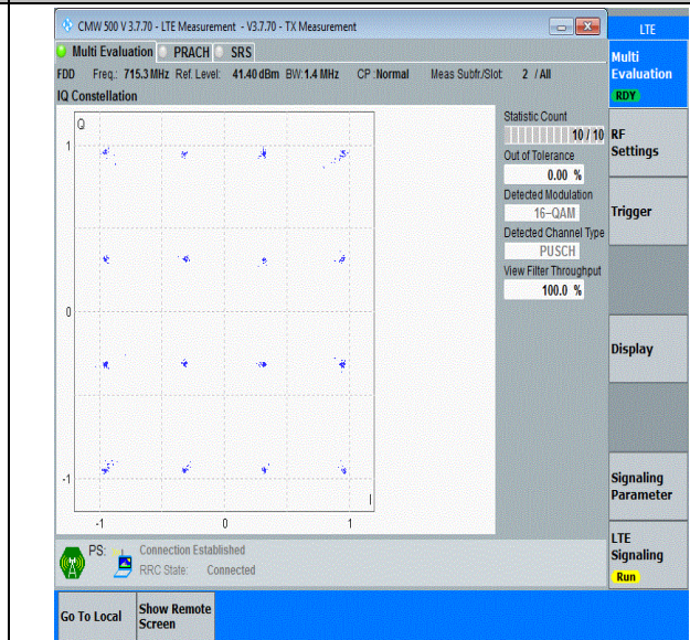
Band12-1.4MHz-16QAM-23173-6RB#0-PASS
