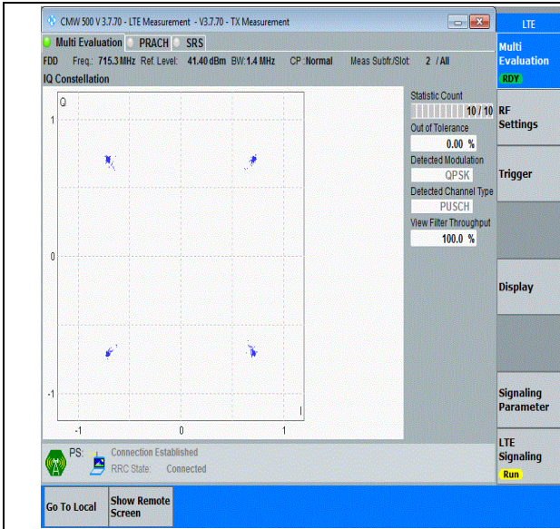
Band12-1.4MHz-QPSK-23173-6RB#0-PASS
