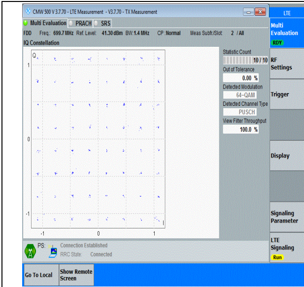
Band12-1.4MHz-64QAM-23017-6RB#0-PASS
