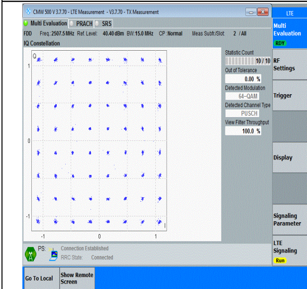
Band7-15MHz-64QAM-20825-75RB#0-PASS
