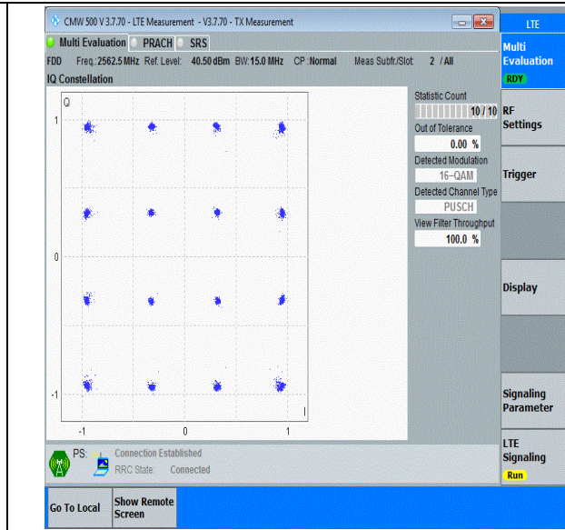
Band7-15MHz-16QAM-21375-75RB#0-PASS
