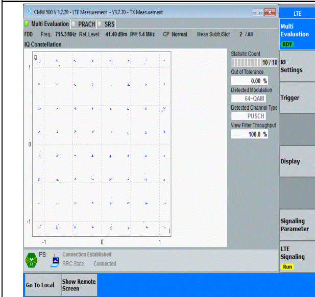
Band12-1.4MHz-64QAM-23173-6RB#0-PASS
