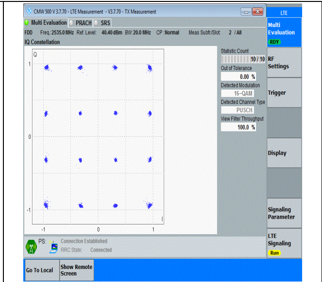
Band7-20MHz-16QAM-21100-100RB#0-PASS
