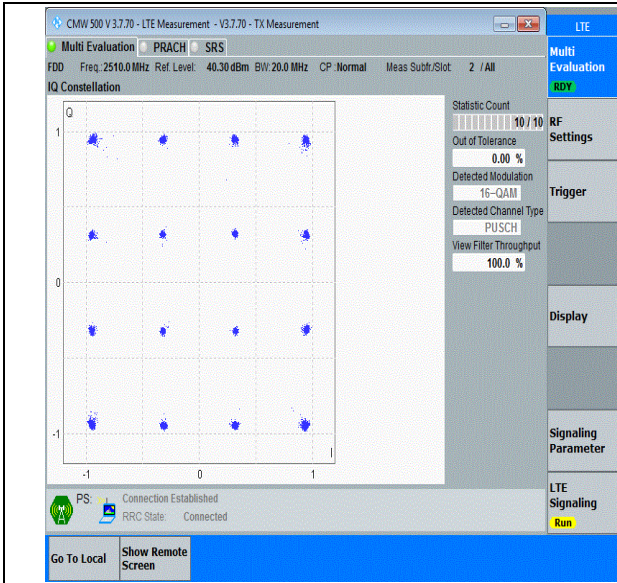
Band7-20MHz-16QAM-20850-100RB#0-PASS
