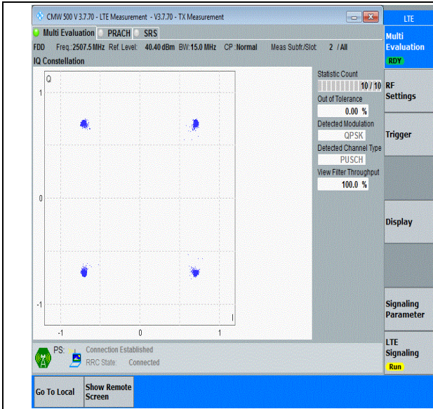
Band7-15MHz-QPSK-20825-75RB#0-PASS
