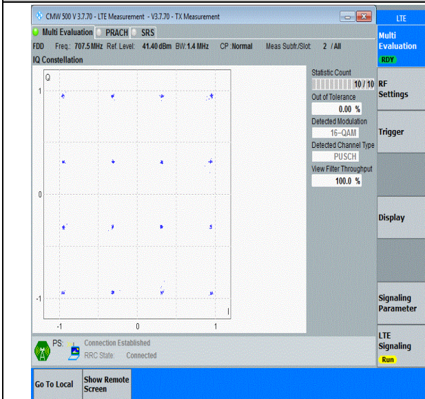
Band12-1.4MHz-16QAM-23095-6RB#0-PASS
