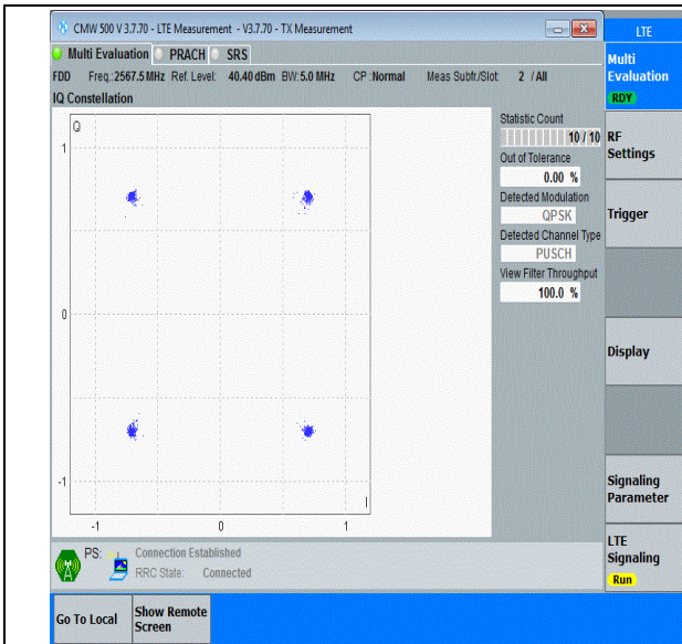
Band7-5MHz-QPSK-21425-25RB#0-PASS
