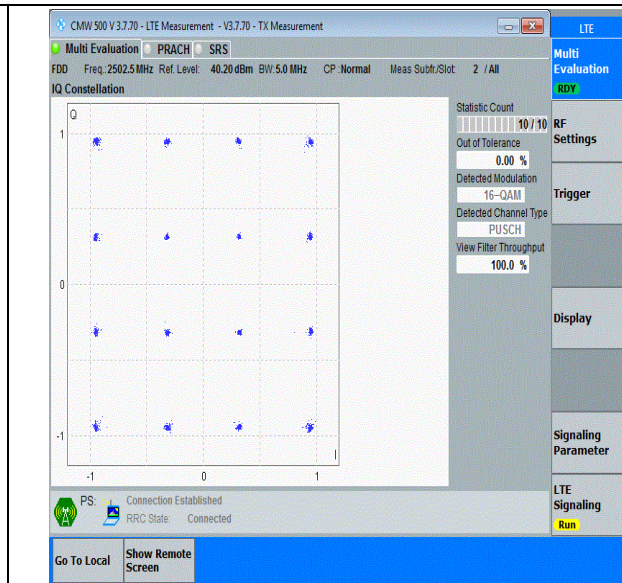
Band7-5MHz-16QAM-20775-25RB#0-PASS
