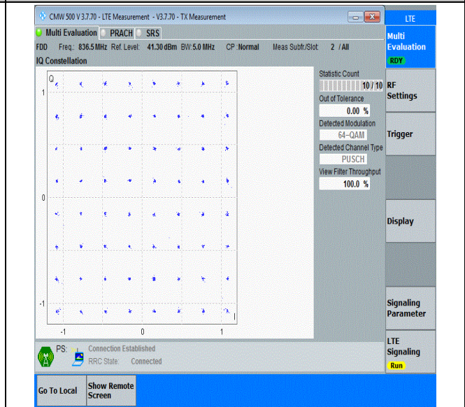
Band5-5MHz-64QAM-20525-25RB#0-PASS
