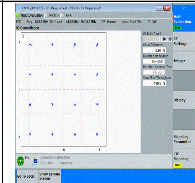
Band5-5MHz-16QAM-20425-25RB#0-PASS
