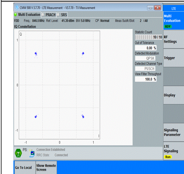
Band5-5MHz-QPSK-20625-25RB#0-PASS
