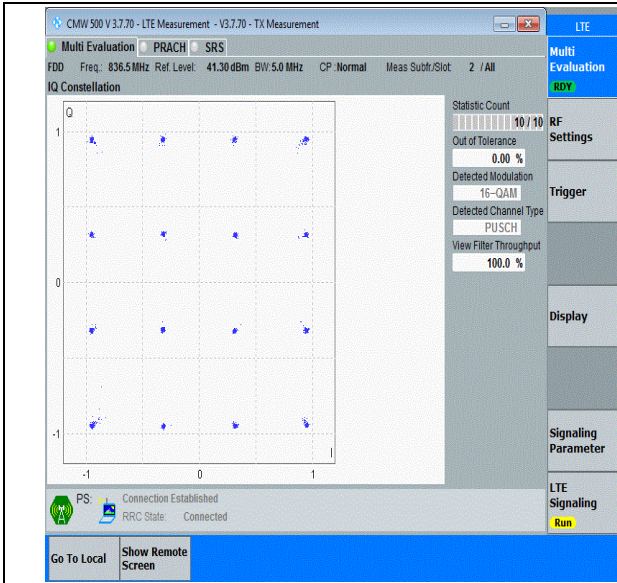
Band5-5MHz-16QAM-20525-25RB#0-PASS
