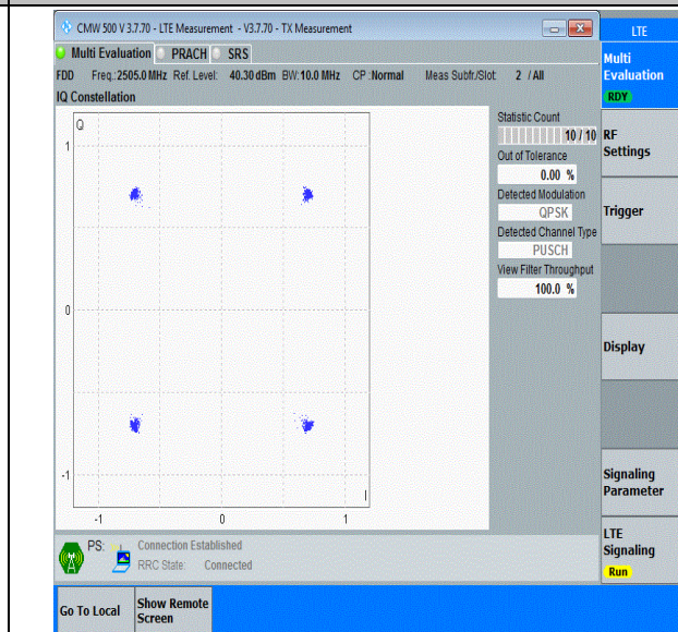
Band7-10MHz-QPSK-20800-50RB#0-PASS
