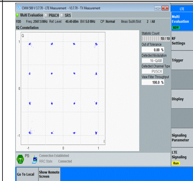
Band7-5MHz-16QAM-21425-25RB#0-PASS
