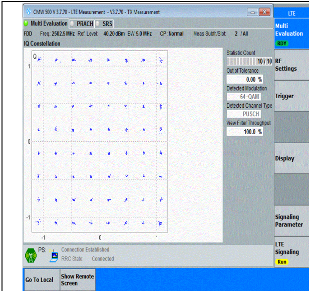
Band7-5MHz-64QAM-20775-25RB#0-PASS
