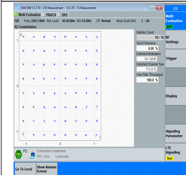
Band7-5MHz-64QAM-21425-25RB#0-PASS
