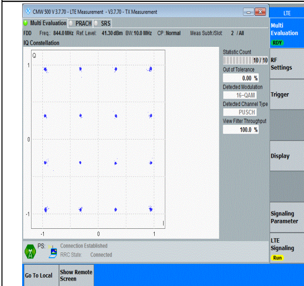
Band5-10MHz-16QAM-20600-50RB#0-PASS
