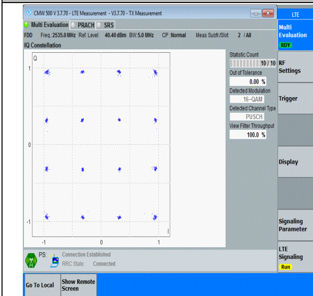
Band7-5MHz-16QAM-21100-25RB#0-PASS
