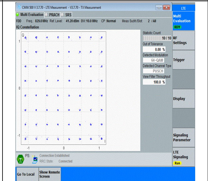
Band5-10MHz-64QAM-20450-50RB#0-PASS
