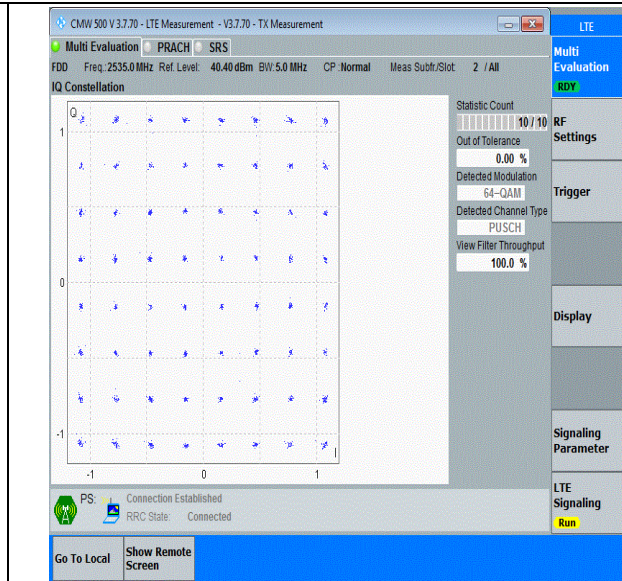
Band7-5MHz-64QAM-21100-25RB#0-PASS
