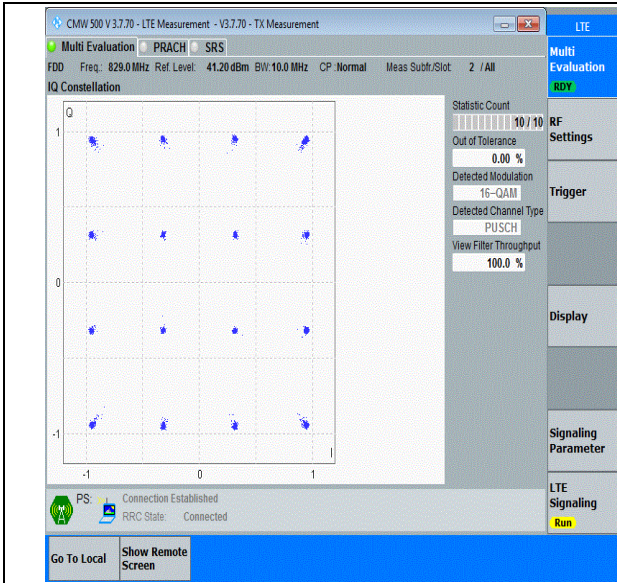
Band5-10MHz-16QAM-20450-50RB#0-PASS
