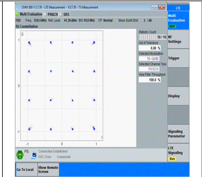
Band5-10MHz-16QAM-20525-50RB#0-PASS
