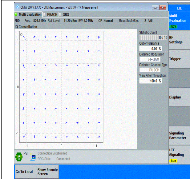
Band5-5MHz-64QAM-20425-25RB#0-PASS
