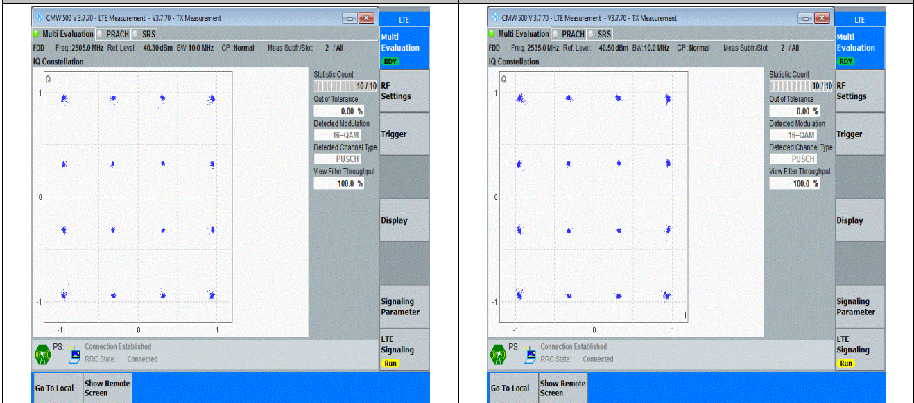
Band7-10MHz-16QAM-20800-50RB#0-PASS
