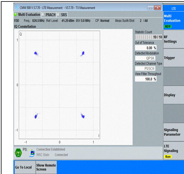
Band5-5MHz-QPSK-20425-25RB#0-PASS
