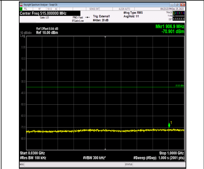
Band41_15MHz_QPSK_40640_1RB#0_30~1000_30~1000
