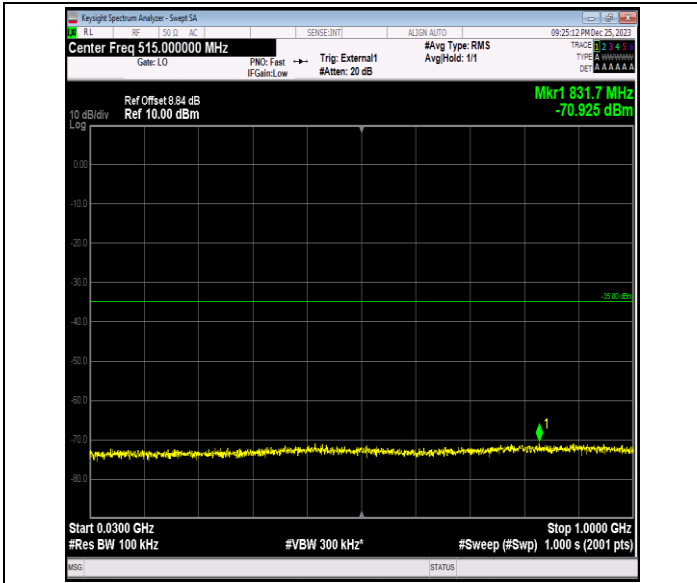
Band41_15MHz_16QAM_40640_1RB#0_30~1000_30~1000
