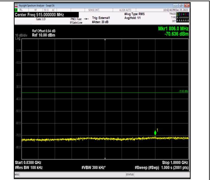
Band41_20MHz_QPSK_40140_1RB#0_30~1000_30~1000
