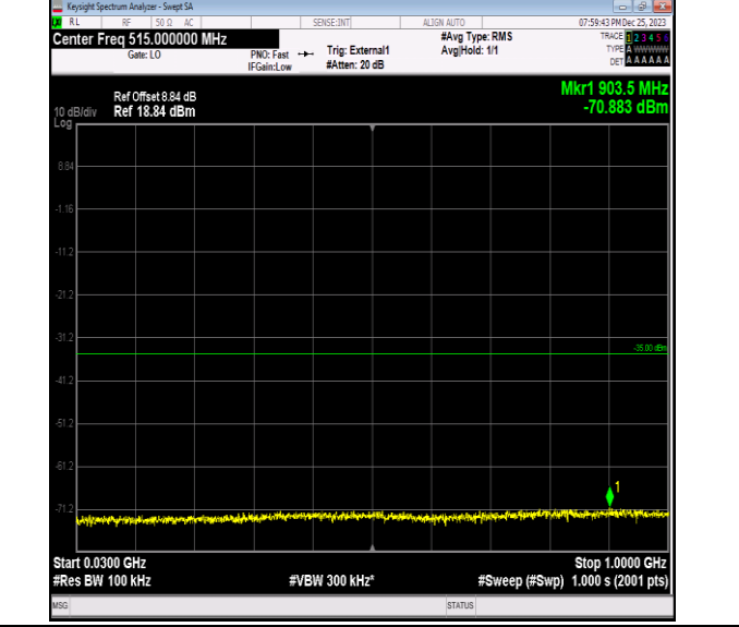
Band41_10MHz_16QAM_40640_1RB#0_30~1000_30~1000
