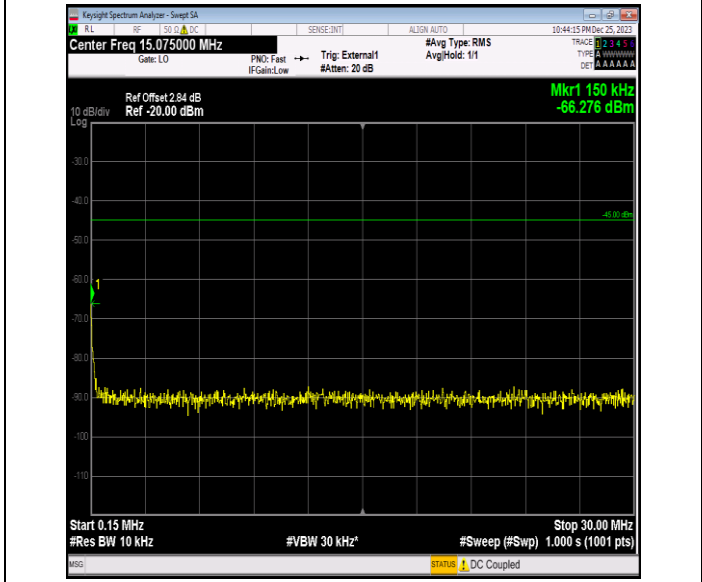
Band41_20MHz_16QAM_40140_1RB#0_0.15~30_0.15~30
