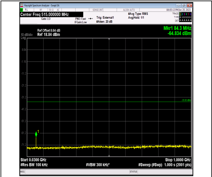
Band41_10MHz_16QAM_41190_1RB#0_30~1000_30~1000
