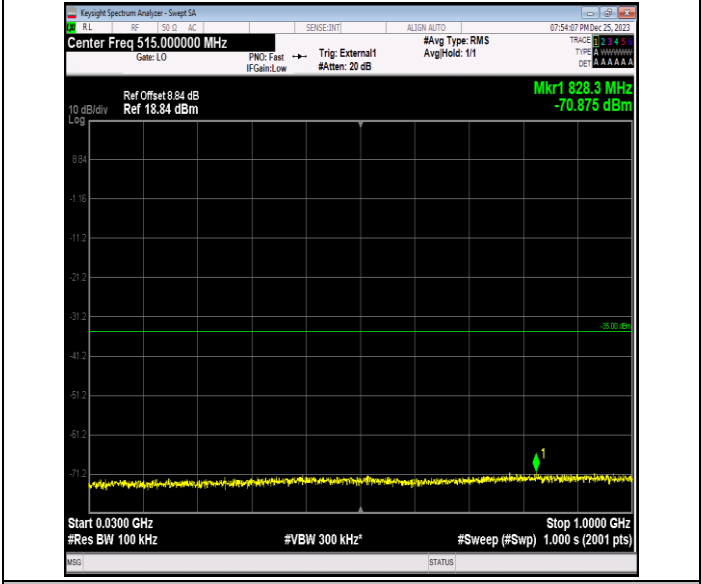
Band41_10MHz_16QAM_40090_1RB#0_30~1000_30~1000
