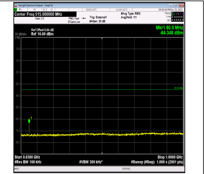
Band41_15MHz_16QAM_41165_1RB#0_30~1000_30~1000
