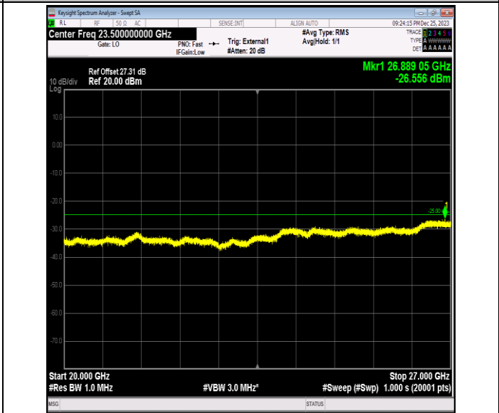
Band41_15MHz_QPSK_40640_1RB#0_20000~27000_20000~27000
