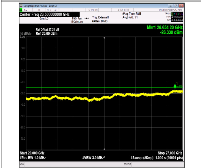
Band41_15MHz_16QAM_40640_1RB#0_20000~27000_20000~27000
