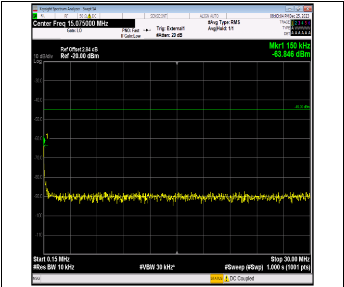
Band41_10MHz_QPSK_41190_1RB#0_0.15~30_0.15~30
