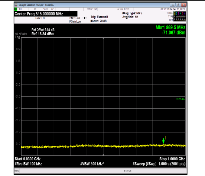
Band41_10MHz_64QAM_40090_1RB#0_30~1000_30~1000
