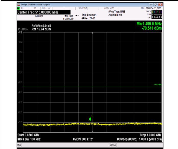
Band41_10MHz_64QAM_40640_1RB#0_30~1000_30~1000
