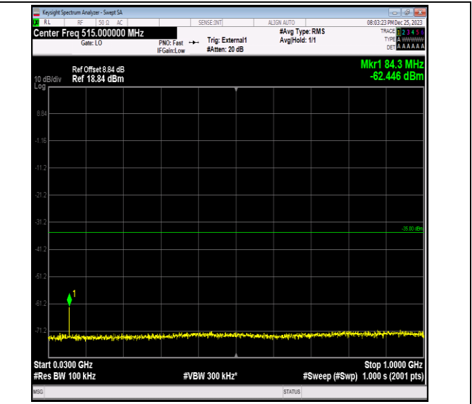
Band41_10MHz_QPSK_41190_1RB#0_30~1000_30~1000
