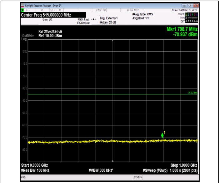
Band41_20MHz_16QAM_40140_1RB#0_30~1000_30~1000
