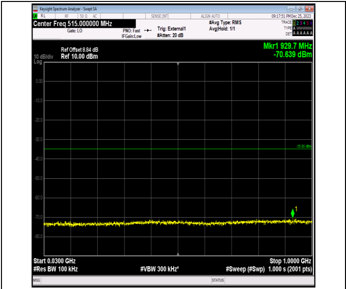
Band41_15MHz_QPSK_40115_1RB#0_30~1000_30~1000
