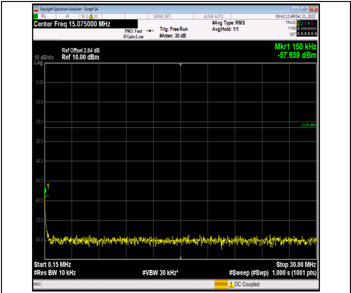
Band12_10MHz_16QAM_23095_1RB#0_0.15~30_0.15~30
