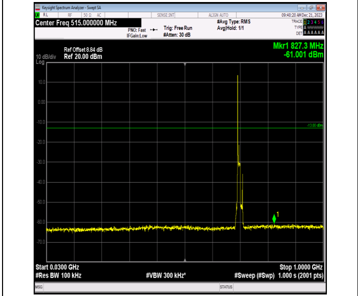
Band12_10MHz_64QAM_23060_1RB#0_30~1000_30~1000
