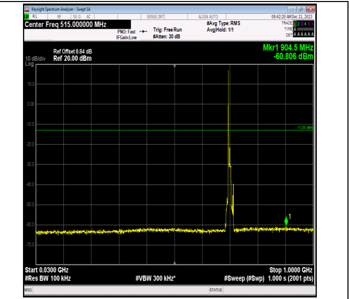
Band12_10MHz_16QAM_23095_1RB#0_30~1000_30~1000
