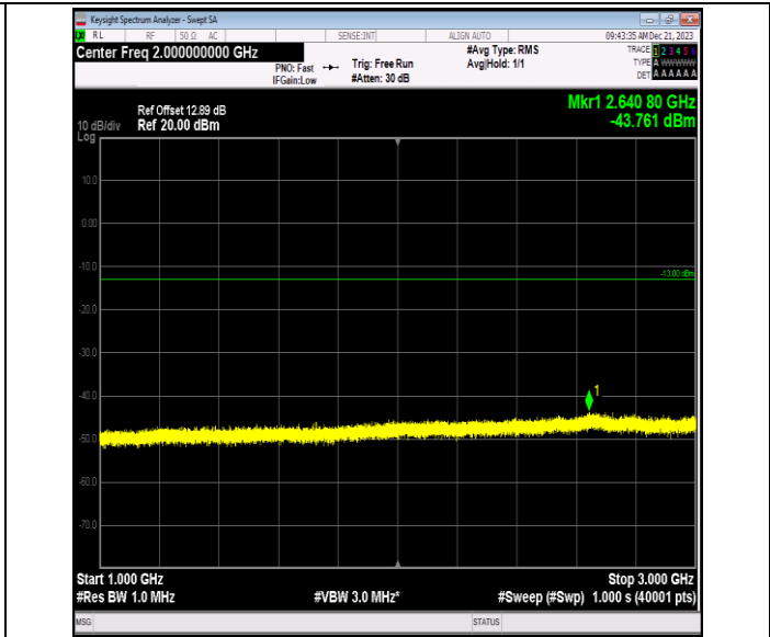
Band12_10MHz_64QAM_23095_1RB#0_1000~3000_1000~3000
