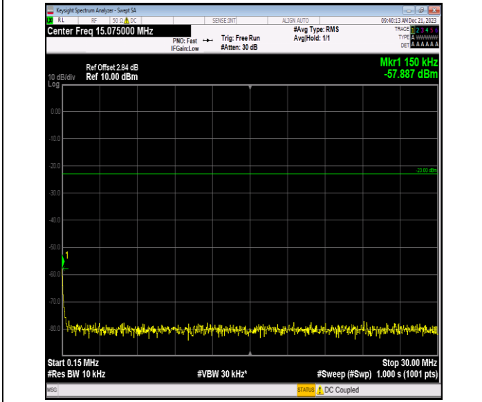
Band12_10MHz_64QAM_23060_1RB#0_0.15~30_0.15~30
