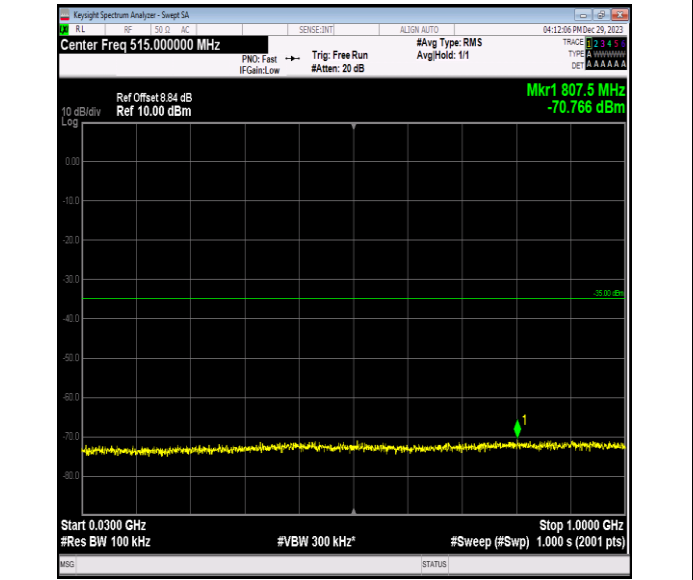
Band7_10MHz_QPSK_20800_1RB#0_30~1000_30~1000
