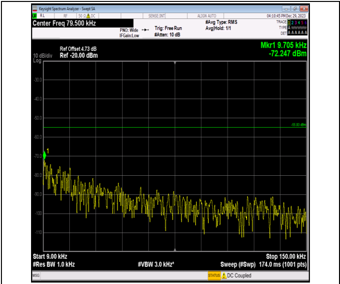
Band7_5MHz_64QAM_21425_1RB#0_0.009~0.15_0.009~0.1 5
