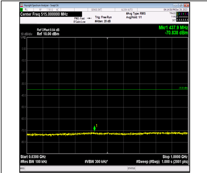
Band7_10MHz_QPSK_21100_1RB#0_30~1000_30~1000
