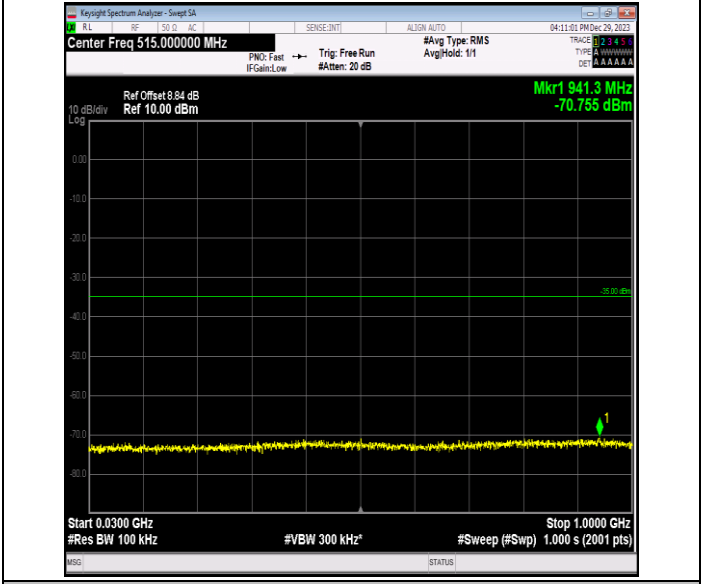
Band7_5MHz_64QAM_21425_1RB#0_30~1000_30~1000
