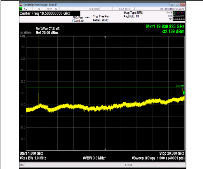
Band7_10MHz_QPSK_21400_1RB#0_1000~20000_1000~20000
