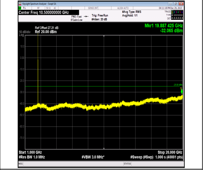
Band7_5MHz_64QAM_21425_1RB#0_1000~20000_1000~20000
