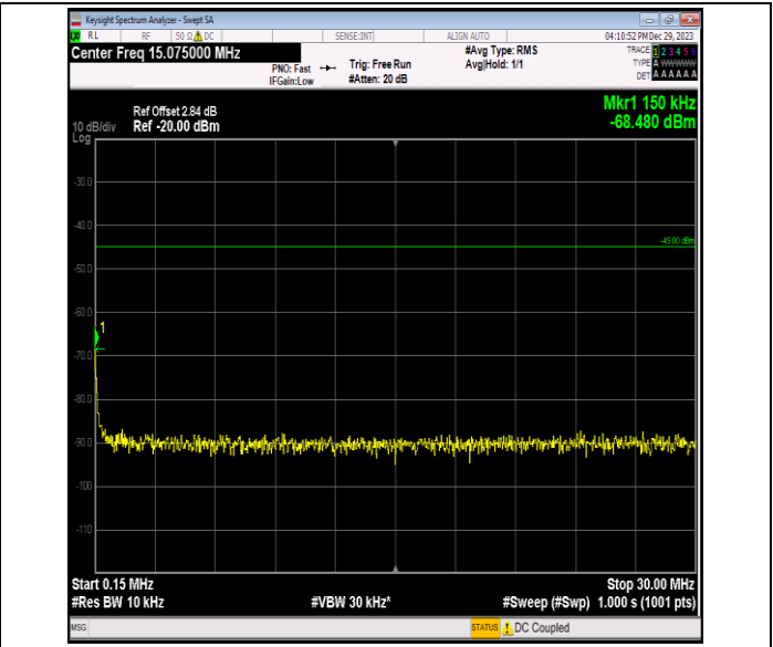
Band7_5MHz_64QAM_21425_1RB#0_0.15~30_0.15~30
