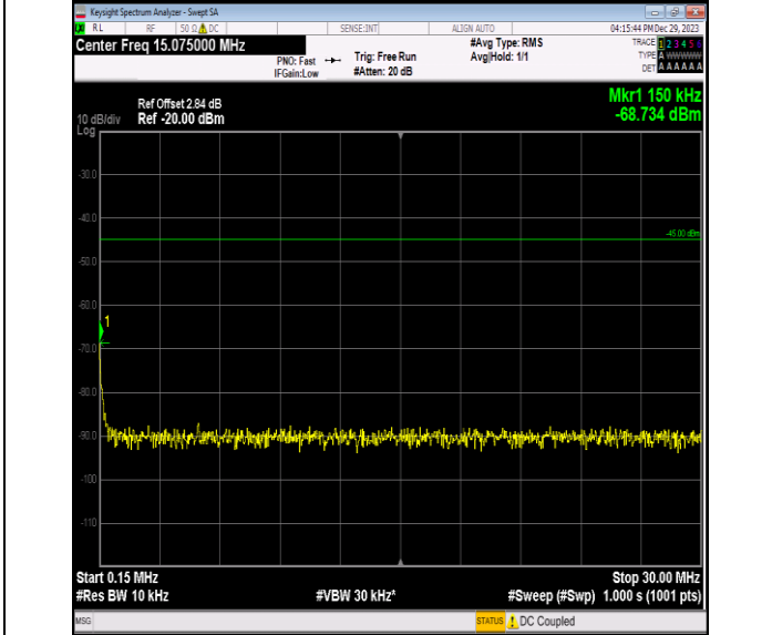
Band7_10MHz_16QAM_21100_1RB#0_0.15~30_0.15~30
