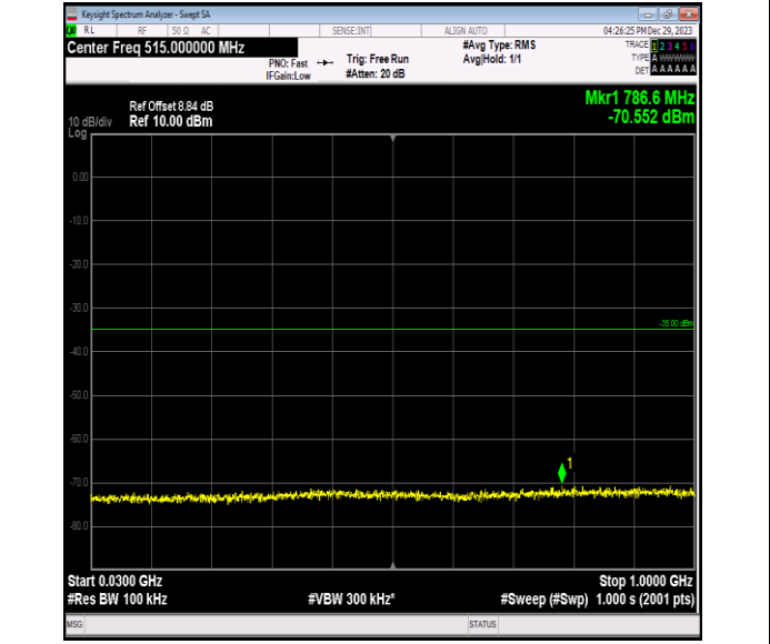
Band7_15MHz_16QAM_20825_1RB#0_30~1000_30.6~1000
