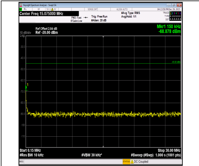
Band7_10MHz_64QAM_20800_1RB#0_0.15~30.0.15~30
