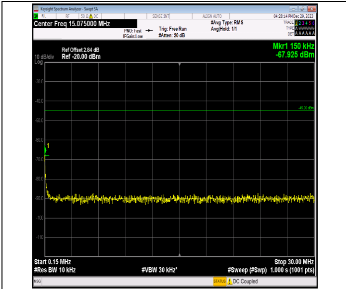
Band7_15MHz_QPSK_21100_1RB#0_0.15~30_0.15~30
