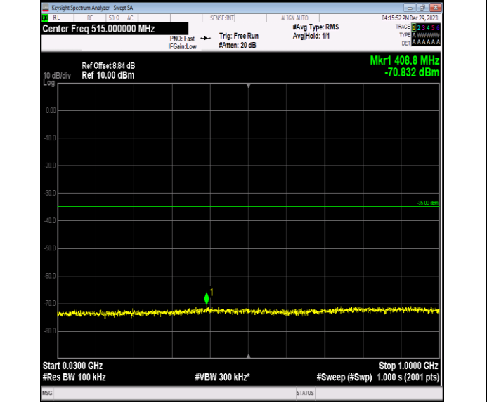
Band7_10MHz_16QAM_21100_1RB#0_30~1000_30~1000
