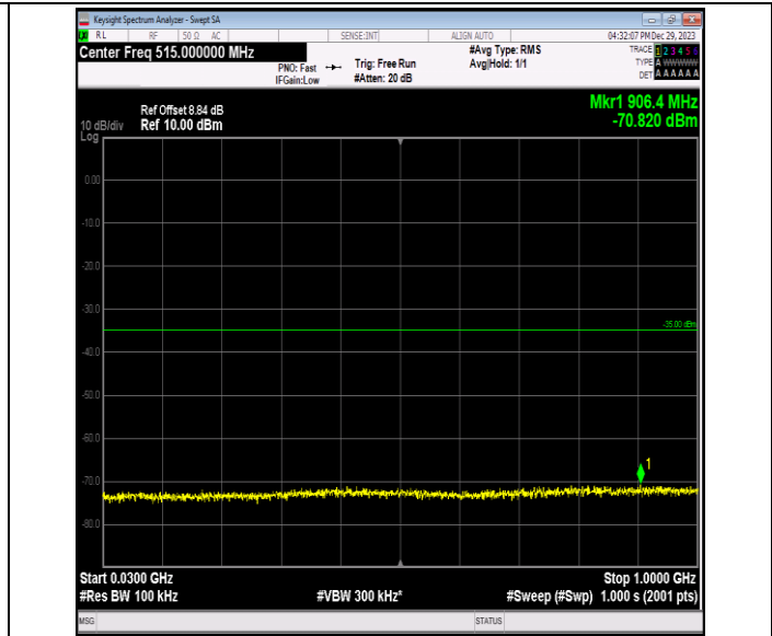
Band7_15MHz_16QAM_21375_1RB#0_30~1000_30~1000
