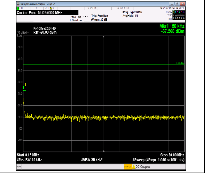
Band7_15MHz_QPSK_20825_1RB#0_0.15~30_0.15~30
