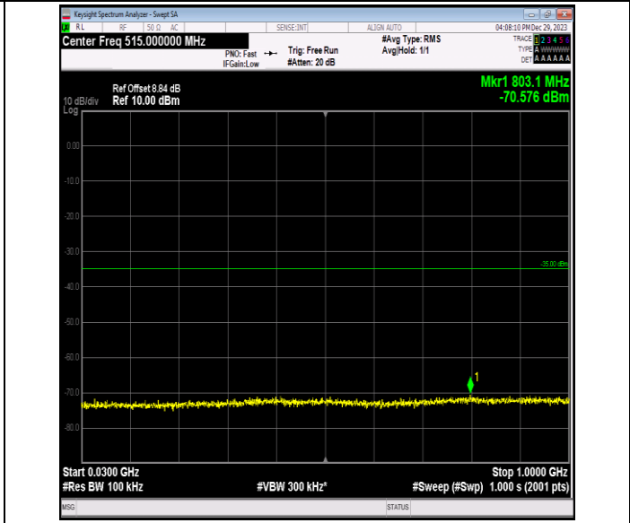
Band7_5MHz_64QAM_21100_1RB#0_30~1000_30~1000
