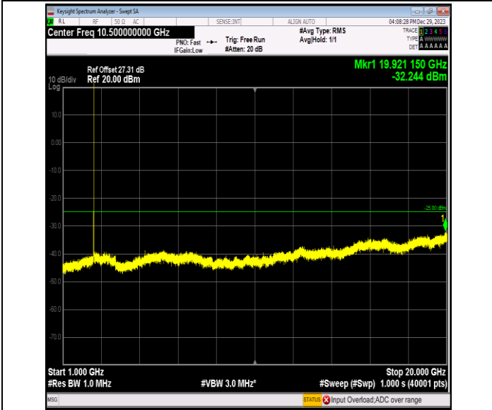
Band7_5MHz_64QAM_21100_1RB#0_1000~20000_1000~20000
