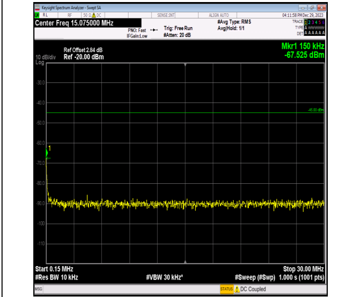
Band7_10MHz_QPSK_20800_1RB#0_0.15~30_0.15~30
