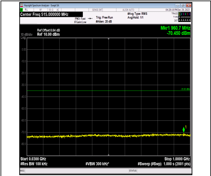
Band7_15MHz_16QAM_21100_1RB#0_30~1000_30~1000
