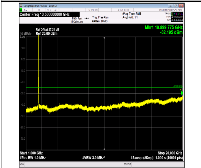
Band7_15MHz_QPSK_21100_1RB#0_1000~20000_1000~20000
