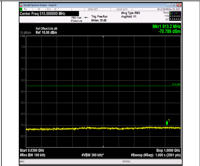
Band7_10MHz_64QAM_20800_1RB#0_30~1000.30~1000
