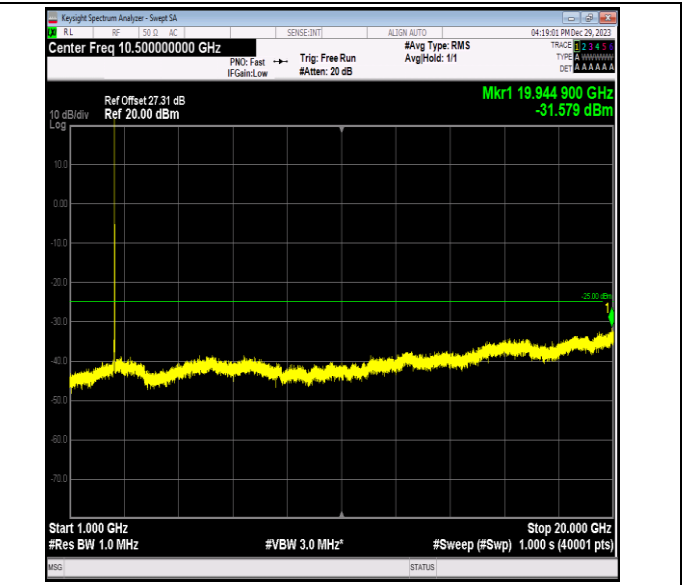
Band7_10MHz_16QAM_21400_1RB#0_1000~20000_1000~20000
