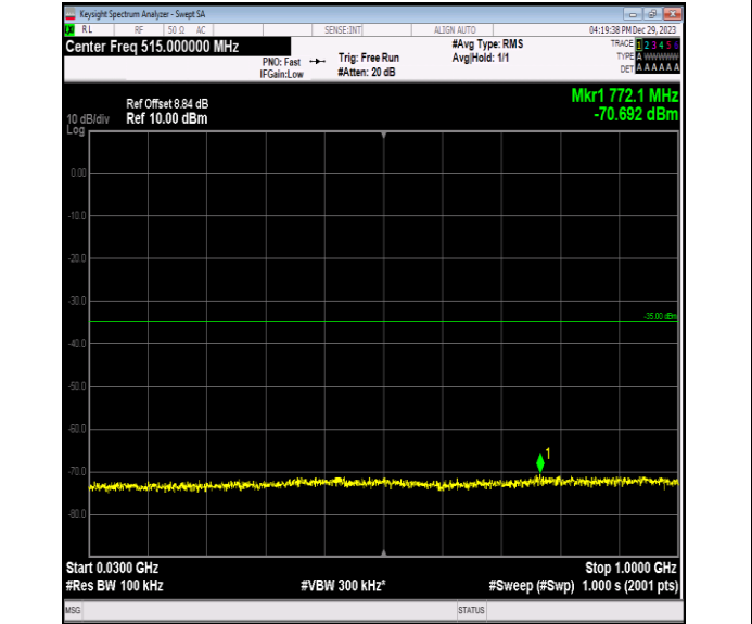
Band7_10MHz_64QAM_21400_1RB#0_30~1000_30.1~1000
