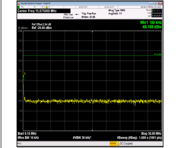
Band7_15MHz_16QAM_20825_1RB#0_0.15~30_0.15~30
