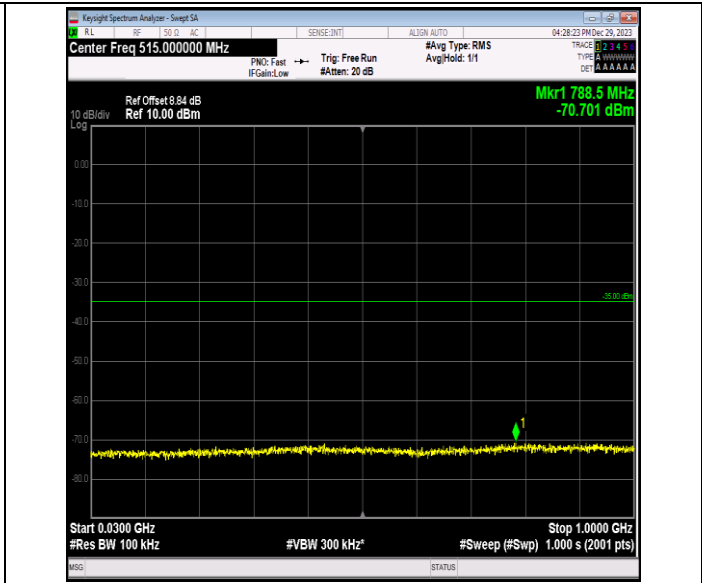
Band7_15MHz_QPSK_21100_1RB#0_30~1000_30~1000
