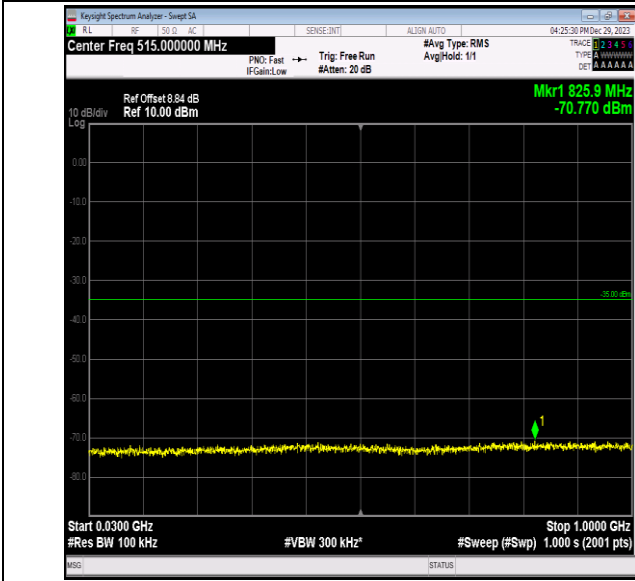
Band7_15MHz_QPSK_20825_1RB#0_30~1000_30~1000
