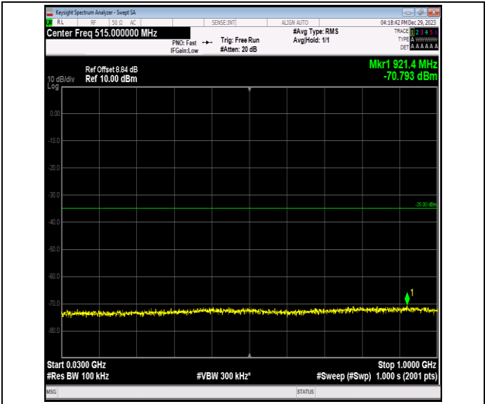
Band7_10MHz_16QAM_21400_1RB#0_30~1000_30~1000
