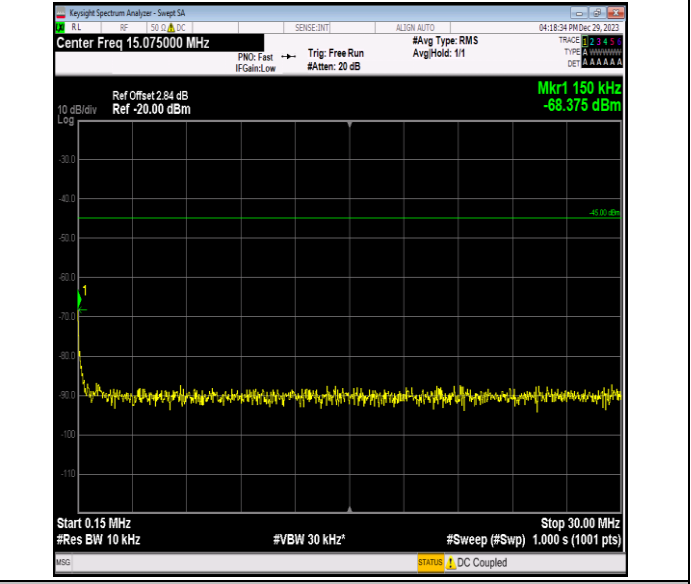
Band7_10MHz_16QAM_21400_1RB#0_0.15~30_0.15~30
