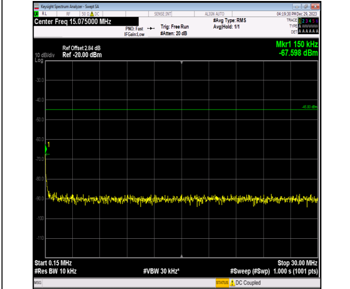
Band7_10MHz_64QAM_21400_1RB#0_0.15~30_0.15~30
