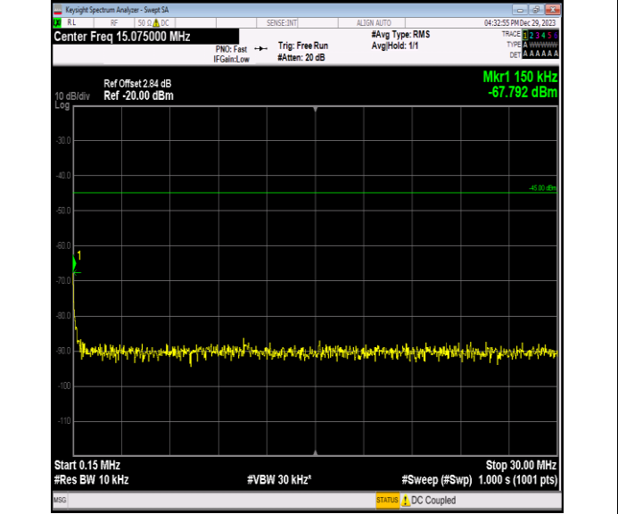
Band7_15MHz_64QAM_21375_1RB#0_0.15~30_0.15~30
