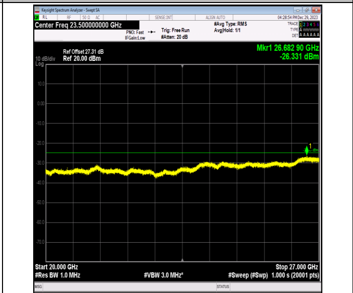
Band7_15MHz_QPSK_21100_1RB#0_20000~27000_20000~27000
