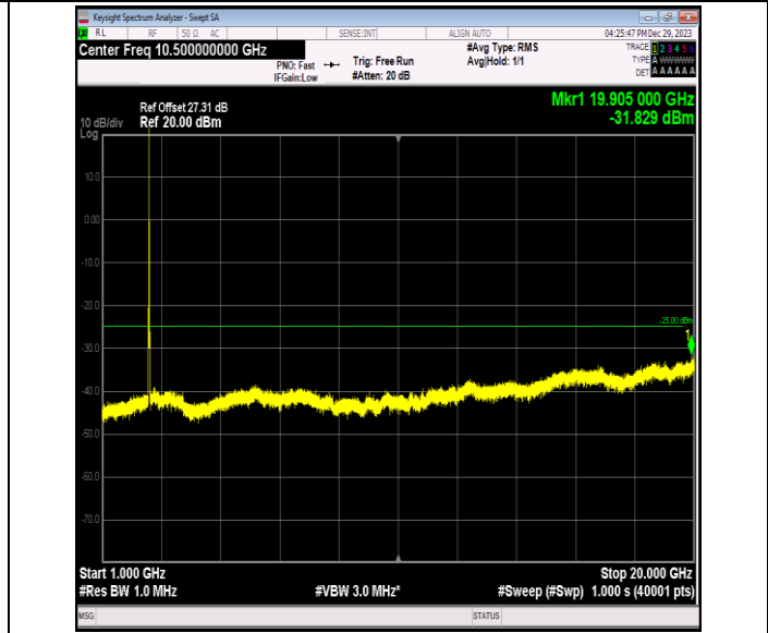
Band7_15MHz_QPSK_20825_1RB#0_1000~20000_1000~20000
