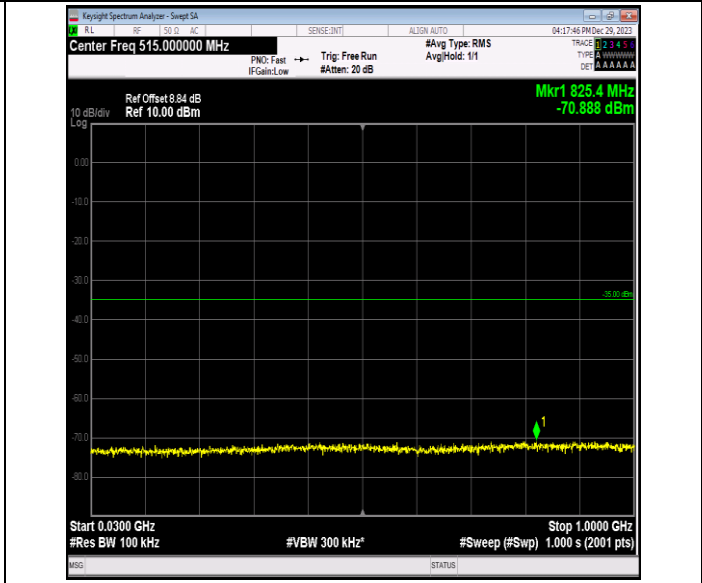
Band7_10MHz_QPSK_21400_1RB#0_30~1000_30~1000
