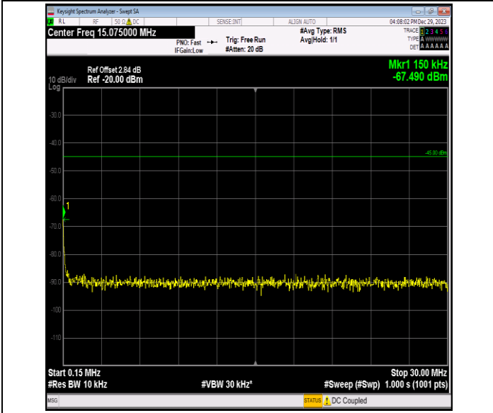
Band7_5MHz_64QAM_21100_1RB#0_0.15~30_0.15~30
