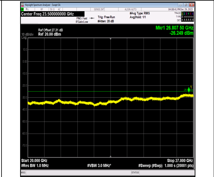
Band7_5MHz_64QAM_21100_1RB#0_20000~27000_20000~27000
