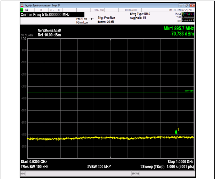
Band7_15MHz_64QAM_21375_1RB#0_30~1000_30~1000
