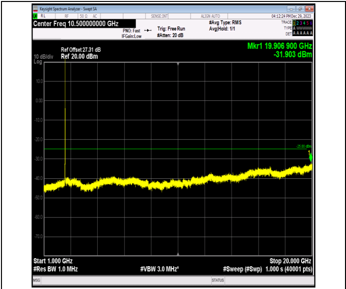
Band7_10MHz_QPSK_20800_1RB#0_1000~20000_1000~20000
