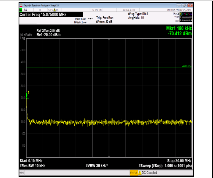
Band7_15MHz_QPSK_21375_1RB#0_0.15~30_0.15~30
