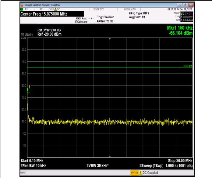
Band7_10MHz_QPSK_21400_1RB#0_0.15~30_0.15~30
