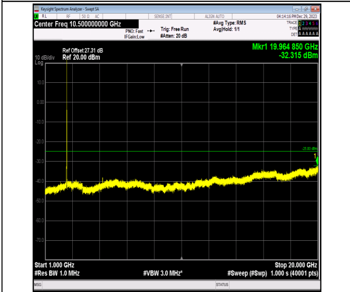
Band7_10MHz_64QAM_20800_1RB#0_1000~20000_1000~20000
