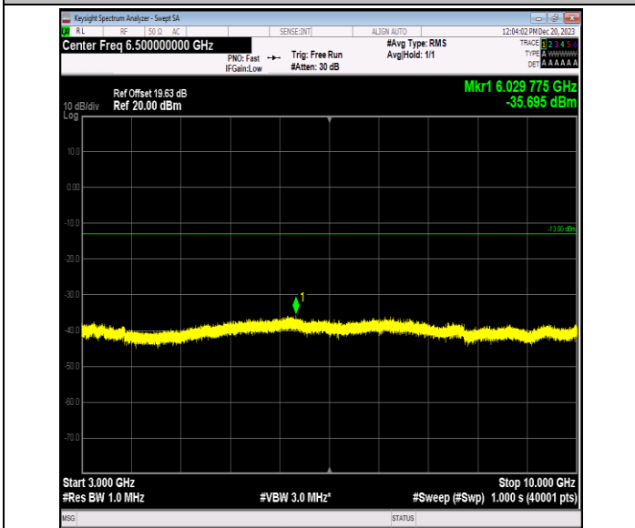
Band5_5MHz_QPSK_20425_1RB#0_3000~10000_3000~10000
