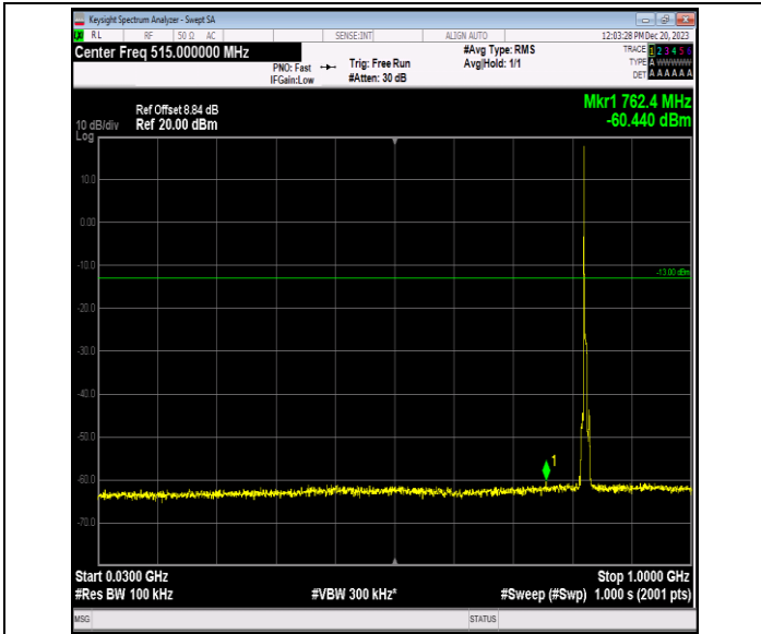
Band5_5MHz_QPSK_20425_1RB#0_30~1000_30~1000
