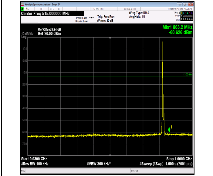
Band5_5MHz_16QAM_20425_1RB#0_30~1000_30~1000
