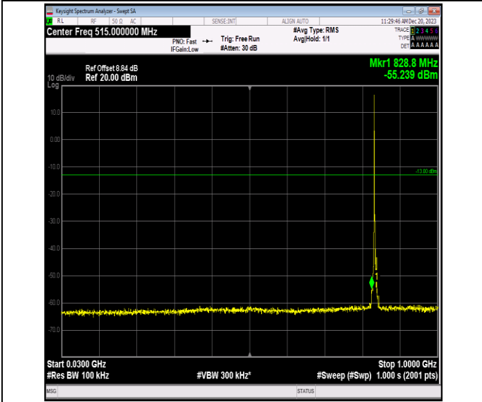
Band5_3MHz_QPSK_20525_1RB#0_30~1000_30~1000
