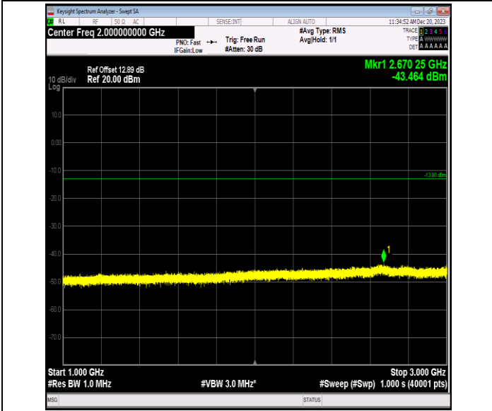
Band5_3MHz_64QAM_20635_1RB#0_1000~3000_1000~300
