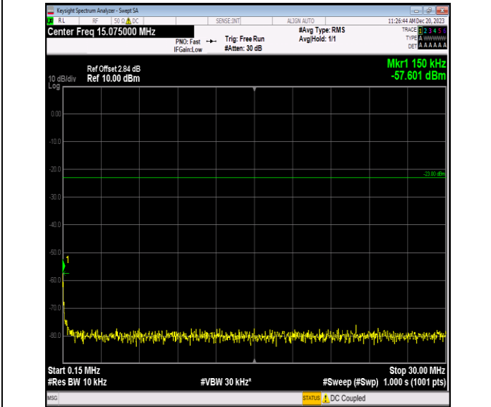
Band5_3MHz_QPSK_20415_1RB#0_0.15~30_0.15~30
