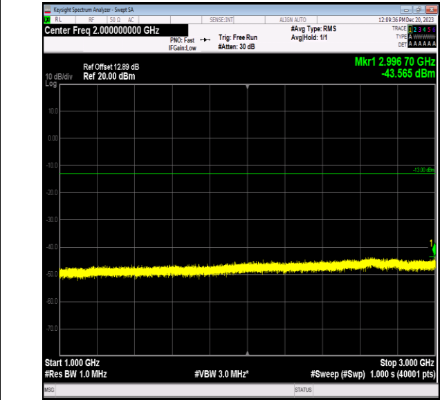
Band5_5MHz_QPSK_20625_1RB#0_1000~3000_1000~3000
