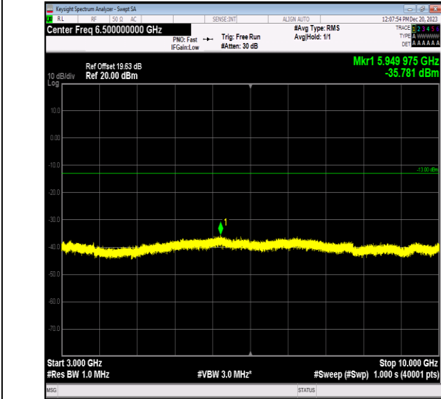
Band5_5MHz_16QAM_20525_1RB#0_3000~10000_3000~10000 000
