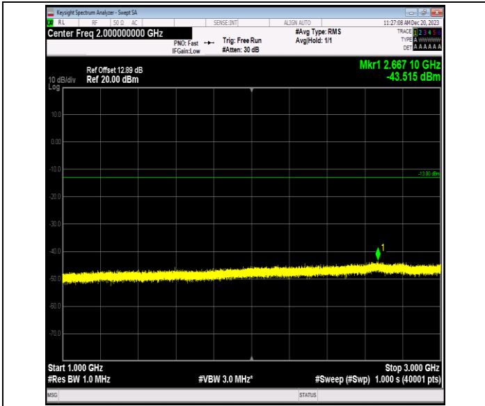
Band5_3MHz_QPSK_20415_1RB#0_1000~3000_1000~3000
