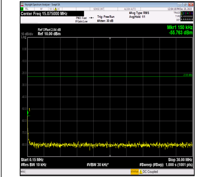
Band5_5MHz_16QAM_20425_1RB#0_0.15~30_0.15~30
