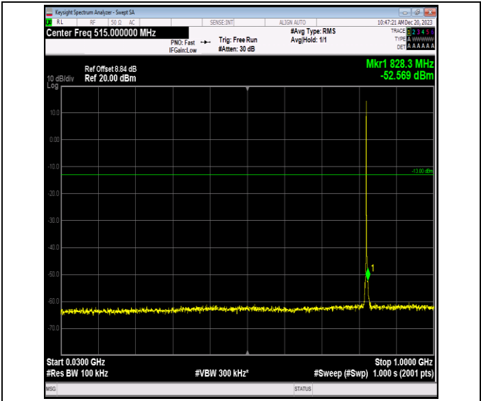
Band5_1.4MHz_64QAM_20407_1RB#0_30~1000_30~1000
