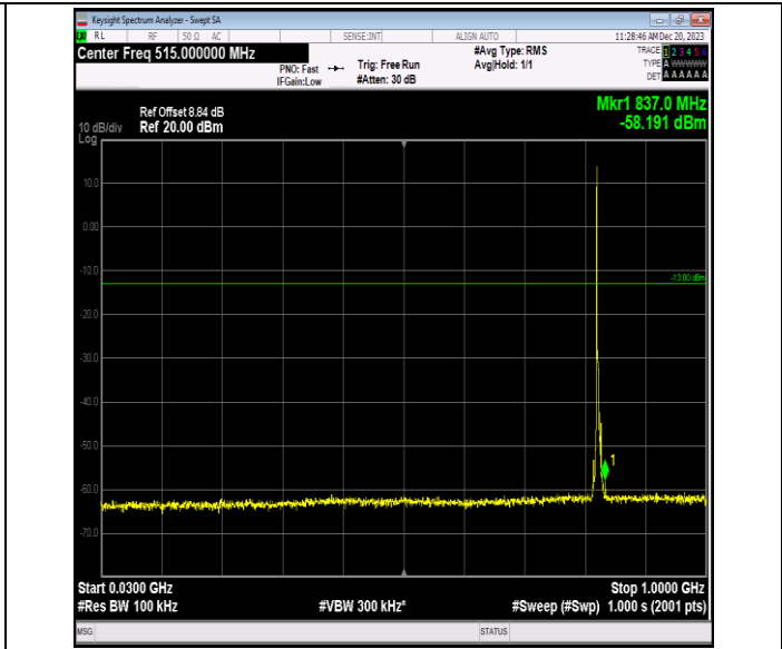
Band5_3MHz_64QAM_20415_1RB#0_30~1000_30~1000
