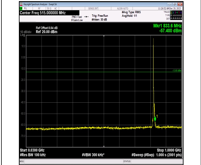
Band5_3MHz_QPSK_20415_1RB#0_30~1000_30~1000
