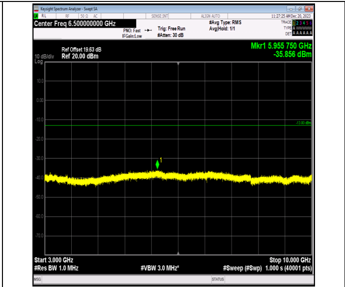
Band5_3MHz_QPSK_20415_1RB#0_3000~10000_3000~10000
