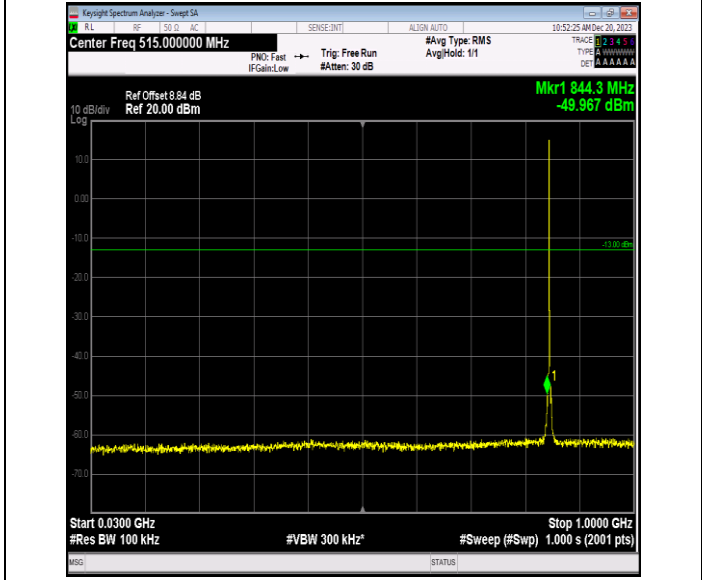
Band5_1.4MHz_16QAM_20643_1RB#0_30~1000_30~1000
