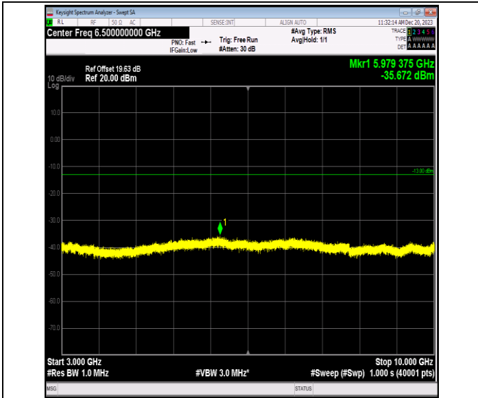
Band5_3MHz_64QAM_20525_1RB#0_3000~10000_3000~10000 000
