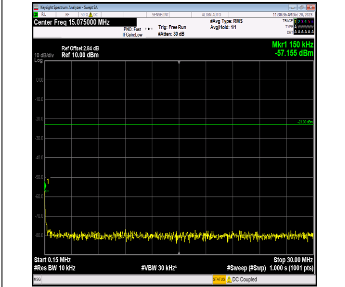
Band5_3MHz_16QAM_20525_1RB#0_0.15~30_0.15~30
