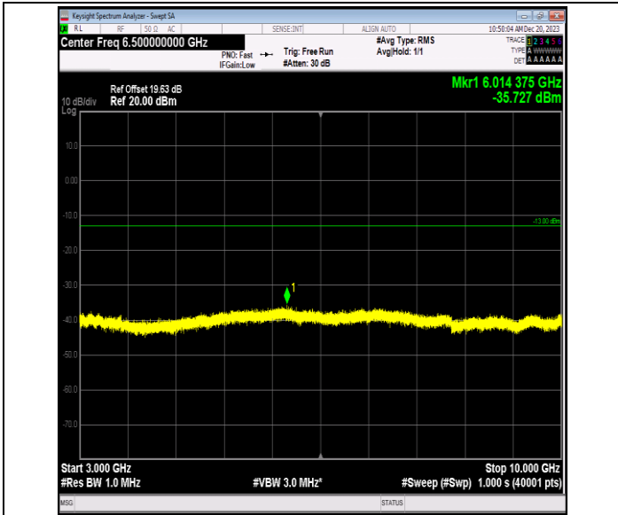
Band5_1.4MHz_16QAM_20525_1RB#0_3000~10000_3000~10000
