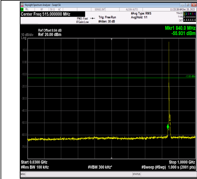
Band5_3MHz_16QAM_20635_1RB#0_30~1000_30~1000
