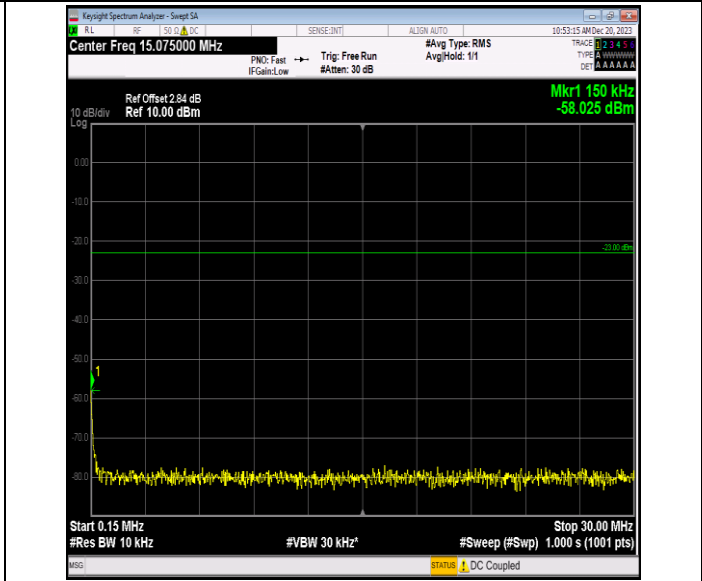
Band5_1.4MHz_64QAM_20643_1RB#0_0.15~30_0.15~30
