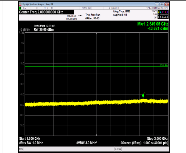
Band5_5MHz_16QAM_20525_1RB#0_1000~3000_1000~3000 0
