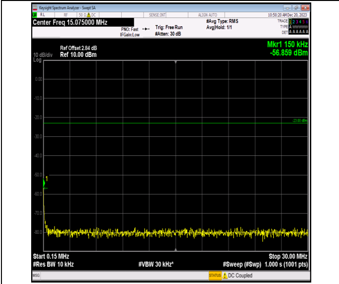
Band5_1.4MHz_64QAM_20525_1RB#0_0.15~30_0.15~30
