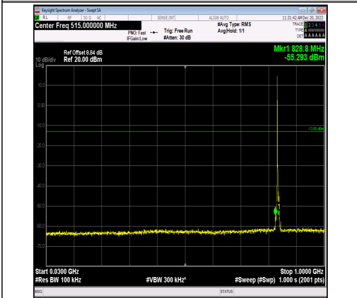
Band5_3MHz_64QAM_20525_1RB#0_30~1000_30~1000
