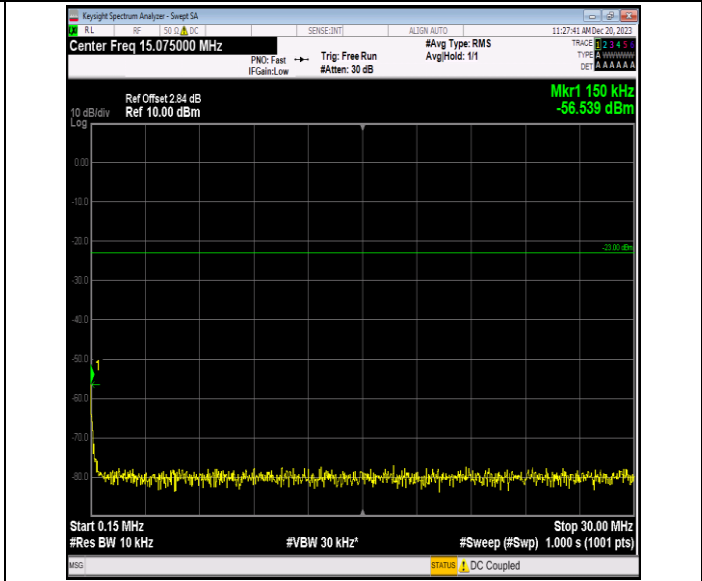
Band5_3MHz_16QAM_20415_1RB#0_0.15~30_0.15~30
