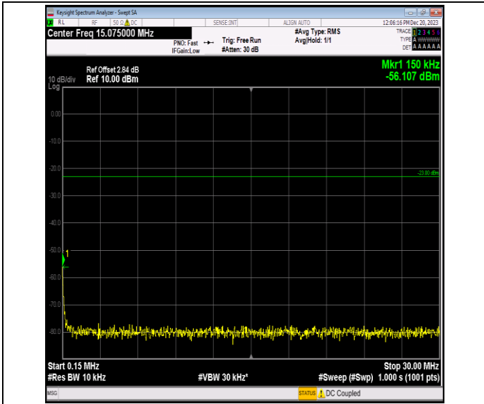
Band5_5MHz_QPSK_20525_1RB#0_0.15~30_0.15~30
