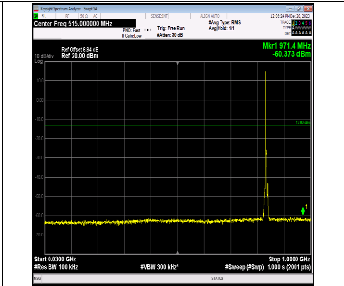
Band5_5MHz_QPSK_20525_1RB#0_30~1000_30~1000
