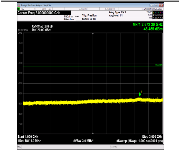
Band5_3MHz_64QAM_20415_1RB#0_1000~3000_1000~300
