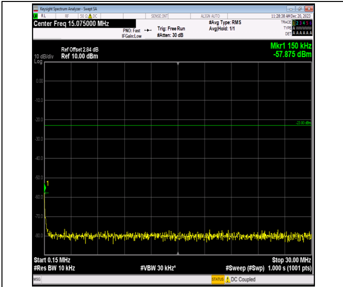
Band5_3MHz_64QAM_20415_1RB#0_0.15~30_0.15~30
