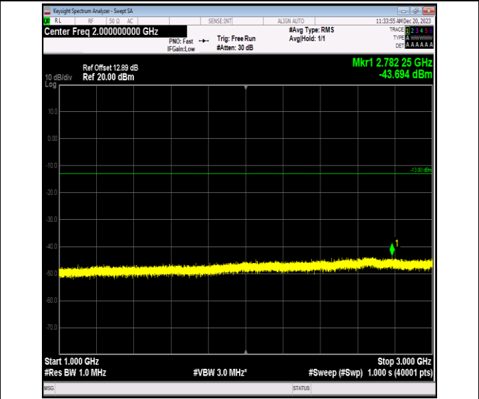
Band5_3MHz_16QAM_20635_1RB#0_1000~3000_1000~3000 0
