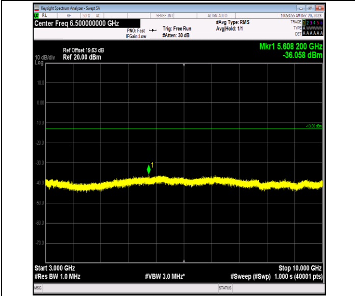
Band5_1.4MHz_64QAM_20643_1RB#0_3000~10000_3000~10000
