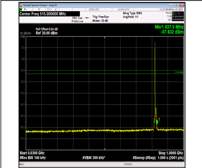
Band5_3MHz_16QAM_20415_1RB#0_30~1000_30~1000
