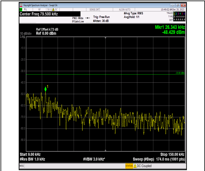
Band5_1.4MHz_16QAM_20525_1RB#0_0.009~0.15_0.009~0.15
