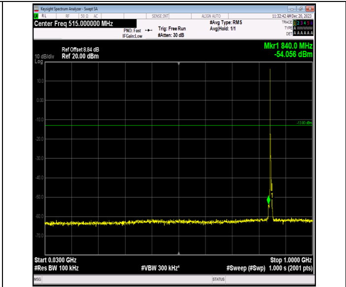
Band5_3MHz_QPSK_20635_1RB#0_30~1000_30~1000
