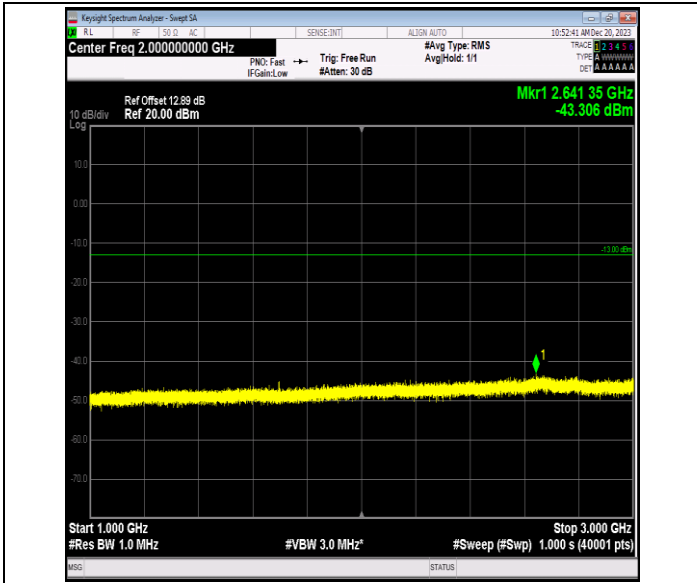
Band5_1.4MHz_16QAM_20643_1RB#0_1000~3000_1000~3000
