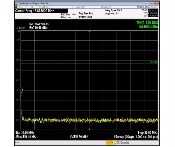
Band5_3MHz_16QAM_20635_1RB#0_0.15~30_0.15~30
