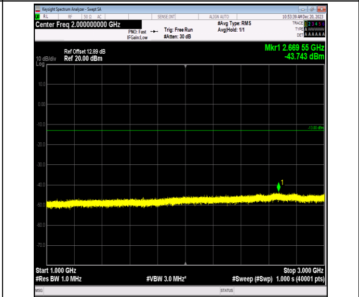
Band5_1.4MHz_64QAM_20643_1RB#0_1000~3000_1000~3000
