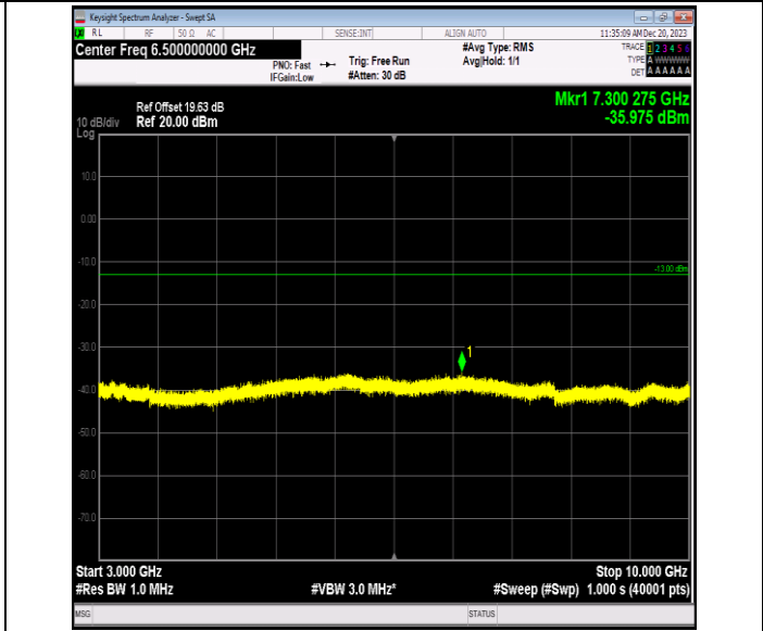
Band5_3MHz_64QAM_20635_1RB#0_3000~10000_3000~10
