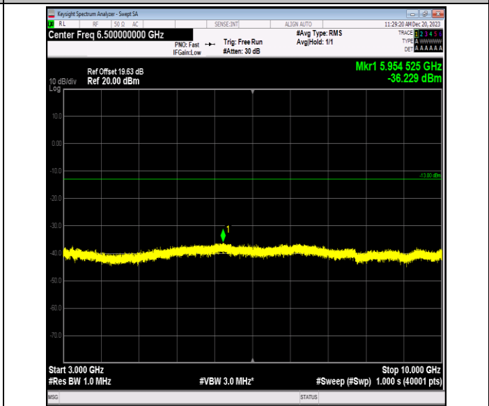
Band5_3MHz_64QAM_20415_1RB#0_3000~10000_3000~10
