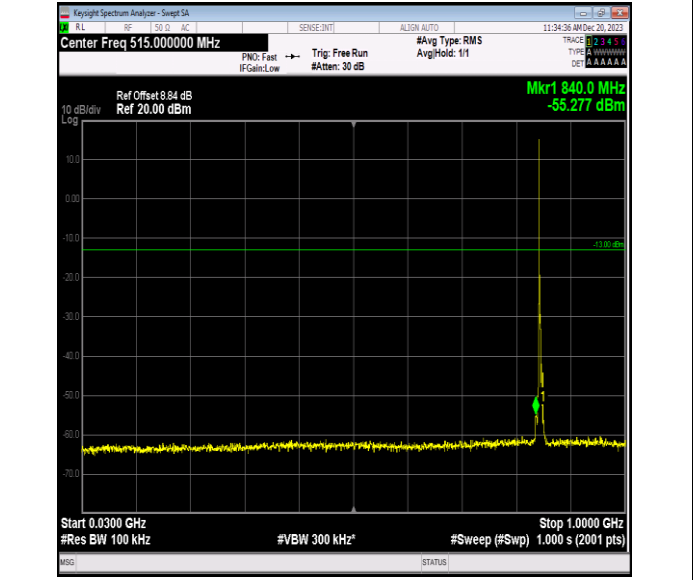
Band5_3MHz_64QAM_20635_1RB#0_30~1000_30~1000
