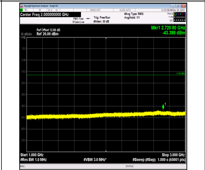
Band5_3MHz_64QAM_20525_1RB#0_1000~3000_1000~300 0
