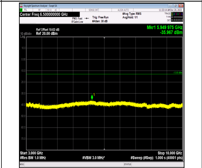
Band5_3MHz_QPSK_20635_1RB#0_3000~10000_3000~10000
