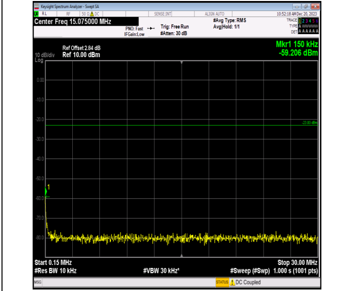
Band5_1.4MHz_16QAM_20643_1RB#0_0.15~30_0.15~30
