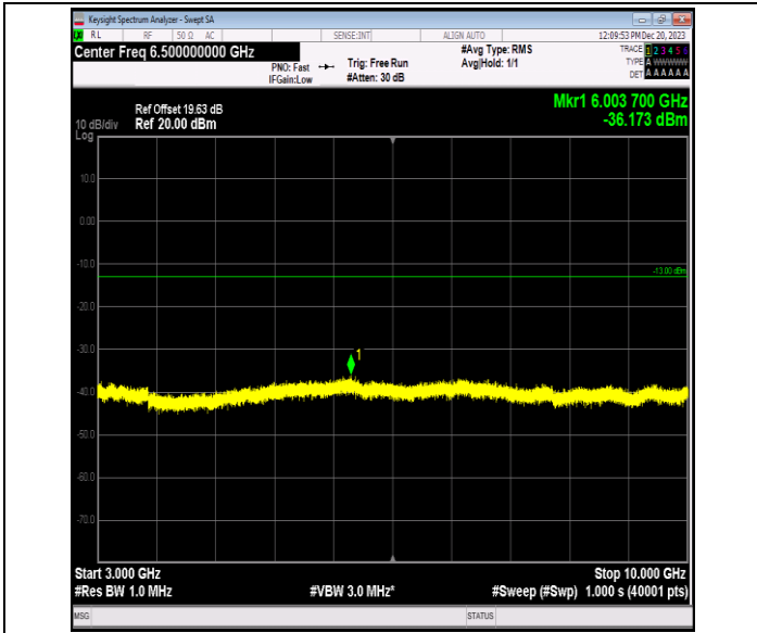
Band5_5MHz_QPSK_20625_1RB#0_3000~10000_3000~10000 00
