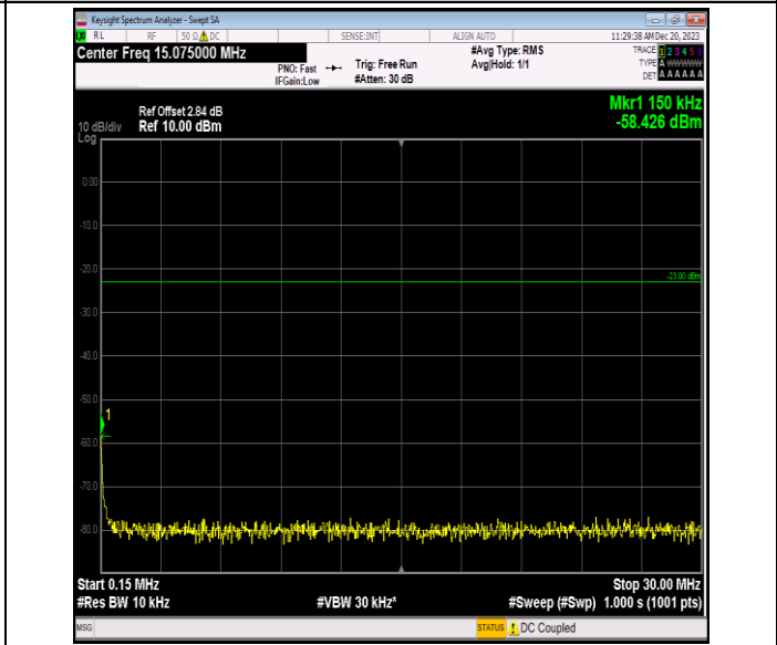
Band5_3MHz_QPSK_20525_1RB#0_0.15~30_0.15~30
