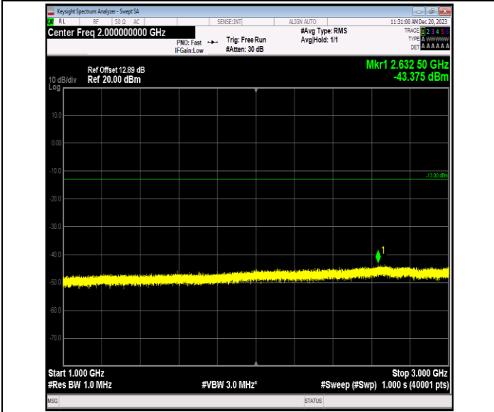
Band5_3MHz_16QAM_20525_1RB#0_1000~3000_1000~300 0
