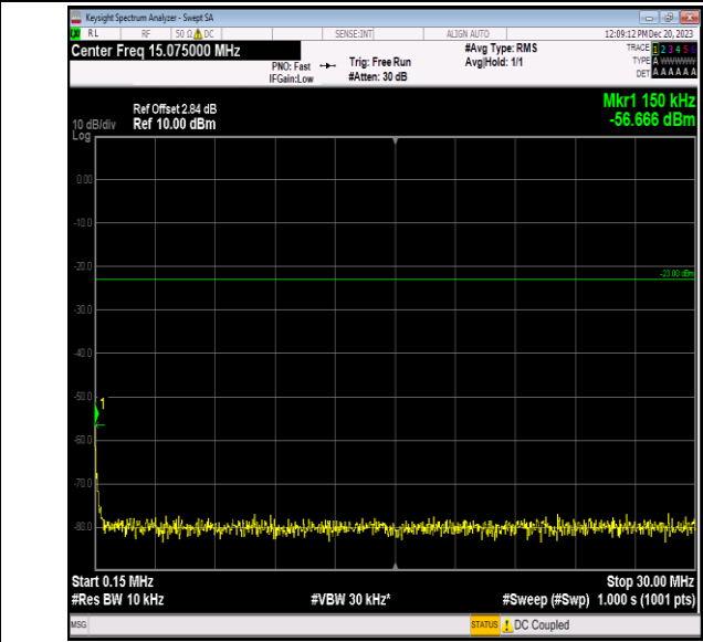
Band5_5MHz_QPSK_20625_1RB#0_0.15~30_0.15~30
