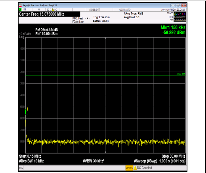
Band5_1.4MHz_16QAM_20525_1RB#0_0.15~30_0.15~30
