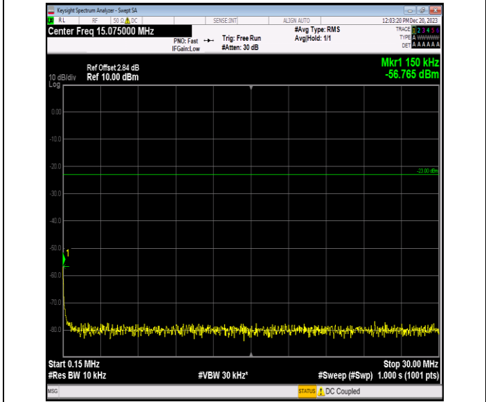
Band5_5MHz_QPSK_20425_1RB#0_0.15~30_0.15~30
