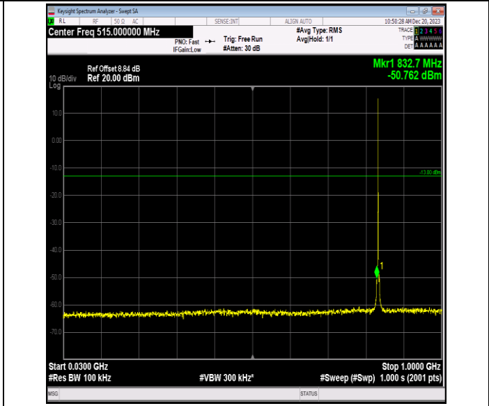
Band5_1.4MHz_64QAM_20525_1RB#0_30~1000_30~1000
