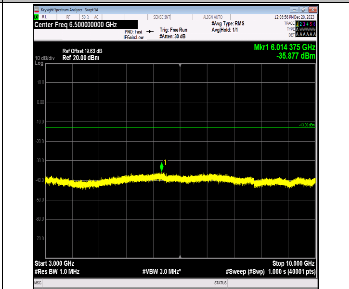
Band5_5MHz_QPSK_20525_1RB#0_3000~10000_3000~100
