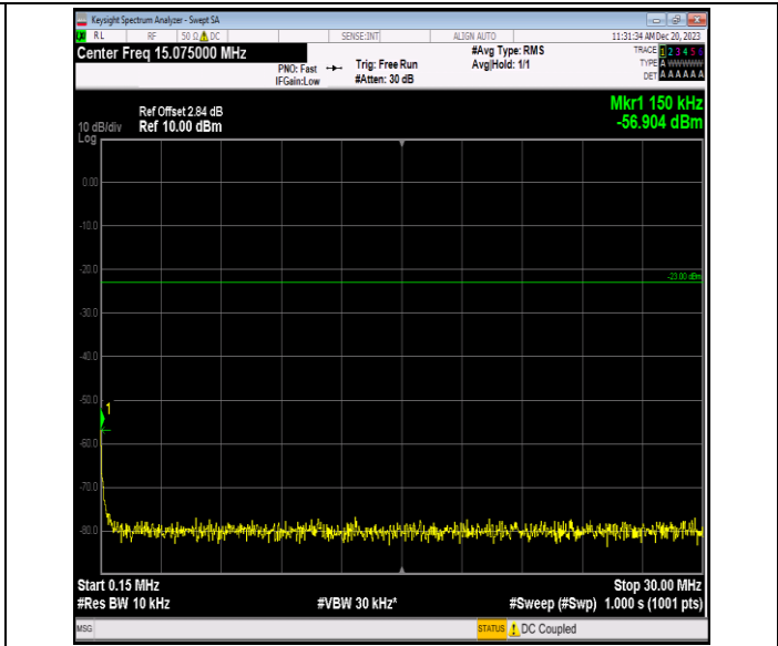
Band5_3MHz_64QAM_20525_1RB#0_0.15~30_0.15~30
