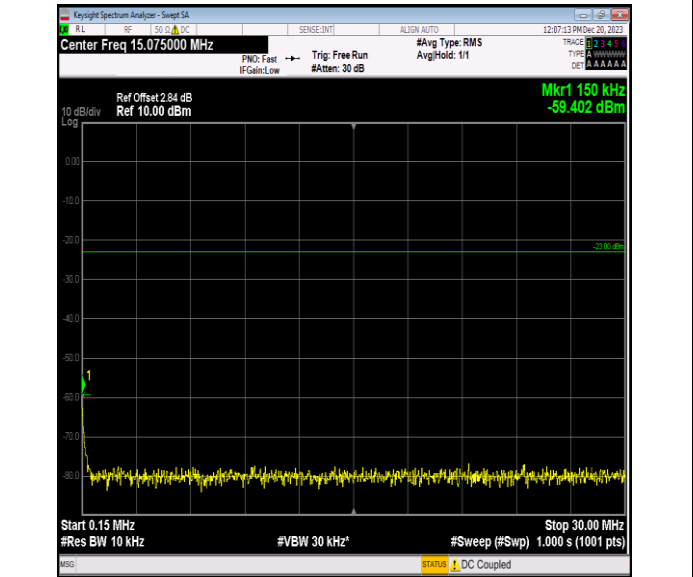
Band5_5MHz_16QAM_20525_1RB#0_0.15~30_0.15~30
