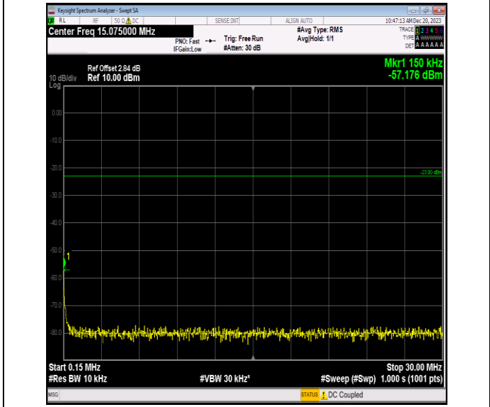
Band5_1.4MHz_64QAM_20407_1RB#0_0.15~30_0.15~30
