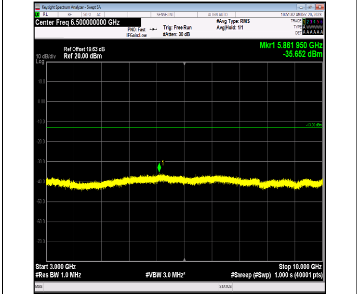
Band5_1.4MHz_64QAM_20525_1RB#0_3000~10000_3000~
