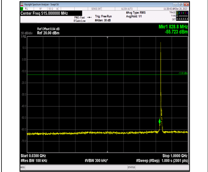
Band5_3MHz_16QAM_20525_1RB#0_30~1000_30~1000
