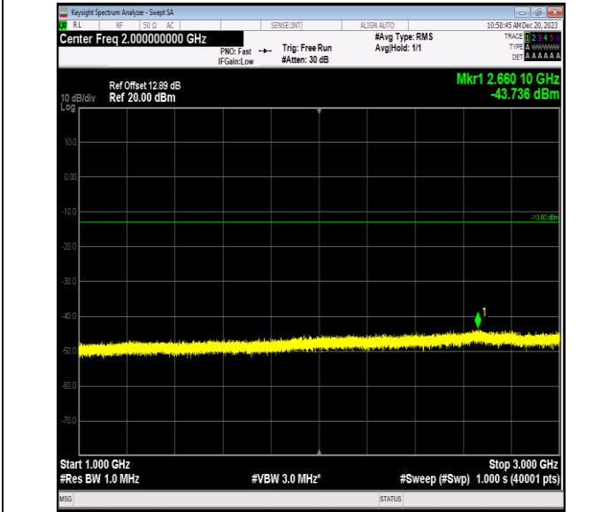
Band5_1.4MHz_64QAM_20525_1RB#0_1000~3000_1000~3
