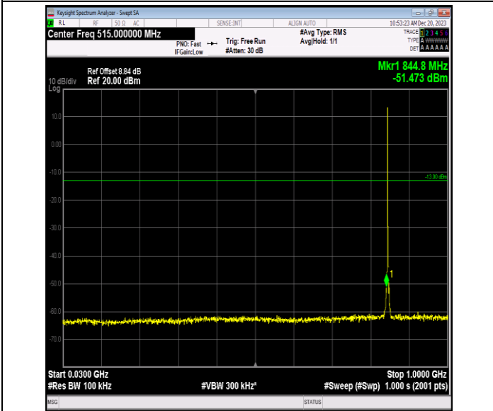
Band5_1.4MHz_64QAM_20643_1RB#0_30~1000_30~1000
