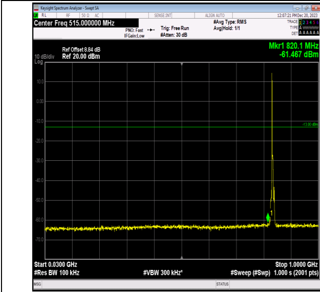
Band5_5MHz_16QAM_20525_1RB#0_30~1000_30~1000
