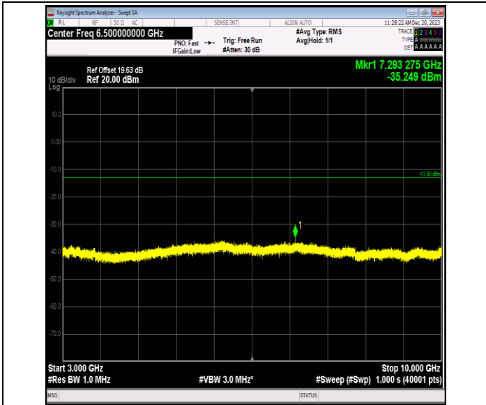
Band5_3MHz_16QAM_20415_1RB#0_3000~10000_3000~10000 000
