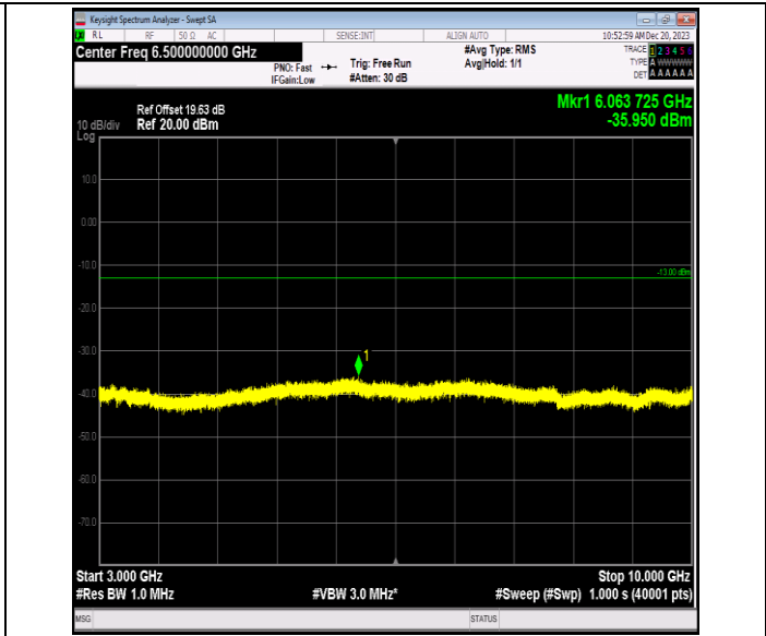
Band5_1.4MHz_16QAM_20643_1RB#0_3000~10000_3000~10000
