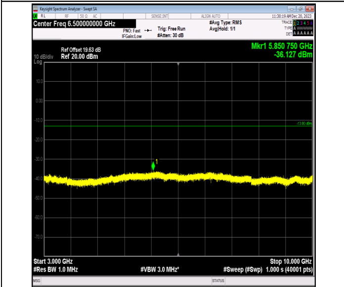
Band5_3MHz_QPSK_20525_1RB#0_3000~10000_3000~1000
