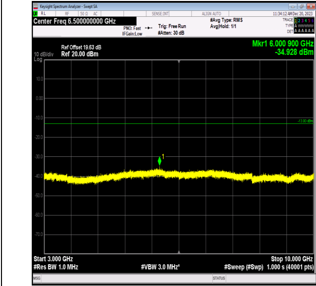
Band5_3MHz_16QAM_20635_1RB#0_3000~10000_3000~10000 000
