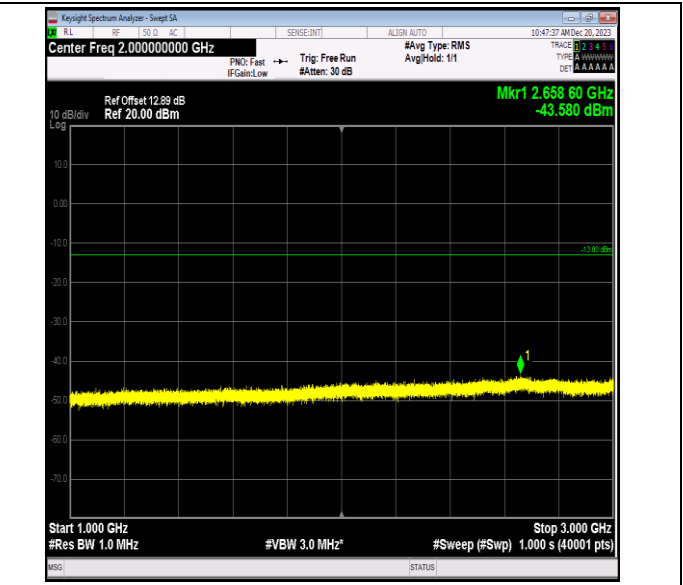
Band5_1.4MHz_64QAM_20407_1RB#0_1000~3000_1000~3000
