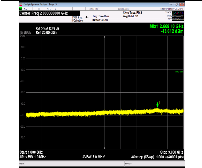
Band5_5MHz_16QAM_20425_1RB#0_1000~3000_1000~300
