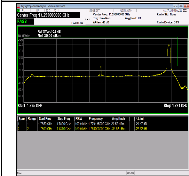
Band66_15MHz_QPSK_132597_1RB#74
