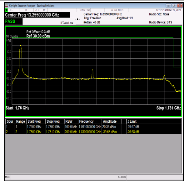
Band66_20MHz_64QAM_132572_1RB#0
