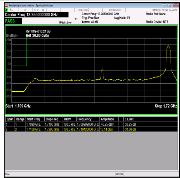
Band66_10MHz_64QAM_132022_1RB#49
