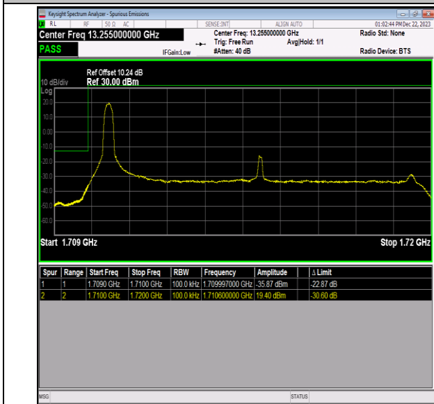
Band66_10MHz_16QAM_132022_1RB#0
