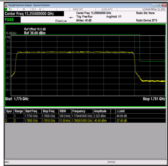
Band66_5MHz_16QAM_132647_25RB#0
