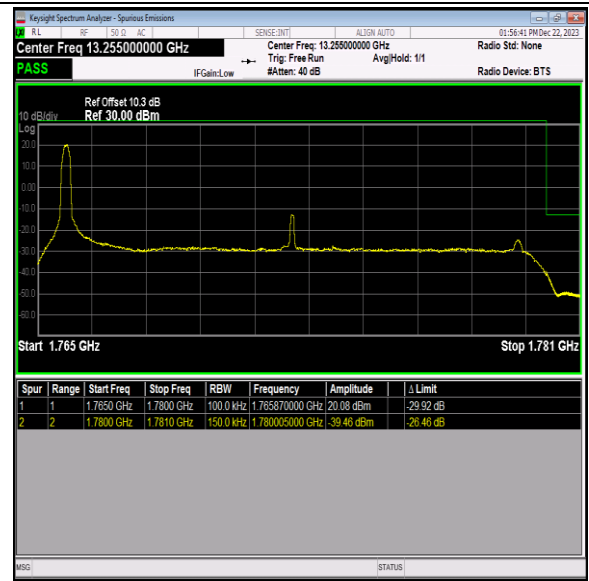
Band66_15MHz_QPSK_132597_1RB#0
