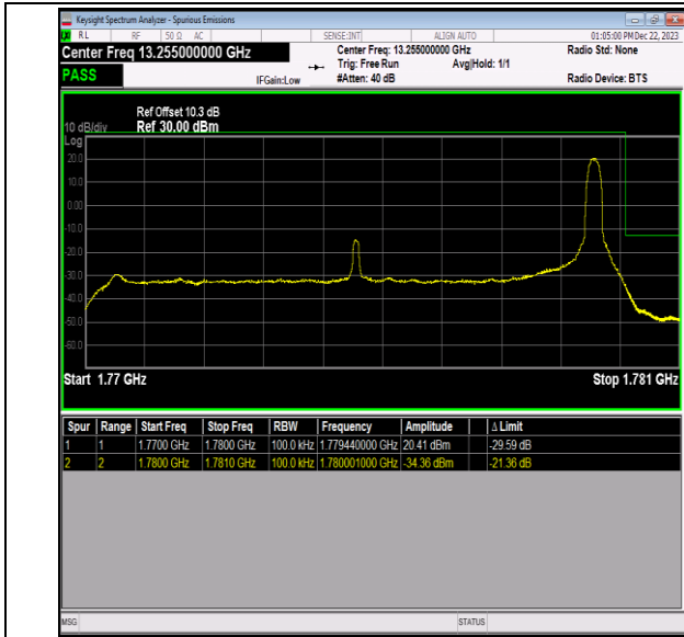
Band66_10MHz_QPSK_132622_1RB#49
