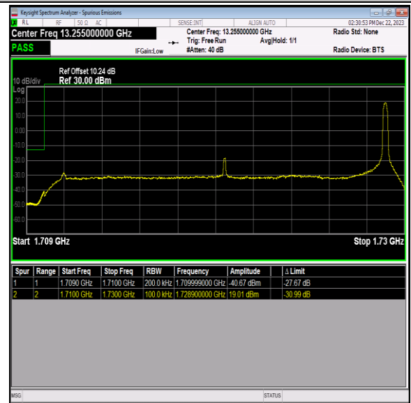
Band66_20MHz_16QAM_132072_1RB#99
