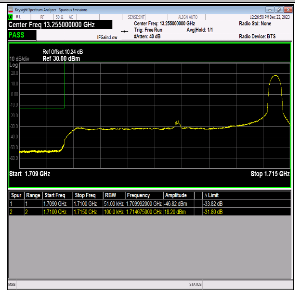
Band66_5MHz_64QAM_131997_1RB#24
