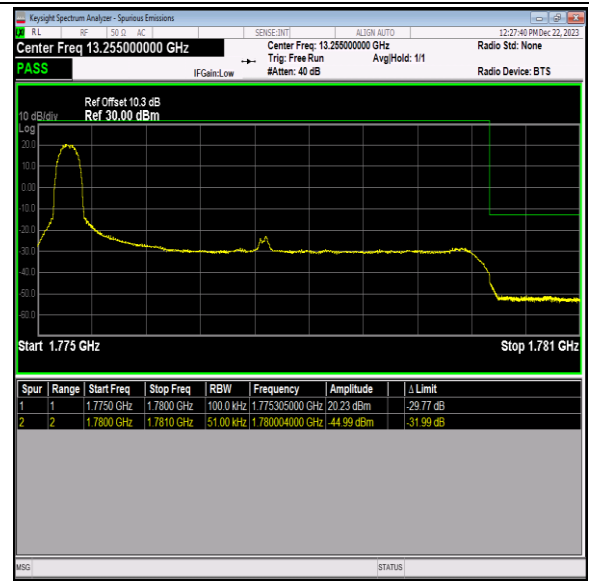
Band66_5MHz_QPSK_132647_1RB#0
