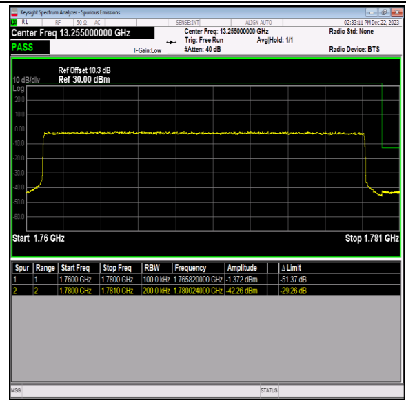
Band66_20MHz_QPSK_132572_100RB#0
