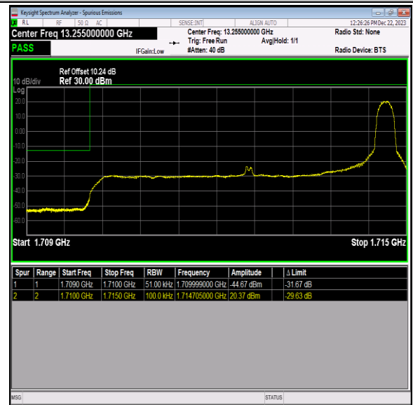
Band66_5MHz_QPSK_131997_1RB#24
