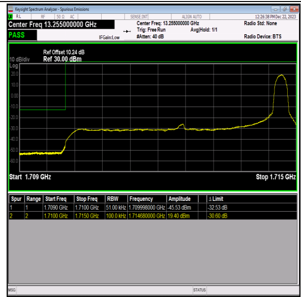
Band66_5MHz_16QAM_131997_1RB#24
