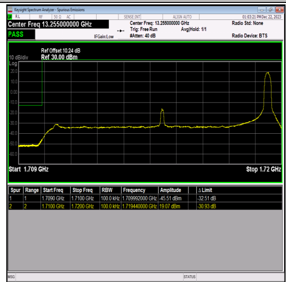
Band66_10MHz_16QAM_132022_1RB#49
