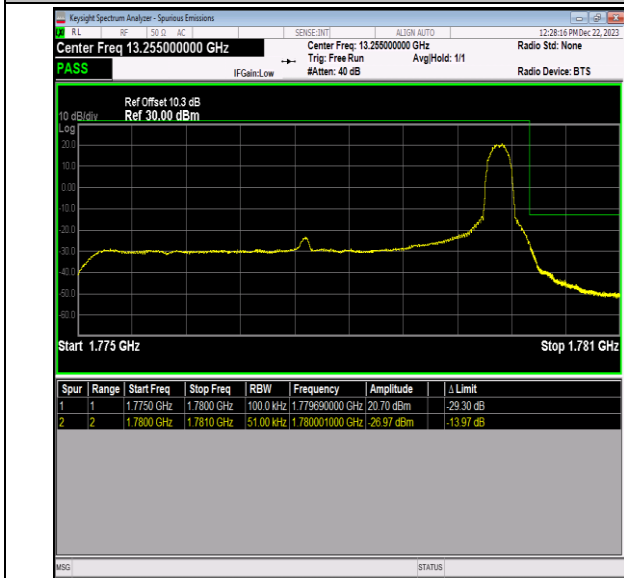
Band66_5MHz_QPSK_132647_1RB#24
