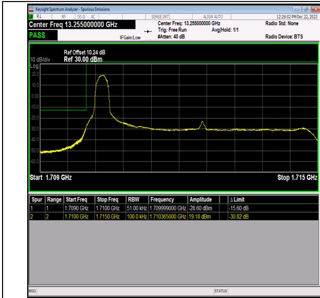
Band66_5MHz_16QAM_131997_1RB#0
