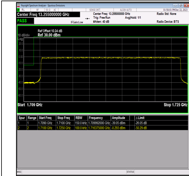
Band66_15MHz_QPSK_132047_75RB#0
