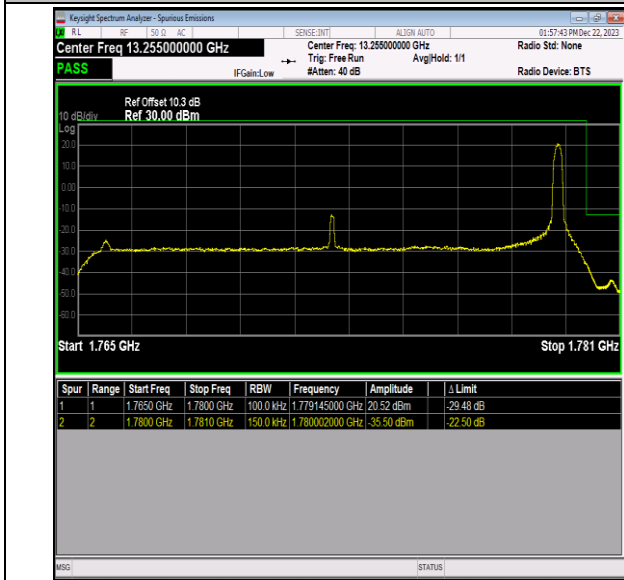
Band66_15MHz_64QAM_132597_1RB#74
