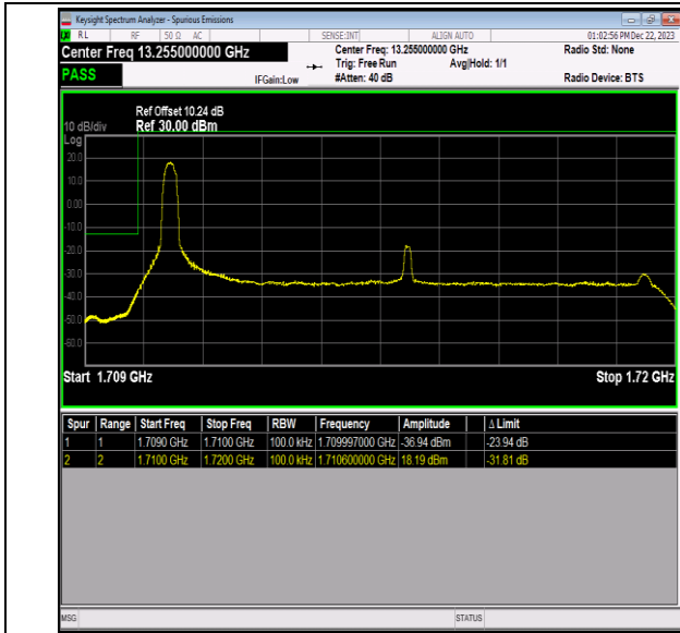
Band66_10MHz_64QAM_132022_1RB#0
