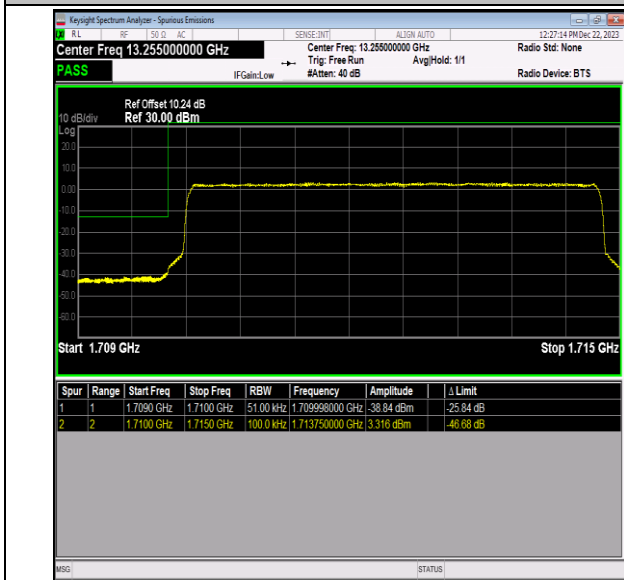
Band66_5MHz_16QAM_131997_25RB#0
