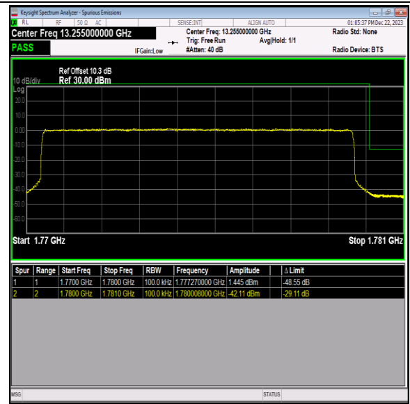
Band66_10MHz_QPSK_132622_50RB#0
