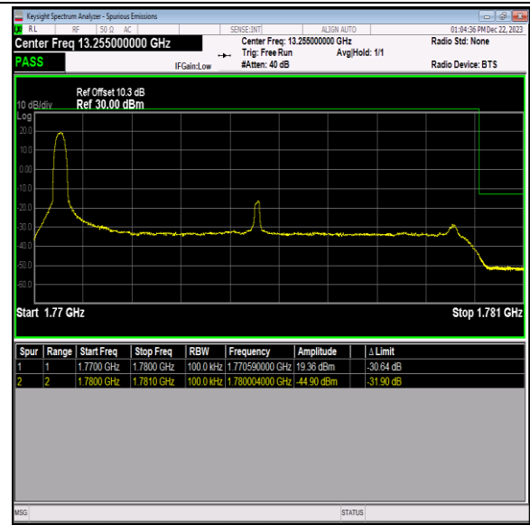
Band66_10MHz_16QAM_132622_1RB#0
