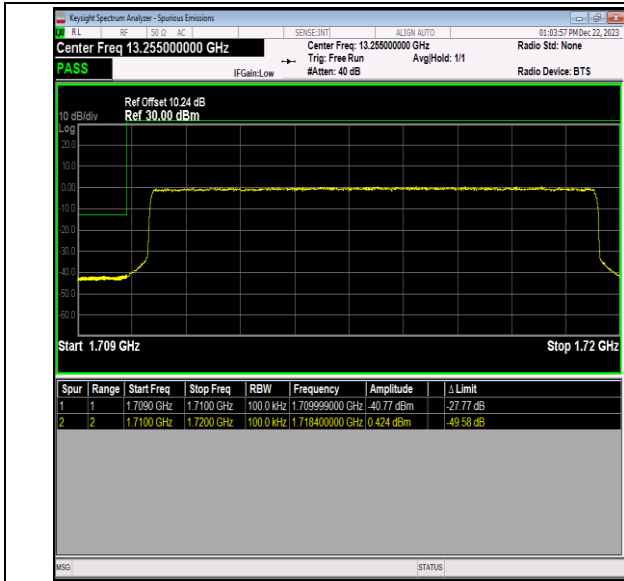
Band66_10MHz_16QAM_132022_50RB#0
