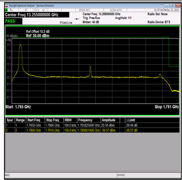
Band66_15MHz_64QAM_132597_1RB#0
