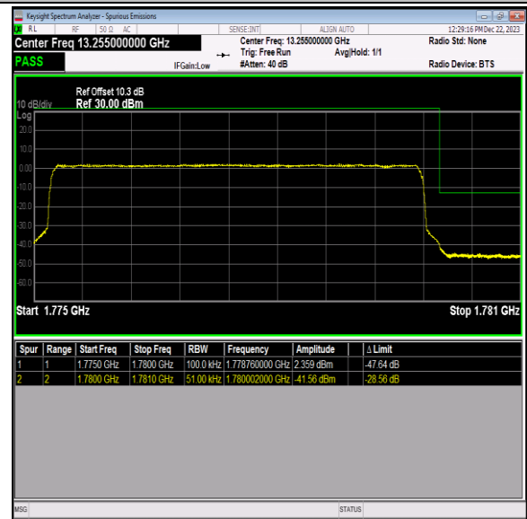
Band66_5MHz_64QAM_132647_25RB#0
