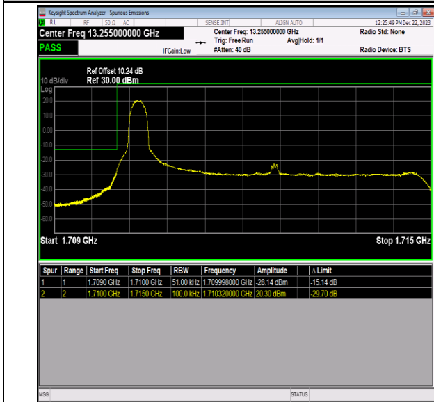
Band66_5MHz_QPSK_131997_1RB#0
