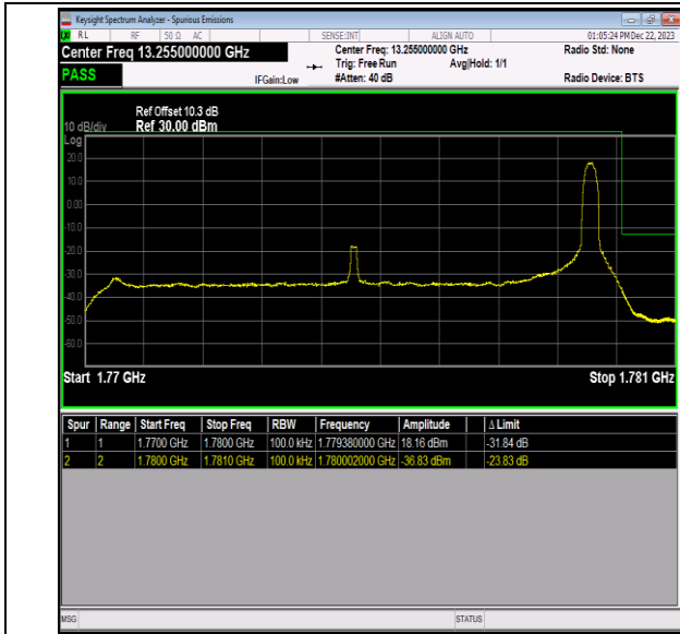
Band66_10MHz_64QAM_132622_1RB#49
