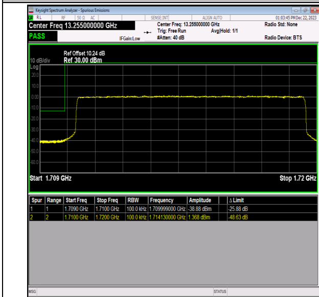
Band66_10MHz_QPSK_132022_50RB#0
