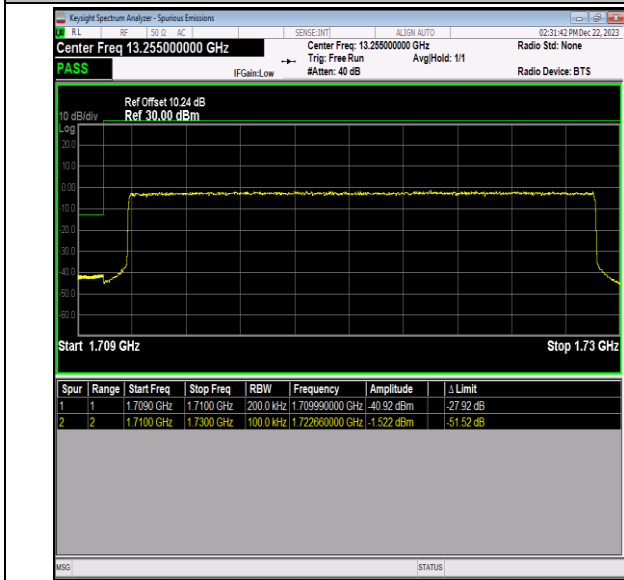
Band66_20MHz_64QAM_132072_100RB#0
