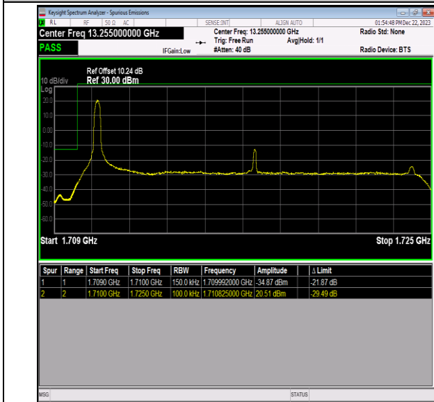
Band66_15MHz_QPSK_132047_1RB#0
