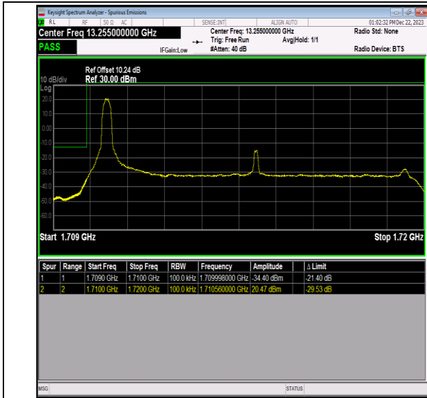
Band66_10MHz_QPSK_132022_1RB#0
