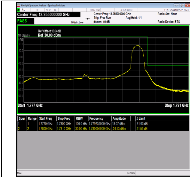
Band66_3MHz_64QAM_132657_1RB#14
