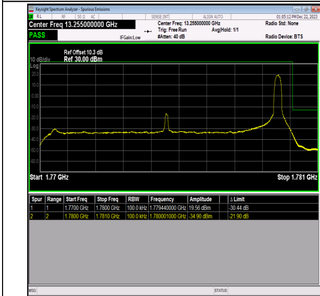
Band66_10MHz_16QAM_132622_1RB#49
