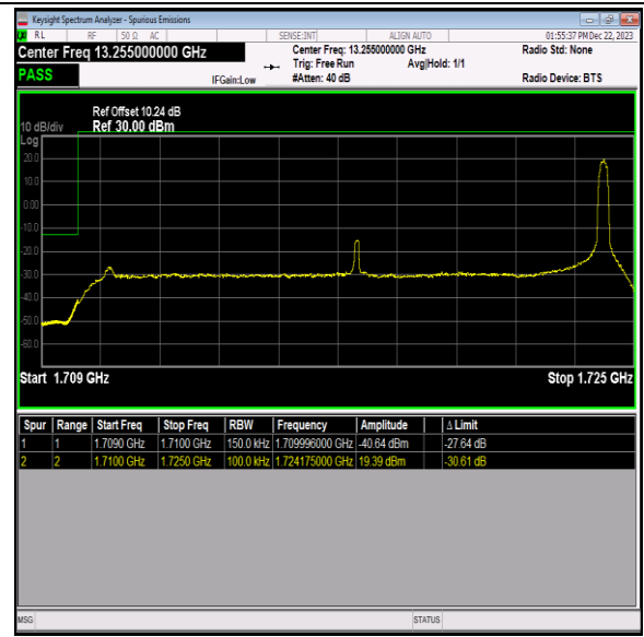
Band66_15MHz_16QAM_132047_1RB#74
