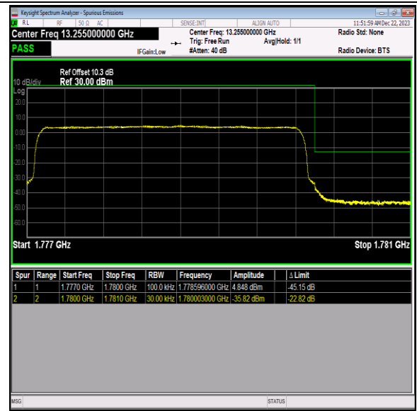
Band66_3MHz_64QAM_132657_15RB#0
