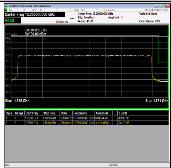
Band66_15MHz_QPSK_132597_75RB#0
