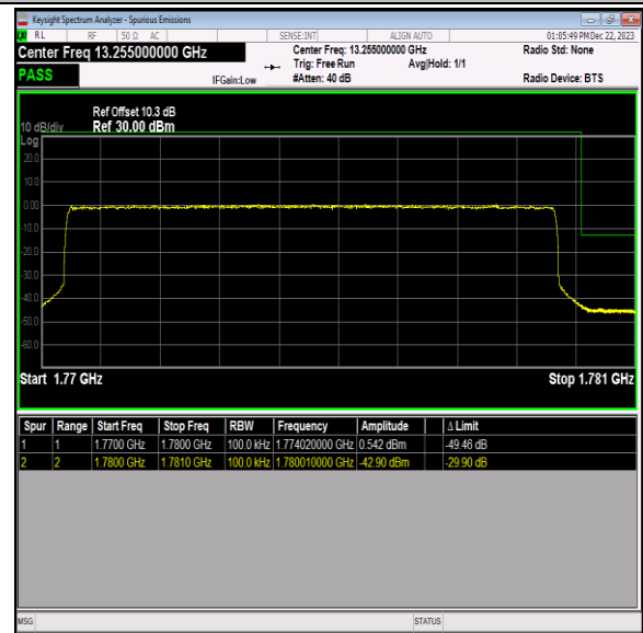
Band66_10MHz_16QAM_132622_50RB#0
