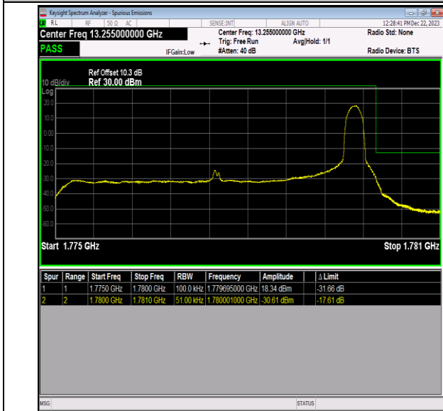
Band66_5MHz_64QAM_132647_1RB#24
