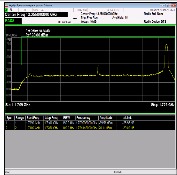
Band66_15MHz_QPSK_132047_1RB#74
