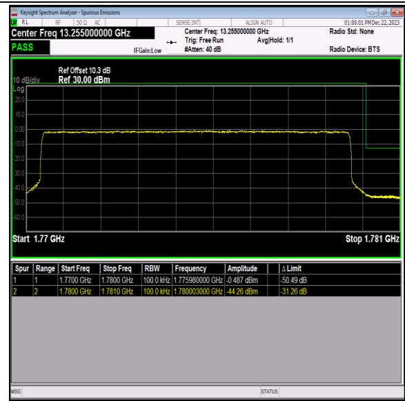
Band66_10MHz_64QAM_132622_50RB#0
