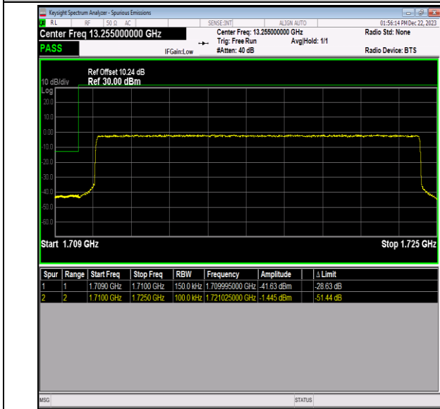
Band66_15MHz_16QAM_132047_75RB#0
