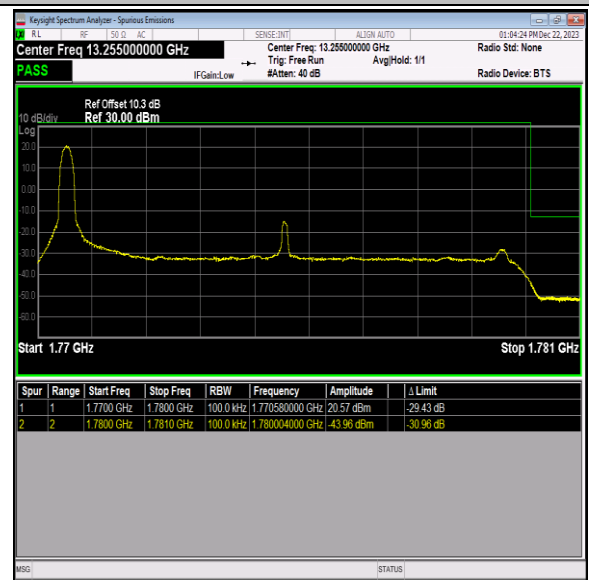
Band66_10MHz_QPSK_132622_1RB#0
