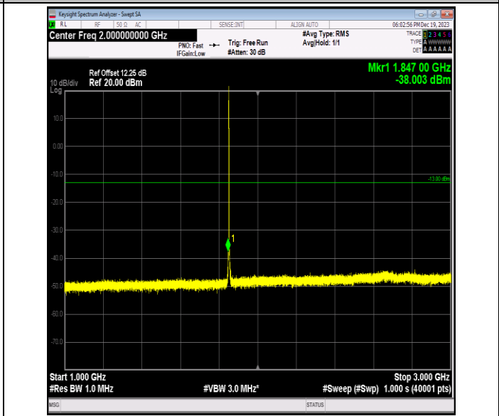
Band2_1.4MHz_QPSK_18607_1RB#0_1000~3000_1000~300 0
