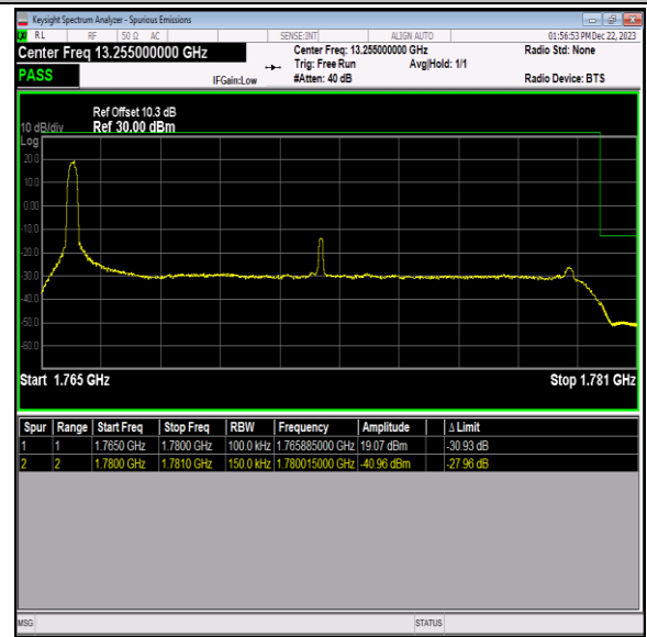
Band66_15MHz_16QAM_132597_1RB#0
