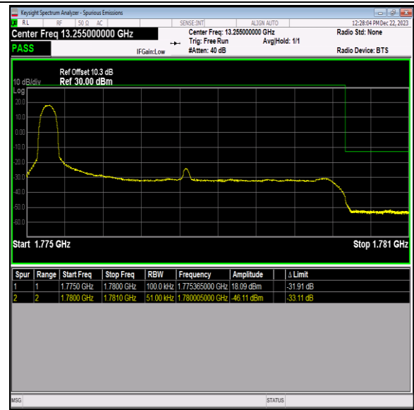
Band66_5MHz_64QAM_132647_1RB#0
