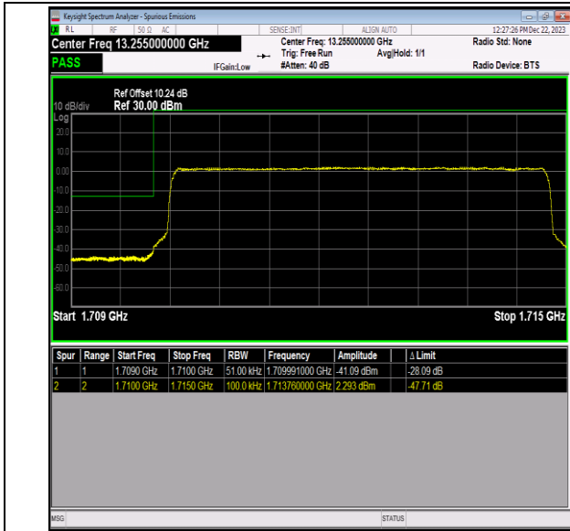
Band66_5MHz_64QAM_131997_25RB#0
