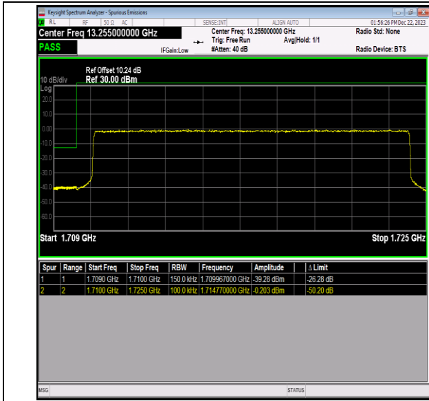
Band66_15MHz_64QAM_132047_75RB#0
