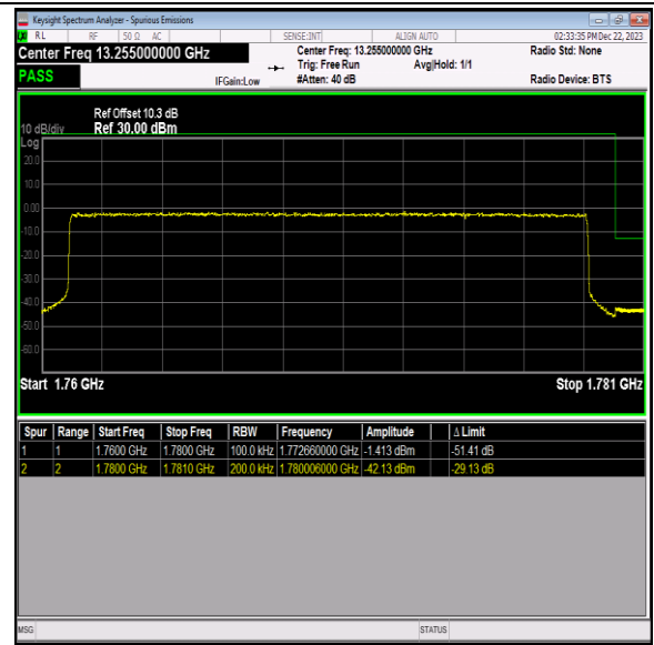
Band66_20MHz_64QAM_132572_100RB#0
