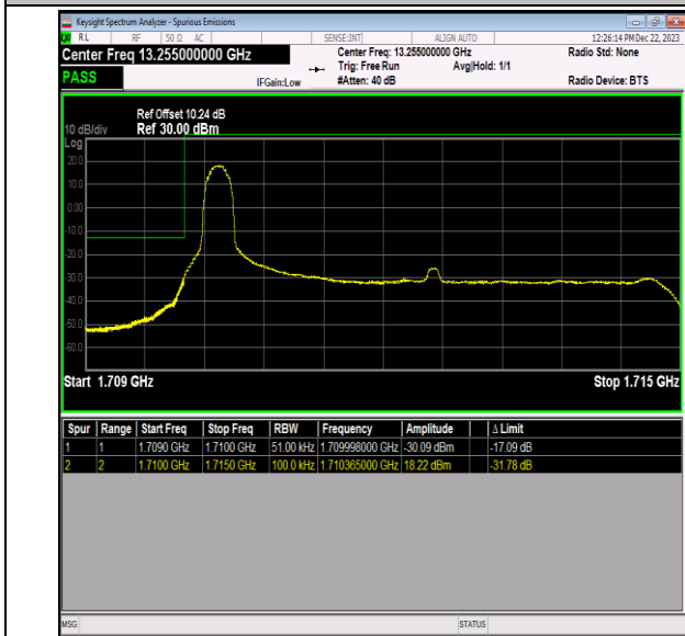
Band66_5MHz_64QAM_131997_1RB#0
