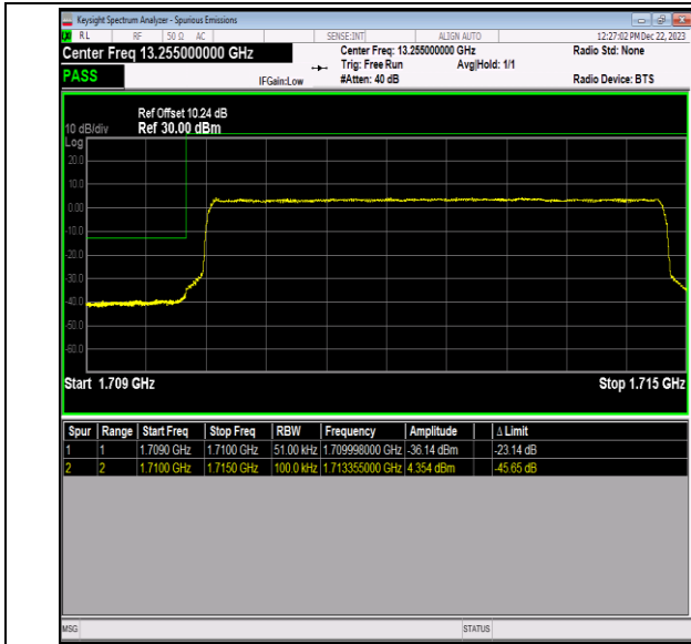
Band66_5MHz_QPSK_131997_25RB#0
