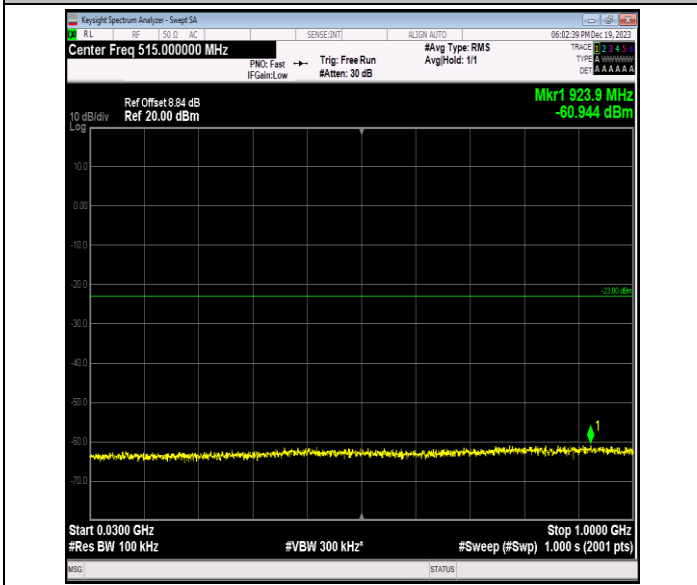
Band2_1.4MHz_QPSK_18607_1RB#0_30~1000_30~1000
