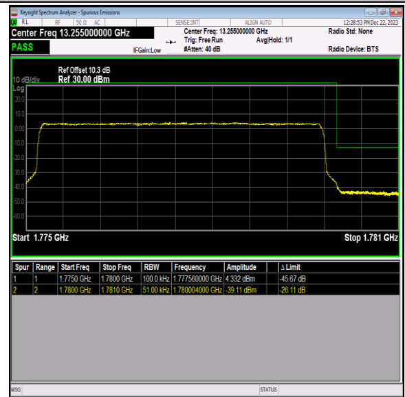
Band66_5MHz_QPSK_132647_25RB#0
