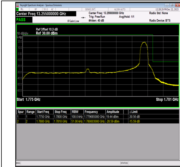
Band66_5MHz_16QAM_132647_1RB#24
