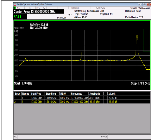
Band66_20MHz_64QAM_132572_1RB#99
