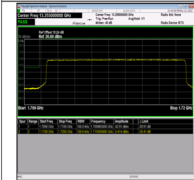
Band66_10MHz_64QAM_132022_50RB#0
