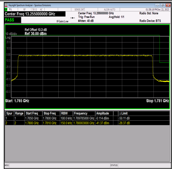
Band66_15MHz_64QAM_132597_75RB#0
