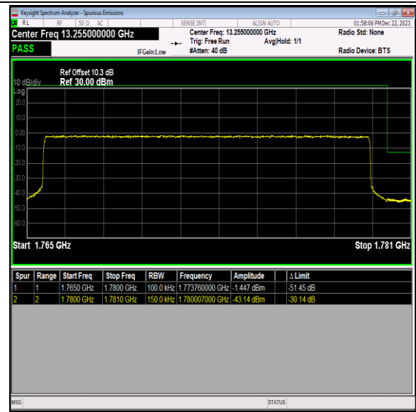
Band66_15MHz_16QAM_132597_75RB#0
