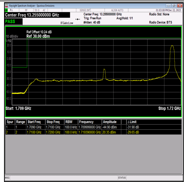
Band66_10MHz_QPSK_132022_1RB#49
