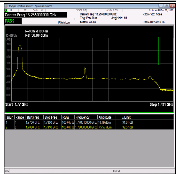
Band66_10MHz_64QAM_132622_1RB#0
