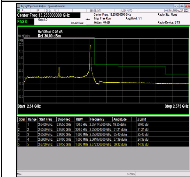
Band41_15MHz_QPSK_41165_1RB#74
