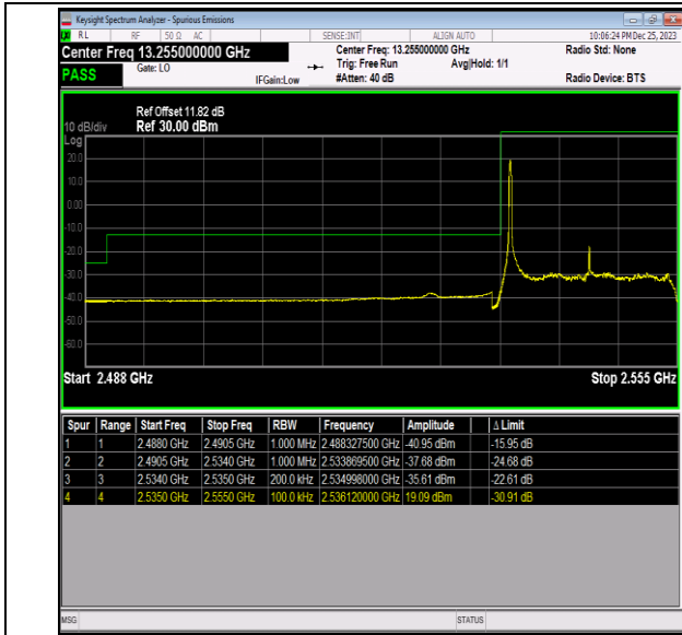
Band41_20MHz_64QAM_40140_1RB#0
