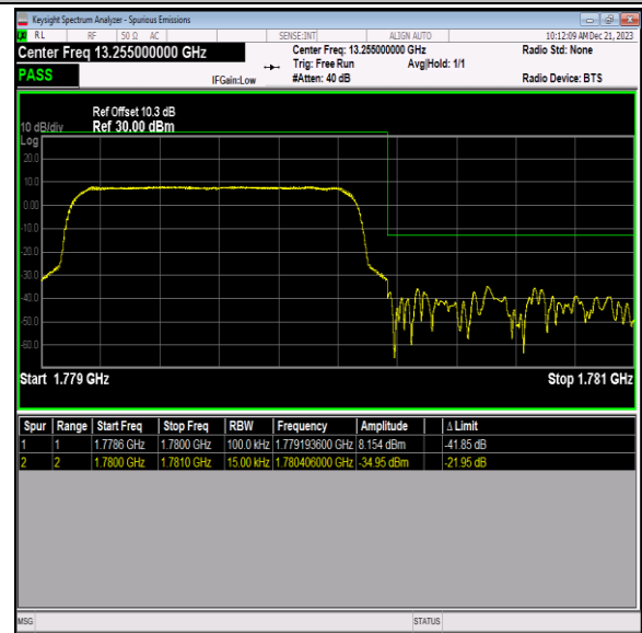
Band66_1.4MHz_64QAM_132665_6RB#0
