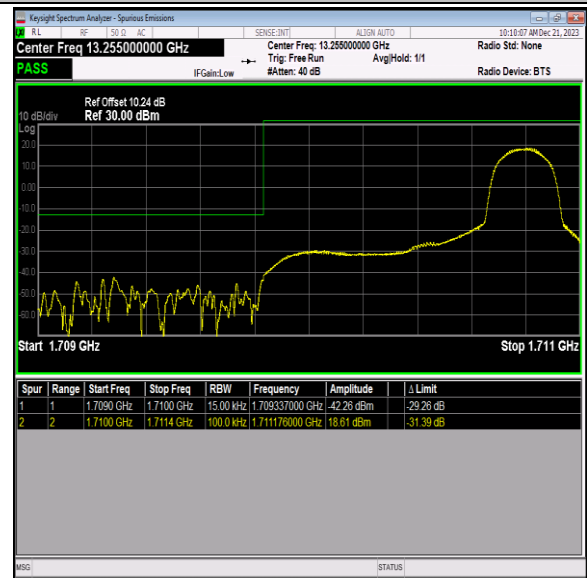
Band66_1.4MHz_64QAM_131979_1RB#5
