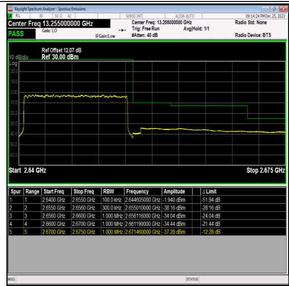
Band41_15MHz_16QAM_41165_75RB#0
