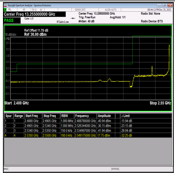
Band41_15MHz_16QAM_40115_1RB#74
