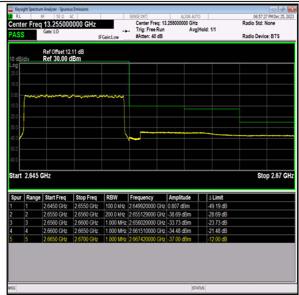
Band41_10MHz_64QAM_41190_50RB#0
