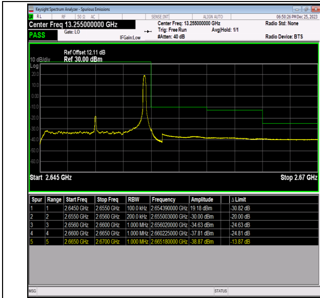
Band41_10MHz_64QAM_41190_1RB#49
