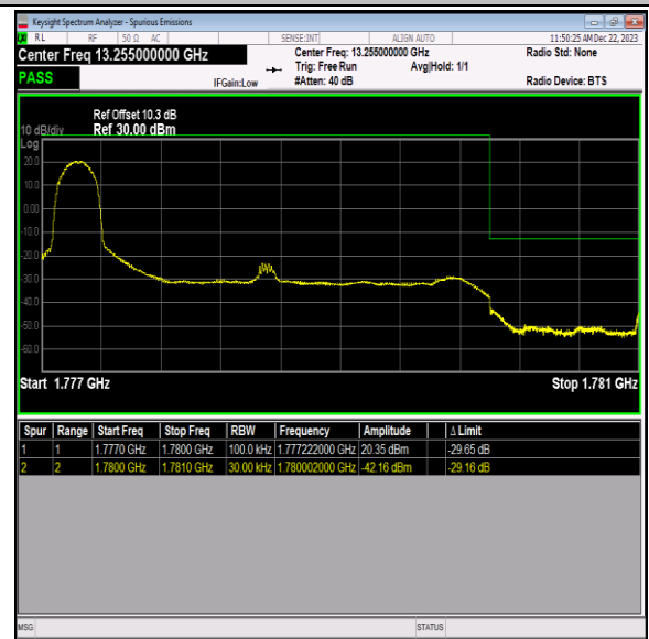
Band66_3MHz_QPSK_132657_1RB#0
