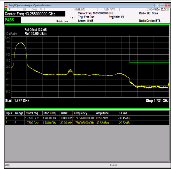
Band66_3MHz_16QAM_132657_1RB#0
