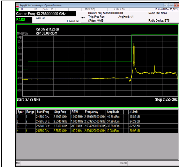
Band41_20MHz_QPSK_40140_1RB#0
