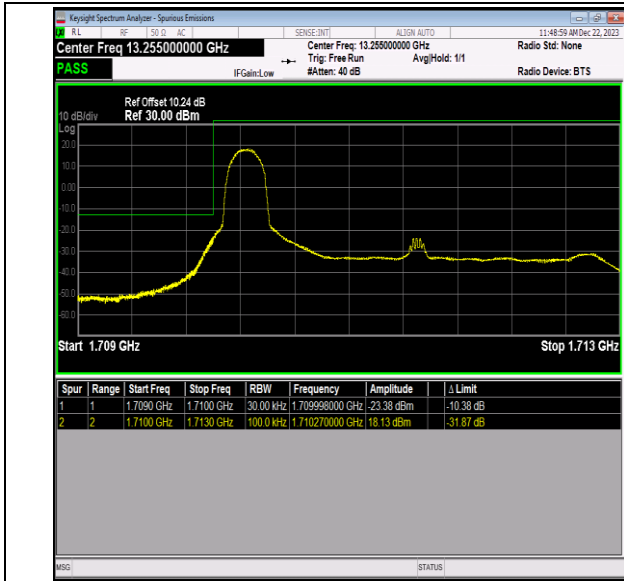
Band66_3MHz_64QAM_131987_1RB#0
