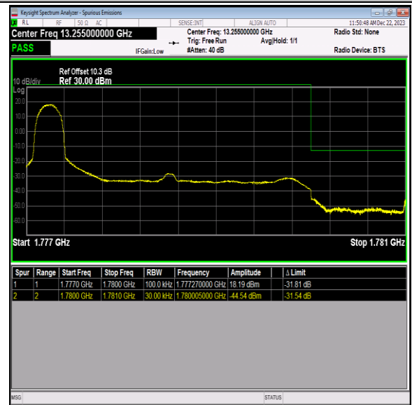
Band66_3MHz_64QAM_132657_1RB#0
