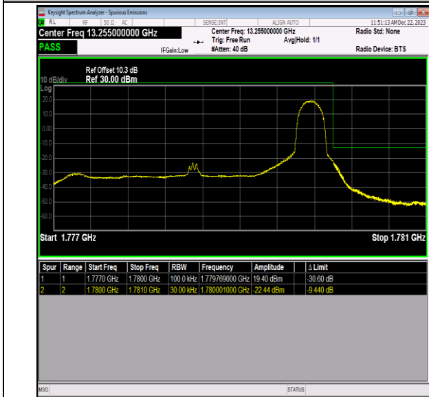
Band66_3MHz_16QAM_132657_1RB#14
