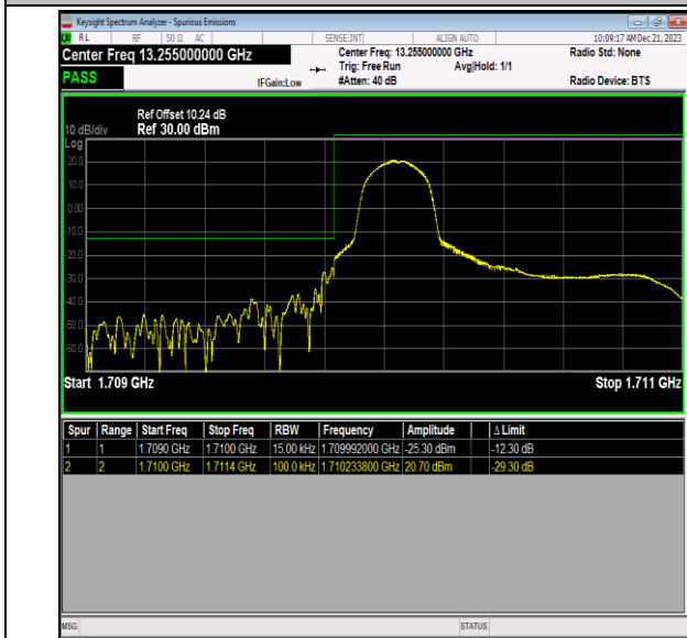
Band66_1.4MHz_QPSK_131979_1RB#0
