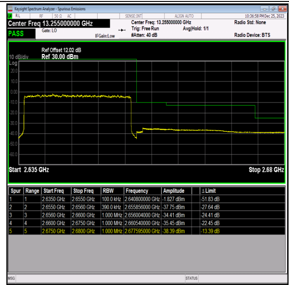
Band41_20MHz_QPSK_41140_100RB#0
