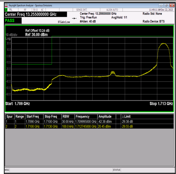
Band66_3MHz_QPSK_131987_1RB#14
