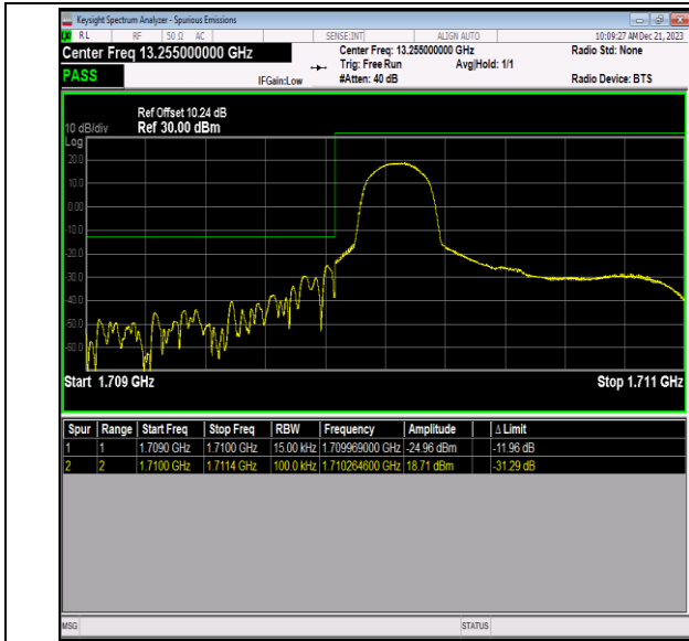
Band66_1.4MHz_16QAM_131979_1RB#0
