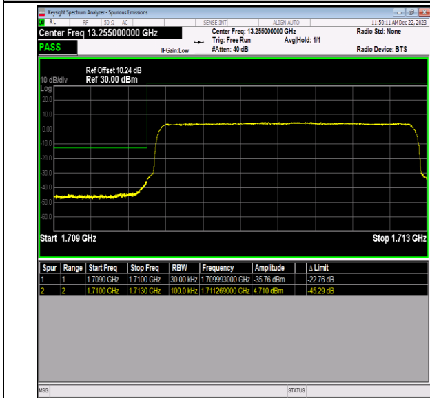
Band66_3MHz_64QAM_131987_15RB#0
