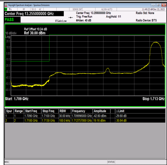
Band66_3MHz_16QAM_131987_1RB#14
