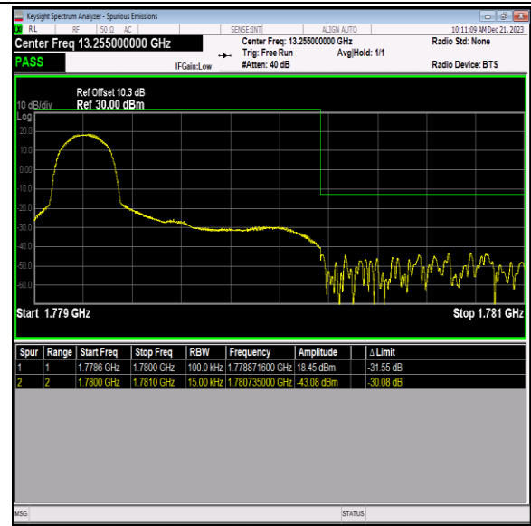
Band66_1.4MHz_64QAM_132665_1RB#0
