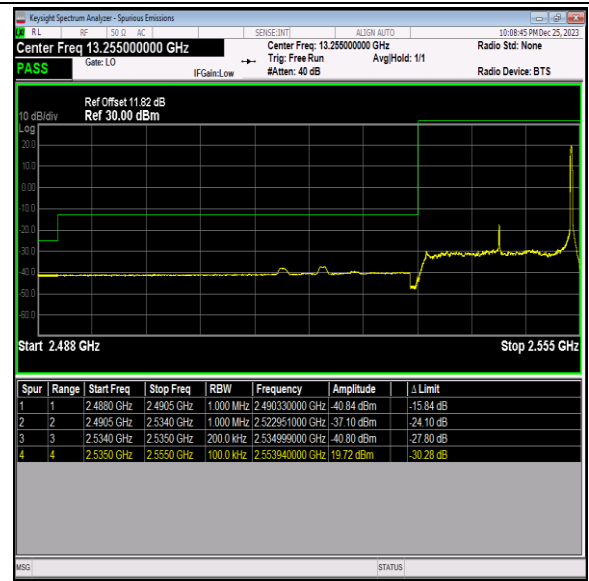
Band41_20MHz_QPSK_40140_1RB#99
