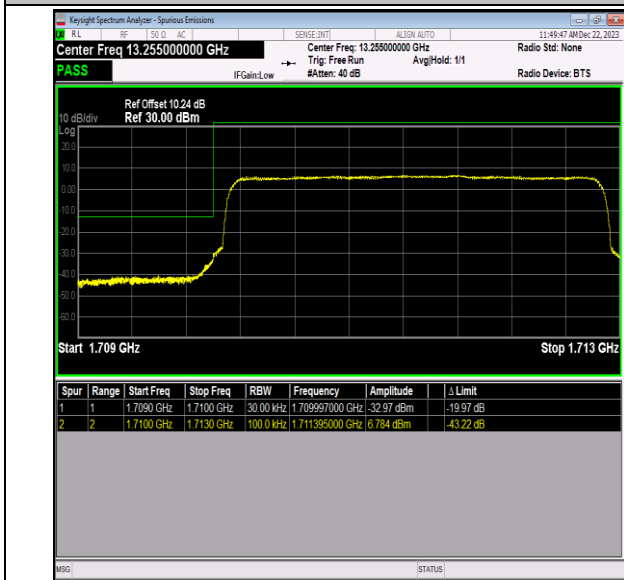
Band66_3MHz_QPSK_131987_15RB#0
