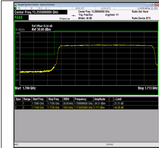
Band66_3MHz_16QAM_131987_15RB#0
