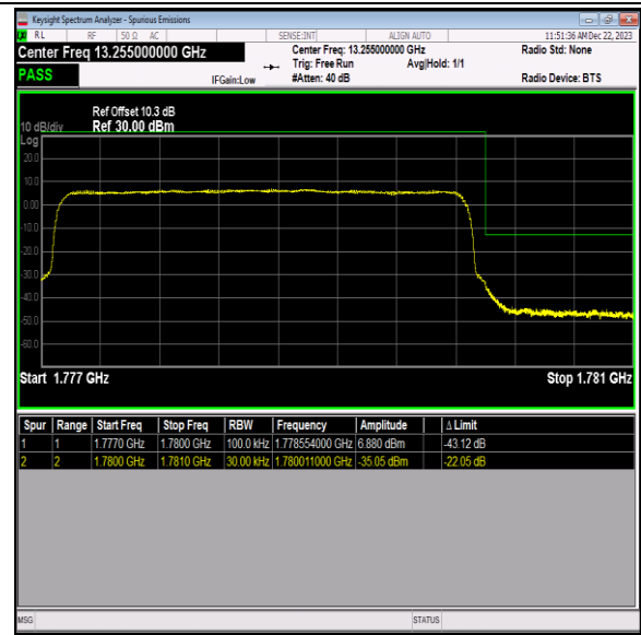
Band66_3MHz_QPSK_132657_15RB#0
