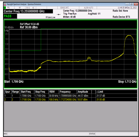
Band66_3MHz_64QAM_131987_1RB#14
