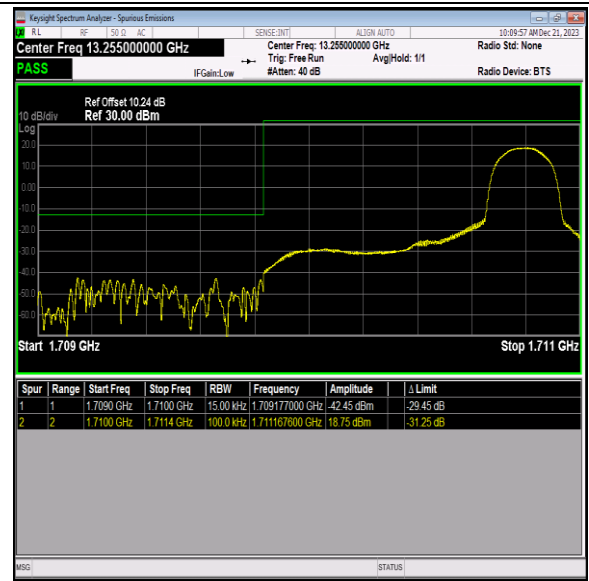
Band66_1.4MHz_16QAM_131979_1RB#5
