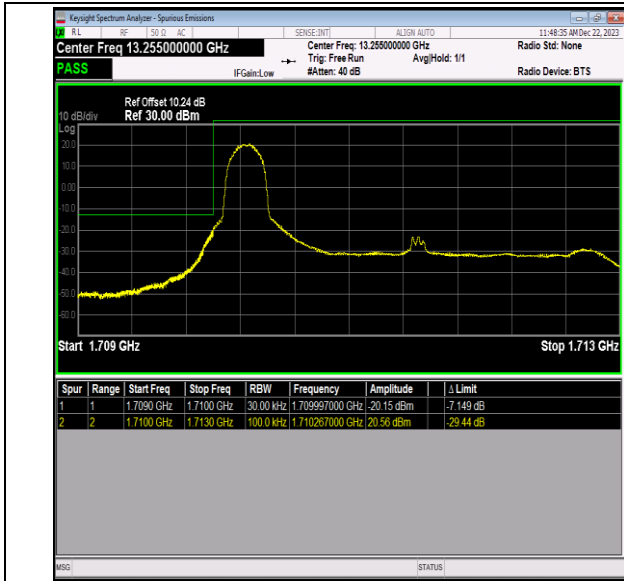
Band66_3MHz_QPSK_131987_1RB#0
