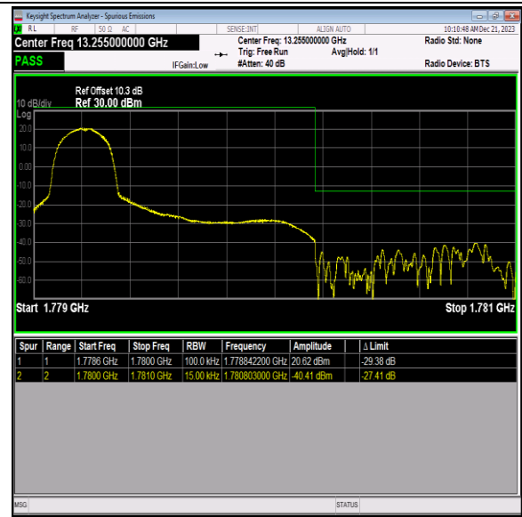
Band66_1.4MHz_QPSK_132665_1RB#0
