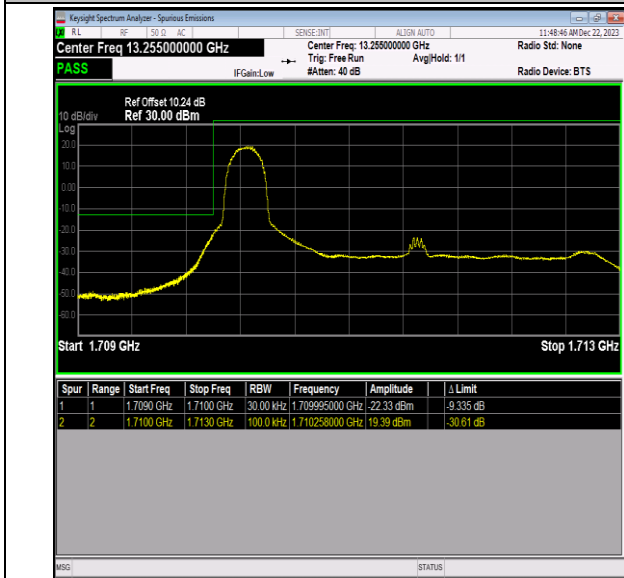
Band66_3MHz_16QAM_131987_1RB#0
