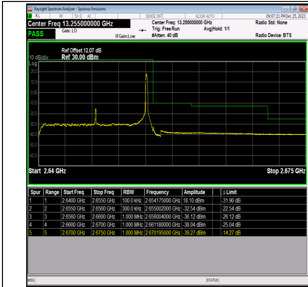
Band41_15MHz_16QAM_41165_1RB#74
