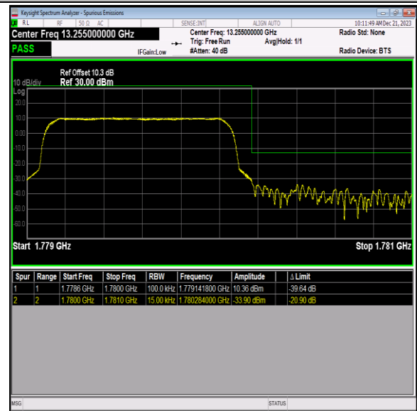
Band66_1.4MHz_QPSK_132665_6RB#0
