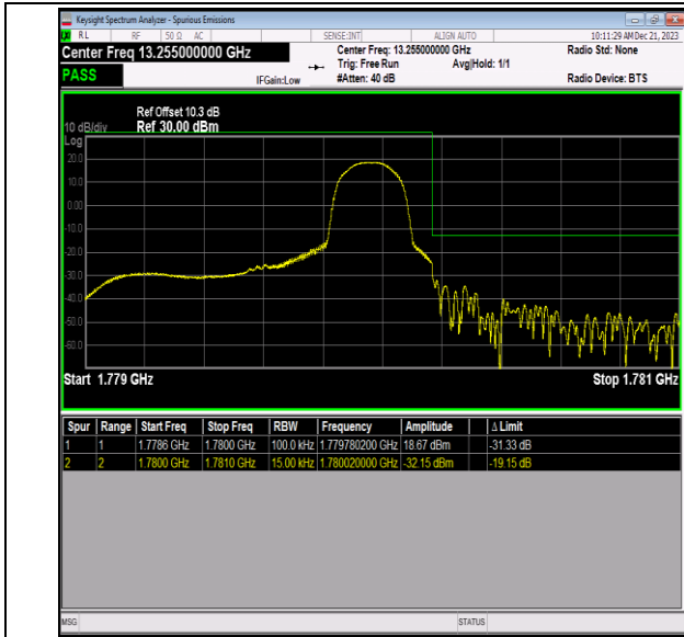
Band66_1.4MHz_16QAM_132665_1RB#5
