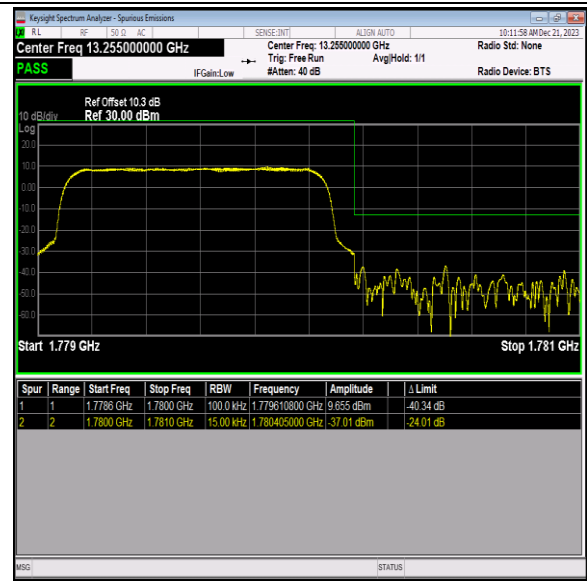
Band66_1.4MHz_16QAM_132665_6RB#0
