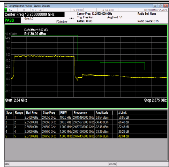
Band41_15MHz_QPSK_41165_75RB#0
