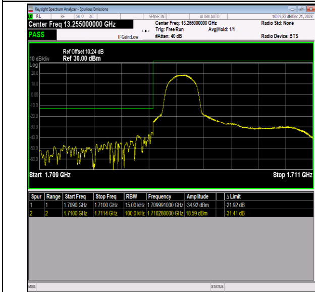
Band66_1.4MHz_64QAM_131979_1RB#0
