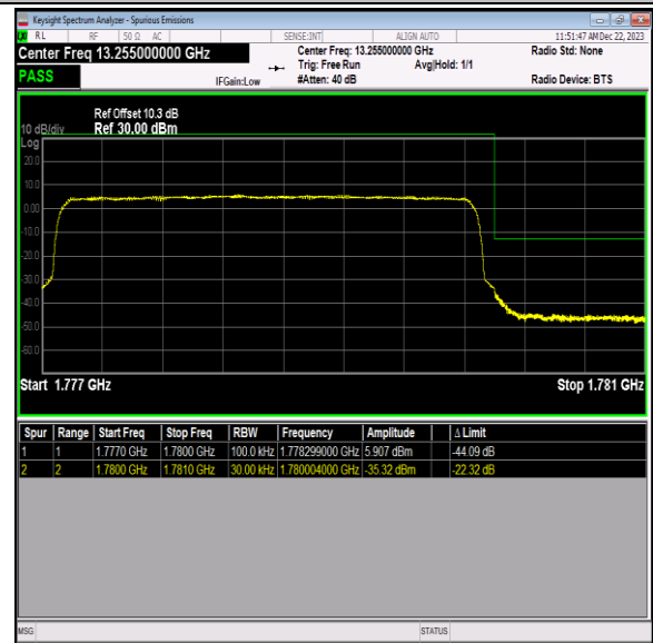
Band66_3MHz_16QAM_132657_15RB#0
