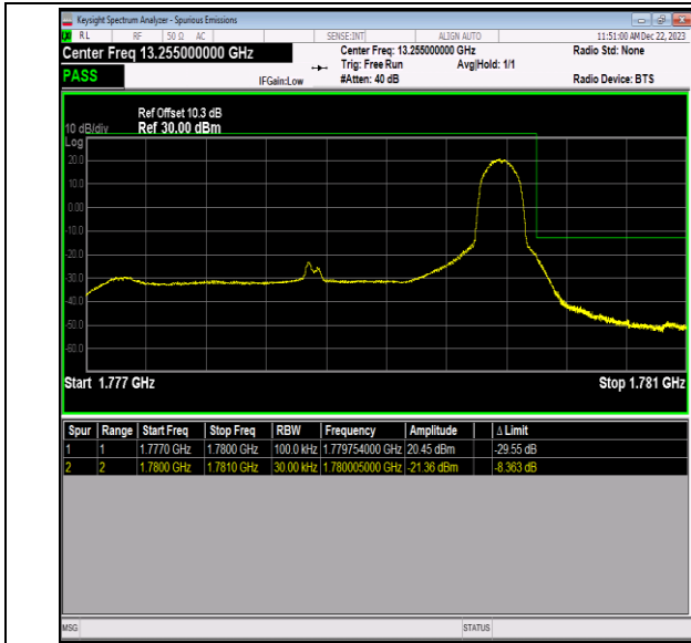
Band66_3MHz_QPSK_132657_1RB#14
