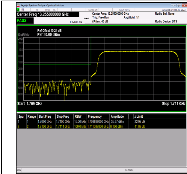
Band66_1.4MHz_64QAM_131979_6RB#0
