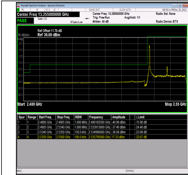
Band41_15MHz_16QAM_40115_1RB#0
