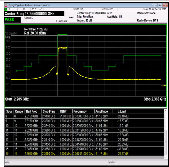
Band40_5MHz_64QAM_38775_25RB#0
