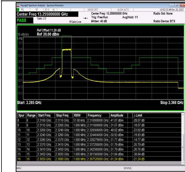
Band40_5MHz_64QAM_38725_25RB#0
