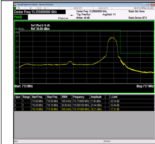
Band12_3MHz_64QAM_23165_1RB#14
