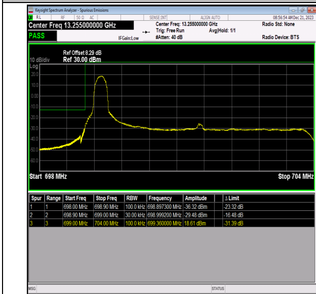
Band12_5MHz_16QAM_23035_1RB#0
