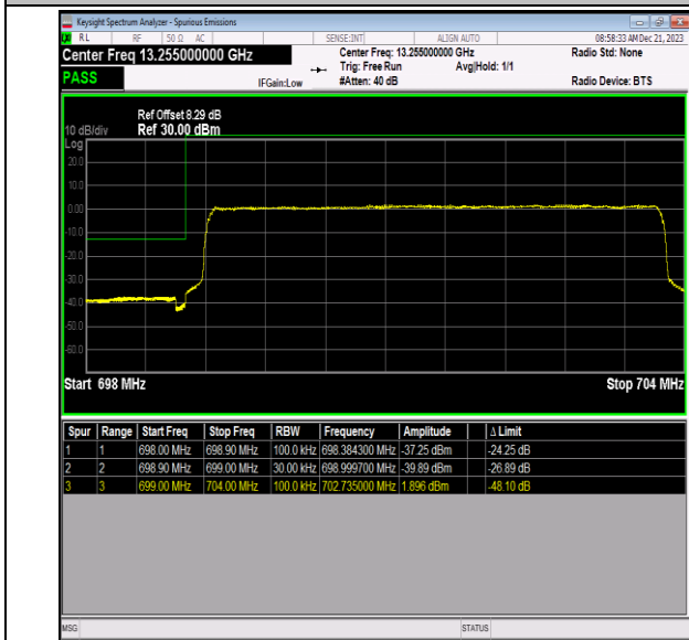
Band12_5MHz_64QAM_23035_25RB#0
