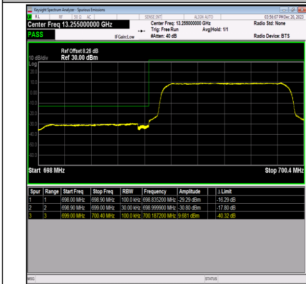
Band12_1.4MHz_QPSK_23017_6RB#0
