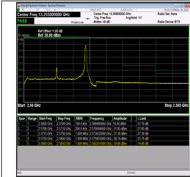
Band7_10MHz_16QAM_21400_1RB#49
