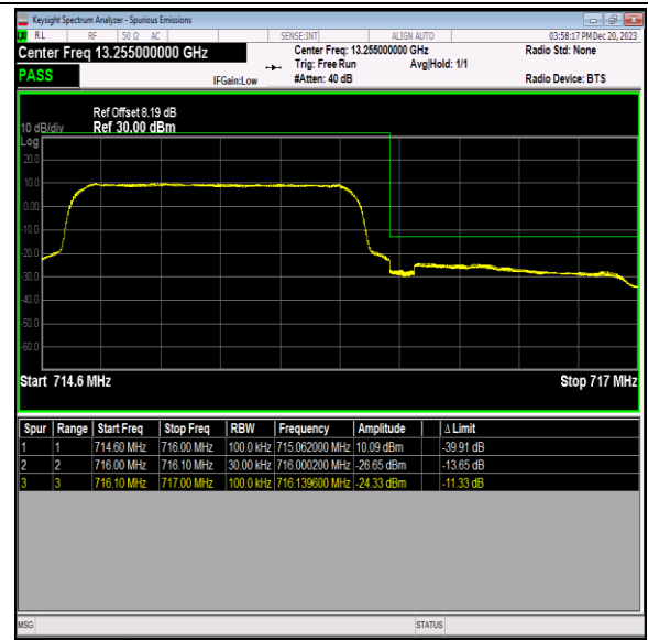
Band12_1.4MHz_QPSK_23173_6RB#0
