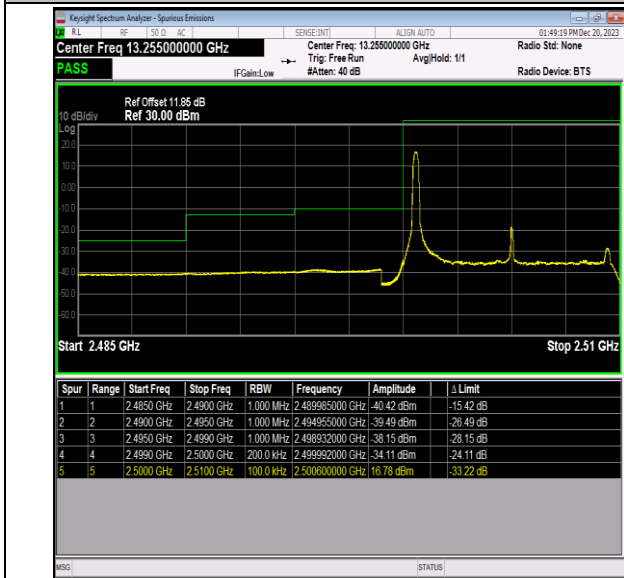
Band7_10MHz_64QAM_20800_1RB#0
