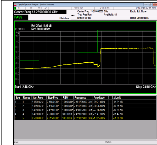
Band7_15MHz_QPSK_20825_75RB#0
