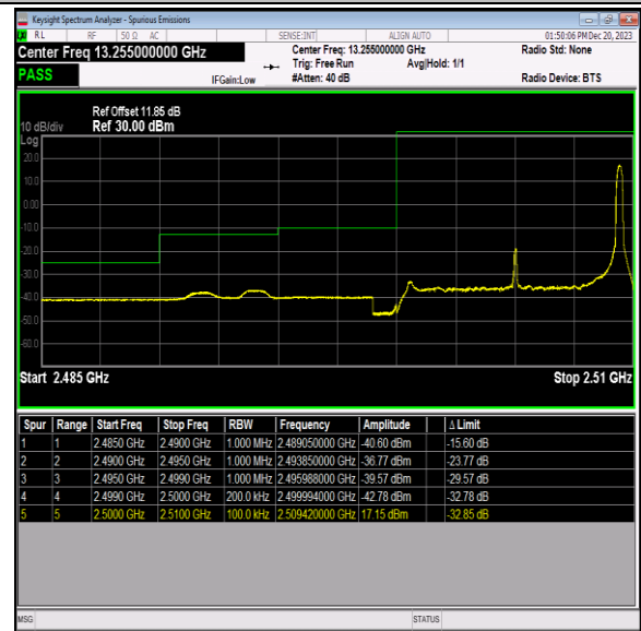
Band7_10MHz_64QAM_20800_1RB#49
