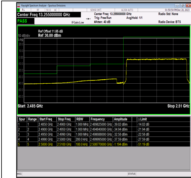
Band7_10MHz_64QAM_20800_50RB#0
