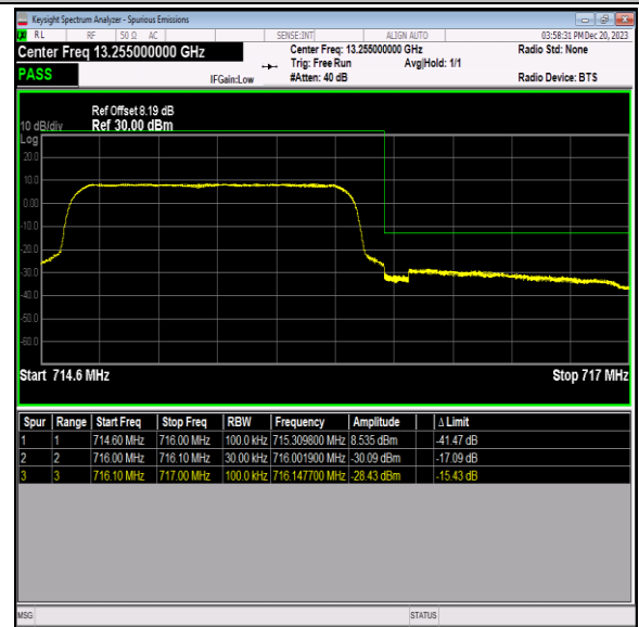
Band12_1.4MHz_16QAM_23173_6RB#0
