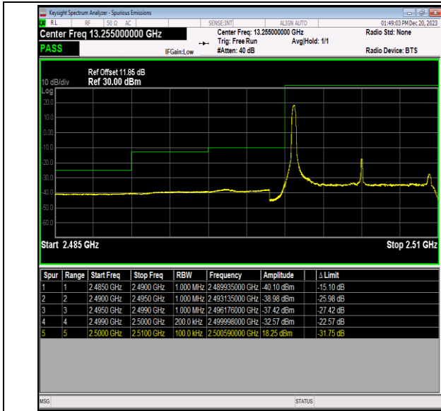
Band7_10MHz_16QAM_20800_1RB#0
