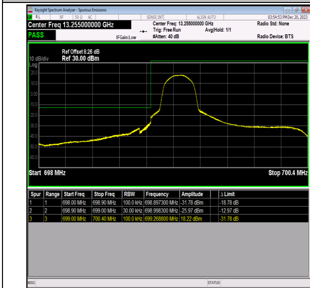
Band12_1.4MHz_16QAM_23017_1RB#0
