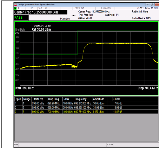
Band12_1.4MHz_16QAM_23017_6RB#0
