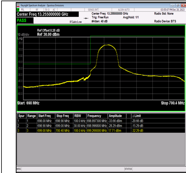
Band12_1.4MHz_64QAM_23017_1RB#0
