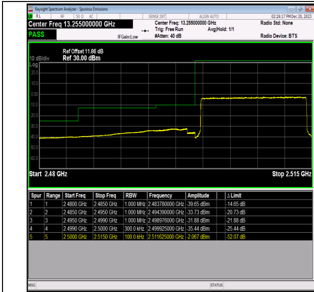
Band7_15MHz_16QAM_20825_75RB#0
