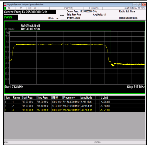
Band12_3MHz_QPSK_23165_15RB#0
