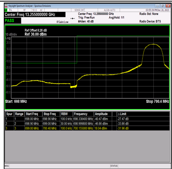
Band12_1.4MHz_16QAM_23017_1RB#5
