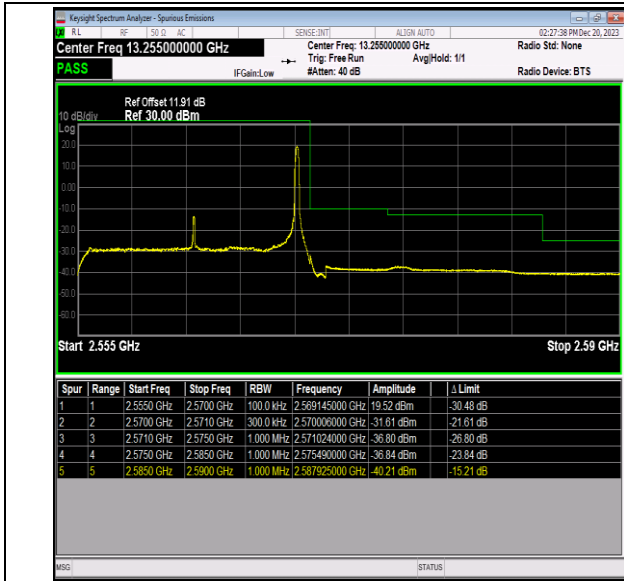
Band7_15MHz_QPSK_21375_1RB#74
