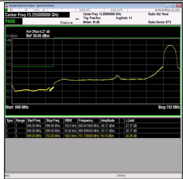
Band12_3MHz_QPSK_23025_1RB#14
