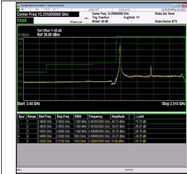
Band7_15MHz_64QAM_20825_1RB#0
