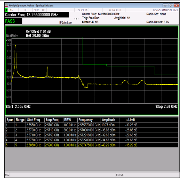
Band7_15MHz_QPSK_21375_1RB#0
