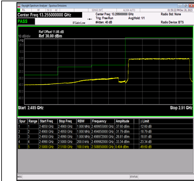
Band7_10MHz_QPSK_20800_50RB#0
