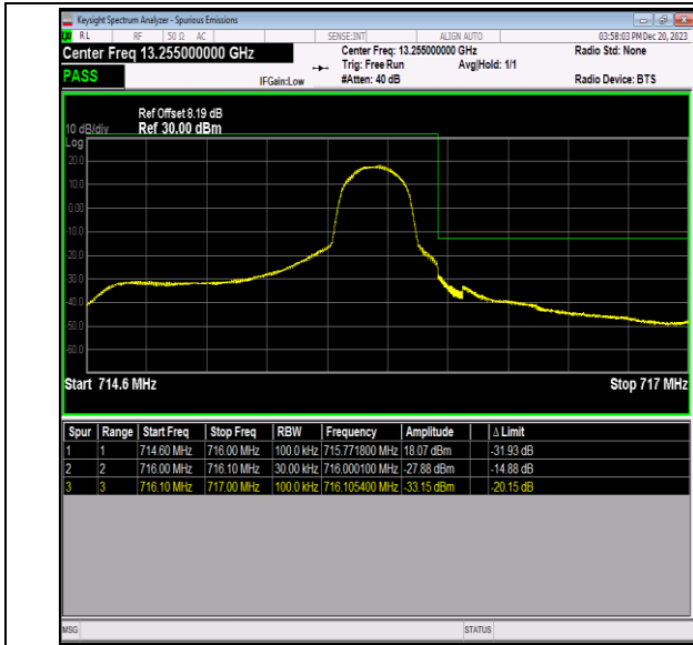
Band12_1.4MHz_64QAM_23173_1RB#5
