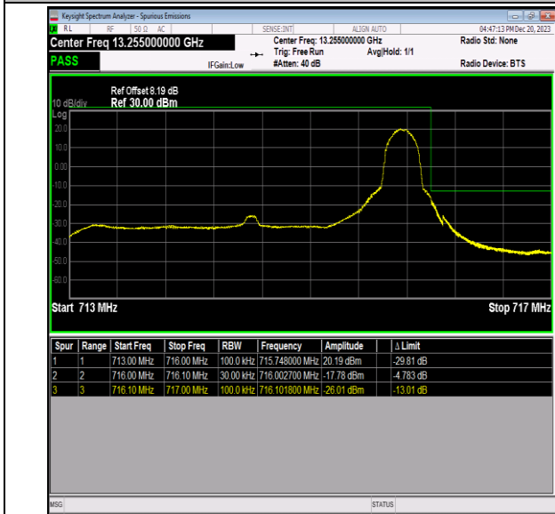
Band12_3MHz_QPSK_23165_1RB#14
