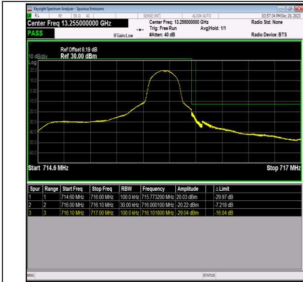
Band12_1.4MHz_QPSK_23173_1RB#5
