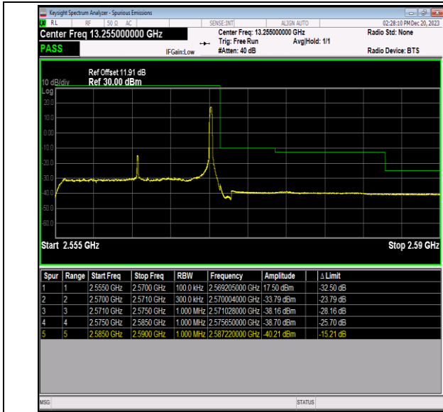
Band7_15MHz_64QAM_21375_1RB#74
