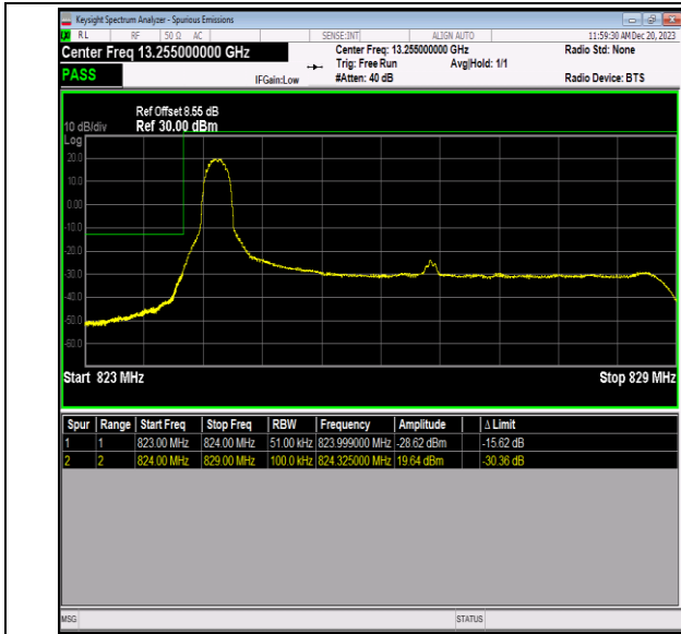
Band5_5MHz_QPSK_20425_1RB#0
