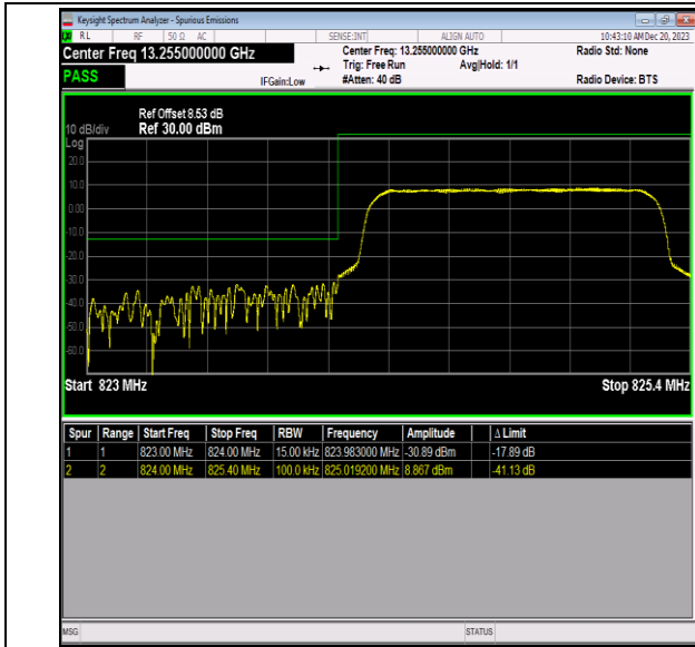
Band5_1.4MHz_16QAM_20407_6RB#0
