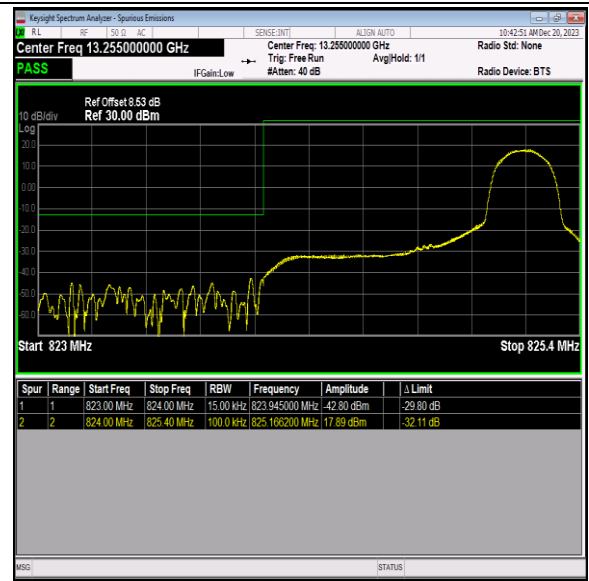
Band5_1.4MHz_64QAM_20407_1RB#5
