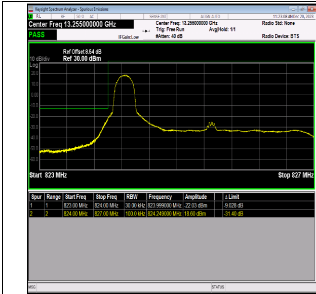
Band5_3MHz_16QAM_20415_1RB#0
