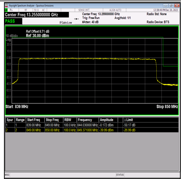
Band5_10MHz_16QAM_20600_50RB#0
