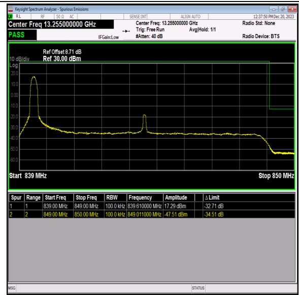
Band5_10MHz_64QAM_20600_1RB#0
