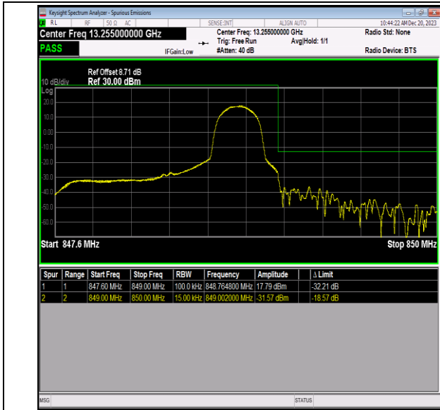
Band5_1.4MHz_64QAM_20643_1RB#5
