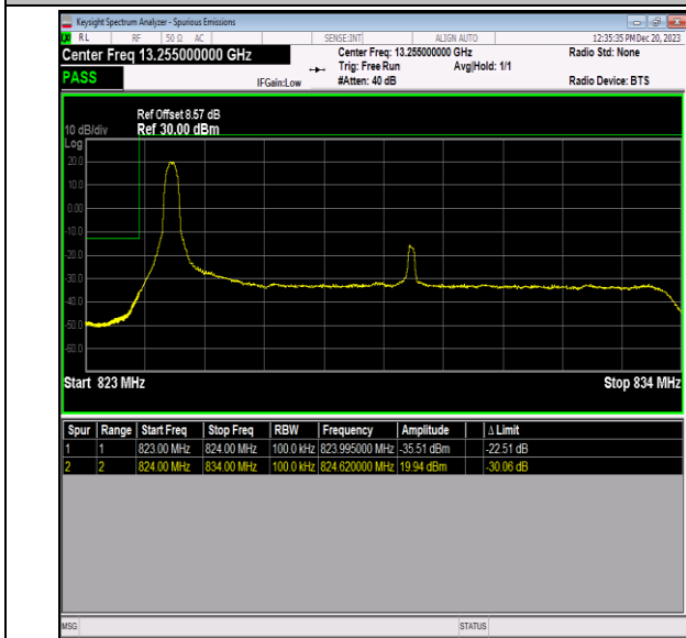
Band5_10MHz_QPSK_20450_1RB#0
