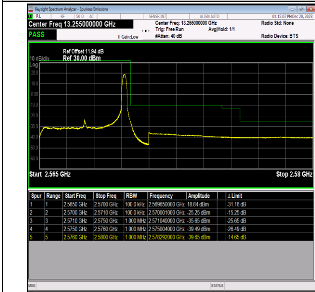
Band7_5MHz_16QAM_21425_1RB#24
