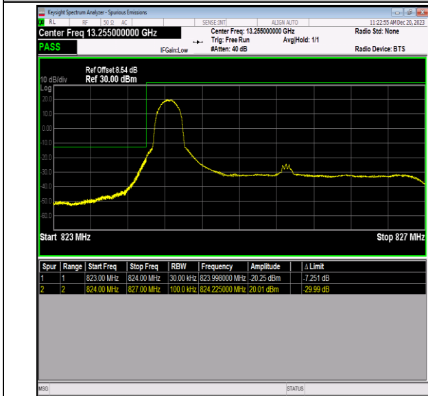
Band5_3MHz_QPSK_20415_1RB#0
