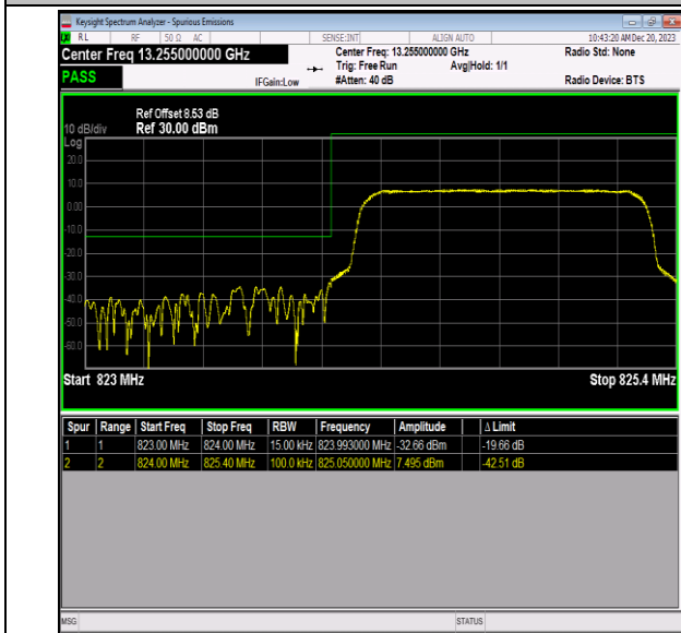
Band5_1.4MHz_64QAM_20407_6RB#0
