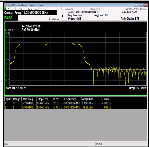
Band5_1.4MHz_16QAM_20643_6RB#0
