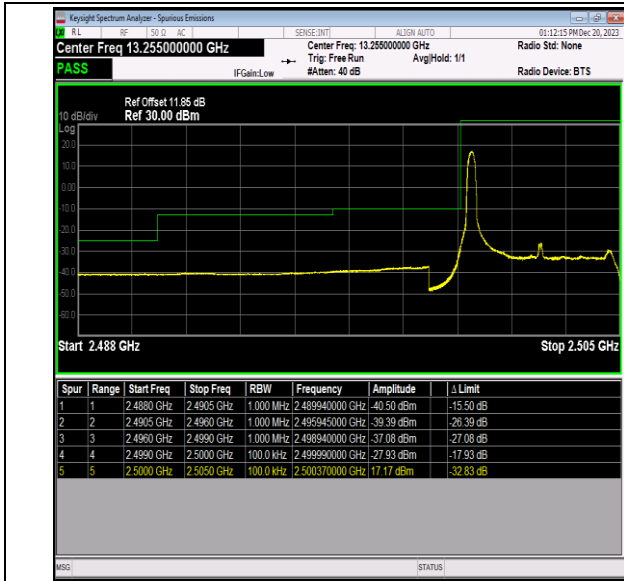
Band7_5MHz_64QAM_20775_1RB#0
