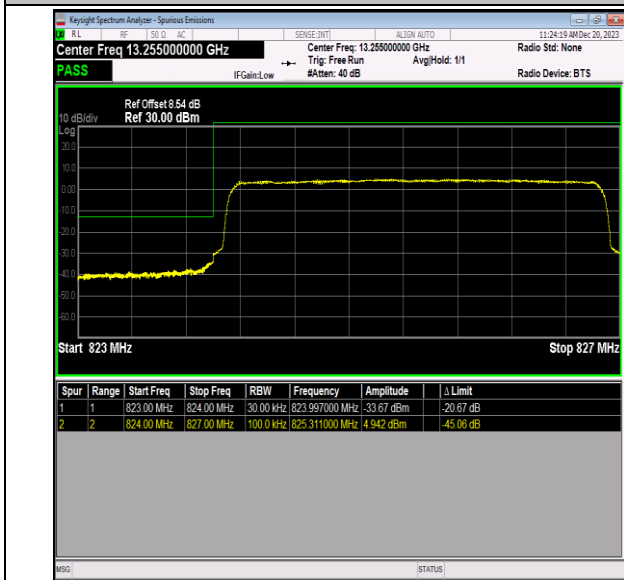
Band5_3MHz_16QAM_20415_15RB#0
