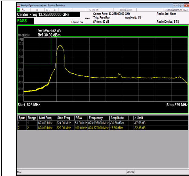
Band5_5MHz_64QAM_20425_1RB#0
