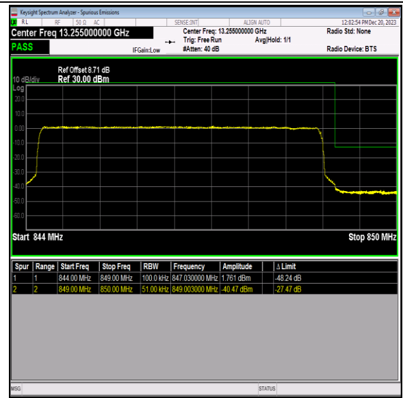
Band5_5MHz_64QAM_20625_25RB#0
