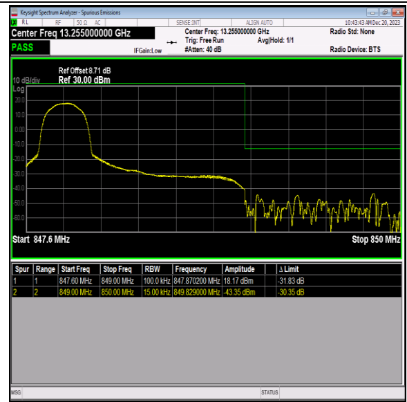
Band5_1.4MHz_16QAM_20643_1RB#0
