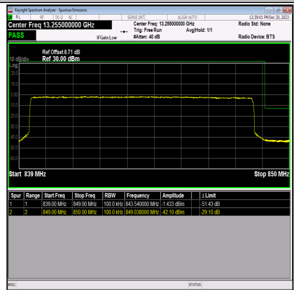
Band5_10MHz_64QAM_20600_50RB#0
