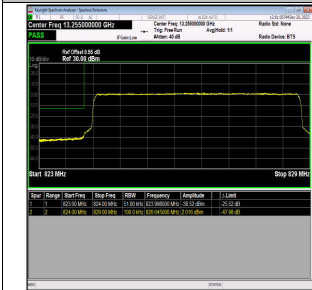
Band5_5MHz_64QAM_20425_25RB#0
