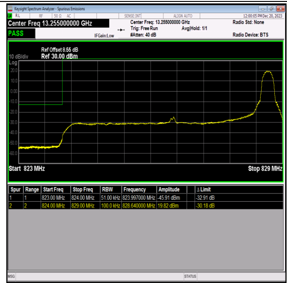
Band5_5MHz_QPSK_20425_1RB#24
