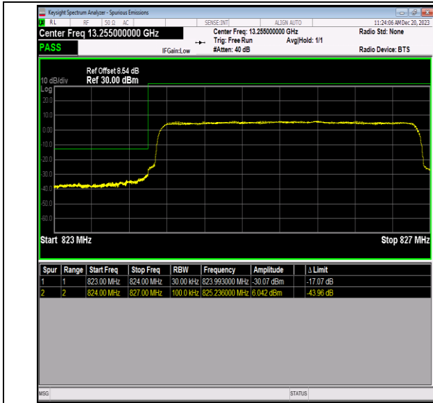
Band5_3MHz_QPSK_20415_15RB#0
