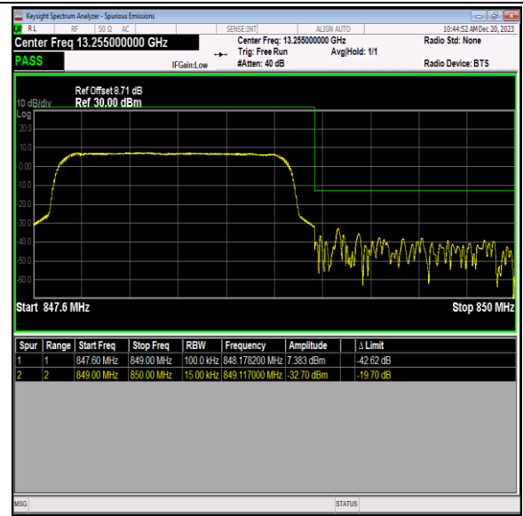
Band5_1.4MHz_64QAM_20643_6RB#0
