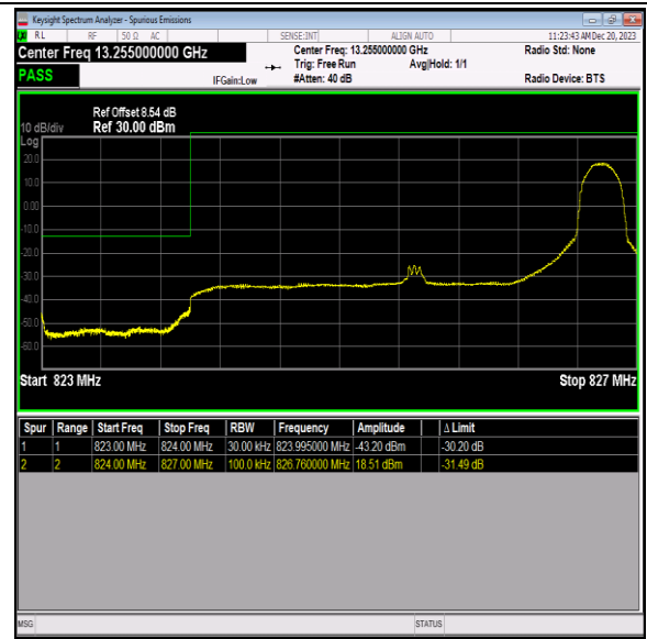
Band5_3MHz_16QAM_20415_1RB#14
