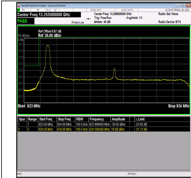
Band5_10MHz_16QAM_20450_1RB#0
