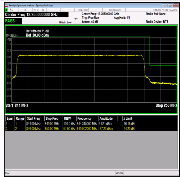
Band5_5MHz_QPSK_20625_25RB#0
