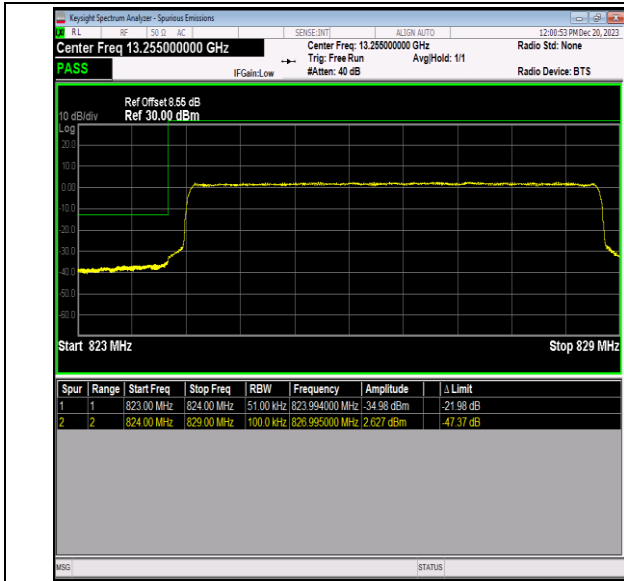
Band5_5MHz_16QAM_20425_25RB#0
