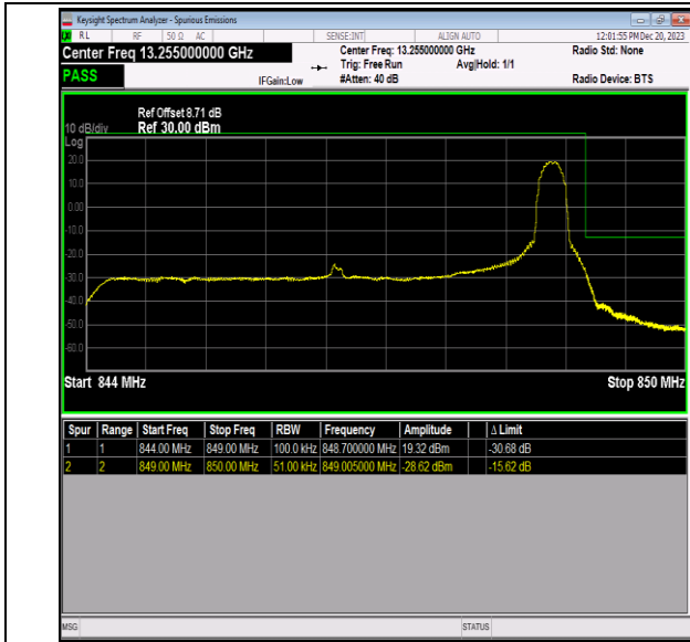
Band5_5MHz_QPSK_20625_1RB#24
