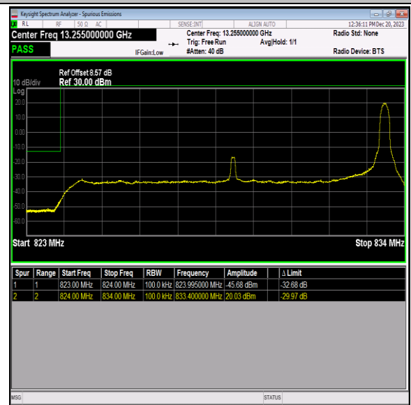
Band5_10MHz_QPSK_20450_1RB#49
