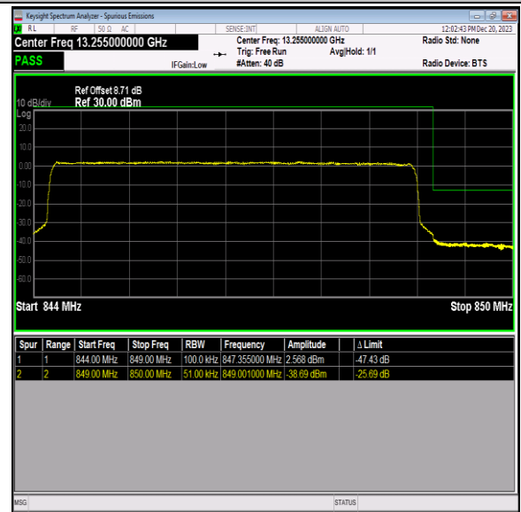
Band5_5MHz_16QAM_20625_25RB#0
