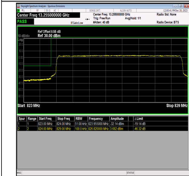
Band5_5MHz_QPSK_20425_25RB#0
