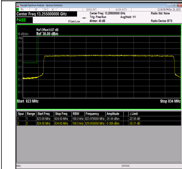
Band5_10MHz_16QAM_20450_50RB#0
