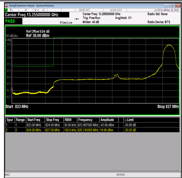
Band5_3MHz_QPSK_20415_1RB#14
