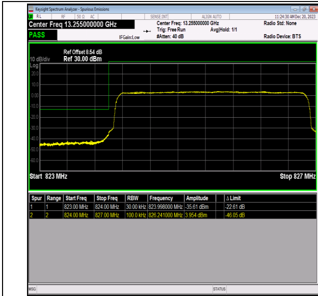
Band5_3MHz_64QAM_20415_15RB#0
