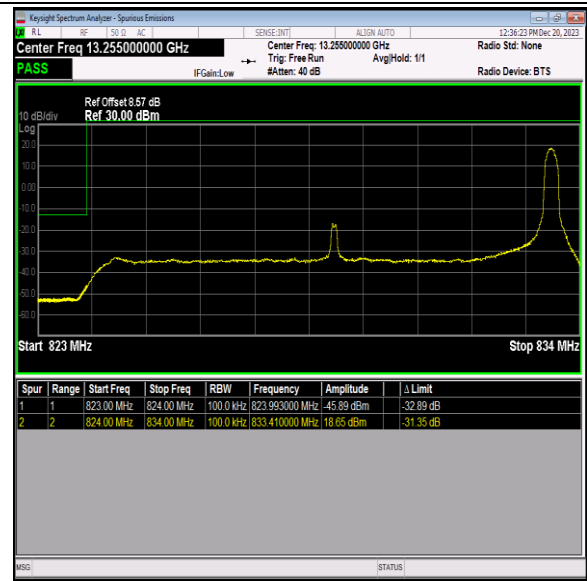
Band5_10MHz_16QAM_20450_1RB#49
