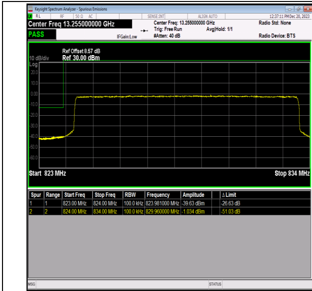
Band5_10MHz_64QAM_20450_50RB#0
