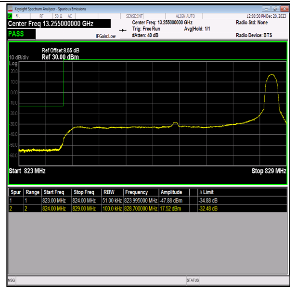
Band5_5MHz_64QAM_20425_1RB#24
