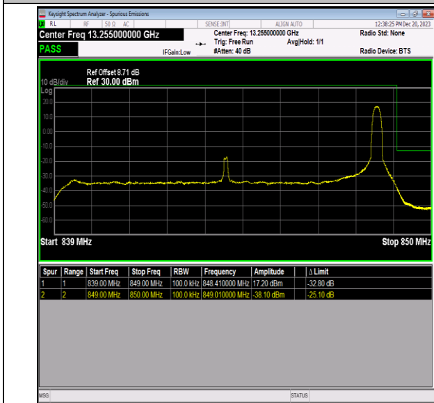
Band5_10MHz_64QAM_20600_1RB#49
