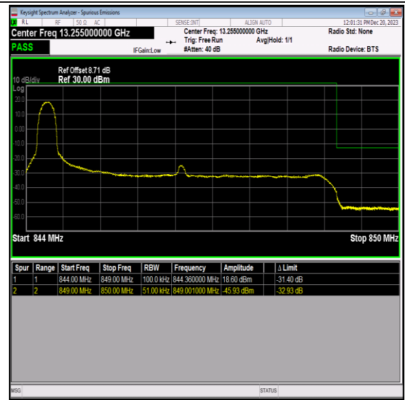
Band5_5MHz_16QAM_20625_1RB#0
