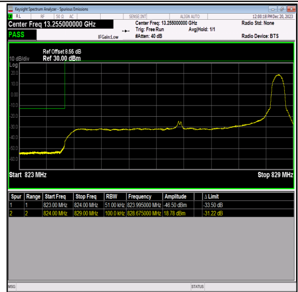
Band5_5MHz_16QAM_20425_1RB#24
