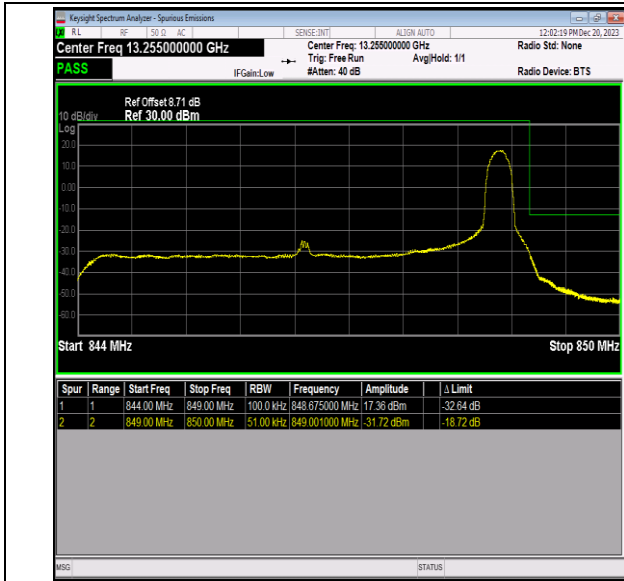
Band5_5MHz_64QAM_20625_1RB#24
