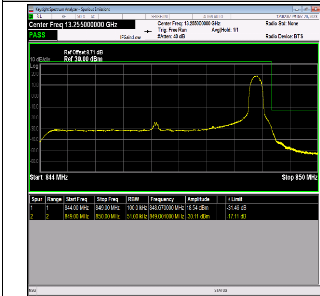
Band5_5MHz_16QAM_20625_1RB#24
