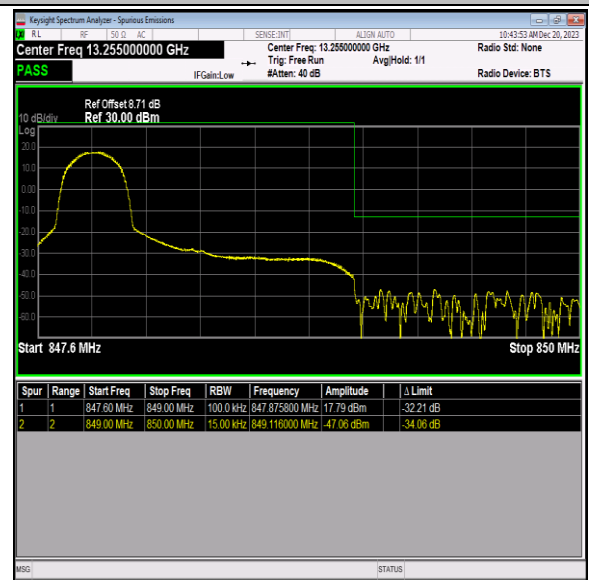
Band5_1.4MHz_64QAM_20643_1RB#0
