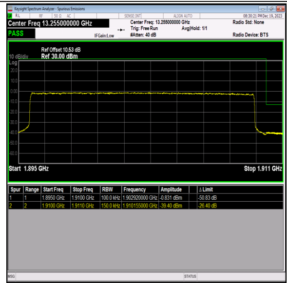
Band2_15MHz_QPSK_19125_75RB#0
