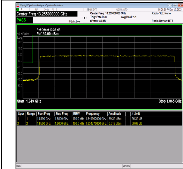
Band2_15MHz_QPSK_18675_75RB#0
