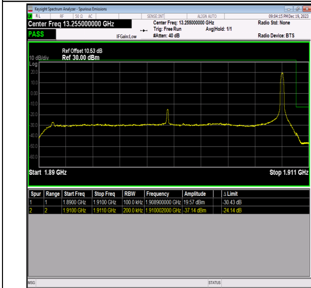
Band2_20MHz_QPSK_19100_1RB#99
