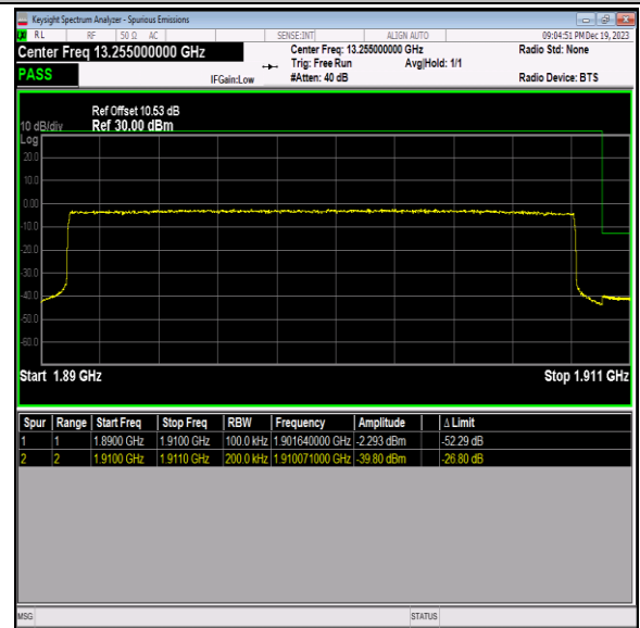
Band2_20MHz_QPSK_19100_100RB#0
