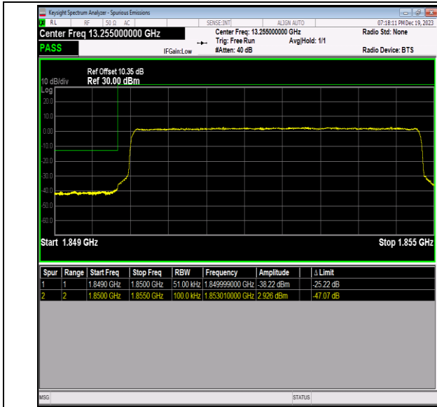
Band2_5MHz_16QAM_18625_25RB#0
