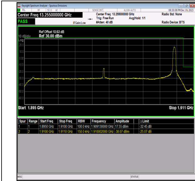
Band2_15MHz_64QAM_19125_1RB#74
