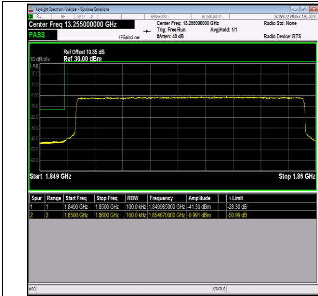
Band2_10MHz_64QAM_18650_50RB#0
