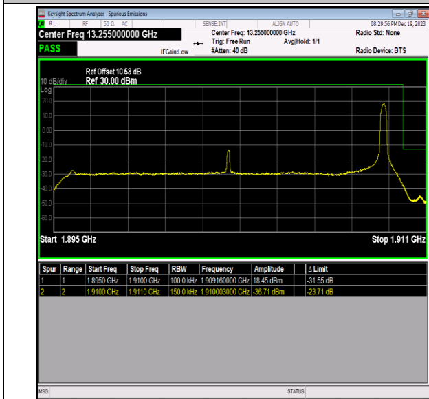
Band2_15MHz_16QAM_19125_1RB#74
