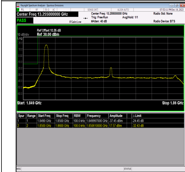
Band2_10MHz_64QAM_18650_1RB#0
