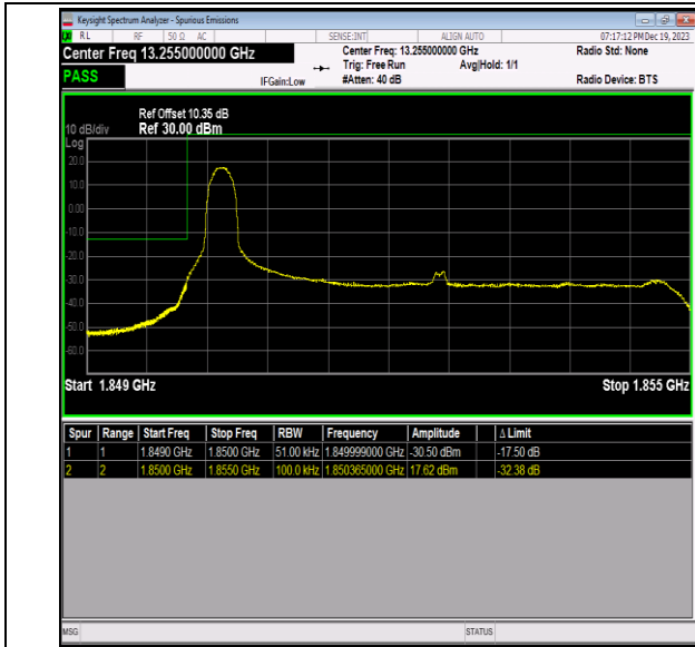
Band2_5MHz_64QAM_18625_1RB#0
