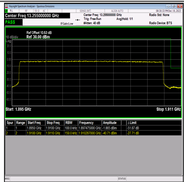
Band2_15MHz_16QAM_19125_75RB#0
