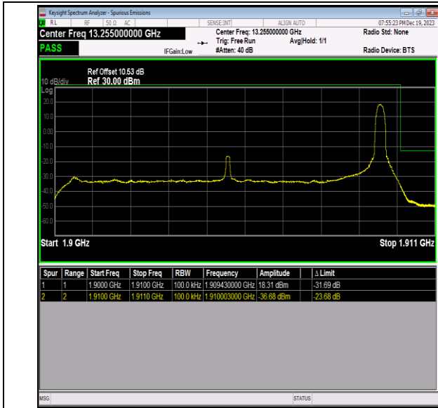
Band2_10MHz_16QAM_19150_1RB#49
