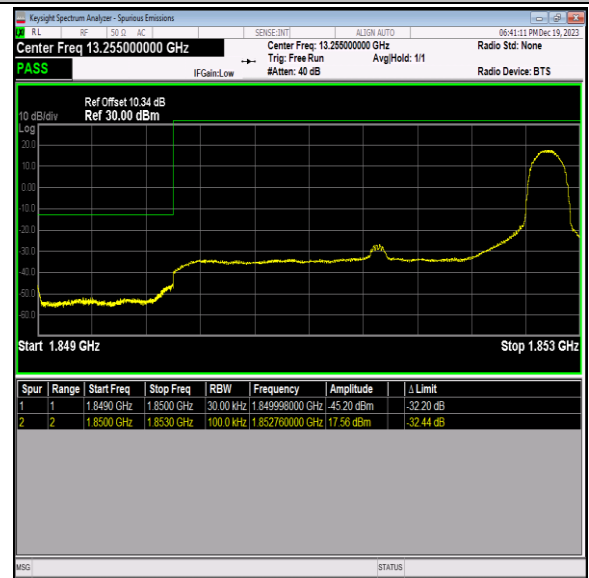
Band2_3MHz_64QAM_18615_1RB#14
