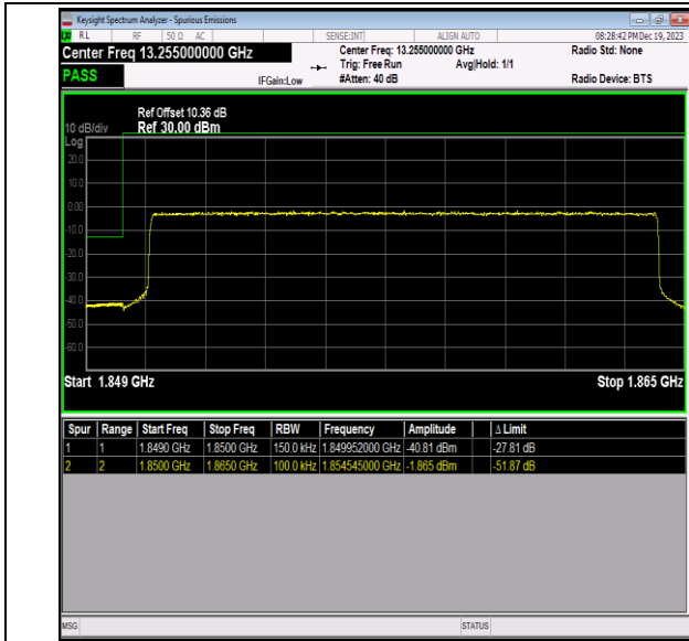
Band2_15MHz_16QAM_18675_75RB#0
