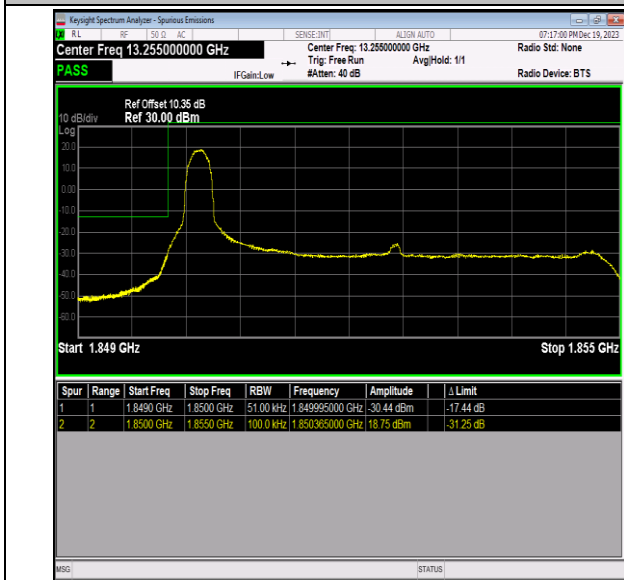
Band2_5MHz_16QAM_18625_1RB#0
