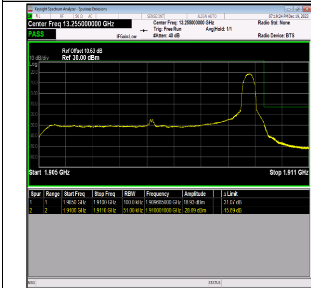
Band2_5MHz_16QAM_19175_1RB#24
