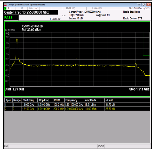
Band2_20MHz_16QAM_19100_1RB#0
