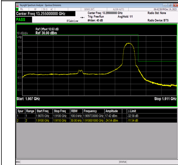
Band2_3MHz_64QAM_19185_1RB#14
