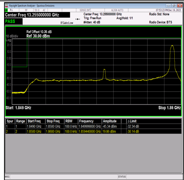
Band2_10MHz_QPSK_18650_1RB#49
