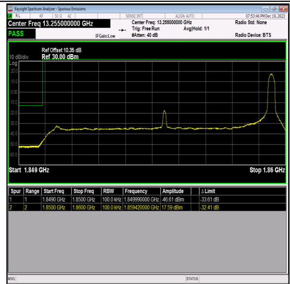
Band2_10MHz_64QAM_18650_1RB#49
