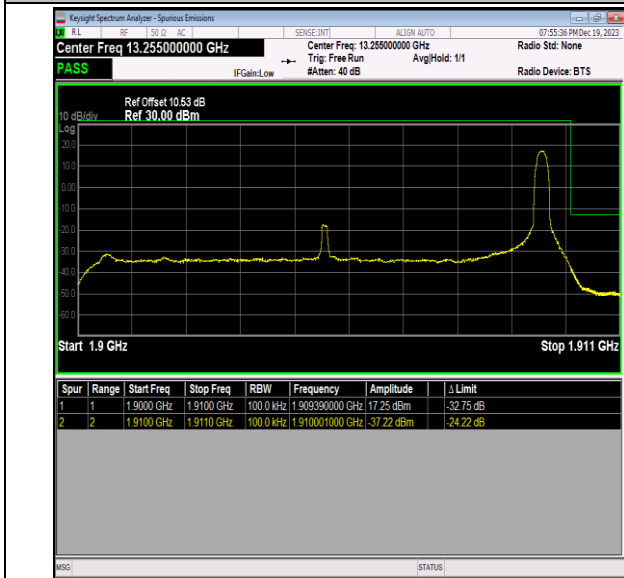
Band2_10MHz_64QAM_19150_1RB#49
