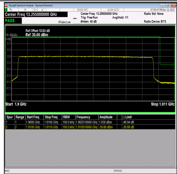
Band2_10MHz_QPSK_19150_50RB#0
