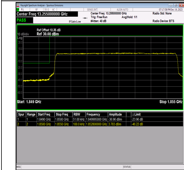
Band2_5MHz_QPSK_18625_25RB#0
