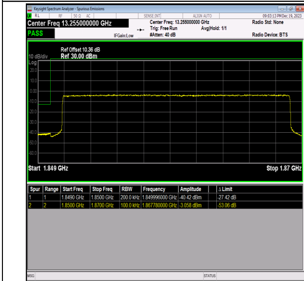
Band2_20MHz_16QAM_18700_100RB#0
