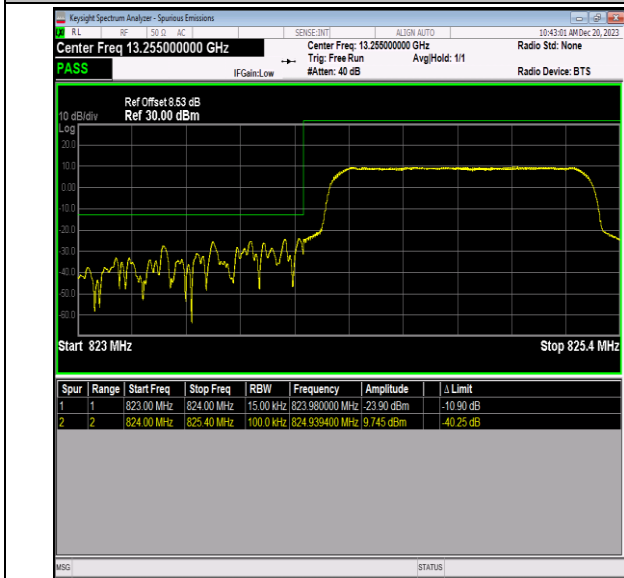
Band5_1.4MHz_QPSK_20407_6RB#0
