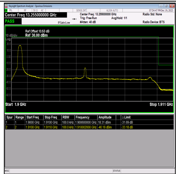
Band2_10MHz_16QAM_19150_1RB#0
