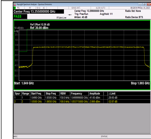
Band2_15MHz_64QAM_18675_75RB#0
