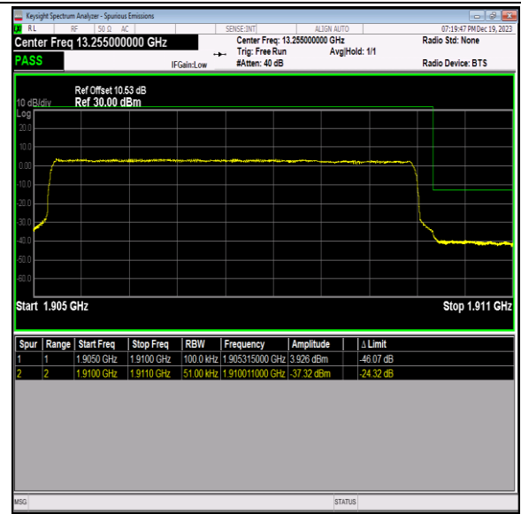
Band2_5MHz_QPSK_19175_25RB#0
