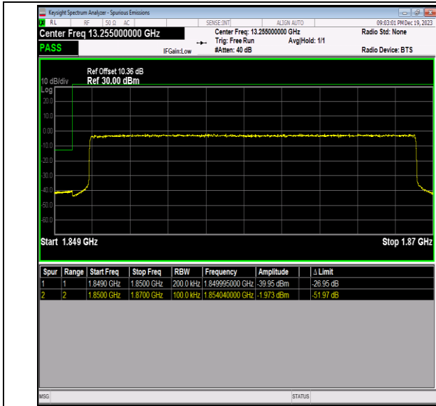
Band2_20MHz_QPSK_18700_100RB#0
