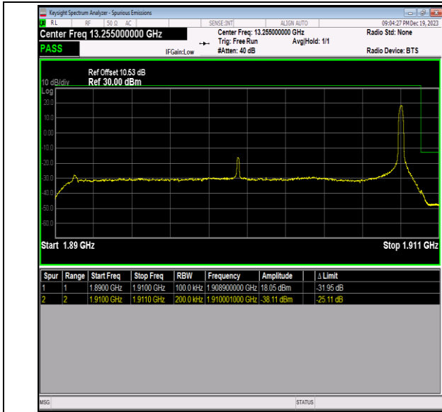
Band2_20MHz_16QAM_19100_1RB#99
