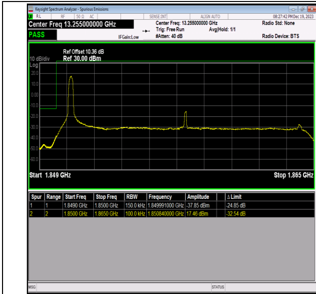
Band2_15MHz_64QAM_18675_1RB#0
