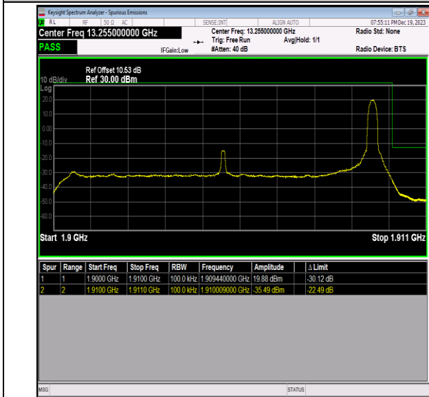
Band2_10MHz_QPSK_19150_1RB#49
