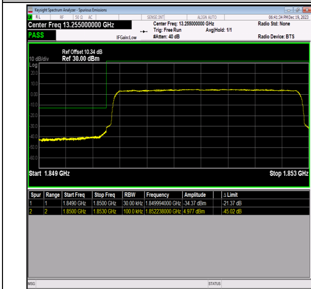
Band2_3MHz_16QAM_18615_15RB#0
