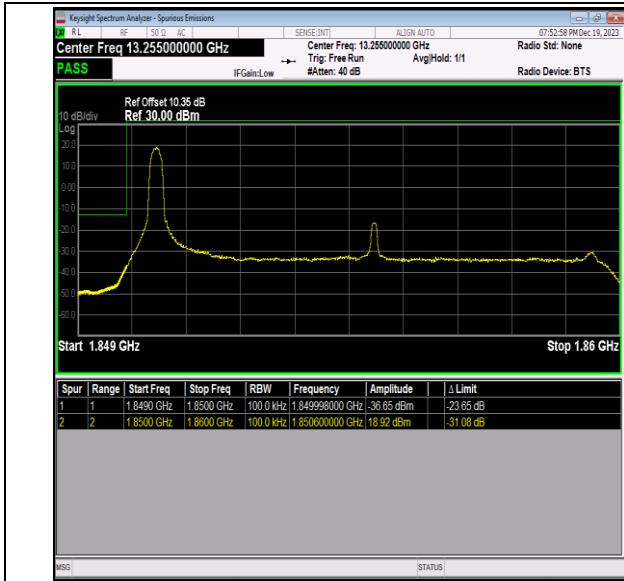
Band2_10MHz_16QAM_18650_1RB#0
