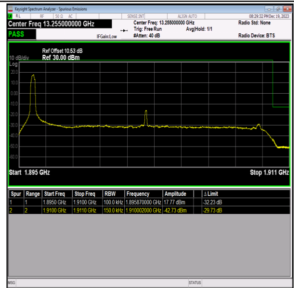
Band2_15MHz_64QAM_19125_1RB#0
