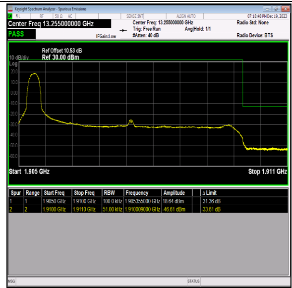
Band2_5MHz_16QAM_19175_1RB#0
