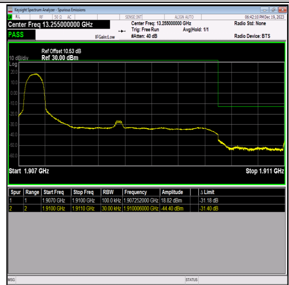
Band2_3MHz_16QAM_19185_1RB#0
