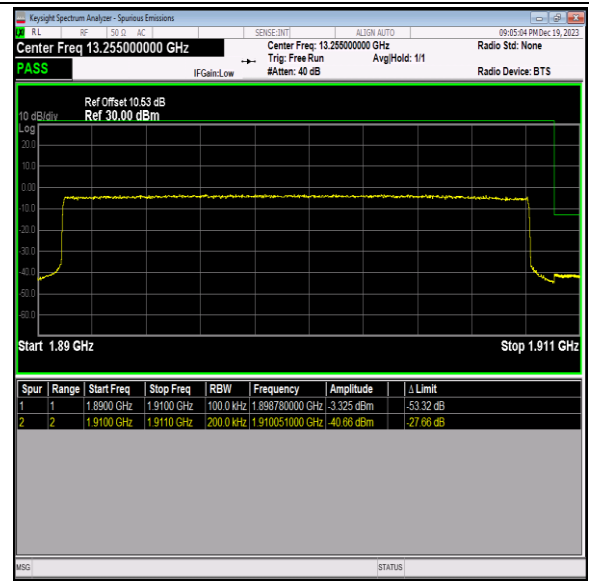
Band2_20MHz_16QAM_19100_100RB#0
