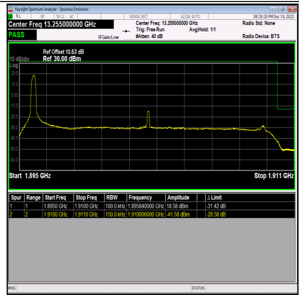
Band2_15MHz_16QAM_19125_1RB#0
