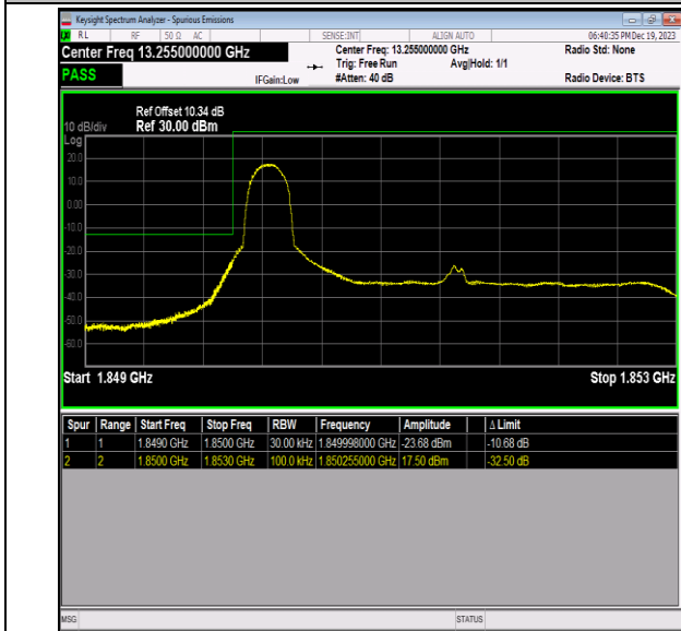
Band2_3MHz_64QAM_18615_1RB#0
