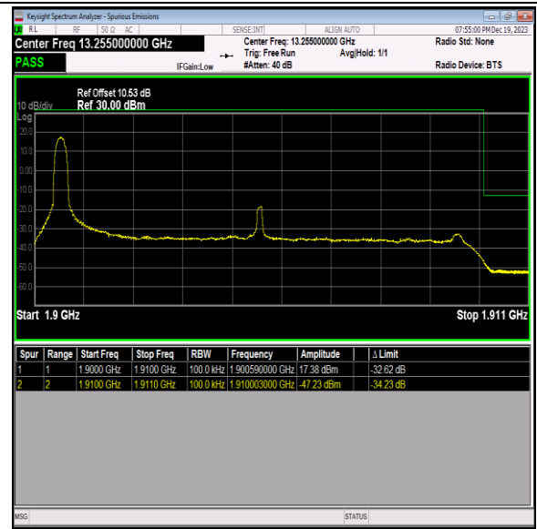
Band2_10MHz_64QAM_19150_1RB#0
