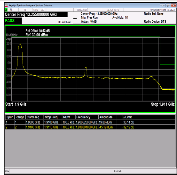
Band2_10MHz_QPSK_19150_1RB#0
