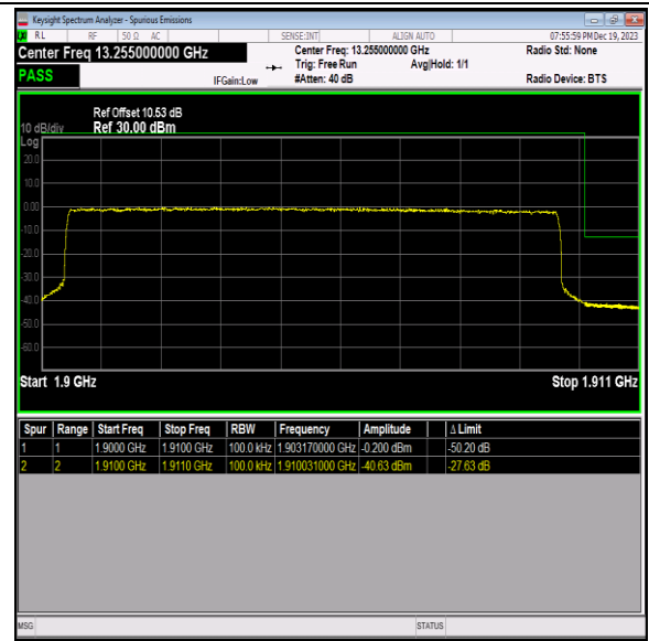
Band2_10MHz_16QAM_19150_50RB#0
