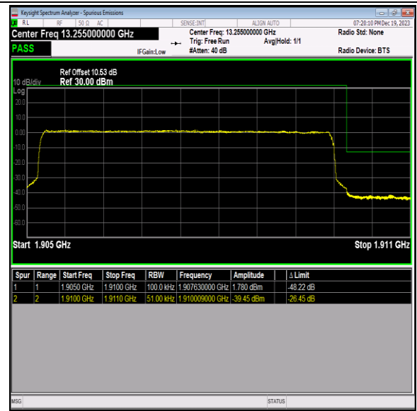
Band2_5MHz_64QAM_19175_25RB#0
