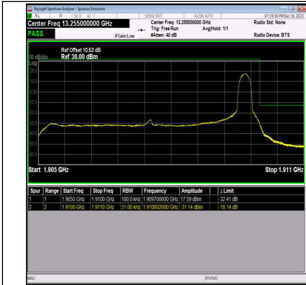
Band2_5MHz_64QAM_19175_1RB#24
