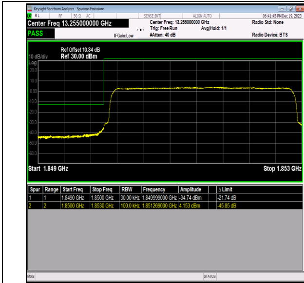
Band2_3MHz_64QAM_18615_15RB#0
