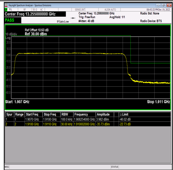
Band2_3MHz_64QAM_19185_15RB#0
