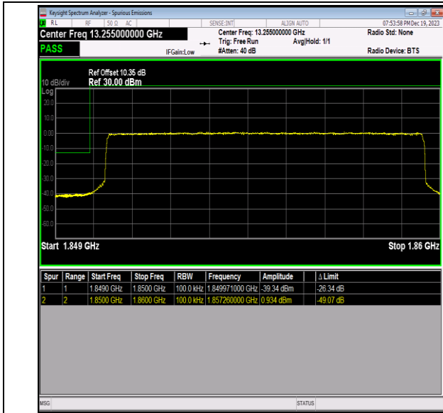
Band2_10MHz_QPSK_18650_50RB#0
