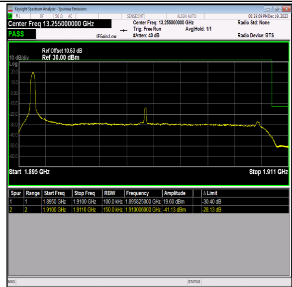
Band2_15MHz_QPSK_19125_1RB#0
