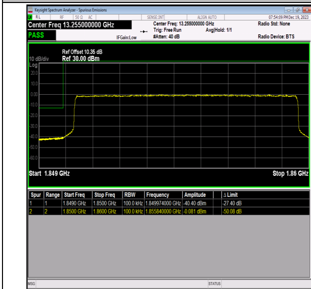
Band2_10MHz_16QAM_18650_50RB#0
