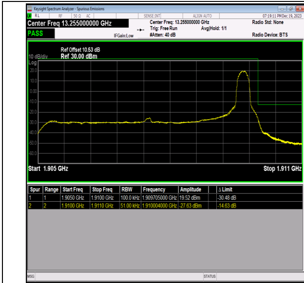
Band2_5MHz_QPSK_19175_1RB#24
