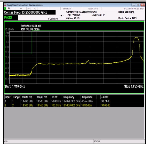
Band2_5MHz_16QAM_18625_1RB#24
