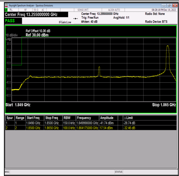
Band2_15MHz_64QAM_18675_1RB#74
