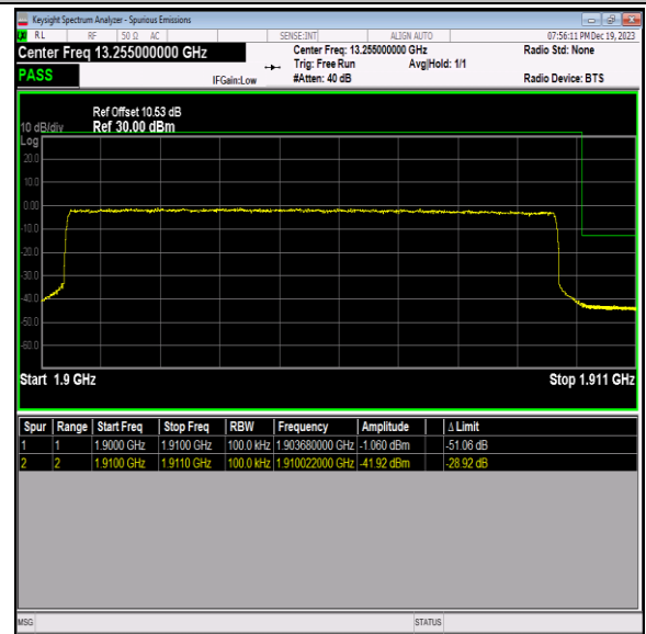
Band2_10MHz_64QAM_19150_50RB#0
