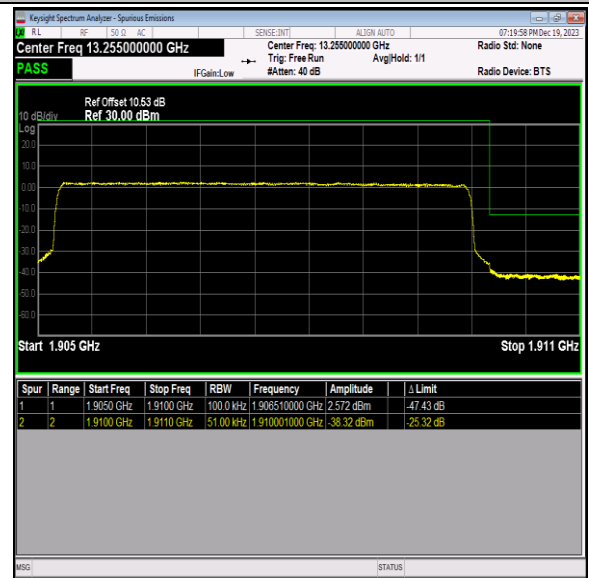
Band2_5MHz_16QAM_19175_25RB#0
