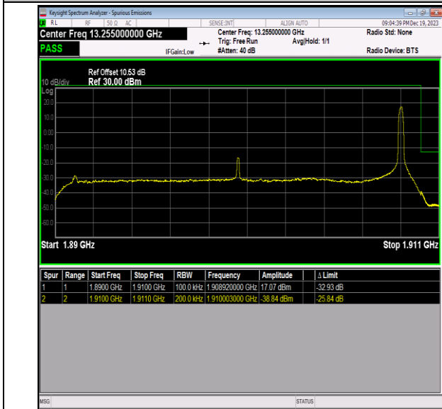
Band2_20MHz_64QAM_19100_1RB#99
