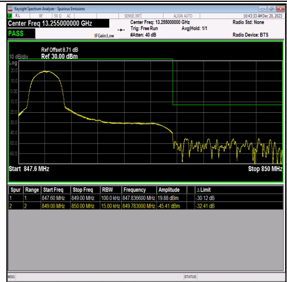
Band5_1.4MHz_QPSK_20643_1RB#0
