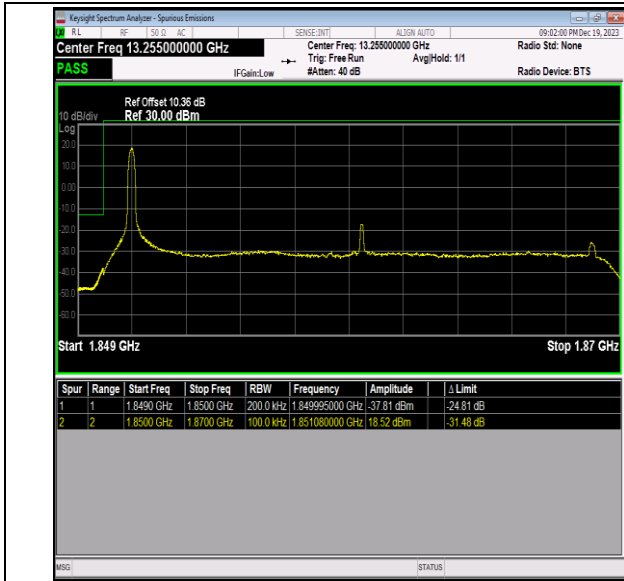
Band2_20MHz_16QAM_18700_1RB#0
