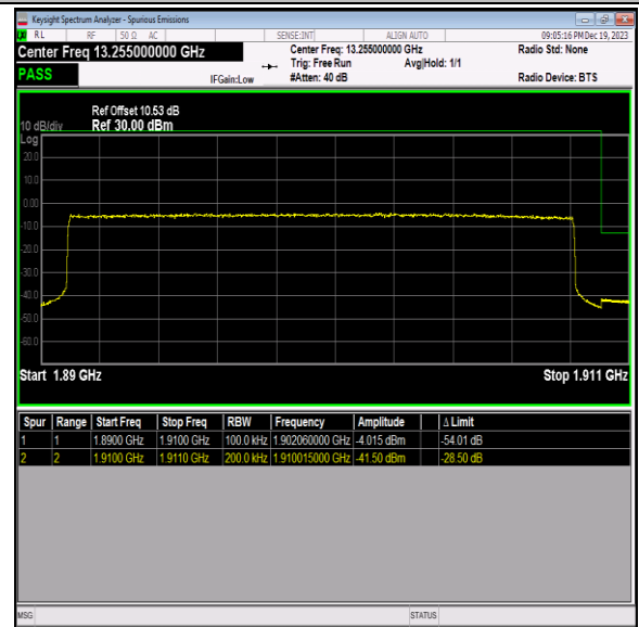
Band2_20MHz_64QAM_19100_100RB#0
