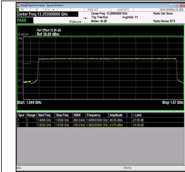
Band2_20MHz_64QAM_18700_100RB#0
