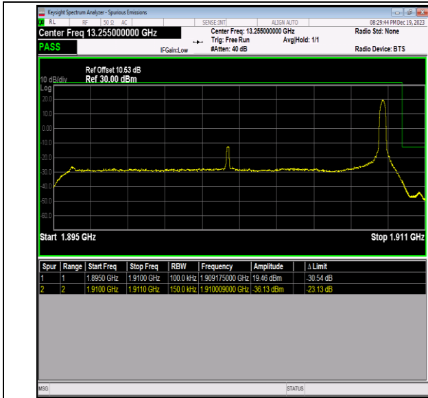
Band2_15MHz_QPSK_19125_1RB#74
