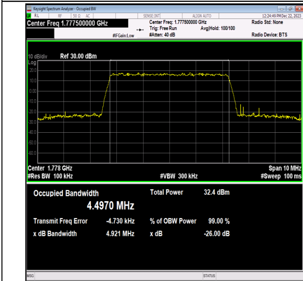
Band66-5MHz-QPSK-132647-25RB#0-PASS
