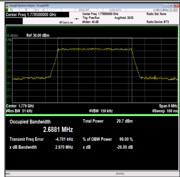
Band66-3MHz-64QAM-132657-15RB#0-PASS
