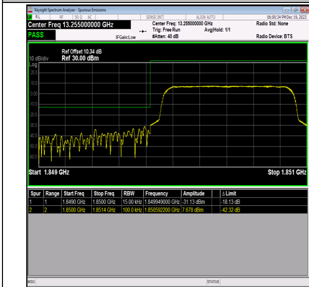
Band2_1.4MHz_64QAM_18607_6RB#0
