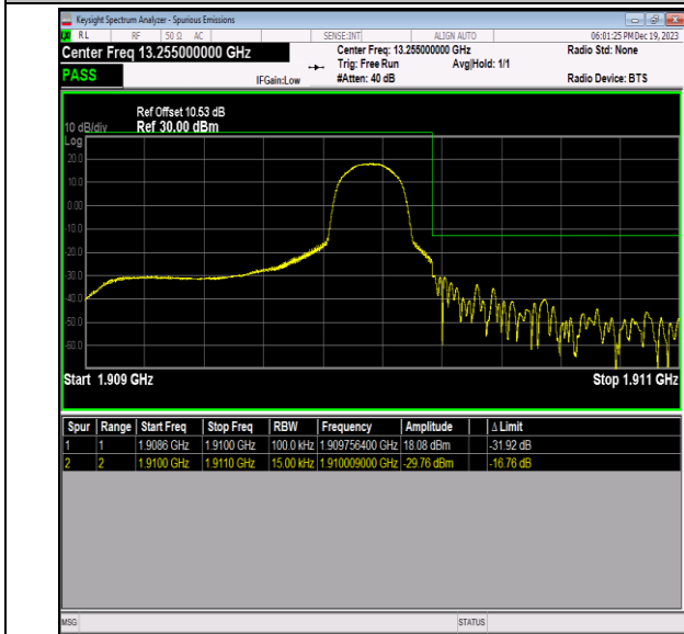
Band2_1.4MHz_16QAM_19193_1RB#5
