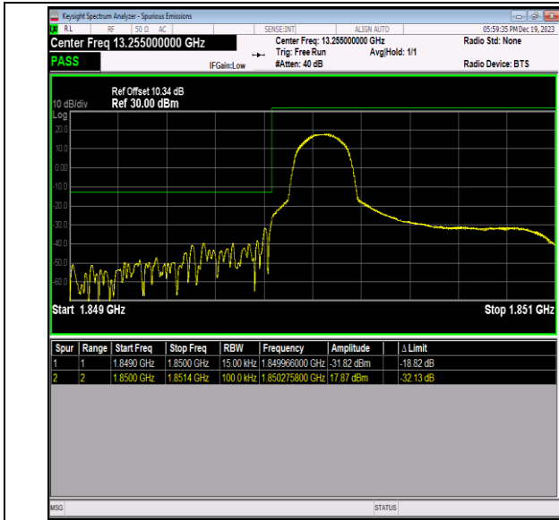
Band2_1.4MHz_64QAM_18607_1RB#0
