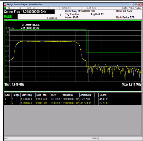
Band2_1.4MHz_16QAM_19193_6RB#0
