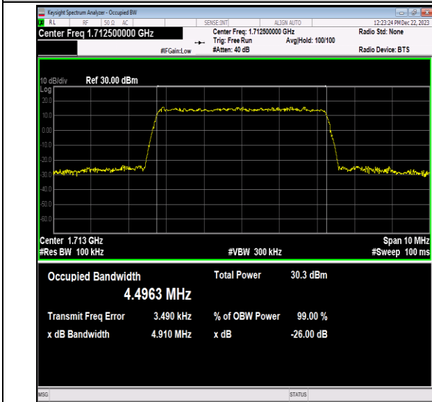
Band66-5MHz-64QAM-131997-25RB#0-PASS
