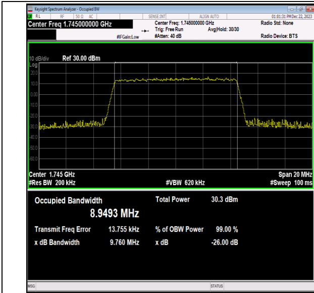
Band66-10MHz-64QAM-132322-50RB#0-PASS
