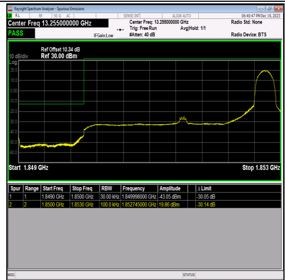
Band2_3MHz_QPSK_18615_1RB#14
