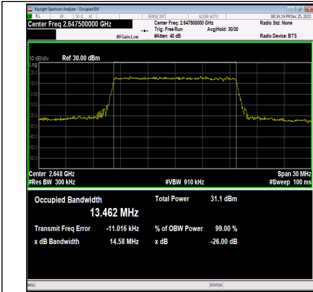
41(2535-2655)-15MHz-64QAM-41165-75RB#0-PASS
