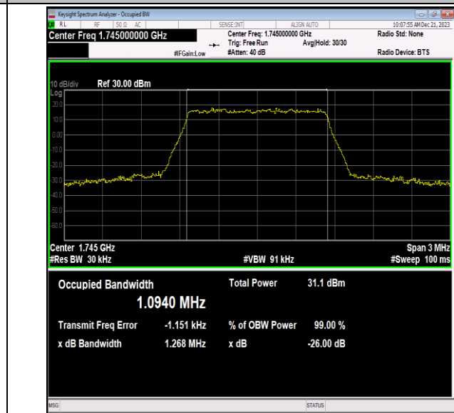
Band66-1.4MHz-QPSK-132322-6RB#0-PASS
