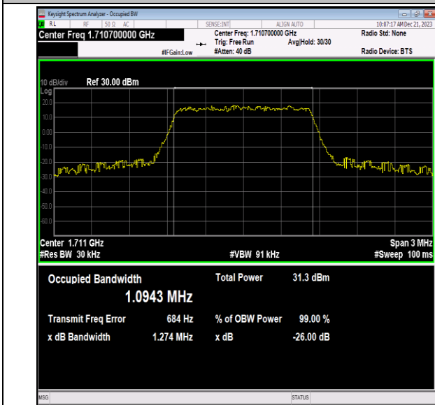
Band66-1.4MHz-QPSK-131979-6RB#0-PASS
