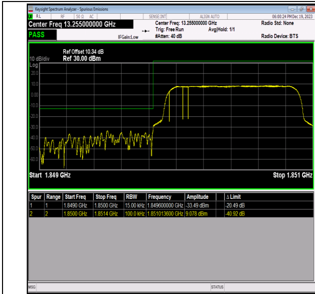
Band2_1.4MHz_16QAM_18607_6RB#0
