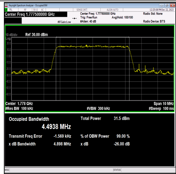
Band66-5MHz-16QAM-132647-25RB#0-PASS
