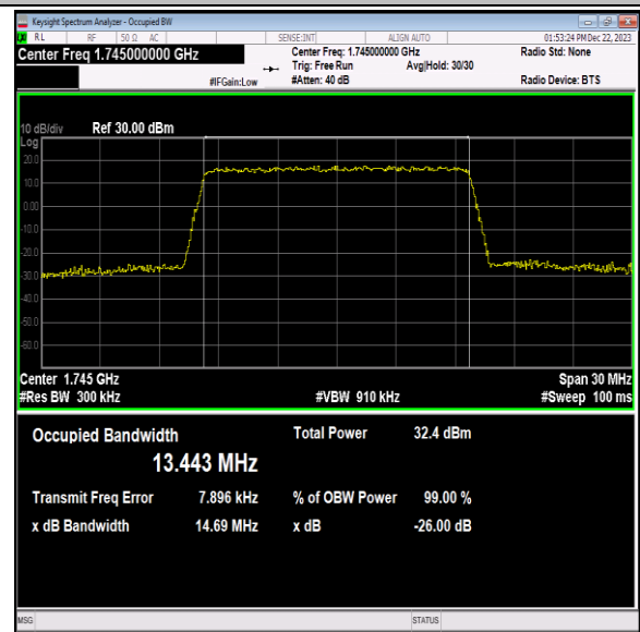
Band66-15MHz-QPSK-132322-75RB#0-PASS
