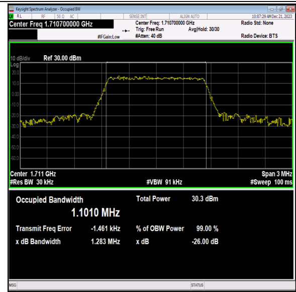
Band66-1.4MHz-16QAM-131979-6RB#0-PASS
