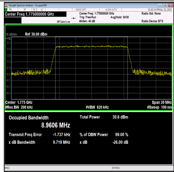
Band66-10MHz-64QAM-132622-50RB#0-PASS
