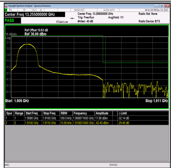
Band2_1.4MHz_64QAM_19193_1RB#0
