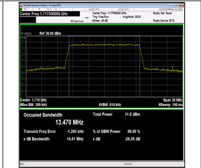
Band66-15MHz-16QAM-132047-75RB#0-PASS
