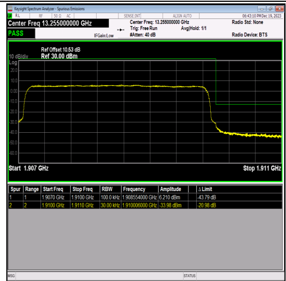
Band2_3MHz_QPSK_19185_15RB#0
