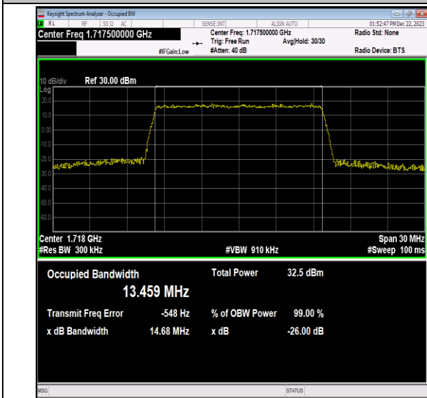
Band66-15MHz-QPSK-132047-75RB#0-PASS
