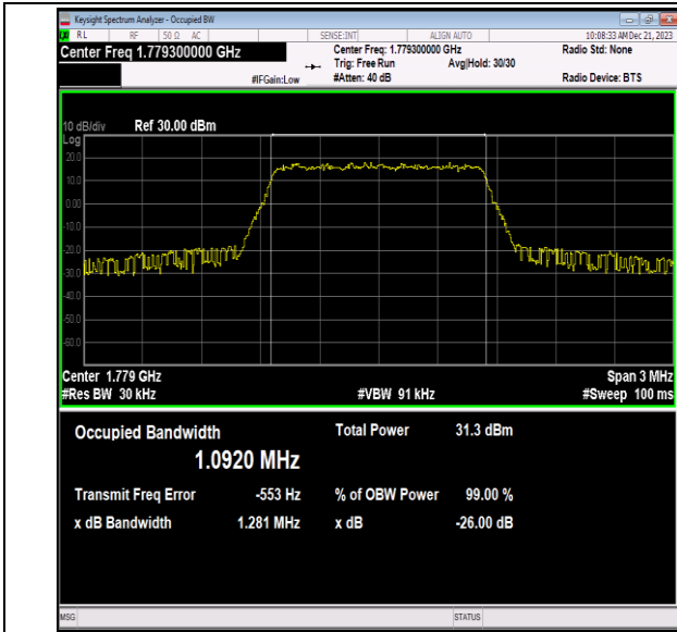
Band66-1.4MHz-QPSK-132665-6RB#0-PASS
