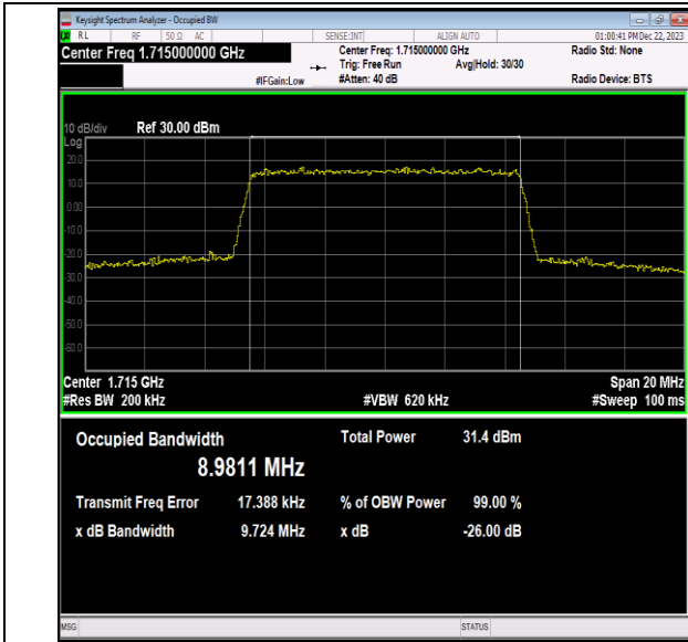
Band66-10MHz-16QAM-132022-50RB#0-PASS
