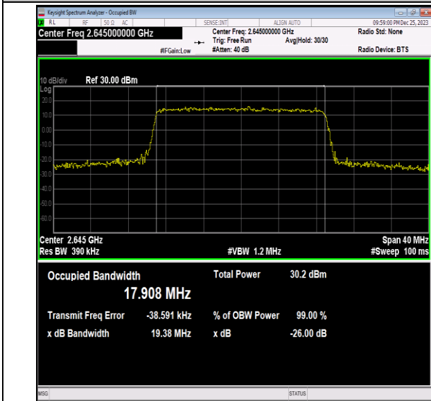
41(2535-2655)-20MHz-16QAM-41140-100RB#0-PASS
