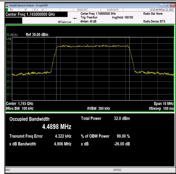
Band66-5MHz-QPSK-132322-25RB#0-PASS
