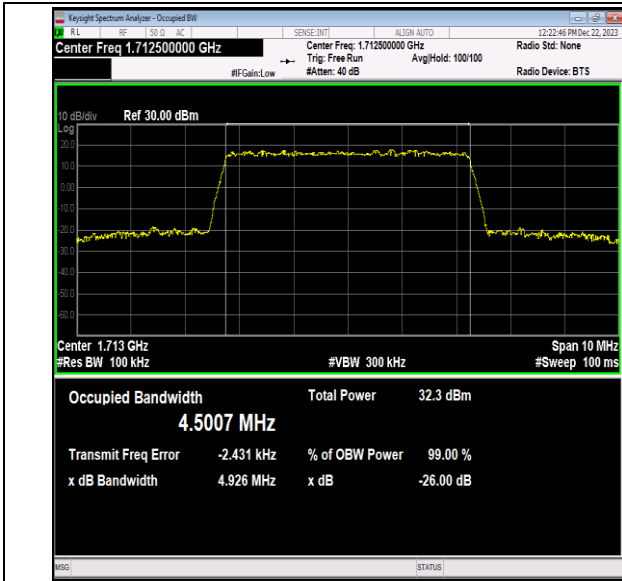
Band66-5MHz-QPSK-131997-25RB#0-PASS
