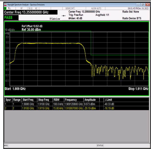
Band2_1.4MHz_QPSK_19193_6RB#0
