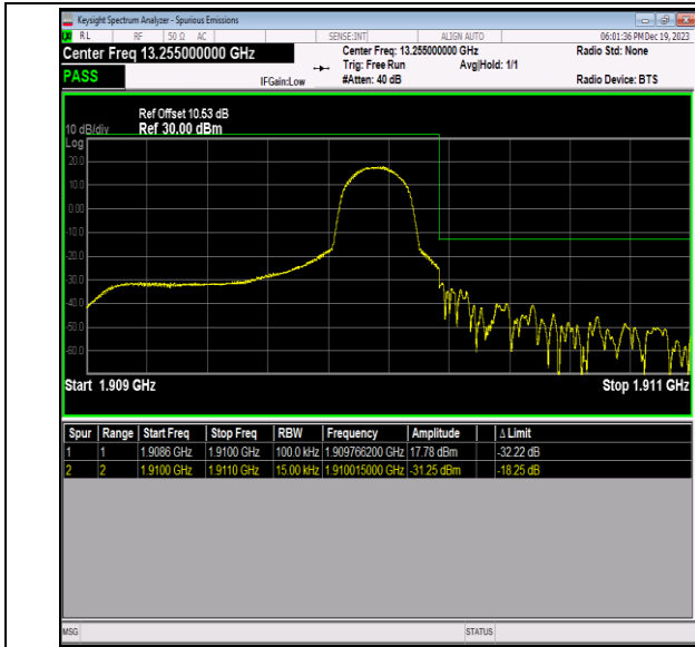
Band2_1.4MHz_64QAM_19193_1RB#5
