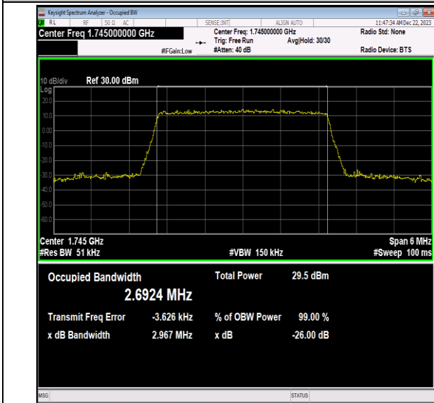
Band66-3MHz-64QAM-132322-15RB#0-PASS
