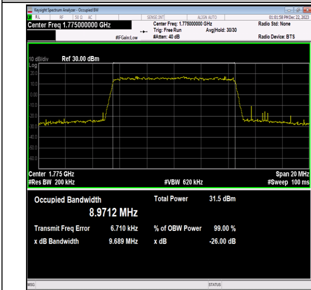
Band66-10MHz-16QAM-132622-50RB#0-PASS
