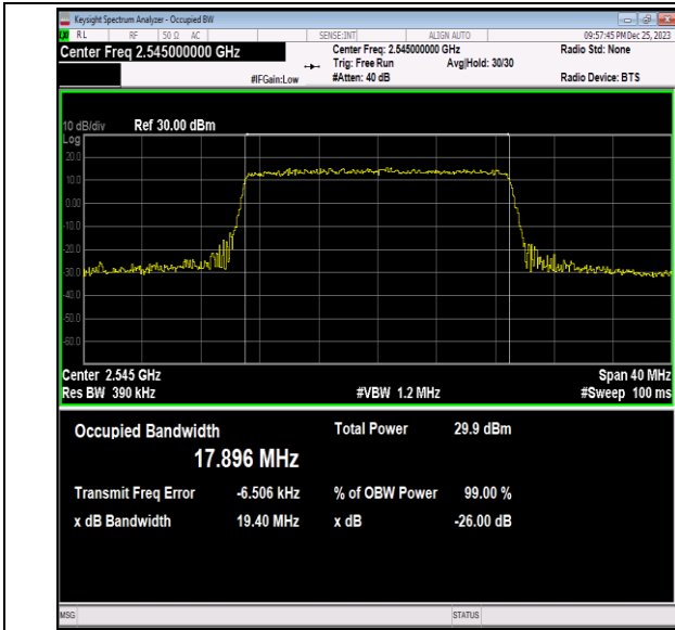
41(2535-2655)-20MHz-16QAM-40140-100RB#0-PASS
