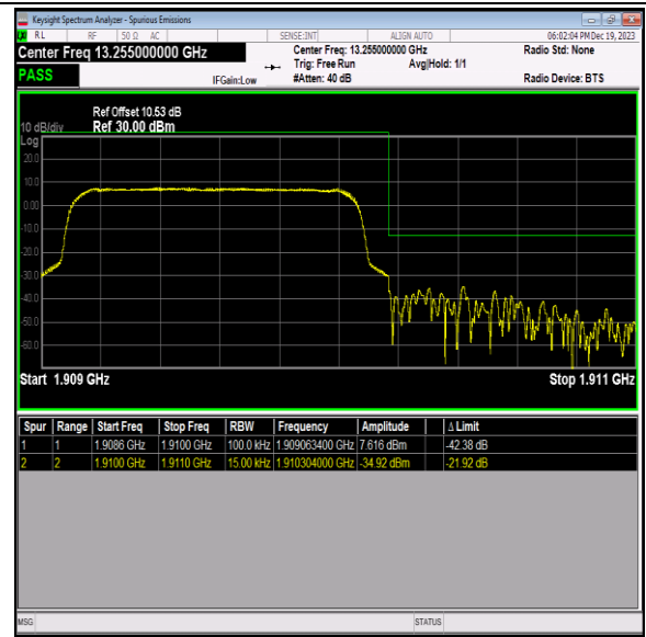
Band2_1.4MHz_64QAM_19193_6RB#0
