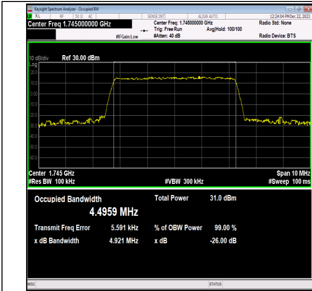
Band66-5MHz-16QAM-132322-25RB#0-PASS
