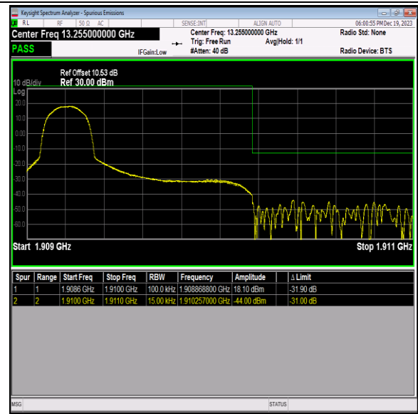
Band2_1.4MHz_16QAM_19193_1RB#0
