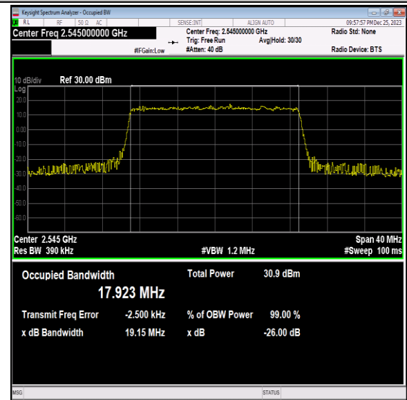
41(2535-2655)-20MHz-64QAM-40140-100RB#0-PASS
