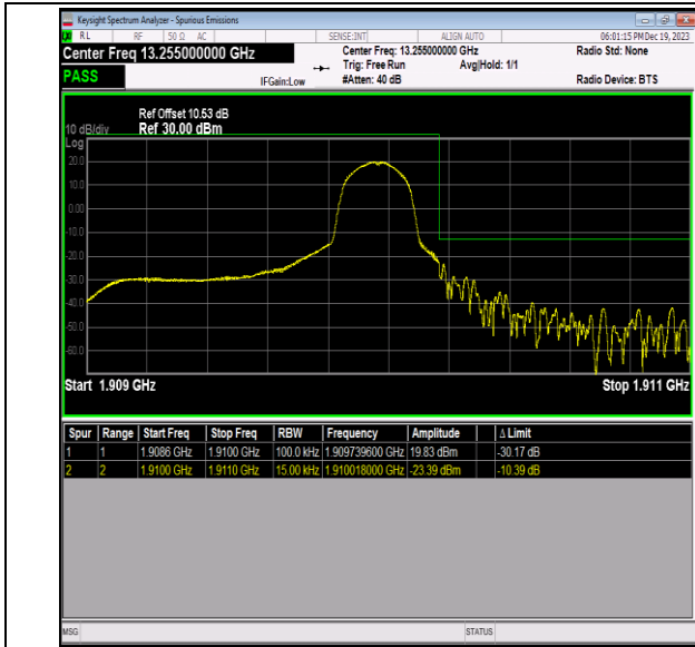
Band2_1.4MHz_QPSK_19193_1RB#5
