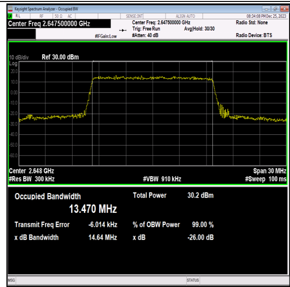
41(2535-2655)-15MHz-16QAM-41165-75RB#0-PASS
