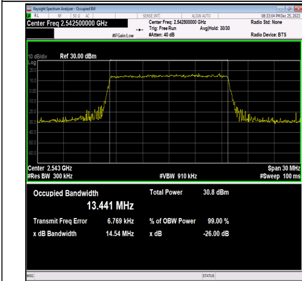
41(2535-2655)-15MHz-64QAM-40115-75RB#0-PASS
