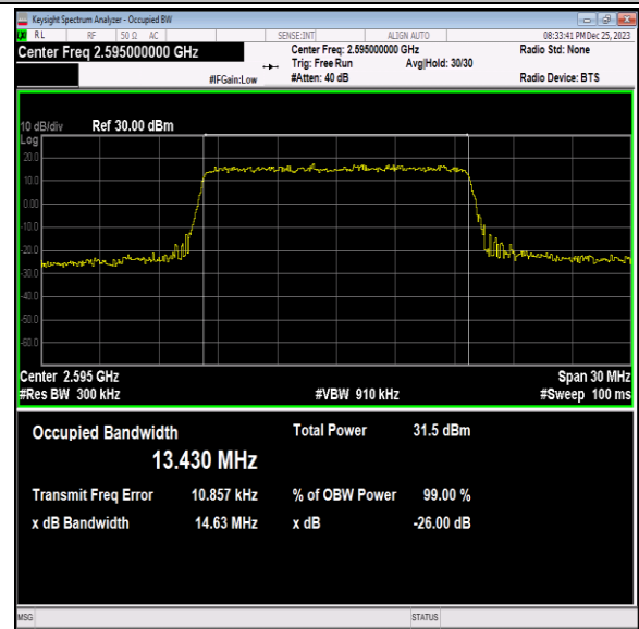
41(2535-2655)-15MHz-64QAM-40640-75RB#0-PASS
