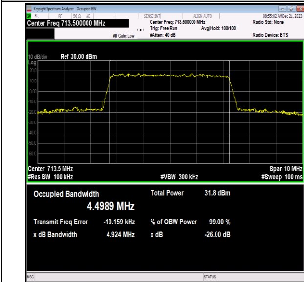
Band12-5MHz-QPSK-23155-25RB#0-PASS
