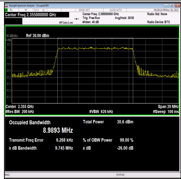
40(2350-2360)-10MHz-64QAM-39200-50RB#0-PASS
