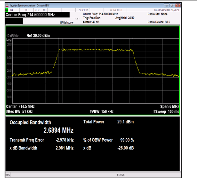
Band12-3MHz-64QAM-23165-15RB#0-PASS
