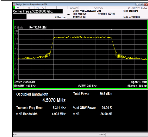
40(2350-2360)-5MHz-QPSK-39175-25RB#0-PASS
