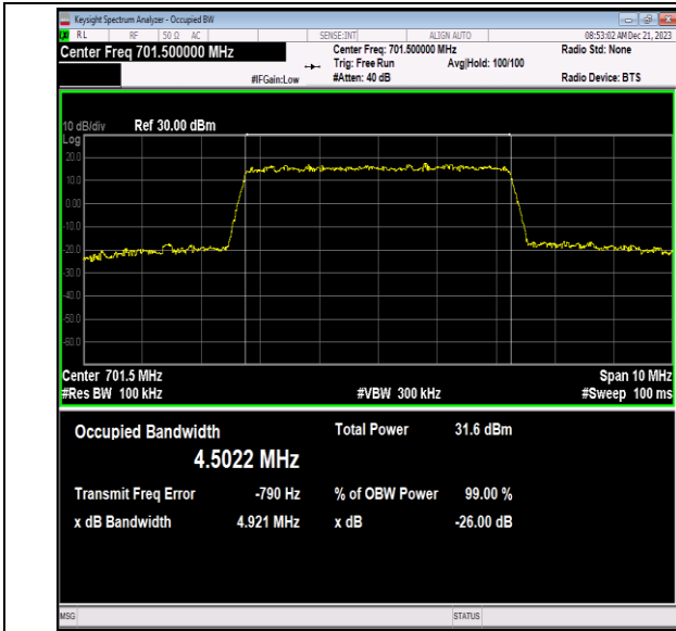
Band12-5MHz-QPSK-23035-25RB#0-PASS
