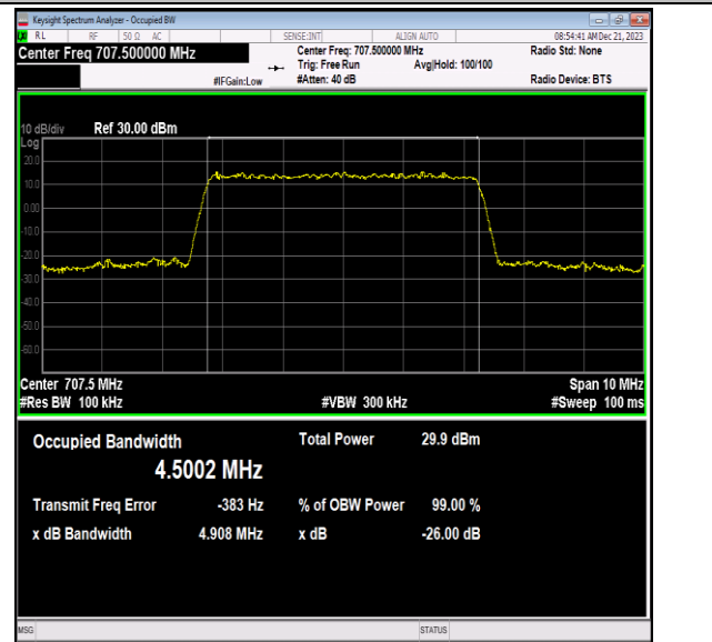
Band12-5MHz-64QAM-23095-25RB#0-PASS
