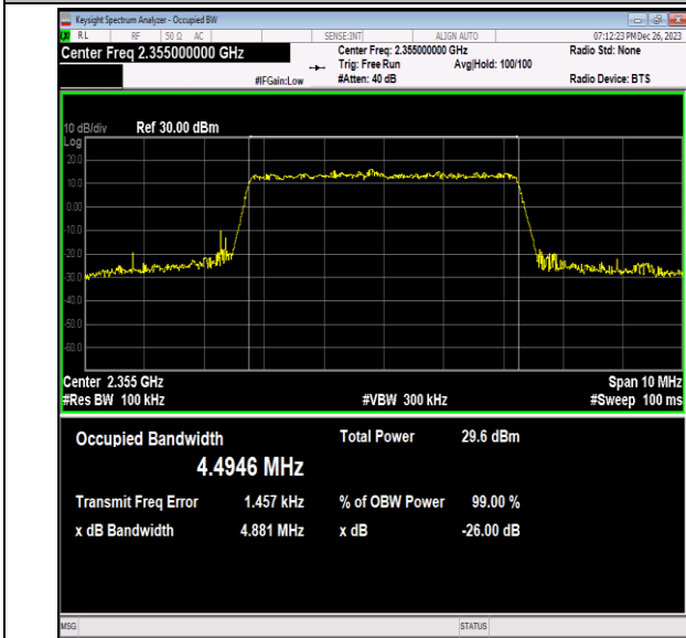
40(2350-2360)-5MHz-16QAM-39200-25RB#0-PASS
