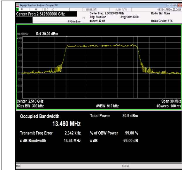
41(2535-2655)-15MHz-QPSK-40115-75RB#0-PASS
