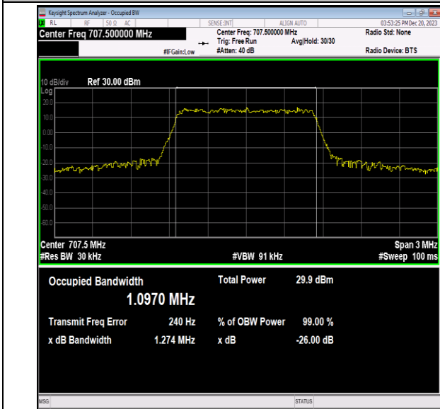
Band12-1.4MHz-16QAM-23095-6RB#0-PASS
