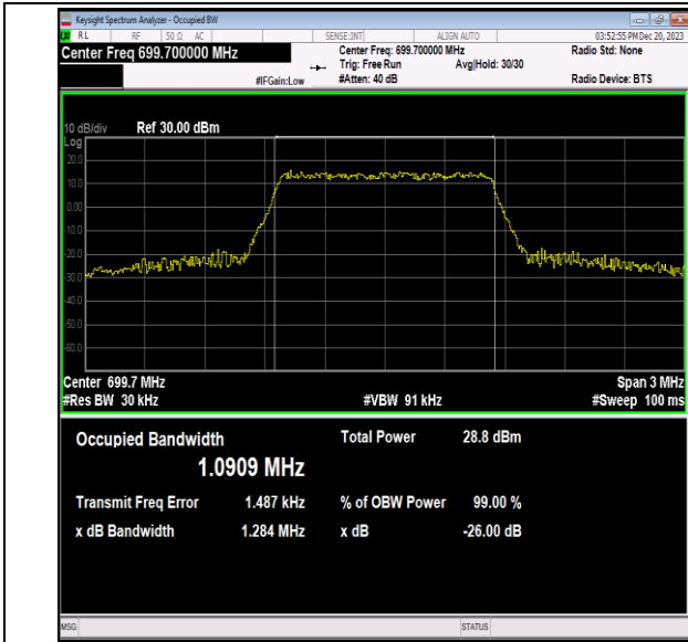
Band12-1.4MHz-64QAM-23017-6RB#0-PASS
