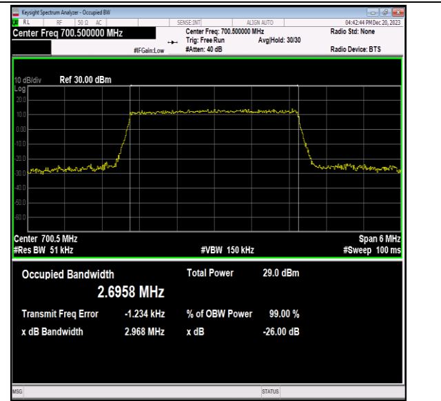
Band12-3MHz-64QAM-23025-15RB#0-PASS
