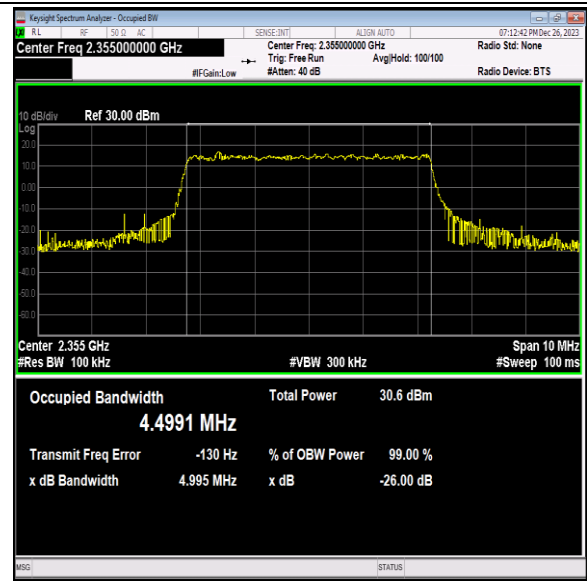
40(2350-2360)-5MHz-64QAM-39200-25RB#0-PASS
