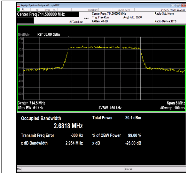
Band12-3MHz-16QAM-23165-15RB#0-PASS
