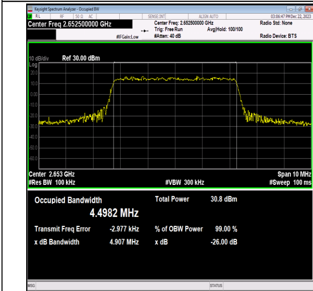
41(2535-2655)-5MHz-64QAM-41215-25RB#0-PASS
