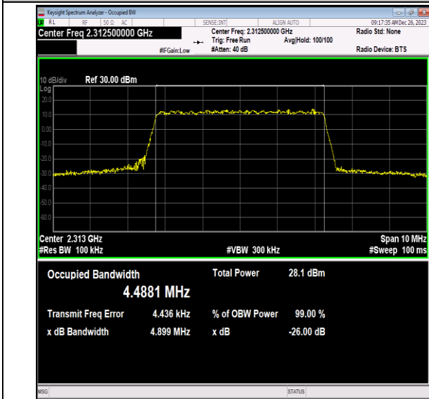
40(2305-2315)-5MHz-64QAM-38775-25RB#0-PASS
