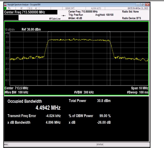
Band12-5MHz-16QAM-23155-25RB#0-PASS
