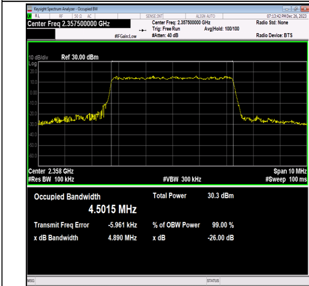
40(2350-2360)-5MHz-64QAM-39225-25RB#0-PASS
