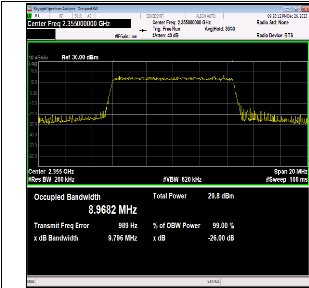
40(2350-2360)-10MHz-16QAM-39200-50RB#0-PASS
