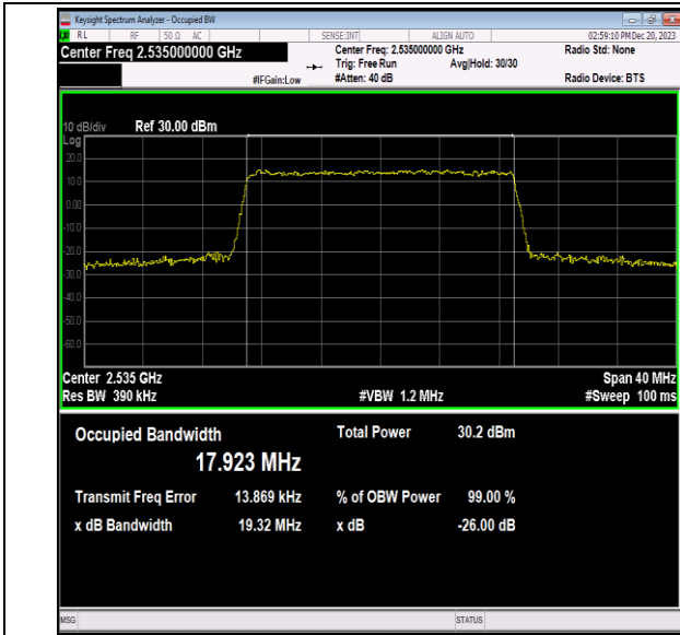
Band7-20MHz-64QAM-21100-100RB#0-PASS
