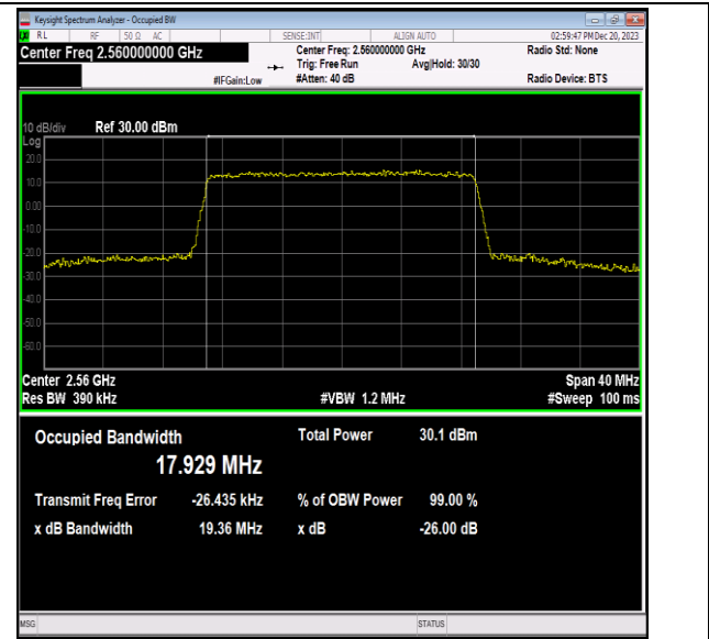
Band7-20MHz-64QAM-21350-100RB#0-PASS
