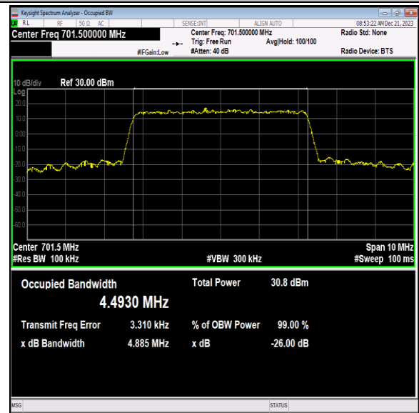
Band12-5MHz-16QAM-23035-25RB#0-PASS
