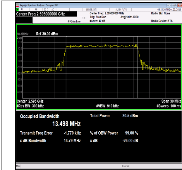
41(2535-2655)-15MHz-16QAM-40640-75RB#0-PASS
