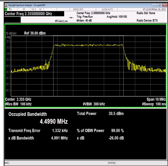
40(2350-2360)-5MHz-QPSK-39200-25RB#0-PASS
