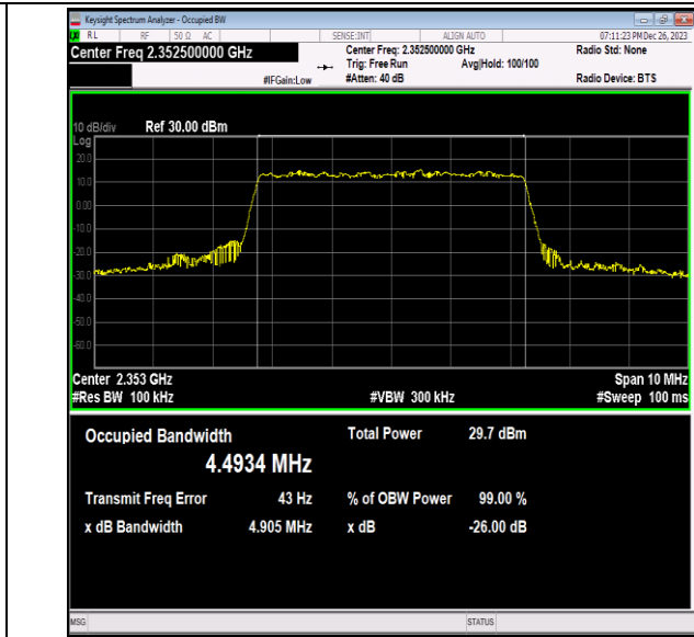
40(2350-2360)-5MHz-16QAM-39175-25RB#0-PASS
