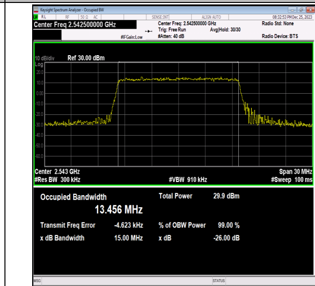
41(2535-2655)-15MHz-16QAM-40115-75RB#0-PASS
