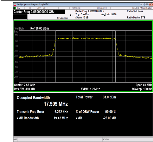
Band7-20MHz-16QAM-21350-100RB#0-PASS
