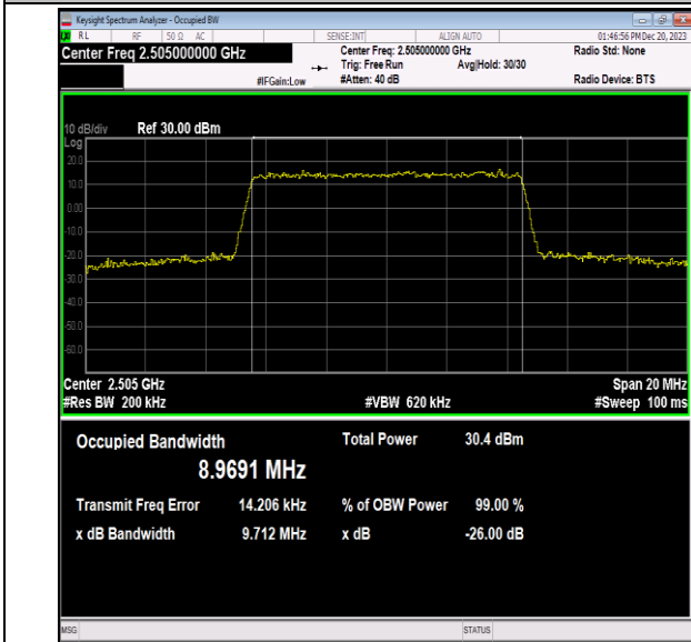
Band7-10MHz-16QAM-20800-50RB#0-PASS
