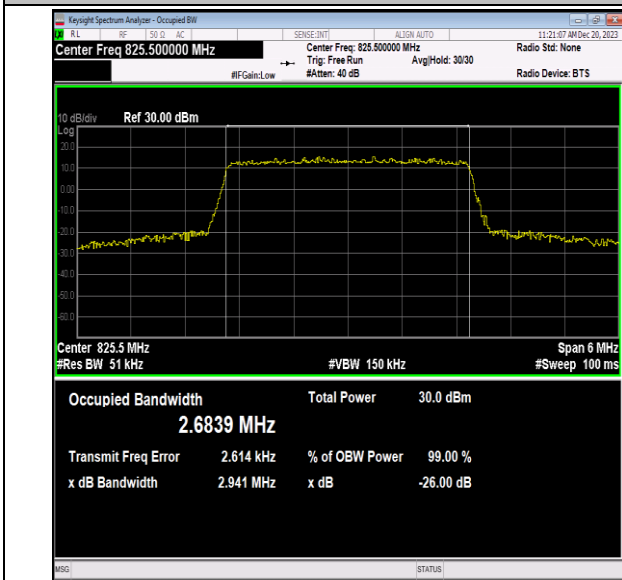
Band5-3MHz-16QAM-20415-15RB#0-PASS
