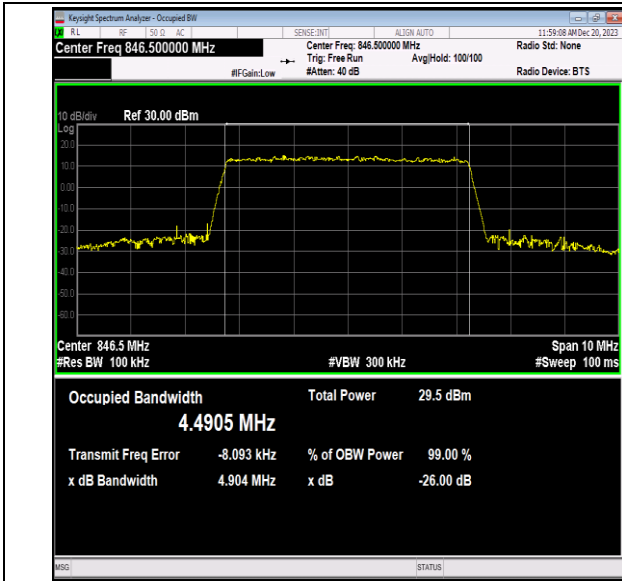
Band5-5MHz-64QAM-20625-25RB#0-PASS
