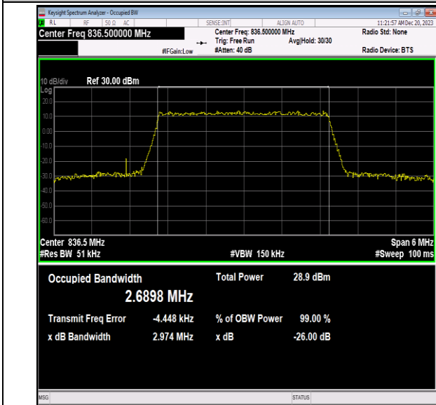
Band5-3MHz-64QAM-20525-15RB#0-PASS
