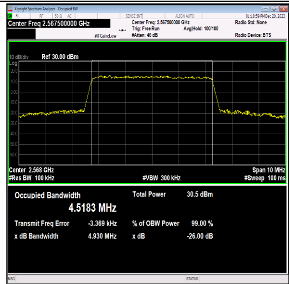
Band7-5MHz-16QAM-21425-25RB#0-PASS
