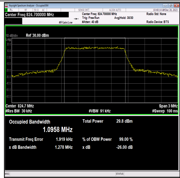
Band5-1.4MHz-16QAM-20407-6RB#0-PASS
