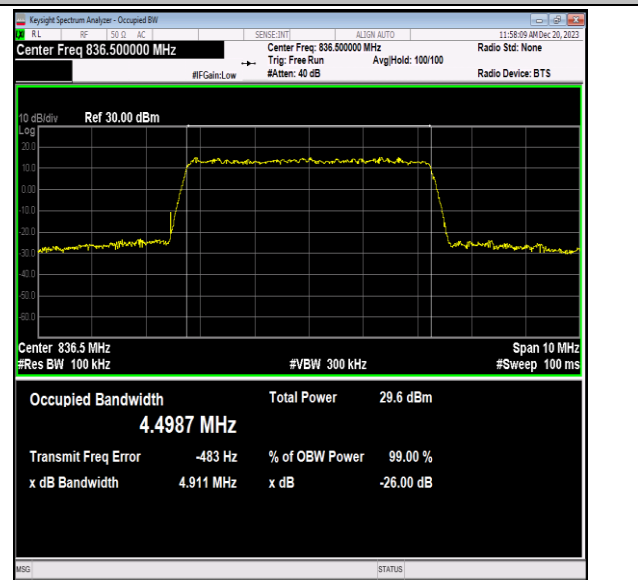
Band5-5MHz-64QAM-20525-25RB#0-PASS
