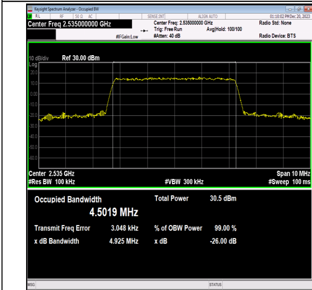
Band7-5MHz-16QAM-21100-25RB#0-PASS
