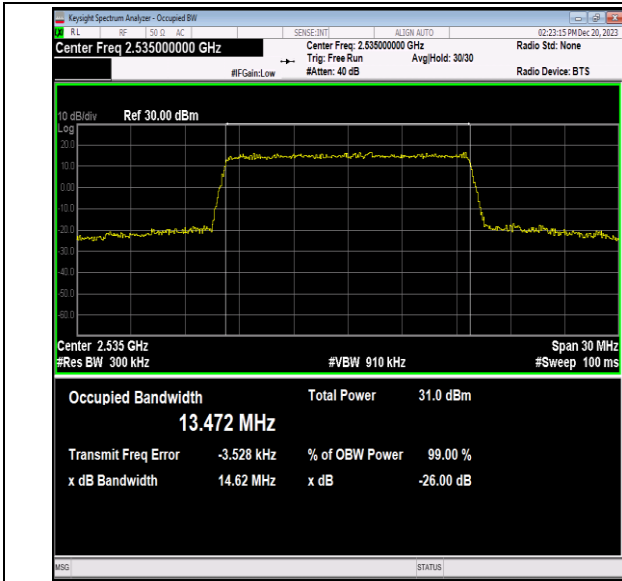
Band7-15MHz-16QAM-21100-75RB#0-PASS
