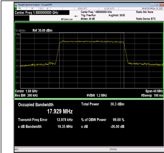
Band2-20MHz-64QAM-18900-100RB#0-PASS
