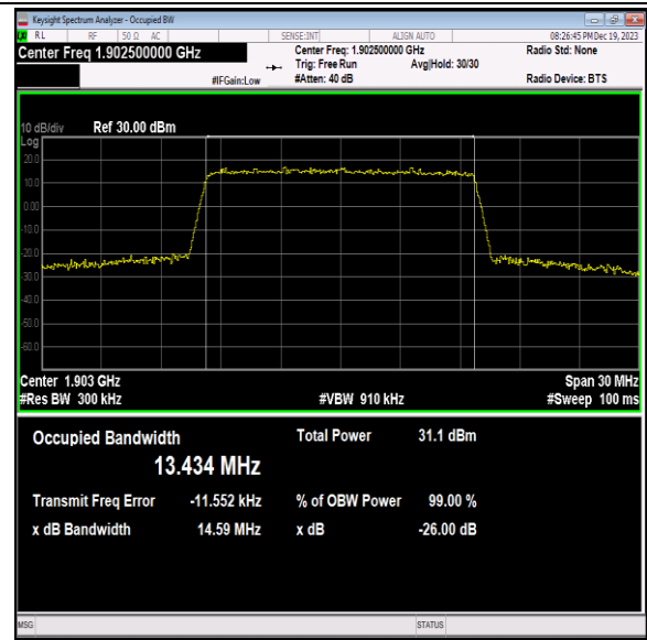
Band2-15MHz-16QAM-19125-75RB#0-PASS
