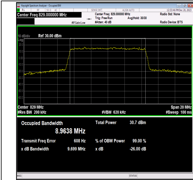
Band5-10MHz-16QAM-20450-50RB#0-PASS
