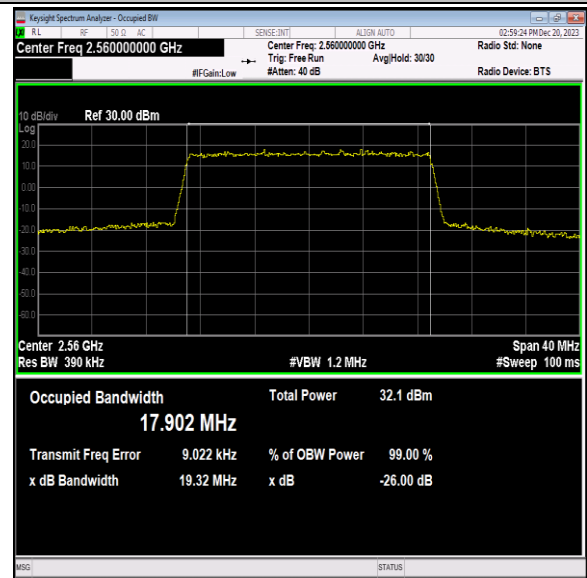
Band7-20MHz-QPSK-21350-100RB#0-PASS
