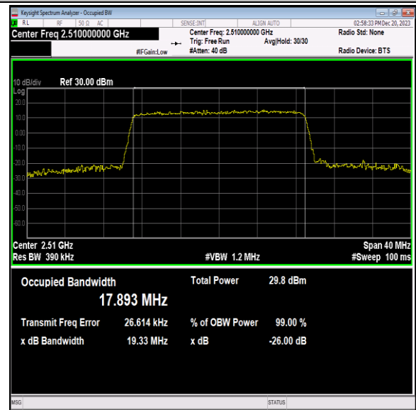
Band7-20MHz-64QAM-20850-100RB#0-PASS
