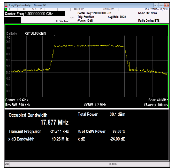
Band2-20MHz-64QAM-19100-100RB#0-PASS
