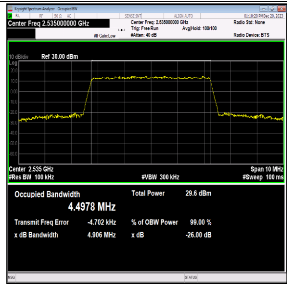
Band7-5MHz-64QAM-21100-25RB#0-PASS
