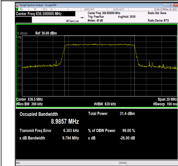
Band5-10MHz-QPSK-20525-50RB#0-PASS
