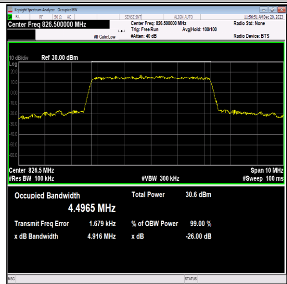
Band5-5MHz-16QAM-20425-25RB#0-PASS
