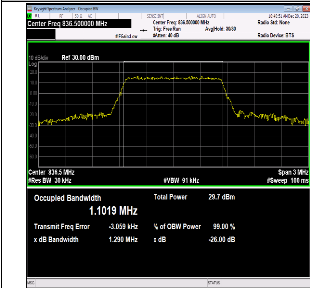
Band5-1.4MHz-16QAM-20525-6RB#0-PASS
