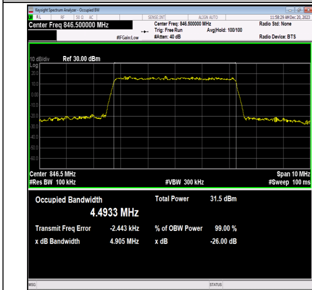
Band5-5MHz-QPSK-20625-25RB#0-PASS
