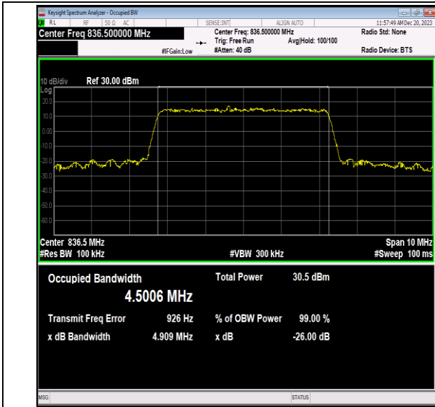
Band5-5MHz-16QAM-20525-25RB#0-PASS
