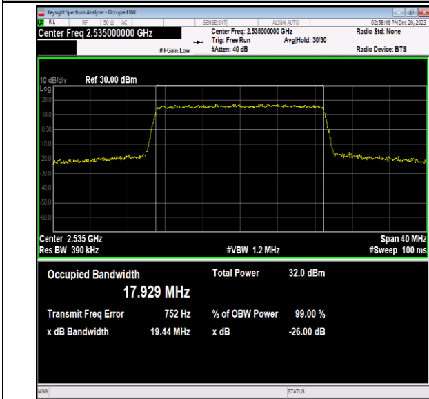
Band7-20MHz-QPSK-21100-100RB#0-PASS
