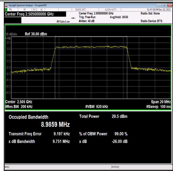
Band7-10MHz-64QAM-20800-50RB#0-PASS
