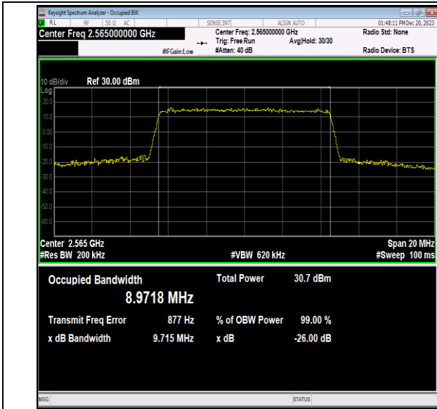
Band7-10MHz-16QAM-21400-50RB#0-PASS
