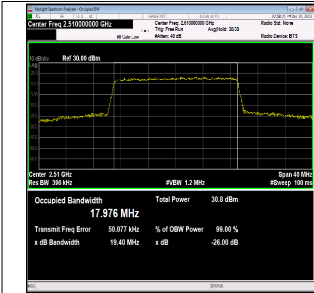
Band7-20MHz-16QAM-20850-100RB#0-PASS
