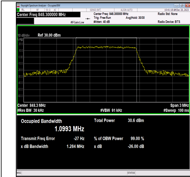
Band5-1.4MHz-QPSK-20643-6RB#0-PASS
