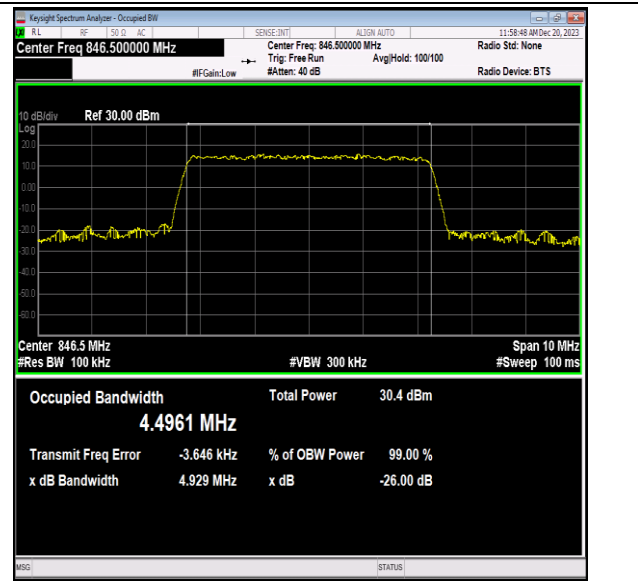
Band5-5MHz-16QAM-20625-25RB#0-PASS
