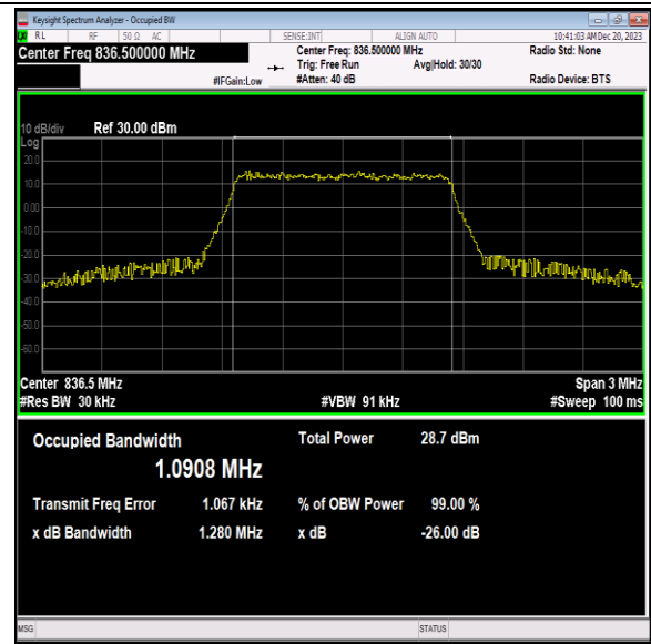
Band5-1.4MHz-64QAM-20525-6RB#0-PASS
