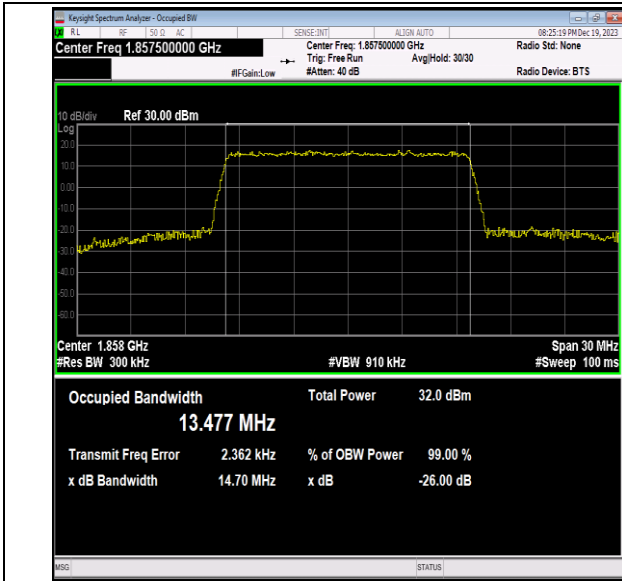
Band2-15MHz-QPSK-18675-75RB#0-PASS
