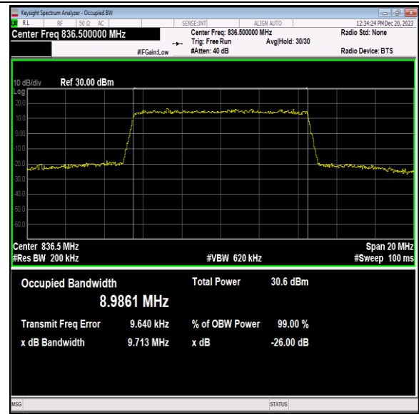
Band5-10MHz-16QAM-20525-50RB#0-PASS
