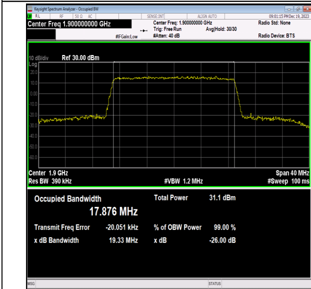
Band2-20MHz-16QAM-19100-100RB#0-PASS
