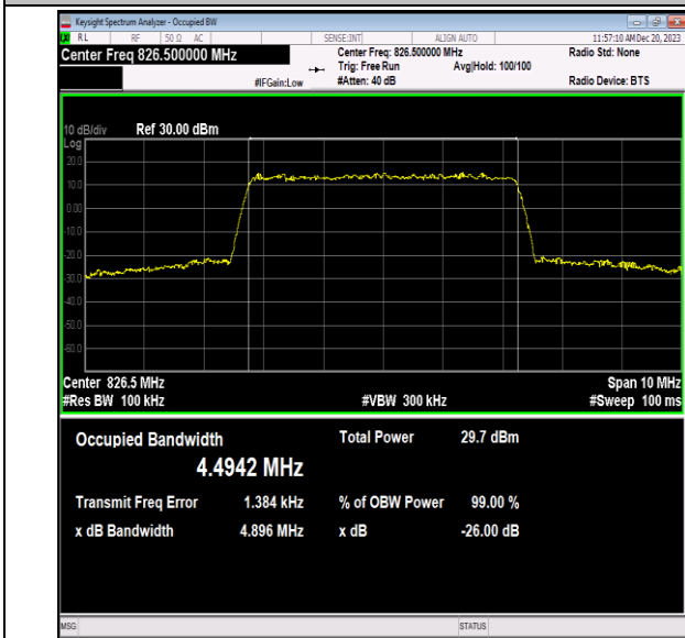
Band5-5MHz-64QAM-20425-25RB#0-PASS
