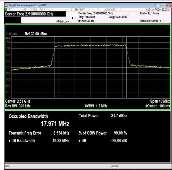
Band7-20MHz-QPSK-20850-100RB#0-PASS
