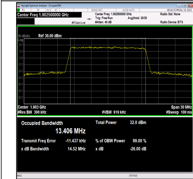
Band2-15MHz-QPSK-19125-75RB#0-PASS
