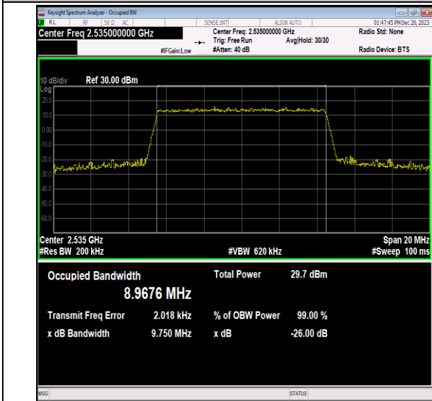
Band7-10MHz-64QAM-21100-50RB#0-PASS
