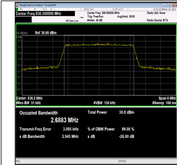
Band5-3MHz-QPSK-20525-15RB#0-PASS
