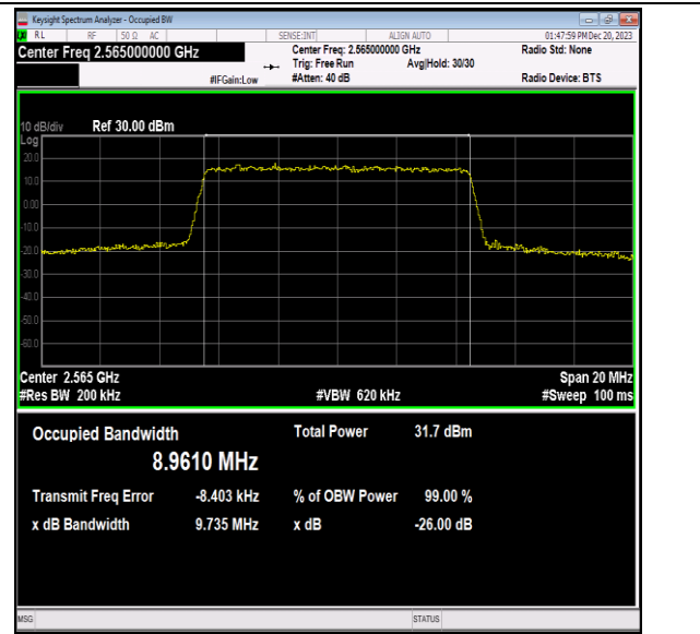
Band7-10MHz-QPSK-21400-50RB#0-PASS
