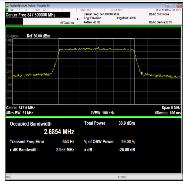
Band5-3MHz-QPSK-20635-15RB#0-PASS
