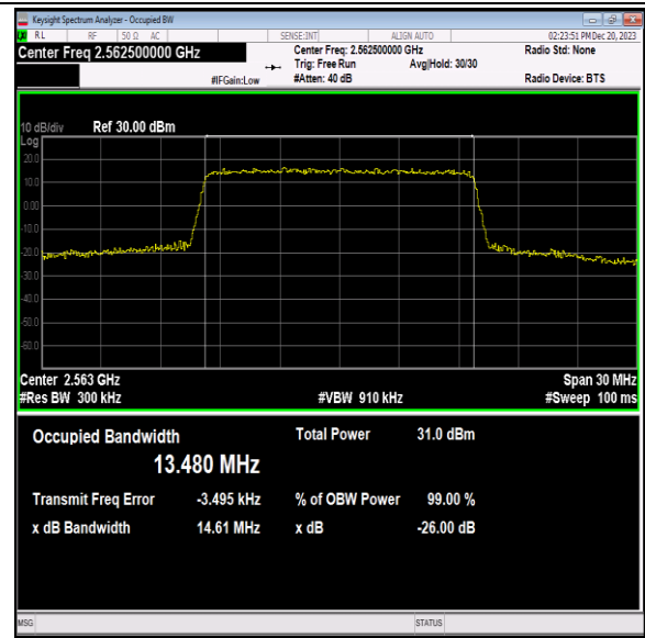
Band7-15MHz-16QAM-21375-75RB#0-PASS
