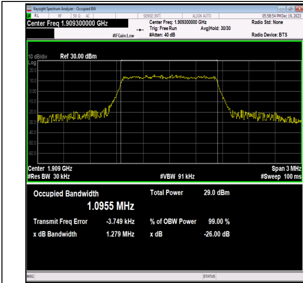
Band2-1.4MHz-64QAM-19193-6RB#0-PASS
