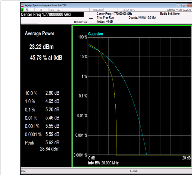
Band66-20MHz-16QAM-132572-1RB#0-PASS
