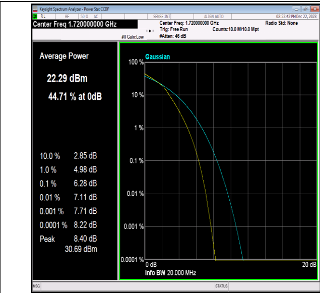
Band66-20MHz-16QAM-132072-100RB#0-PASS
