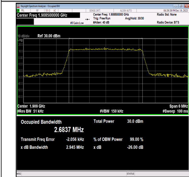
Band2-3MHz-16QAM-19185-15RB#0-PASS
