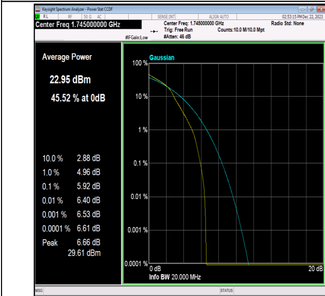
Band66-20MHz-16QAM-132322-1RB#0-PASS
