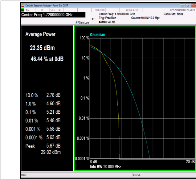
Band66-20MHz-16QAM-132072-1RB#0-PASS
