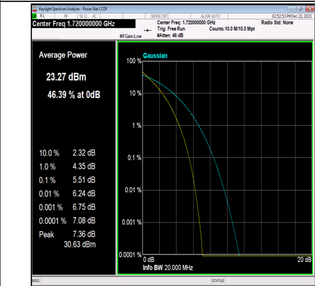
Band66-20MHz-64QAM-132072-100RB#0-PASS
