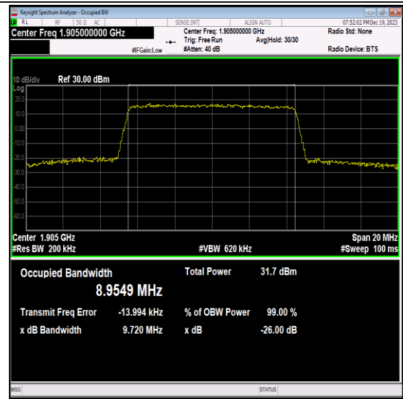
Band2-10MHz-QPSK-19150-50RB#0-PASS
