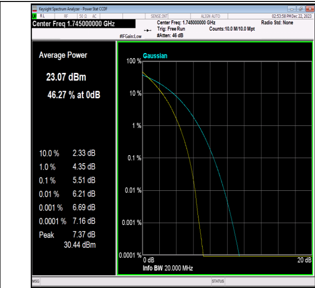
Band66-20MHz-64QAM-132322-100RB#0-PASS
