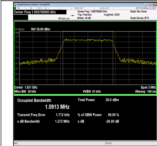
Band2-1.4MHz-64QAM-18607-6RB#0-PASS
