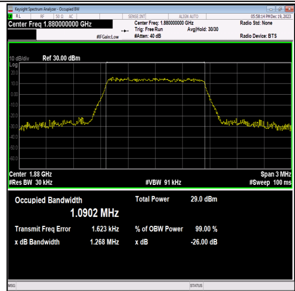
Band2-1.4MHz-64QAM-18900-6RB#0-PASS
