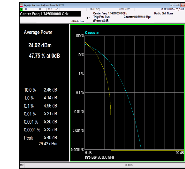
Band66-20MHz-64QAM-132322-1RB#0-PASS
