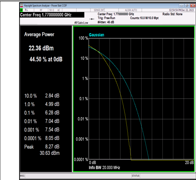
Band66-20MHz-16QAM-132572-100RB#0-PASS
