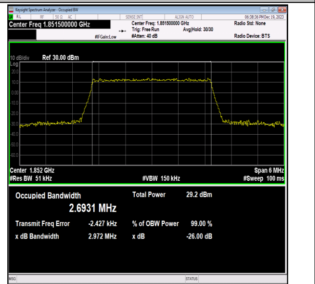
Band2-3MHz-64QAM-18615-15RB#0-PASS
