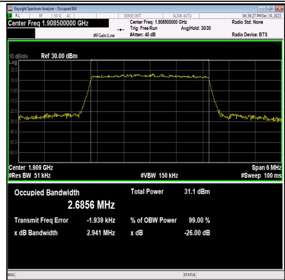
Band2-3MHz-QPSK-19185-15RB#0-PASS
