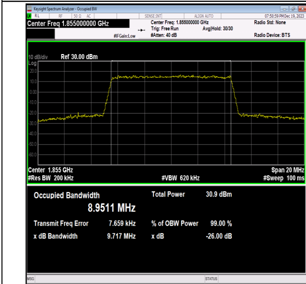
Band2-10MHz-16QAM-18650-50RB#0-PASS
