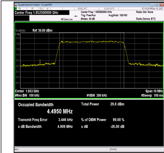
Band2-5MHz-64QAM-18625-25RB#0-PASS
