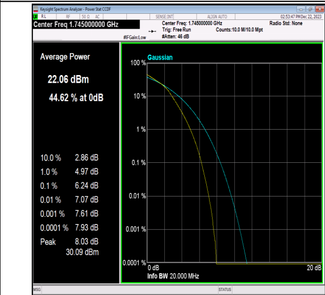
Band66-20MHz-16QAM-132322-100RB#0-PASS
