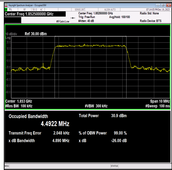
Band2-5MHz-16QAM-18525-25RB#0-PASS
