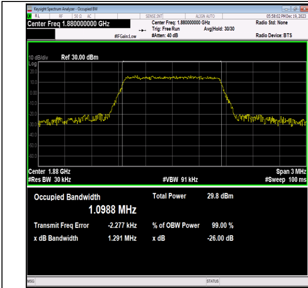
Band2-1.4MHz-16QAM-18900-6RB#0-PASS
