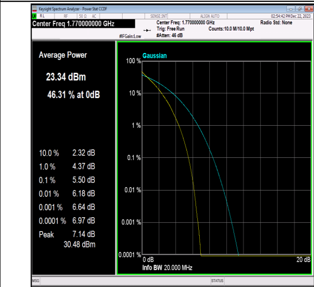
Band66-20MHz-QPSK-132572-100RB#0-PASS
