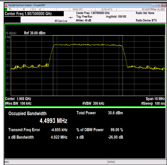
Band2-5MHz-16QAM-19175-25RB#0-PASS
