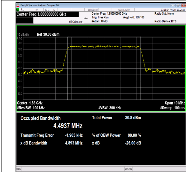
Band2-5MHz-16QAM-18900-25RB#0-PASS
