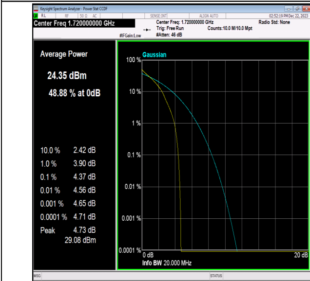
Band66-20MHz-64QAM-132072-1RB#0-PASS
