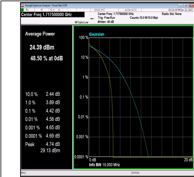
Band66-15MHz-QPSK-132047-1RB#0-PASS
