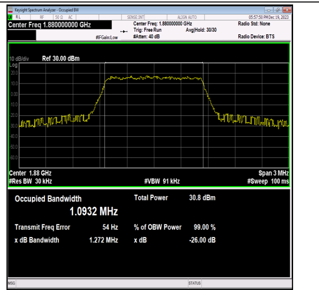
Band2-1.4MHz-QPSK-18900-6RB#0-PASS
