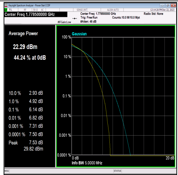
Band66-3MHz-16QAM-132657-15RB#0-PASS
