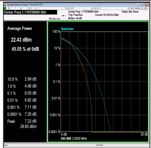
Band66-1.4MHz-16QAM-131979-6RB#0-PASS
