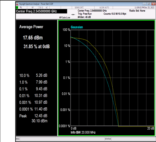
41(2535-2655)-20MHz-64QAM-40140-100RB#0-PASS
