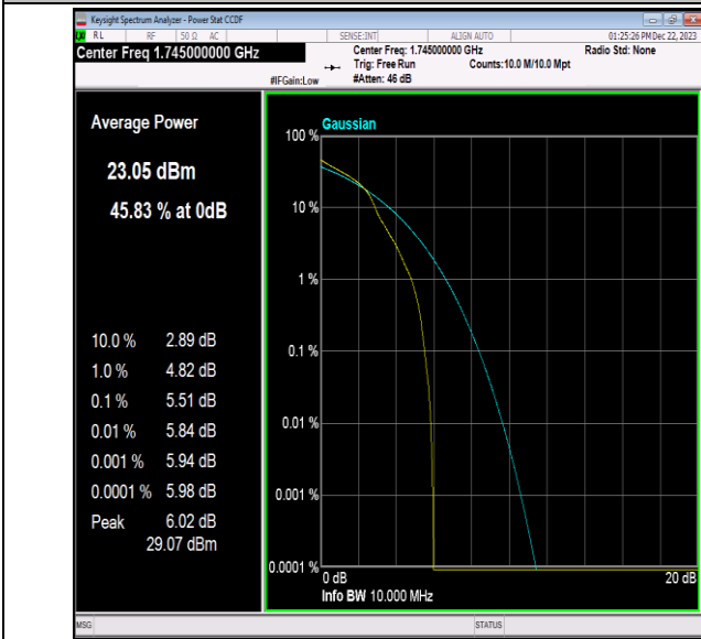
Band66-10MHz-16QAM-132322-1RB#0-PASS
