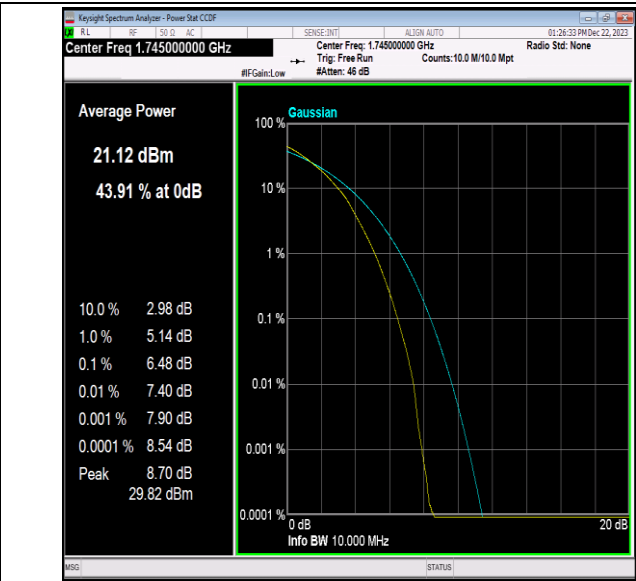
Band66-10MHz-64QAM-132322-50RB#0-PASS
