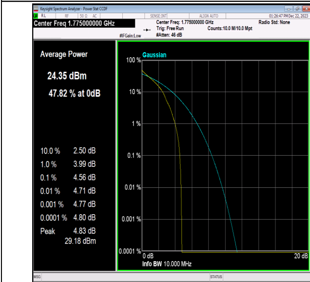
Band66-10MHz-QPSK-132622-1RB#0-PASS
