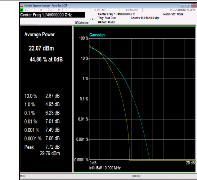
Band66-10MHz-16QAM-132322-50RB#0-PASS
