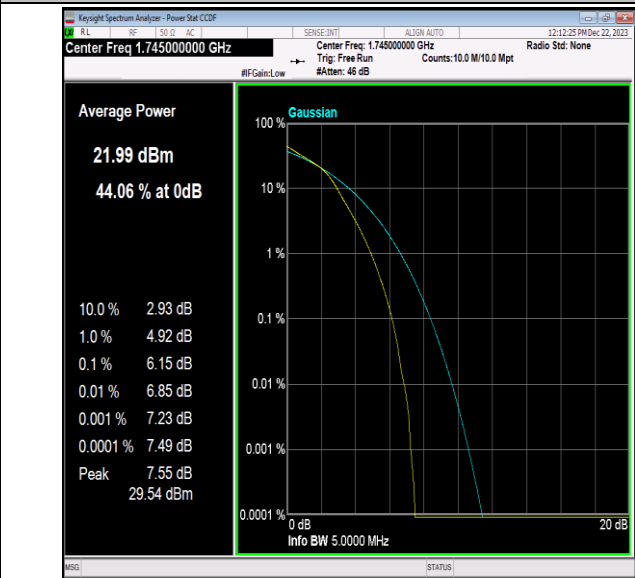
Band66-3MHz-16QAM-132322-15RB#0-PASS
