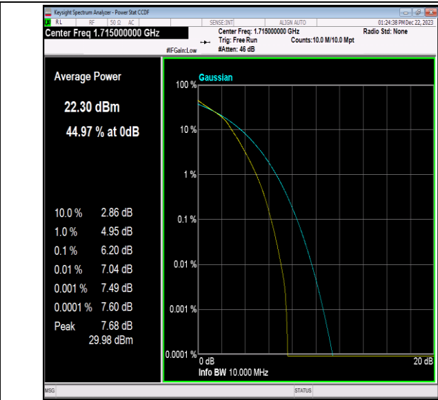
Band66-10MHz-16QAM-132022-50RB#0-PASS
