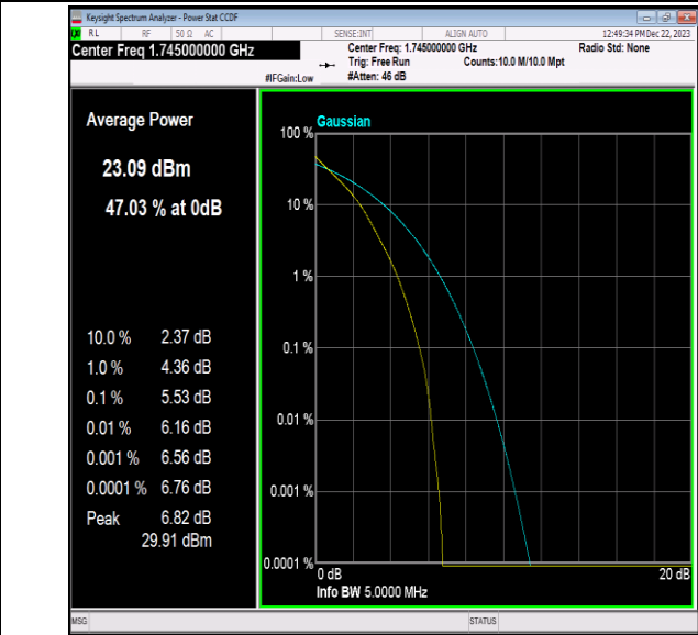
Band66-5MHz-QPSK-132322-25RB#0-PASS
