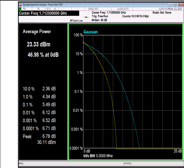
Band66-5MHz-QPSK-131997-25RB#0-PASS
