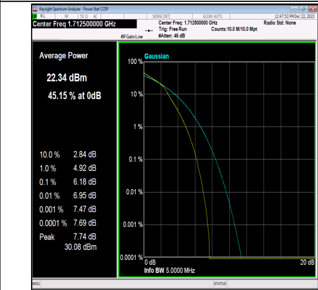
Band66-5MHz-16QAM-131997-25RB#0-PASS
