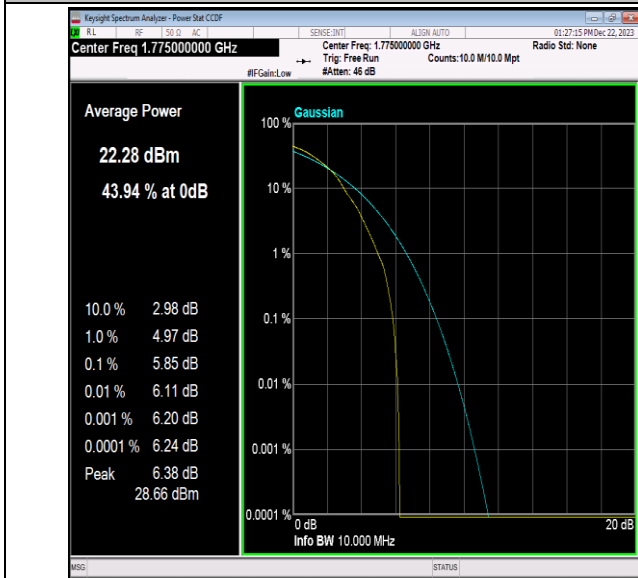
Band66-10MHz-64QAM-132622-1RB#0-PASS
