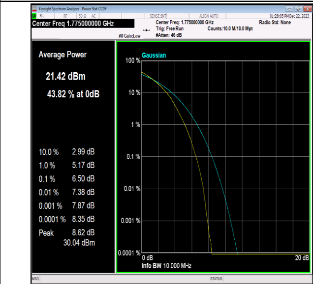
Band66-10MHz-64QAM-132622-50RB#0-PASS
