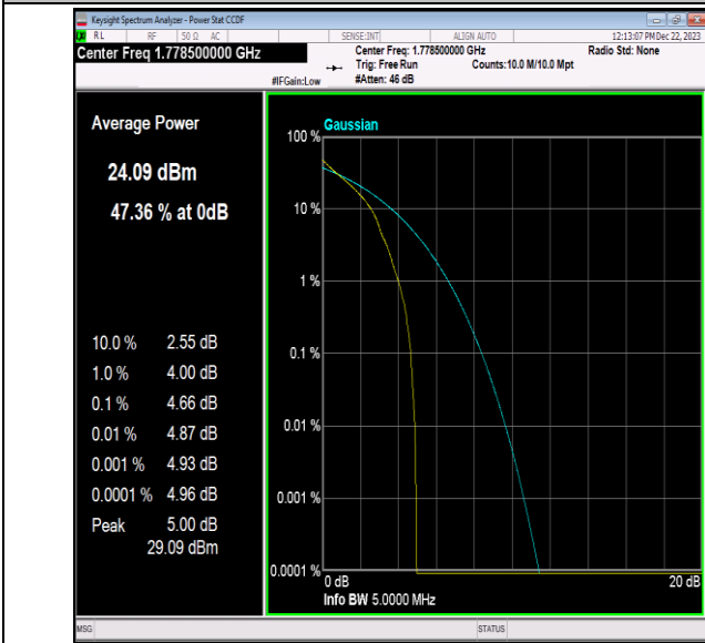
Band66-3MHz-QPSK-132657-1RB#0-PASS
