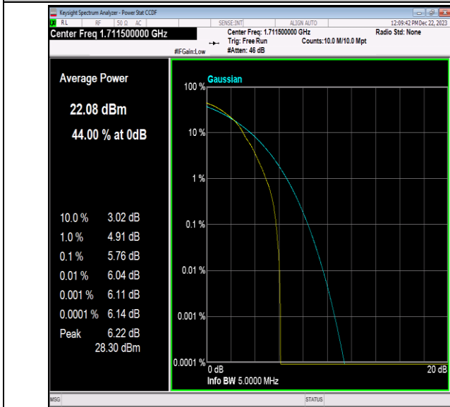
Band66-3MHz-64QAM-131987-1RB#0-PASS
