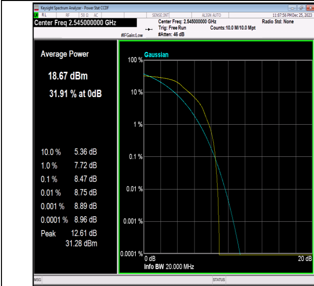
41(2535-2655)-20MHz-64QAM-40140-1RB#0-PASS
