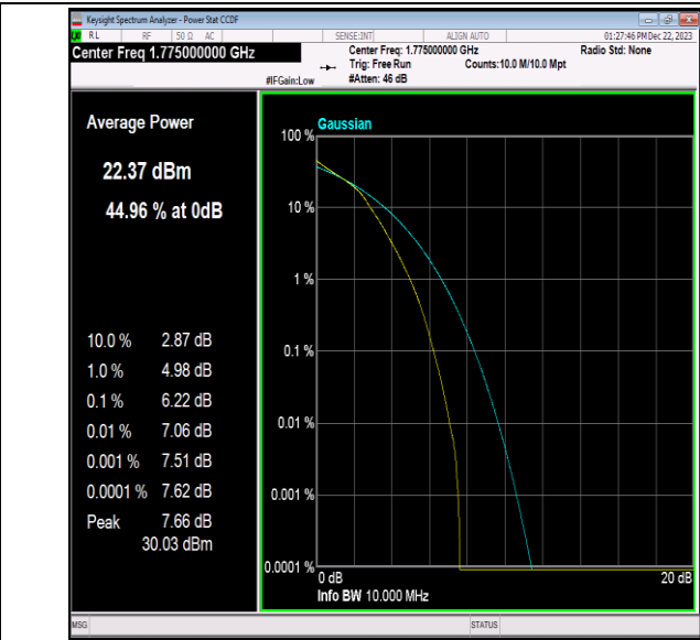
Band66-10MHz-16QAM-132622-50RB#0-PASS
