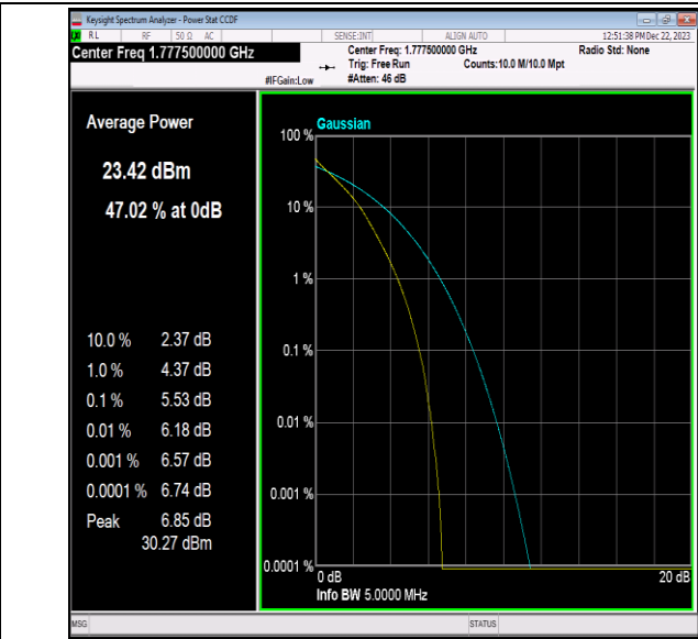
Band66-5MHz-QPSK-132647-25RB#0-PASS
