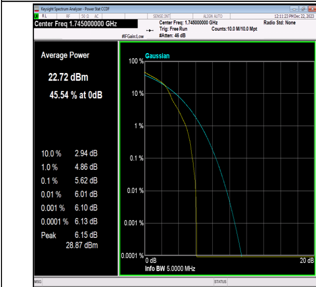
Band66-3MHz-16QAM-132322-1RB#0-PASS
