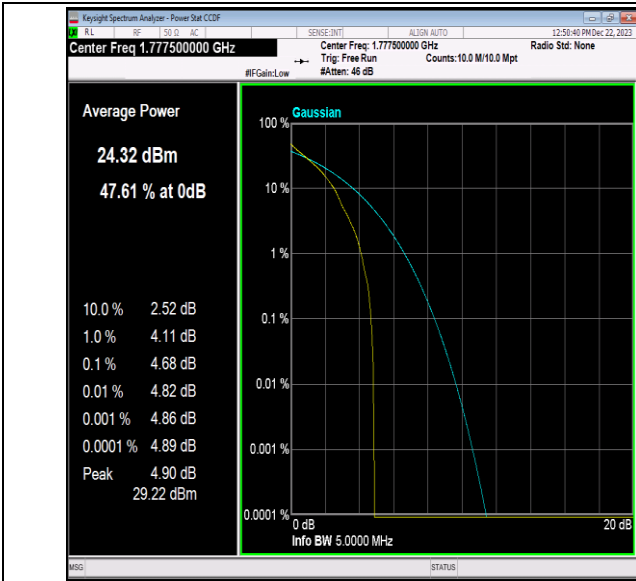
Band66-5MHz-QPSK-132647-1RB#0-PASS
