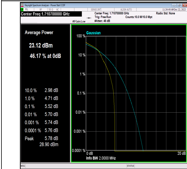
Band66-1.4MHz-16QAM-131979-1RB#0-PASS
