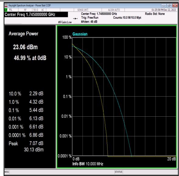
Band66-10MHz-QPSK-132322-50RB#0-PASS
