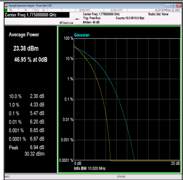
Band66-10MHz-QPSK-132622-50RB#0-PASS
