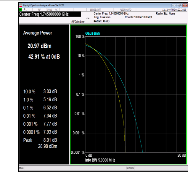
Band66-3MHz-64QAM-132322-15RB#0-PASS
