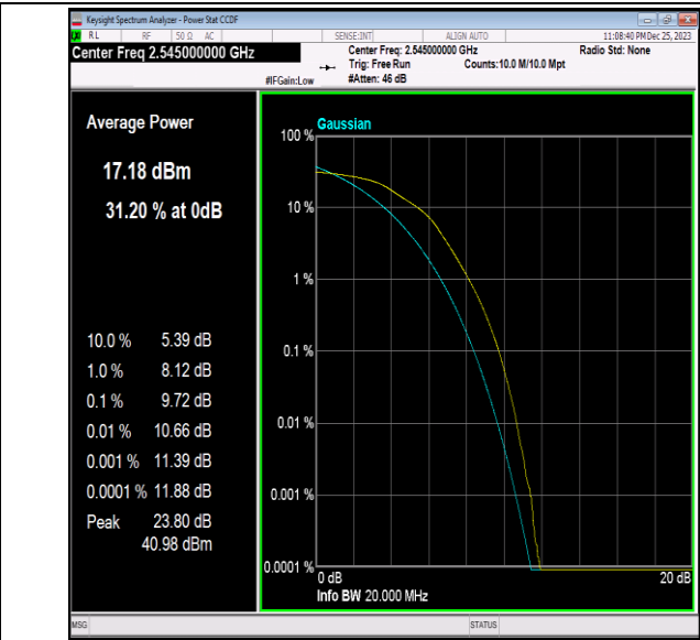
41(2535-2655)-20MHz-16QAM-40140-100RB#0-PASS
