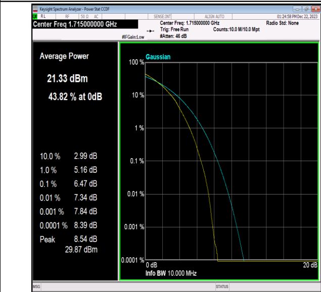
Band66-10MHz-64QAM-132022-50RB#0-PASS
