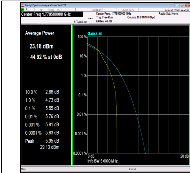
Band66-3MHz-16QAM-132657-1RB#0-PASS
