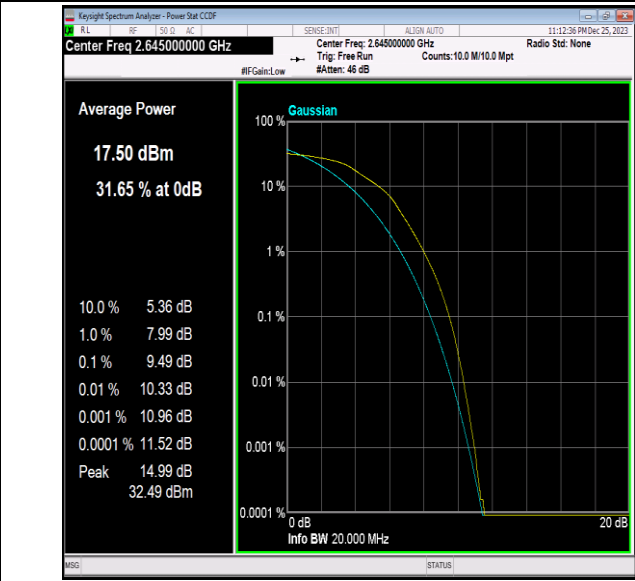
41(2535-2655)-20MHz-16QAM-41140-100RB#0-PASS
