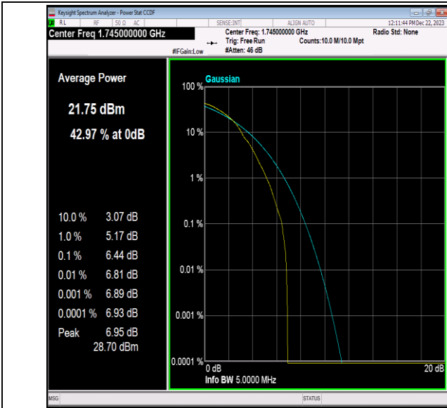
Band66-3MHz-64QAM-132322-1RB#0-PASS
