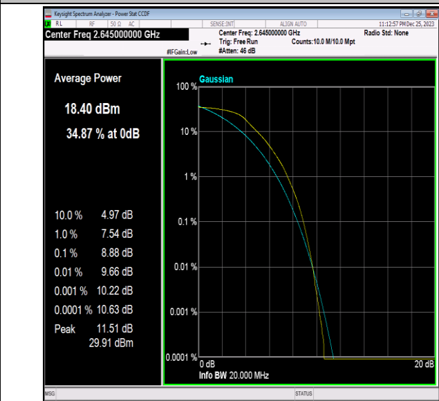
41(2535-2655)-20MHz-64QAM-41140-100RB#0-PASS
