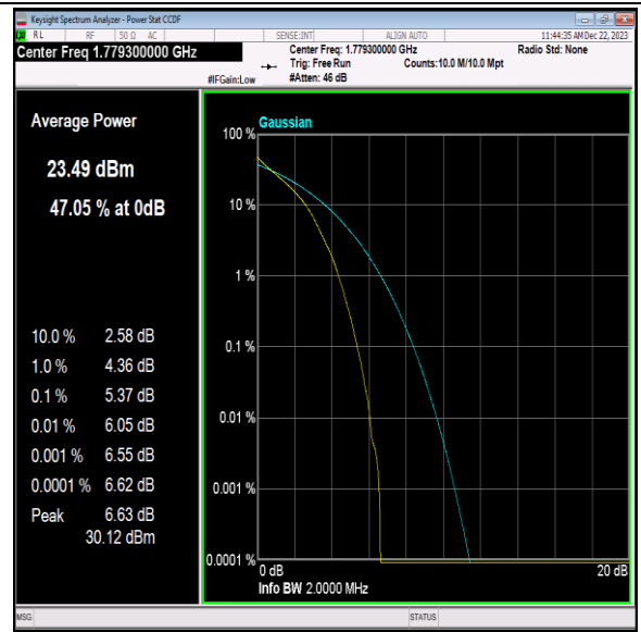
Band66-1.4MHz-QPSK-132665-6RB#0-PASS
