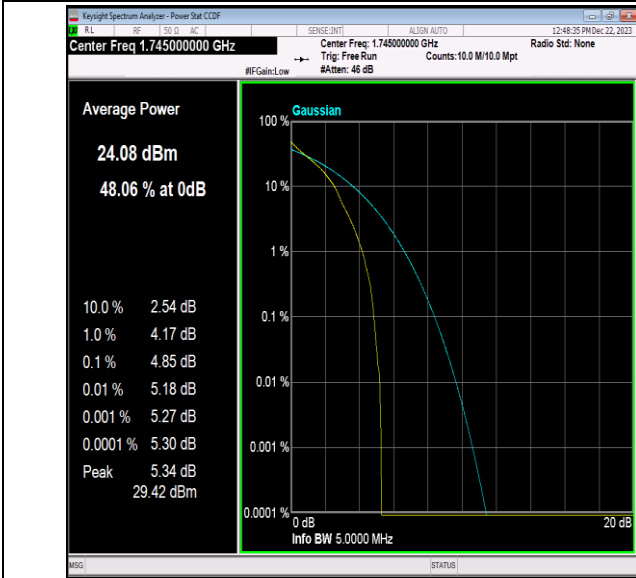
Band66-5MHz-QPSK-132322-1RB#0-PASS
