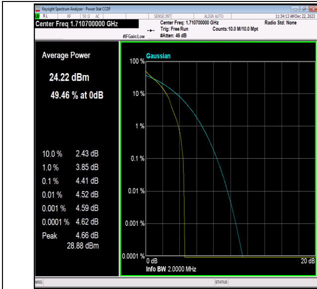
Band66-1.4MHz-QPSK-131979-1RB#0-PASS
