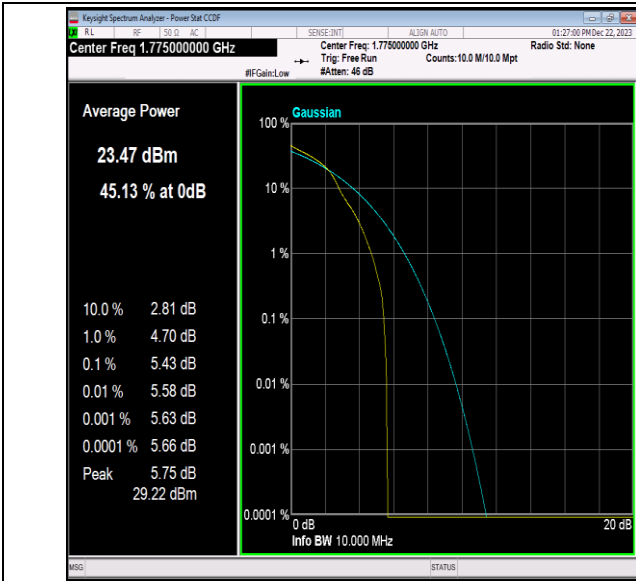
Band66-10MHz-16QAM-132622-1RB#0-PASS
