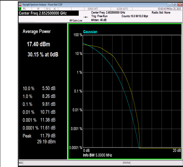
41(2535-2655)-5MHz-16QAM-41215-25RB#0-PASS
