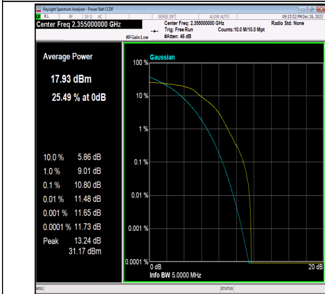
40(2350-2360)-5MHz-64QAM-39200-1RB#0-PASS
