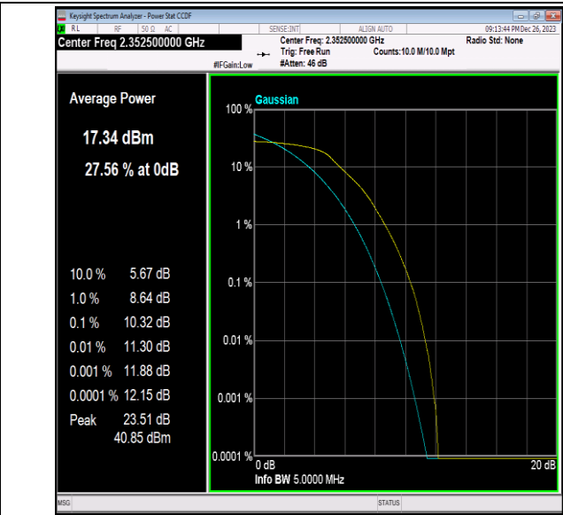
40(2350-2360)-5MHz-64QAM-39175-25RB#0-PASS
