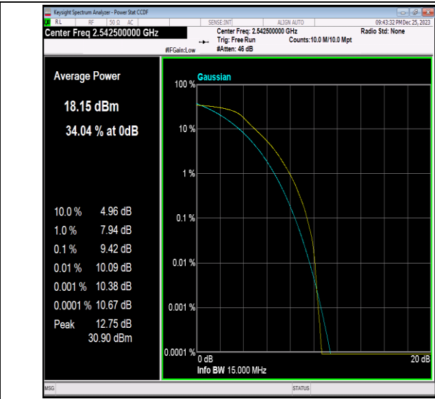
41(2535-2655)-15MHz-QPSK-40115-75RB#0-PASS
