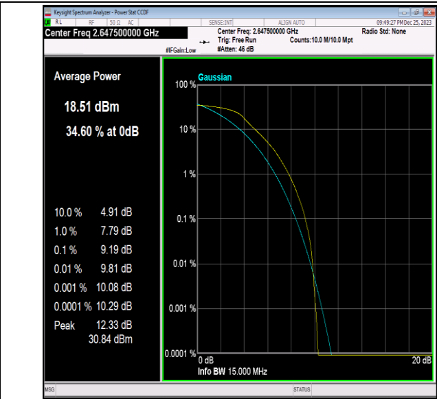
41(2535-2655)-15MHz-64QAM-41165-75RB#0-PASS
