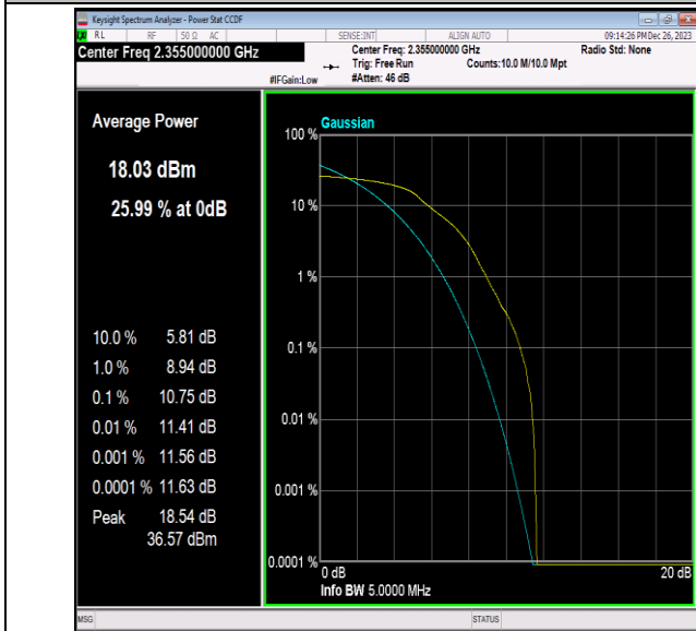
40(2350-2360)-5MHz-QPSK-39200-1RB#0-PASS
