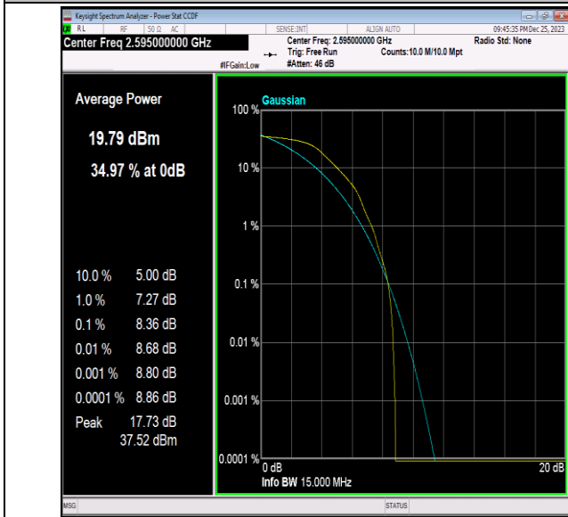
41(2535-2655)-15MHz-64QAM-40640-1RB#0-PASS
