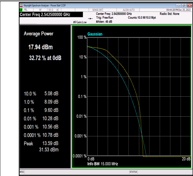
41(2535-2655)-15MHz-64QAM-40115-75RB#0-PASS
