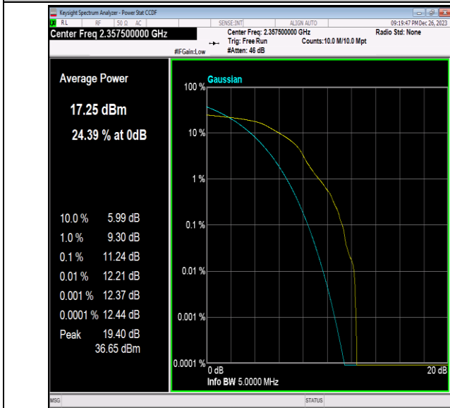
40(2350-2360)-5MHz-16QAM-39225-1RB#0-PASS
