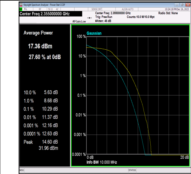
40(2350-2360)-10MHz-64QAM-39200-50RB#0-PASS
