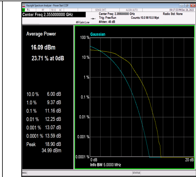
40(2350-2360)-5MHz-16QAM-39200-25RB#0-PASS
