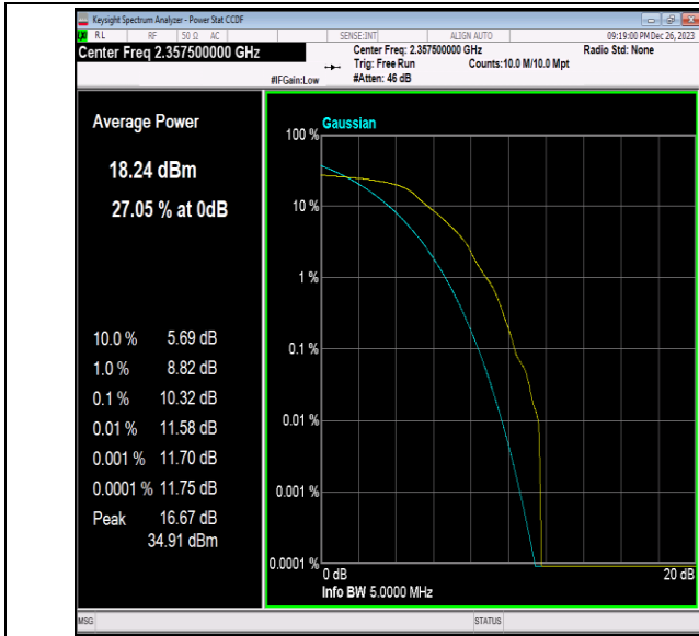
40(2350-2360)-5MHz-QPSK-39225-1RB#0-PASS
