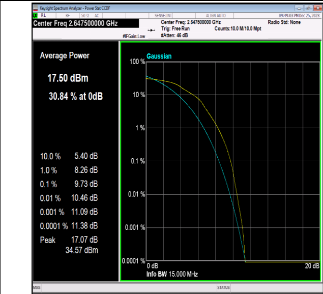
41(2535-2655)-15MHz-16QAM-41165-75RB#0-PASS
