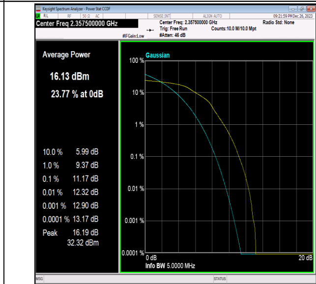
40(2350-2360)-5MHz-16QAM-39225-25RB#0-PASS
