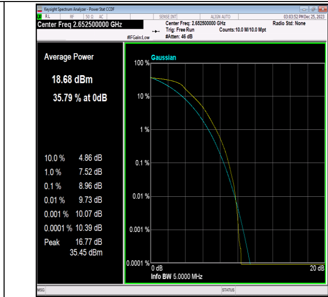
41(2535-2655)-5MHz-64QAM-41215-25RB#0-PASS
