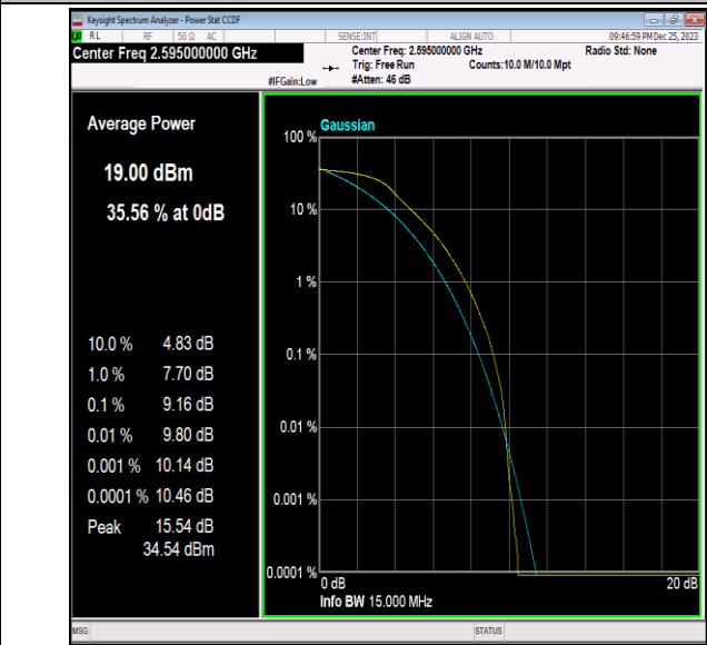
41(2535-2655)-15MHz-64QAM-40640-75RB#0-PASS
