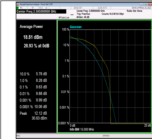
41(2535-2655)-15MHz-16QAM-40640-1RB#0-PASS
