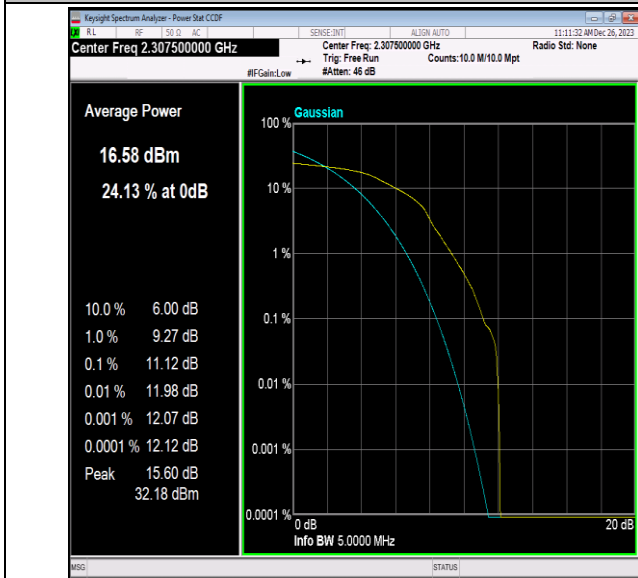
40(2305-2315)-5MHz-16QAM-38725-1RB#0-PASS
