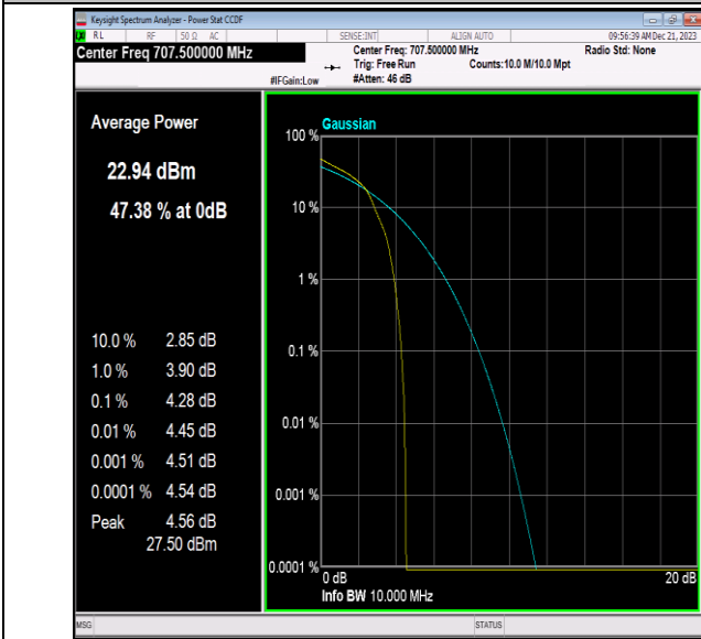
Band12-10MHz-16QAM-23095-1RB#0-PASS
