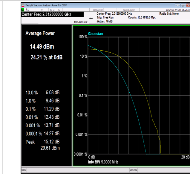
40(2305-2315)-5MHz-64QAM-38775-25RB#0-PASS
