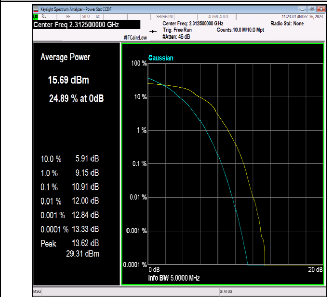
40(2305-2315)-5MHz-16QAM-38775-25RB#0-PASS
