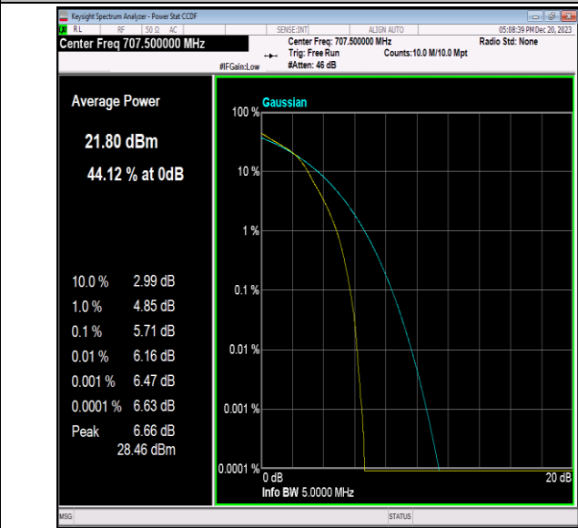
Band12-3MHz-16QAM-23095-15RB#0-PASS
