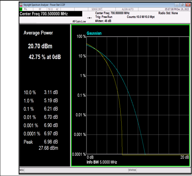
Band12-3MHz-64QAM-23025-15RB#0-PASS
