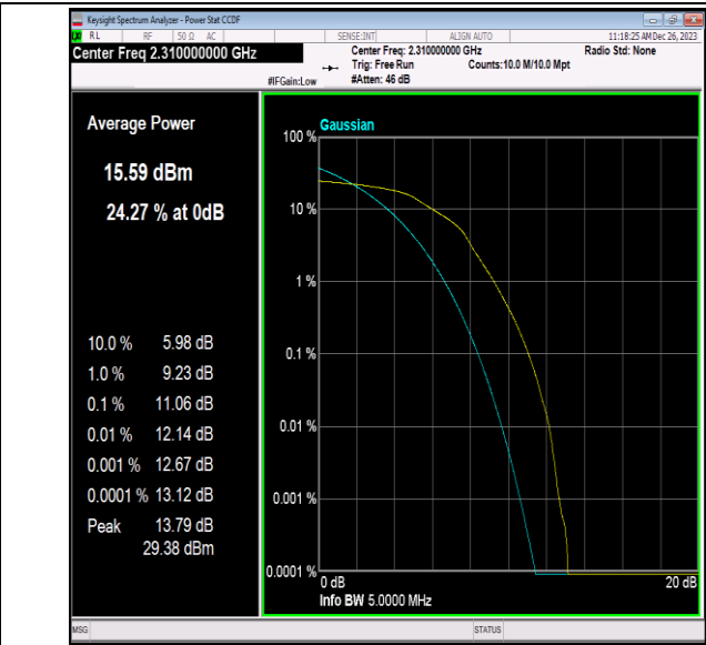
40(2305-2315)-5MHz-16QAM-38750-25RB#0-PASS
