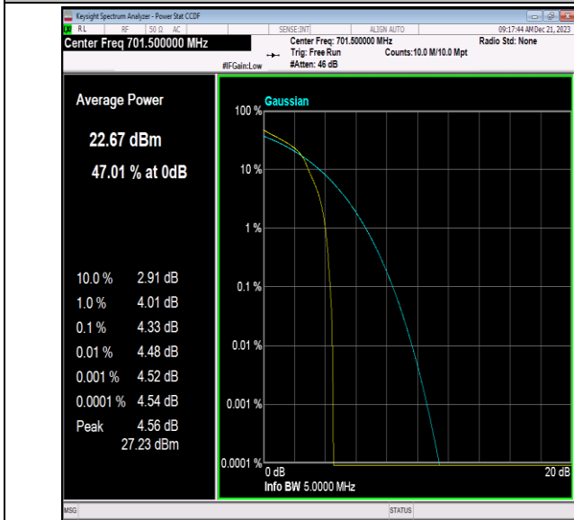
Band12-5MHz-16QAM-23035-1RB#0-PASS
