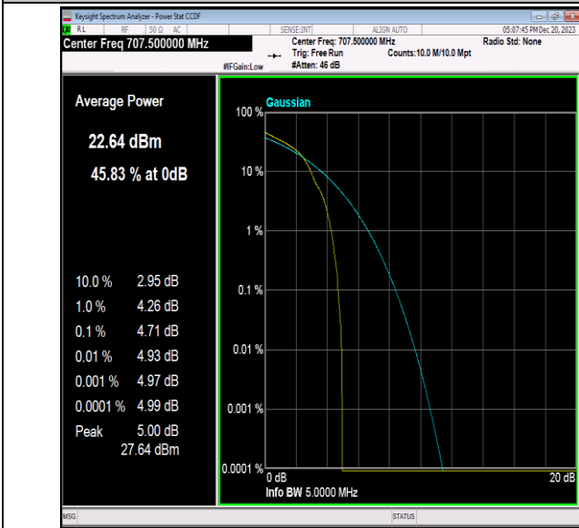
Band12-3MHz-16QAM-23095-1RB#0-PASS
