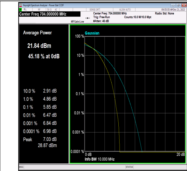
Band12-10MHz-16QAM-23060-50RB#0-PASS
