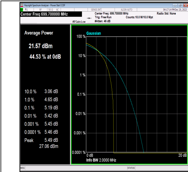
Band12-1.4MHz-64QAM-23017-1RB#0-PASS
