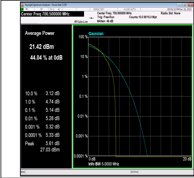
Band12-3MHz-64QAM-23025-1RB#0-PASS
