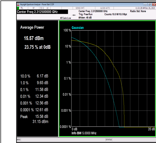
40(2305-2315)-5MHz-64QAM-38775-1RB#0-PASS
