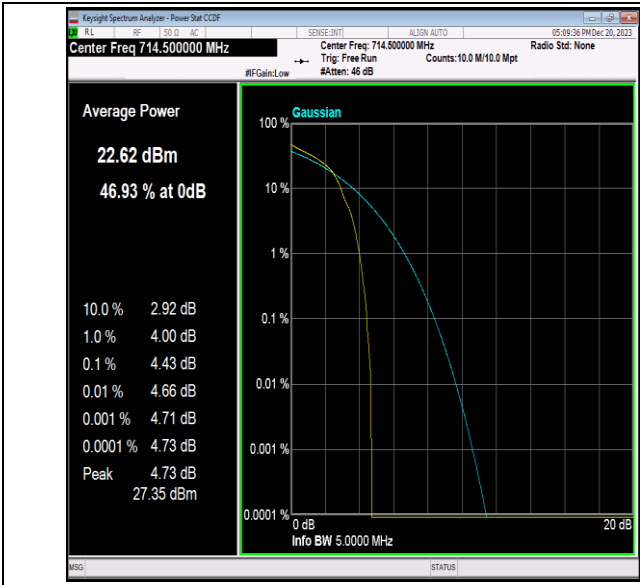
Band12-3MHz-16QAM-23165-1RB#0-PASS
