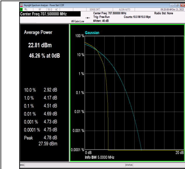
Band12-5MHz-16QAM-23095-1RB#0-PASS
