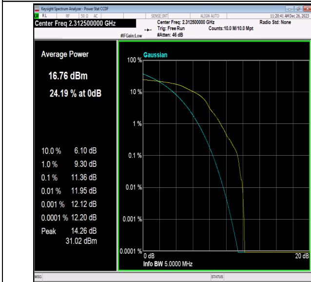
40(2305-2315)-5MHz-16QAM-38775-1RB#0-PASS
