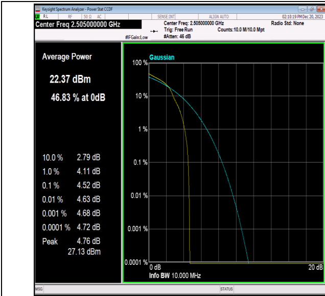
Band7-10MHz-16QAM-20800-1RB#0-PASS
