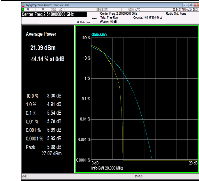
Band7-20MHz-64QAM-20850-1RB#0-PASS
