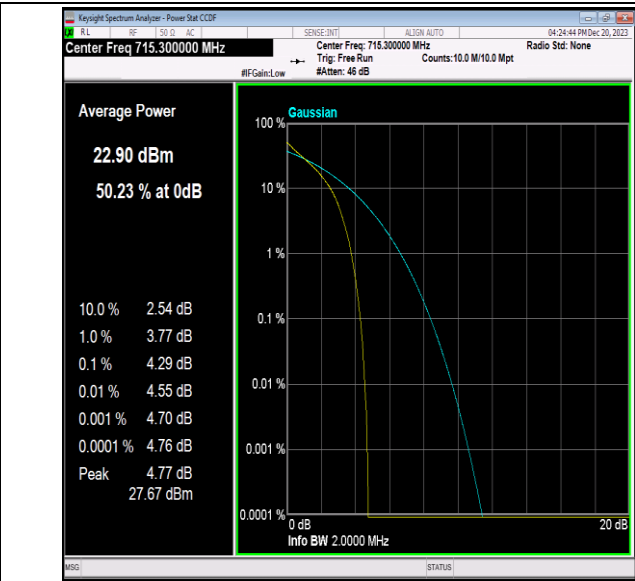
Band12-1.4MHz-QPSK-23173-6RB#0-PASS
