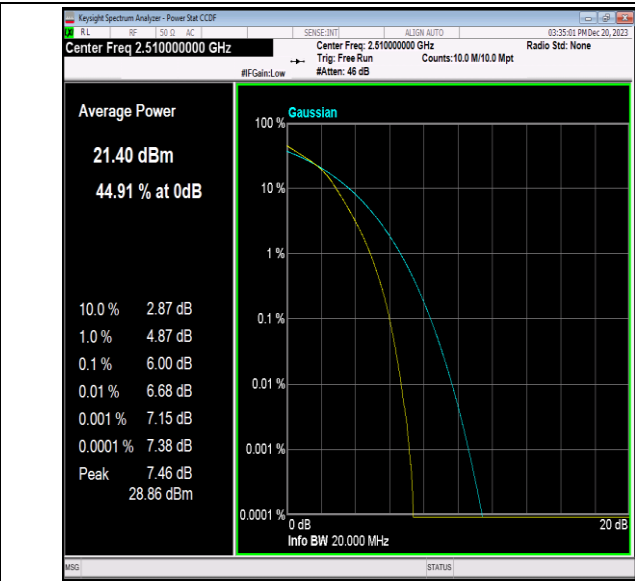
Band7-20MHz-16QAM-20850-100RB#0-PASS
