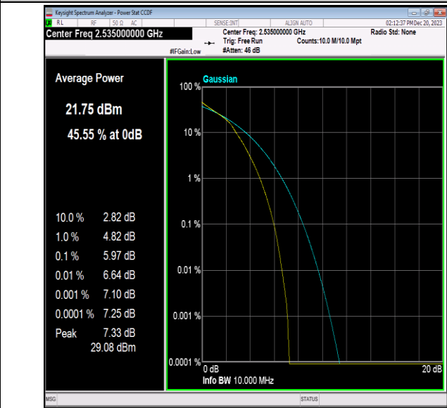
Band7-10MHz-16QAM-21100-50RB#0-PASS
