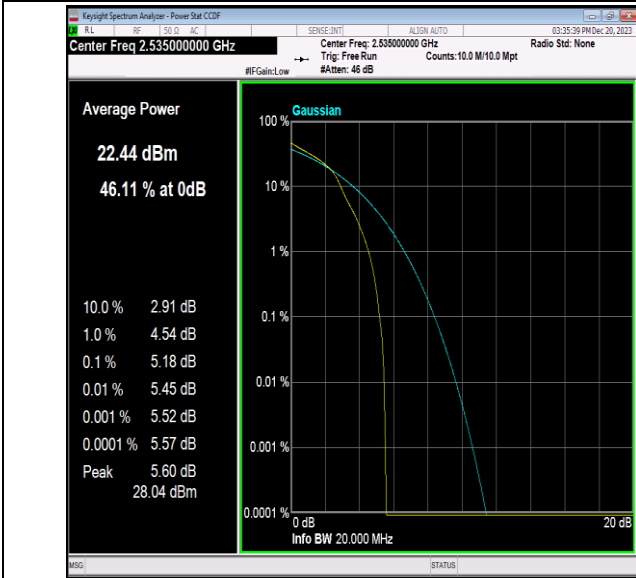
Band7-20MHz-16QAM-21100-1RB#0-PASS
