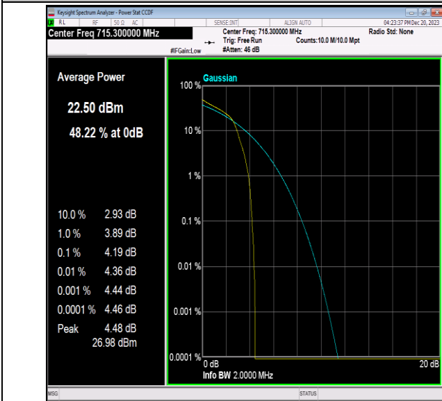
Band12-1.4MHz-16QAM-23173-1RB#0-PASS
