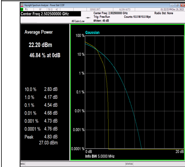
Band7-5MHz-16QAM-20775-1RB#0-PASS
