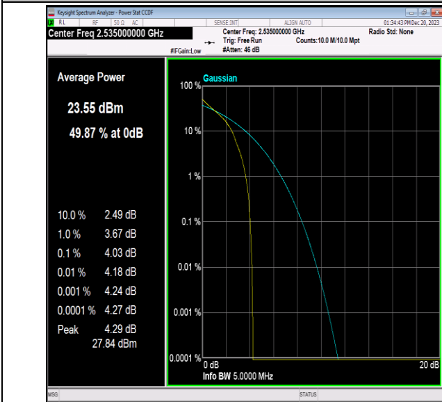
Band7-5MHz-QPSK-21100-1RB#0-PASS
