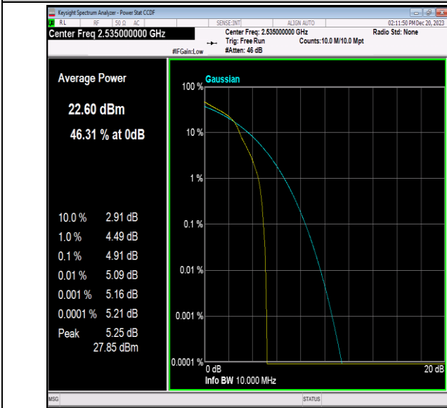
Band7-10MHz-16QAM-21100-1RB#0-PASS
