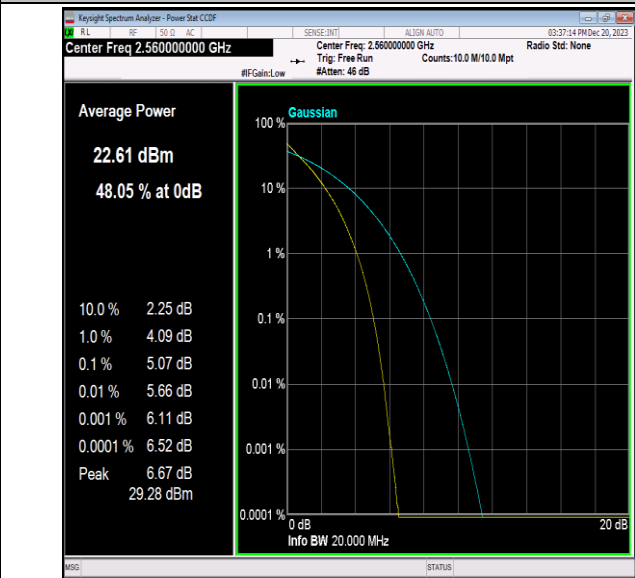
Band7-20MHz-QPSK-21350-100RB#0-PASS
