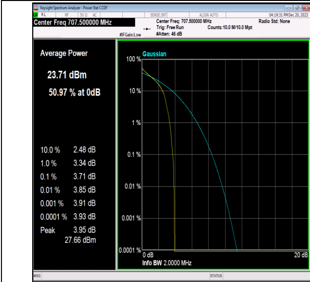
Band12-1.4MHz-QPSK-23095-1RB#0-PASS
