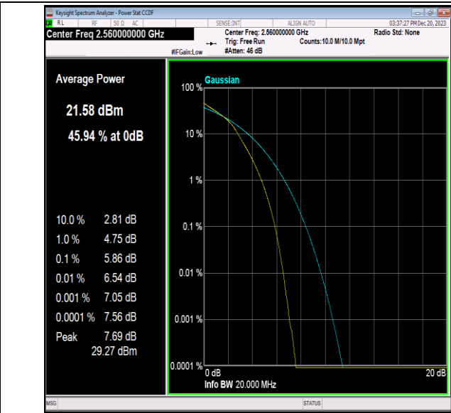
Band7-20MHz-16QAM-21350-100RB#0-PASS
