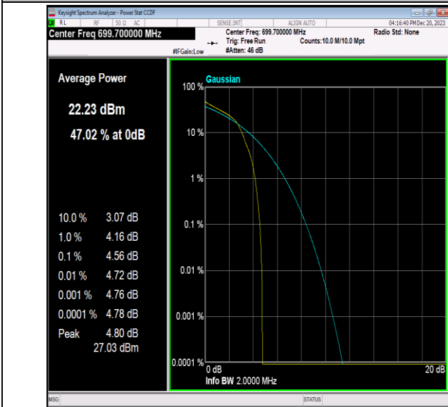
Band12-1.4MHz-16QAM-23017-1RB#0-PASS
