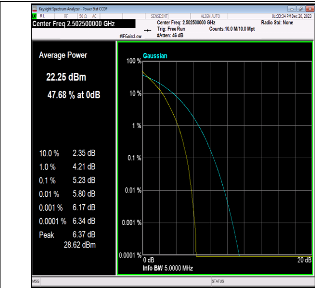
Band7-5MHz-QPSK-20775-25RB#0-PASS
