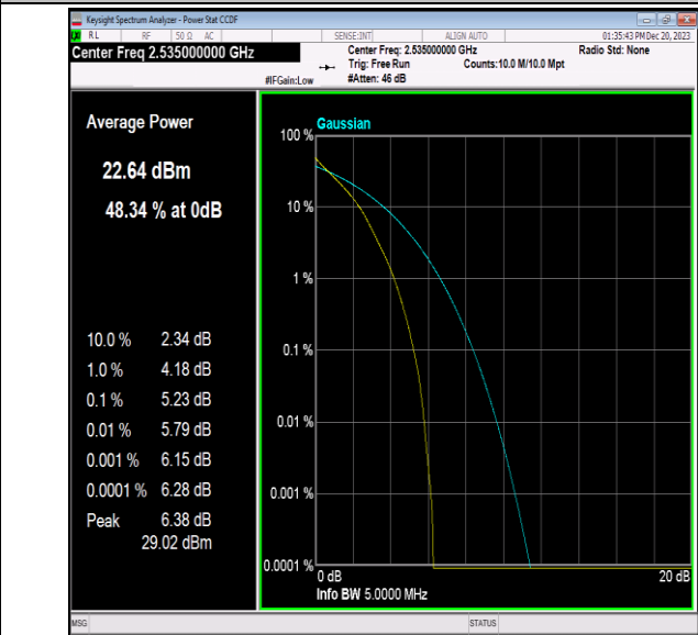
Band7-5MHz-QPSK-21100-25RB#0-PASS
