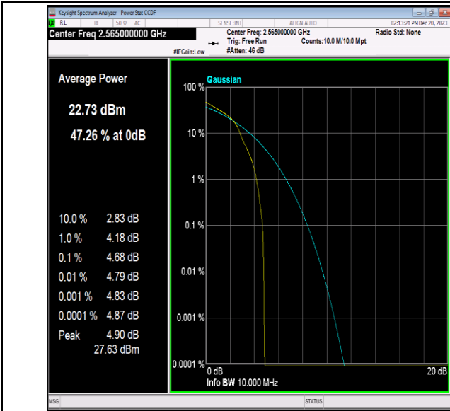
Band7-10MHz-16QAM-21400-1RB#0-PASS
