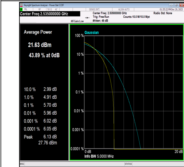
Band7-5MHz-64QAM-21100-1RB#0-PASS
