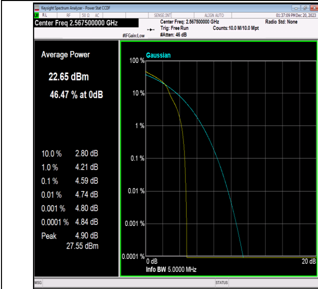
Band7-5MHz-16QAM-21425-1RB#0-PASS
