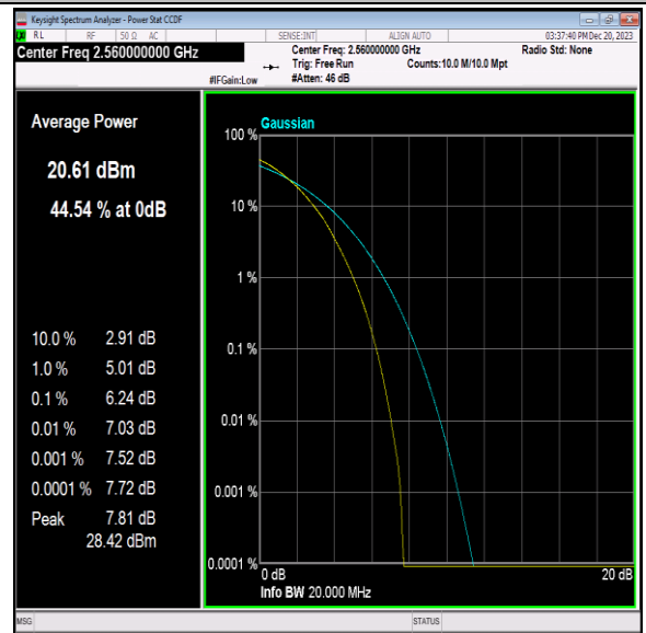
Band7-20MHz-64QAM-21350-100RB#0-PASS
