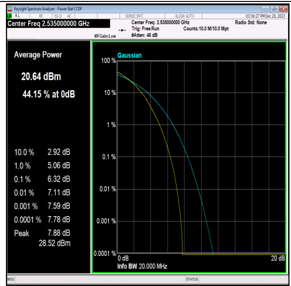
Band7-20MHz-64QAM-21100-100RB#0-PASS
