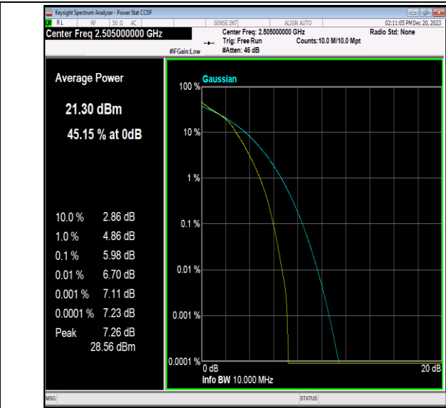
Band7-10MHz-16QAM-20800-50RB#0-PASS
