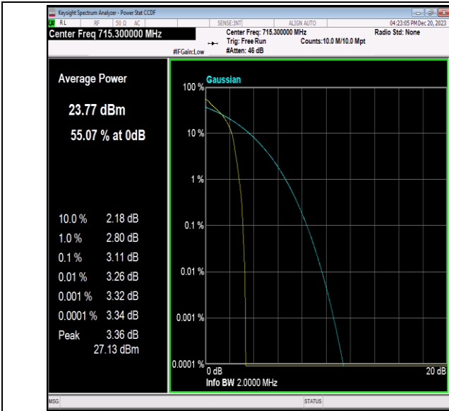
Band12-1.4MHz-QPSK-23173-1RB#0-PASS
