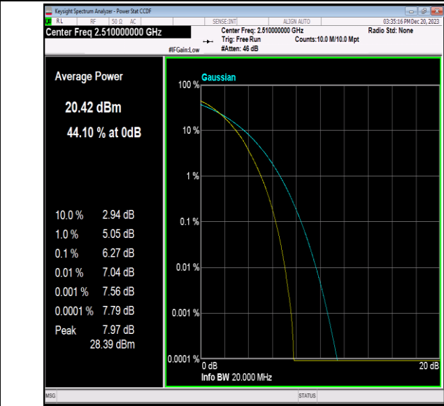
Band7-20MHz-64QAM-20850-100RB#0-PASS
