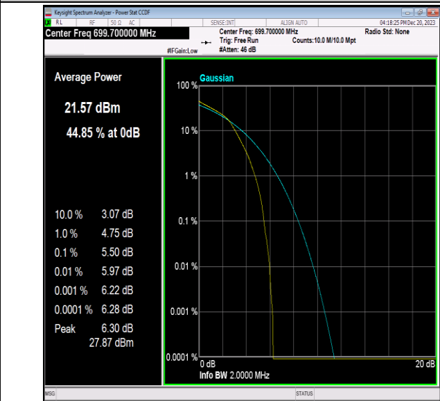
Band12-1.4MHz-16QAM-23017-6RB#0-PASS
