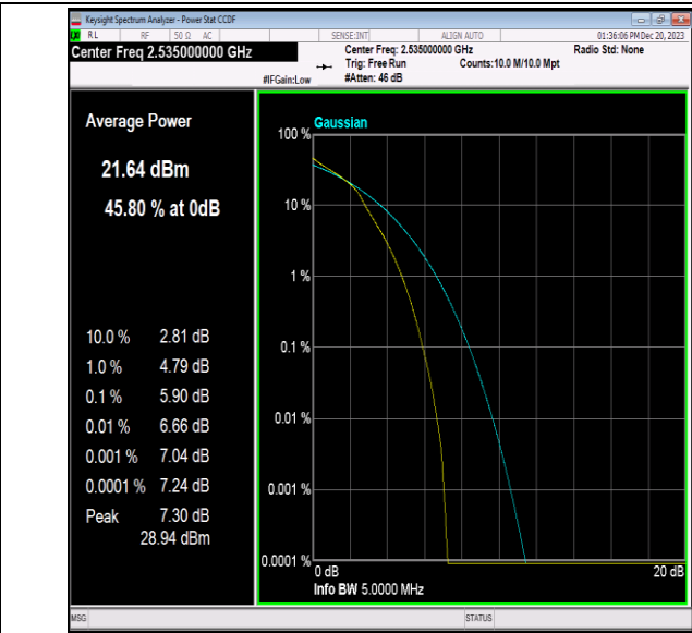
Band7-5MHz-16QAM-21100-25RB#0-PASS
