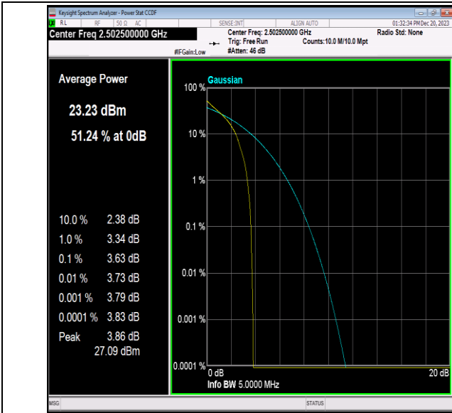
Band7-5MHz-QPSK-20775-1RB#0-PASS
