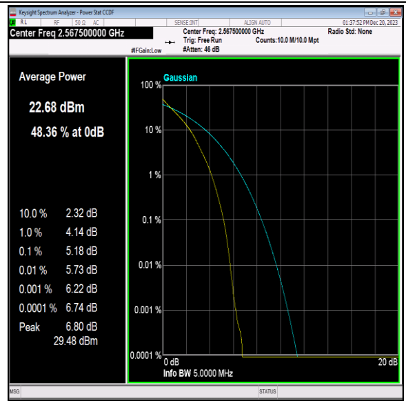
Band7-5MHz-QPSK-21425-25RB#0-PASS
