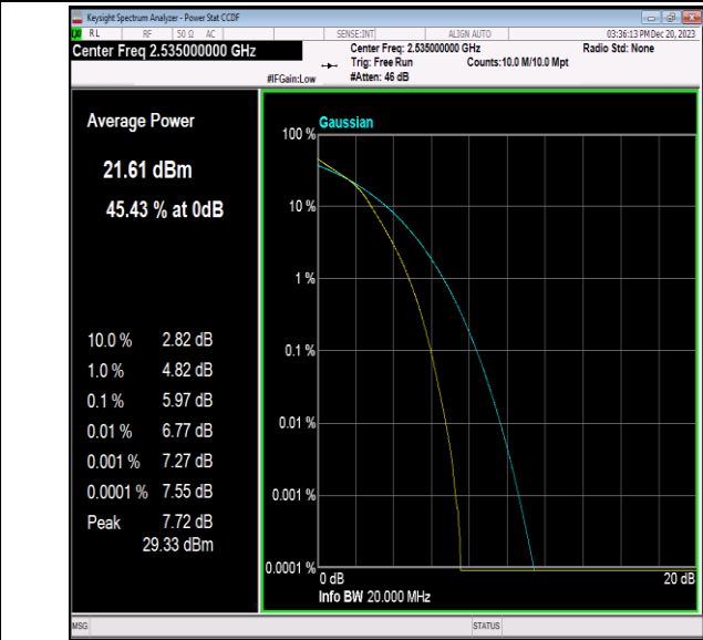
Band7-20MHz-16QAM-21100-100RB#0-PASS
