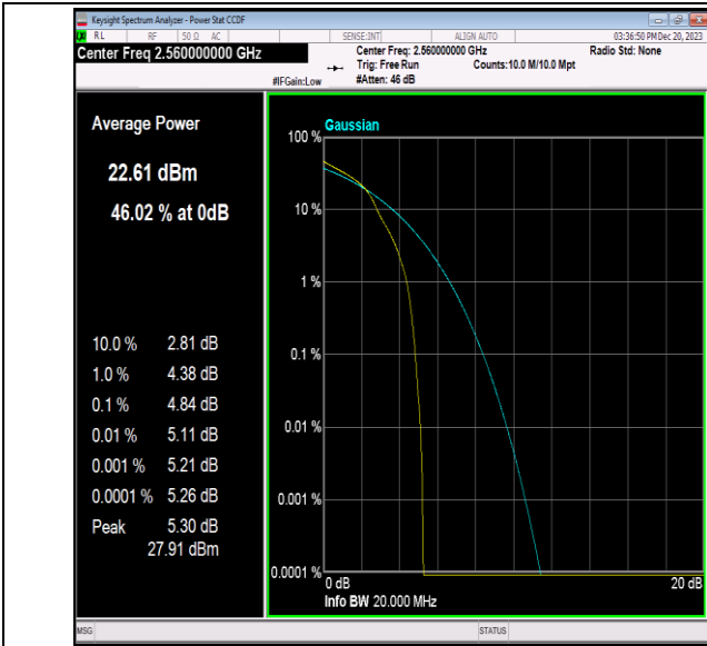
Band7-20MHz-16QAM-21350-1RB#0-PASS
