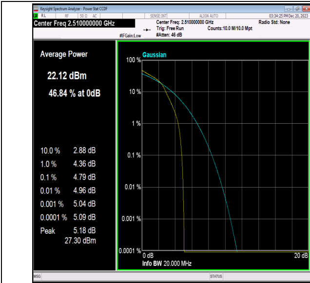
Band7-20MHz-16QAM-20850-1RB#0-PASS
